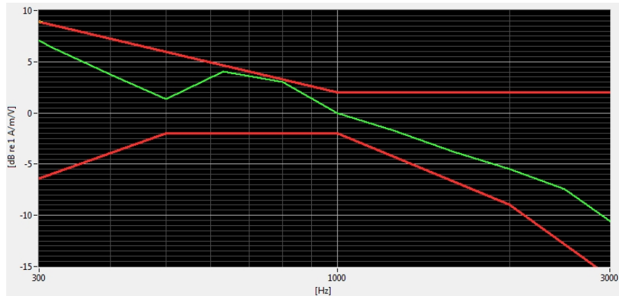
Figure 7-1 Axial Frequency Response
