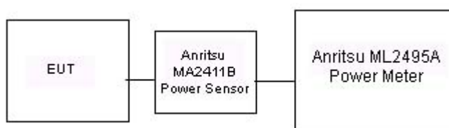
Figure 8-3 Power Measurement Setup for Bandwidths < 50 MHz
