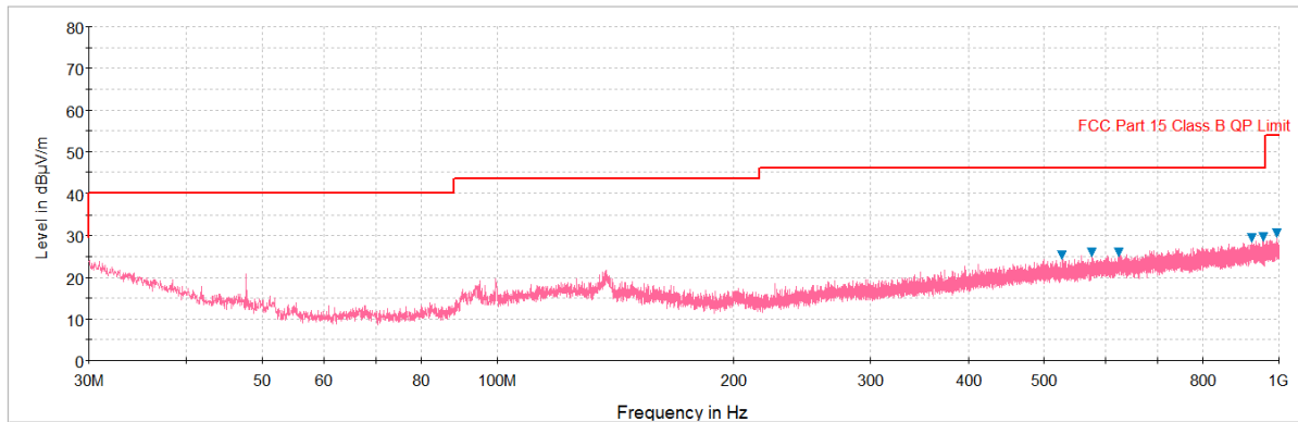
Plot 6-20. Radiated Spurious Plot below 1GHz (Pol. H)
