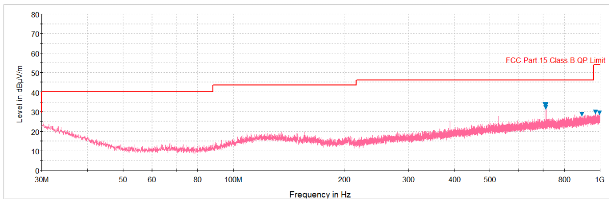
Plot 6-21. Radiated Spurious Plot below 1GHz (Pol. V)
