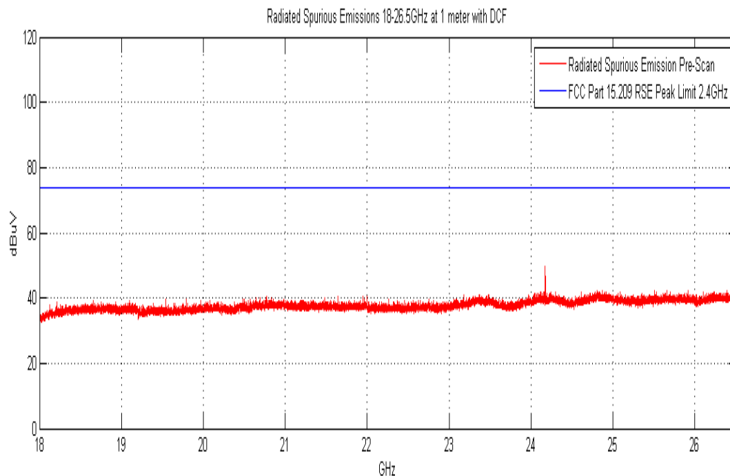
Plot 6-49. Radiated Spurious Plot above 18GHz (Pol. V)
