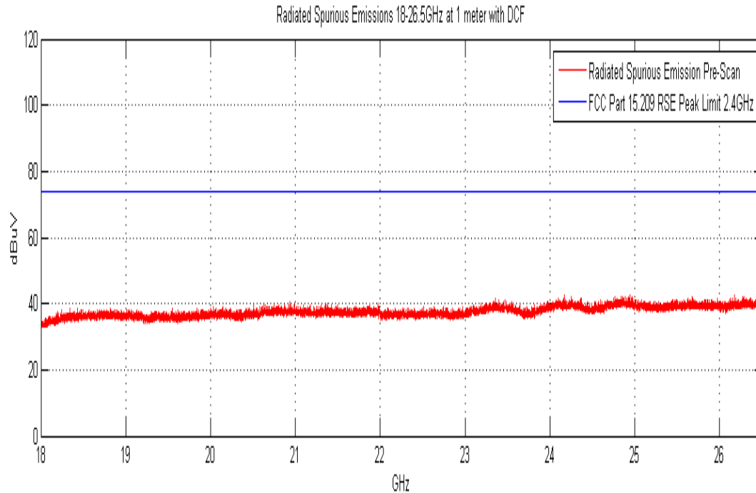
Plot 6-48. Radiated Spurious Plot above 18GHz (Pol. H)
