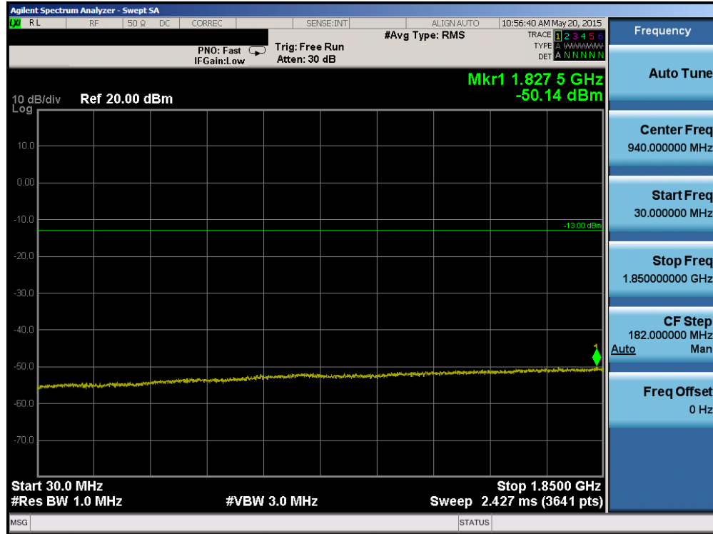
Plot 6-35. Conducted Spurious Plot (PCS WCDMA Mode – Ch. 9400)
