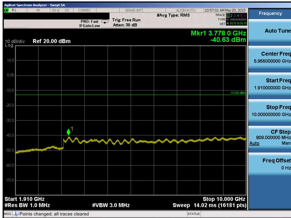
Plot 6-36. Conducted Spurious Plot (PCS WCDMA Mode – Ch. 9400)
