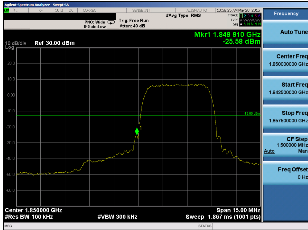
Plot 6-49. Band Edge Plot (PCS WCDMA Mode – Ch. 9262)
