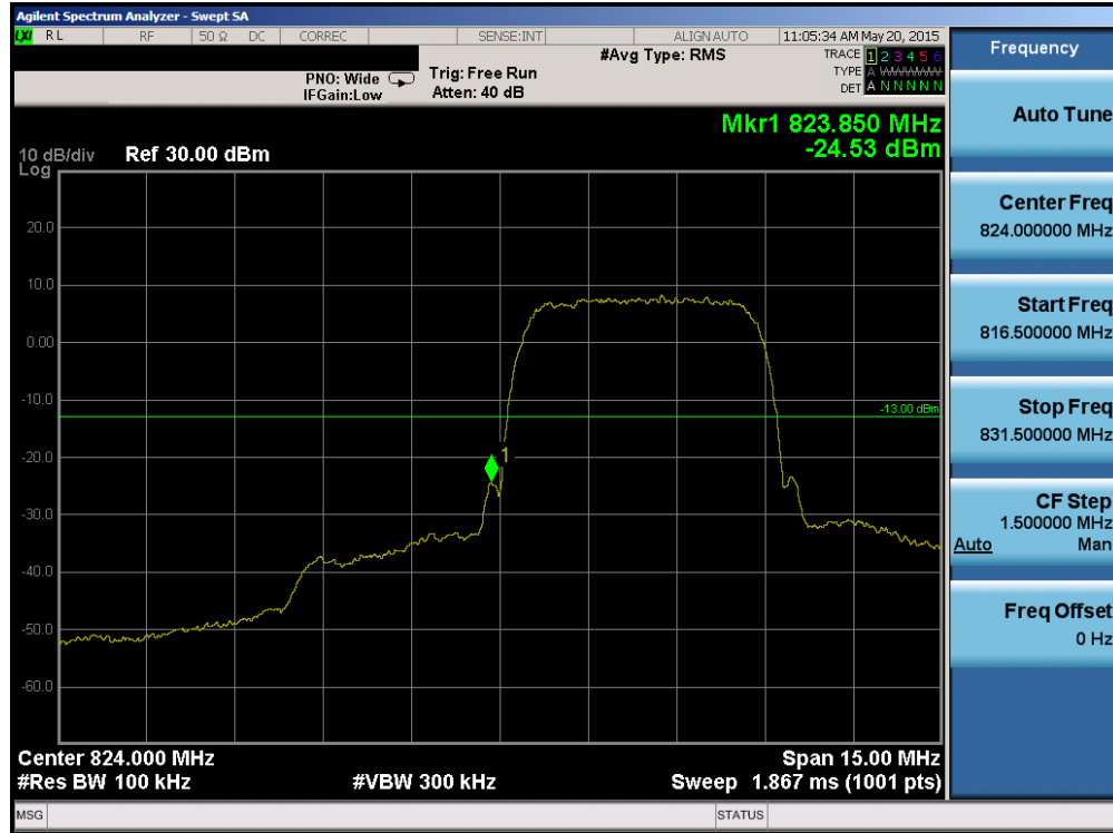
Plot 6-47. Band Edge Plot (Cellular WCDMA Mode – Ch. 4132)
