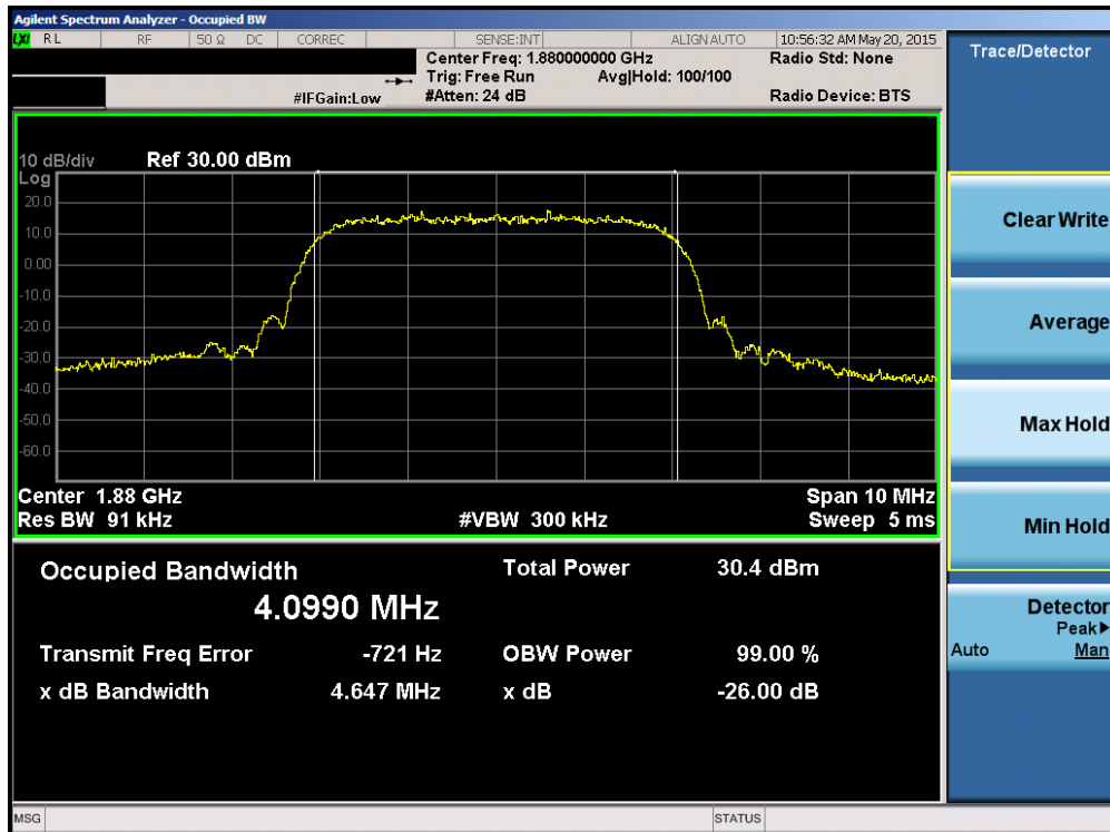
Plot 6-4. Occupied Bandwidth Plot (PCS WCDMA Mode – Ch. 9400)
