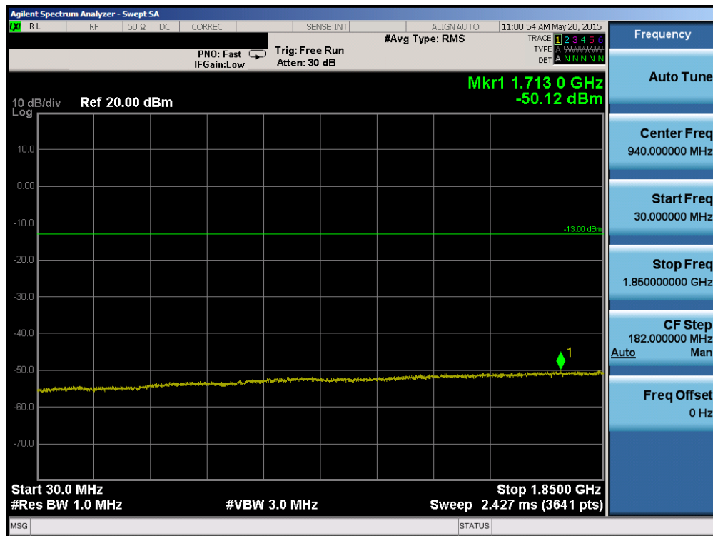
Plot 6-38. Conducted Spurious Plot (PCS WCDMA Mode – Ch. 9538)
