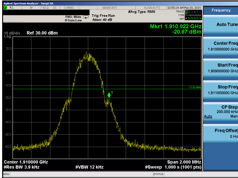
Plot 6-45. Band Edge Plot (PCS GSM Mode – Ch. 810)
