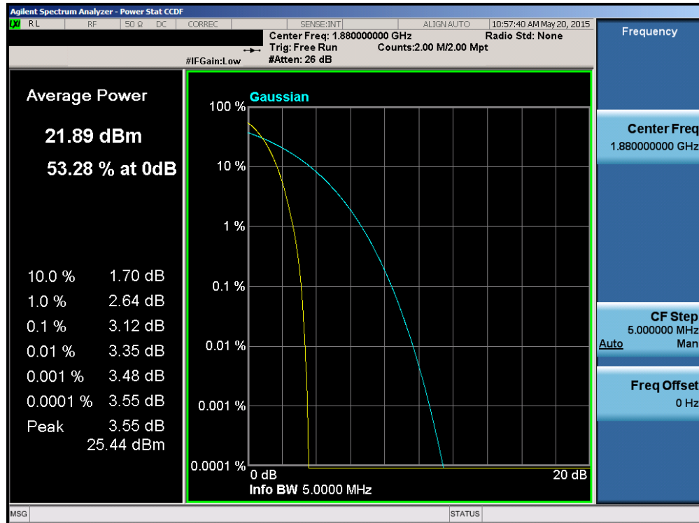
Plot 6-54. Peak-Average Ratio Plot (PCS WCDMA Mode – Ch. 9400)
