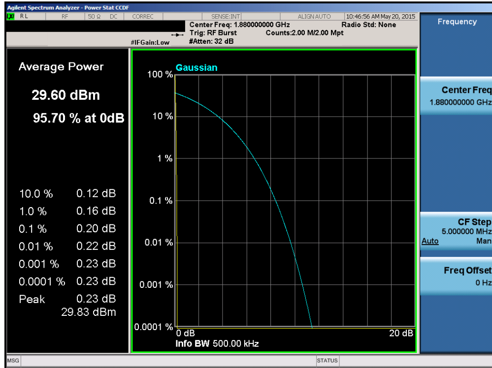
Plot 6-53. Peak-Average Ratio Plot (PCS GSM Mode – Ch. 661)
