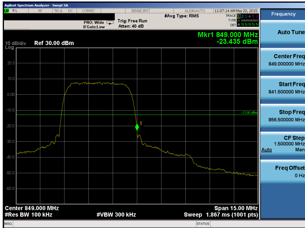
Plot 6-48. Band Edge Plot (Cellular WCDMA Mode – Ch. 4233)
