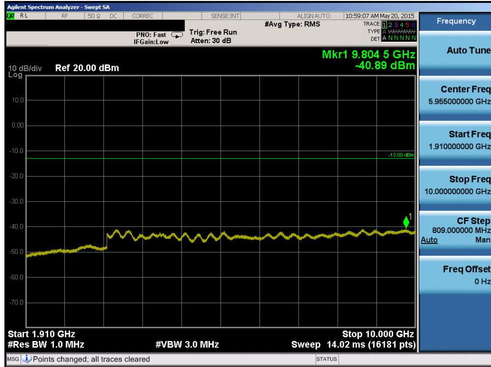
Plot 6-33. Conducted Spurious Plot (PCS WCDMA Mode – Ch. 9262)
