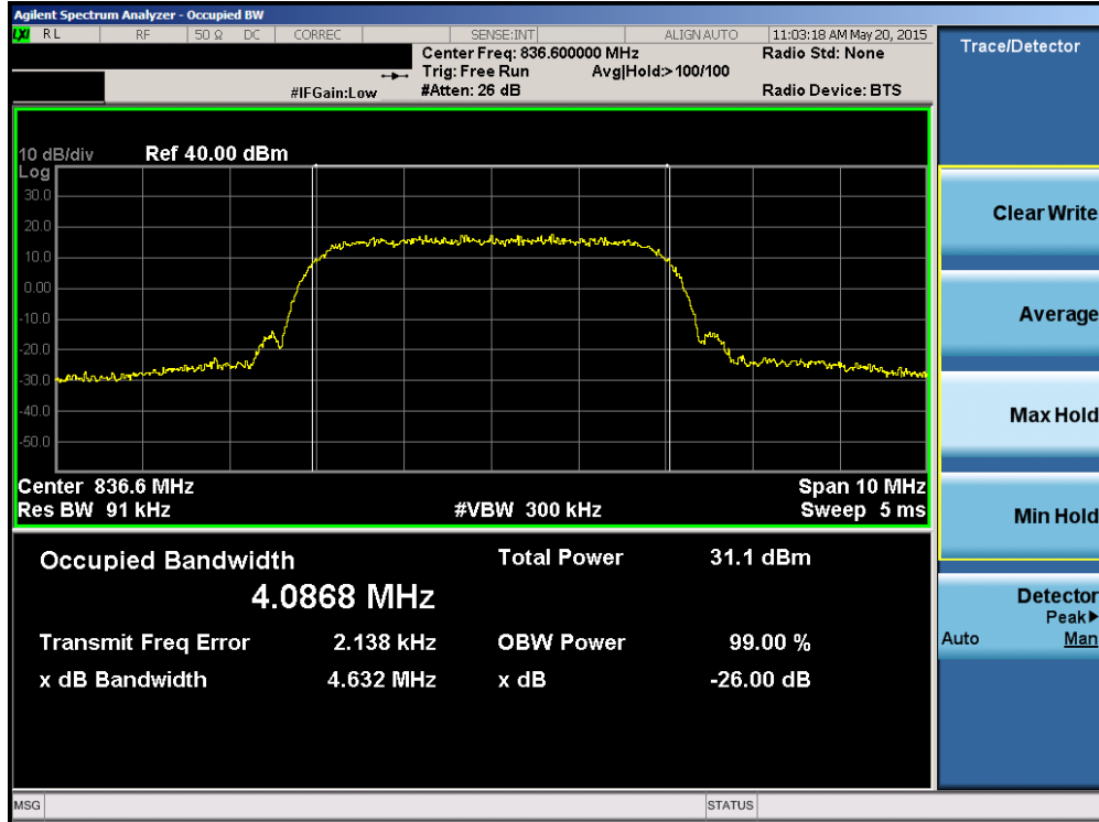
Plot 6-3. Occupied Bandwidth Plot (Cellular WCDMA Mode – Ch. 4183)
