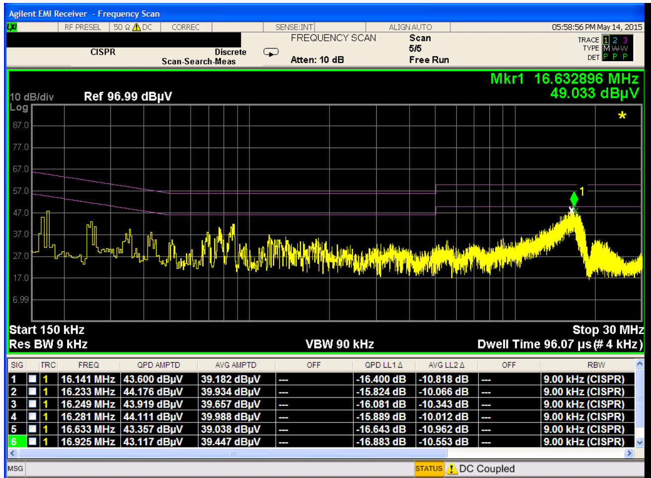
Plot 6-46. Line Conducted Plot with 802.11b (N)
