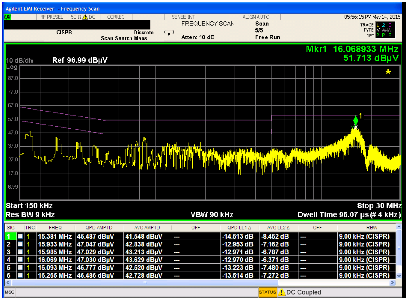
Plot 6-45. Line Conducted Plot with 802.11b (L1)
