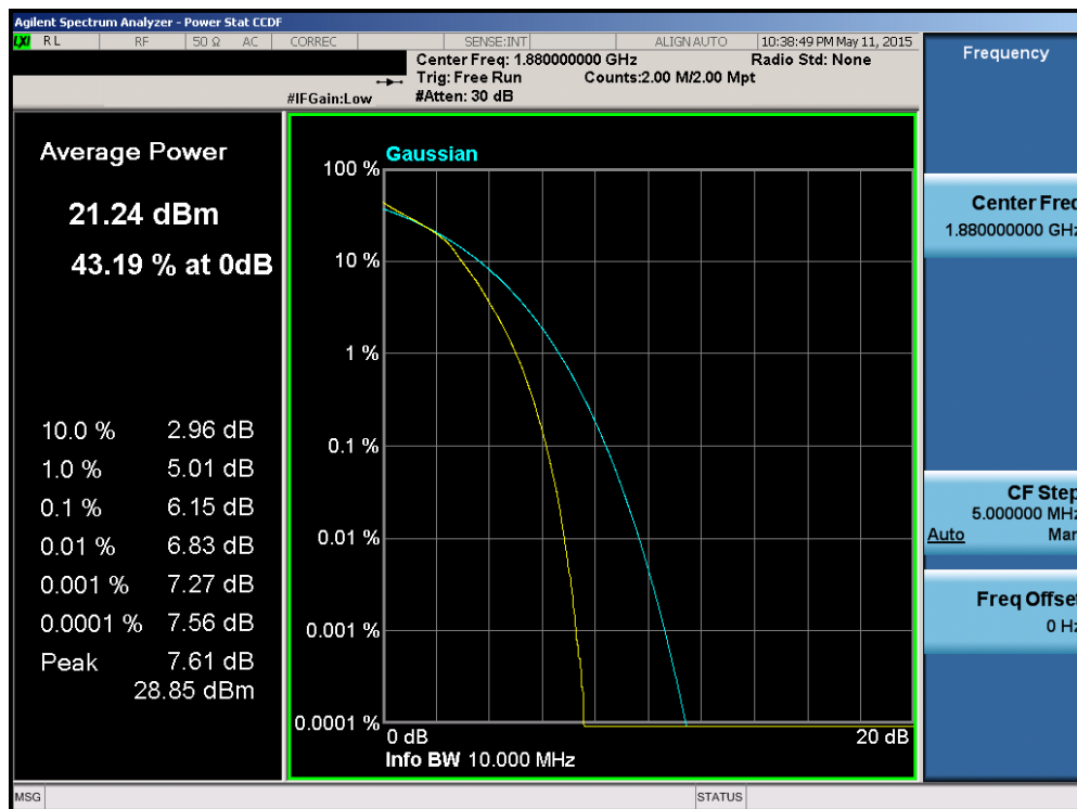
Plot 6-146. PAR Plot (Band 2 – 10.0MHz 16-QAM – RB Size 50)
