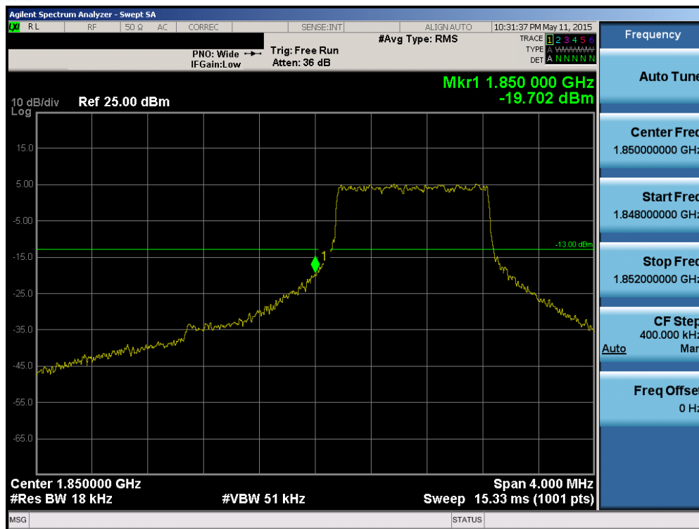
Plot 6-115. Lower Band Edge Plot (Band 2 – 1.4MHz QPSK – RB Size 6)
