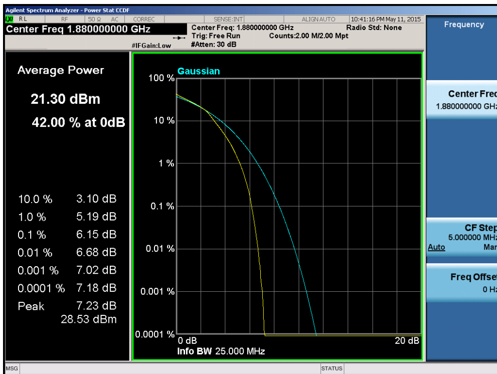
Plot 6-148. PAR Plot (Band 2 – 15.0MHz 16-QAM – RB Size 75)
