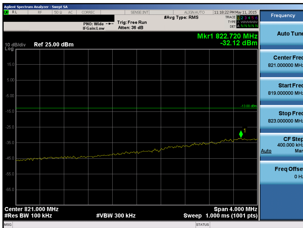
Plot 6-82. Lower Extended Band Edge Plot (Band 5 – 3.0MHz QPSK – RB Size 15)
