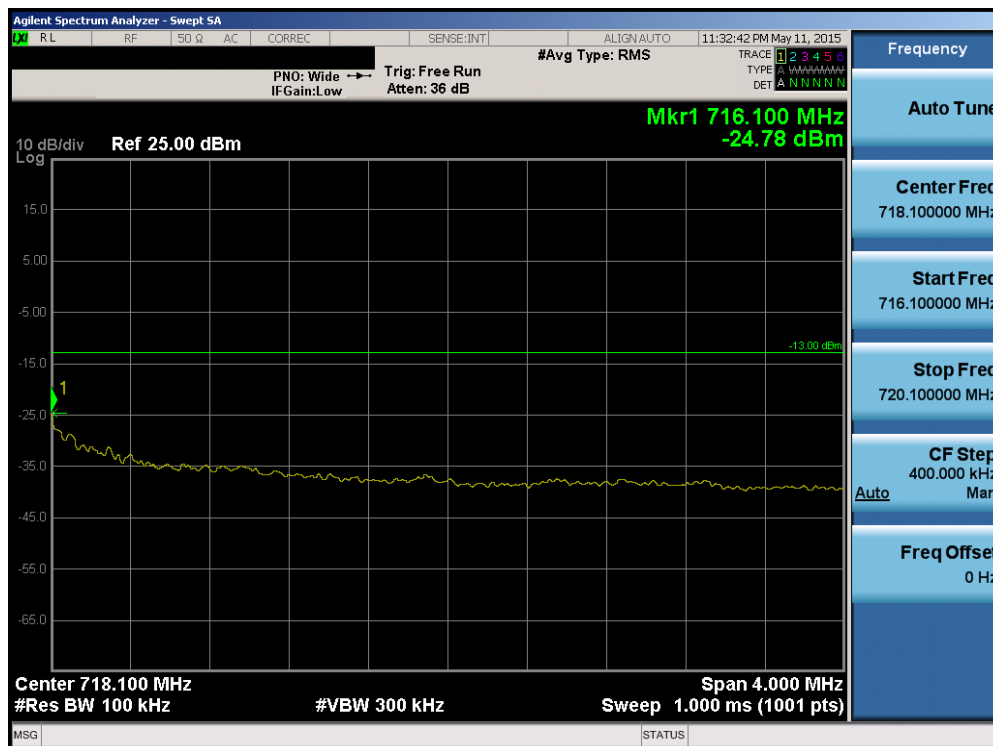
Plot 6-74. Upper Extended Band Edge Plot (Band 17 – 5.0MHz QPSK – RB Size 25)
