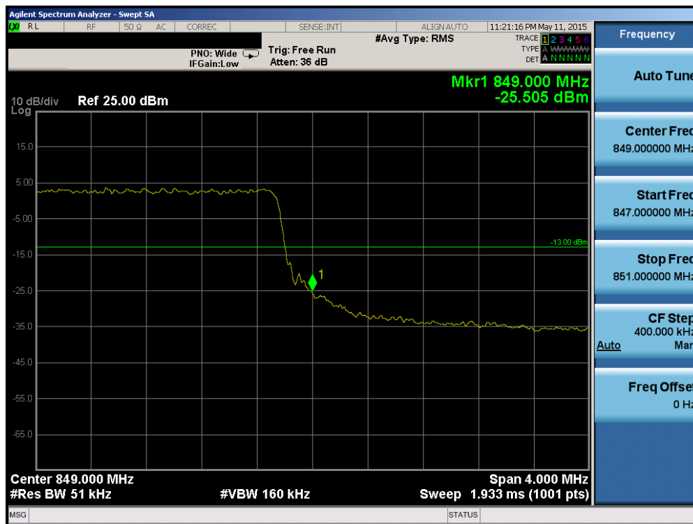
Plot 6-87. Upper Band Edge Plot (Band 5 – 5.0MHz QPSK – RB Size 25)
