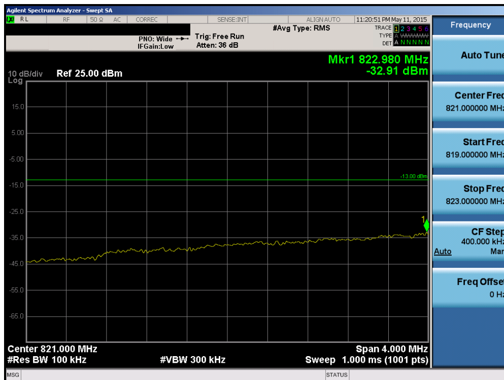
Plot 6-86. Lower Extended Band Edge Plot (Band 5 – 5.0MHz QPSK – RB Size 25)
