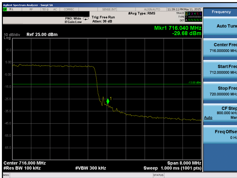
Plot 6-76. Upper Band Edge Plot (Band 17 – 10.0MHz QPSK – RB Size 50)
