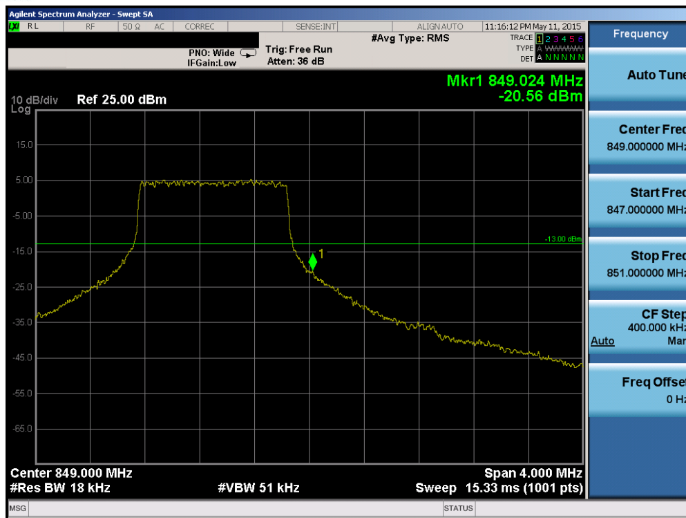
Plot 6-79. Upper Band Edge Plot (Band 5 - 1.4MHz QPSK - RB Size 6)
