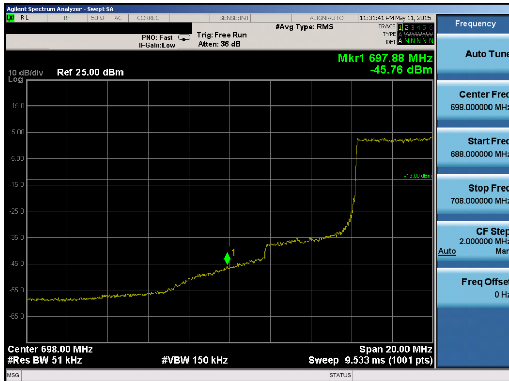
Plot 6-71. Lower Band Edge Plot (Band 17 – 5.0MHz QPSK – RB Size 25)
