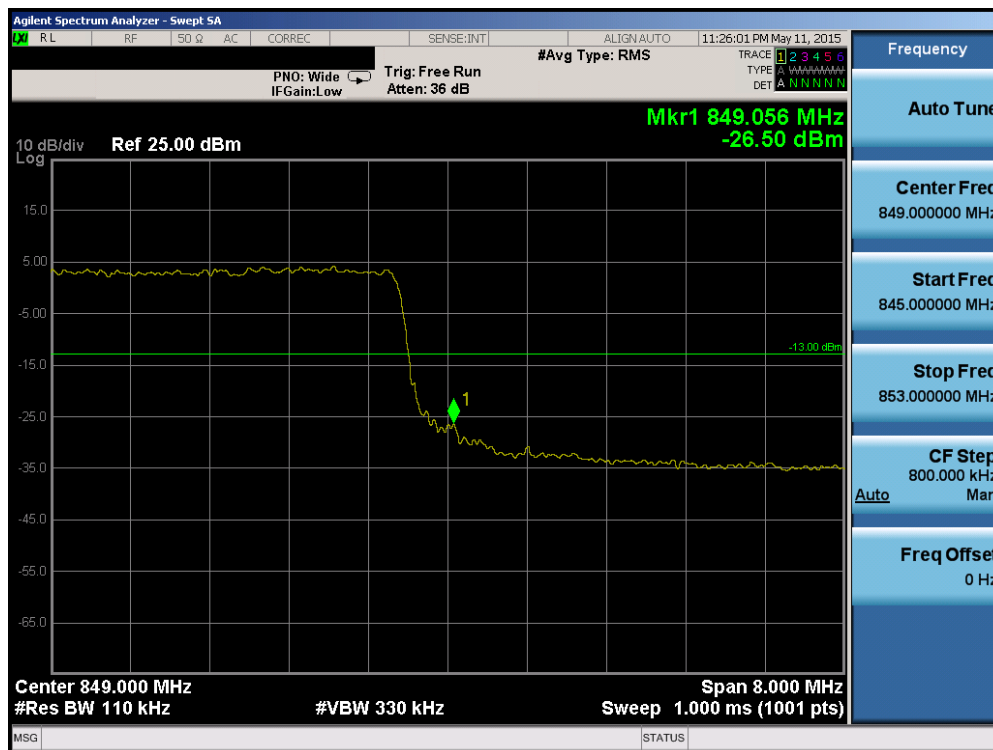
Plot 6-90. Upper Band Edge Plot (Band 5 – 10.0MHz QPSK – RB Size 50)
