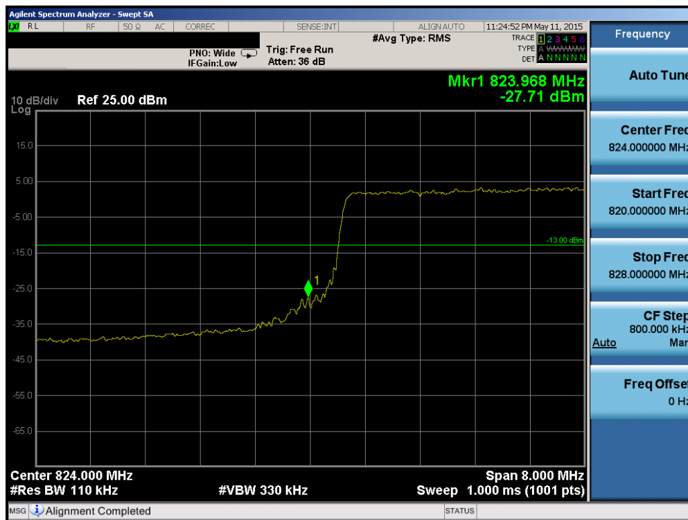
Plot 6-89. Lower Band Edge Plot (Band 5 – 10.0MHz QPSK – RB Size 50)
