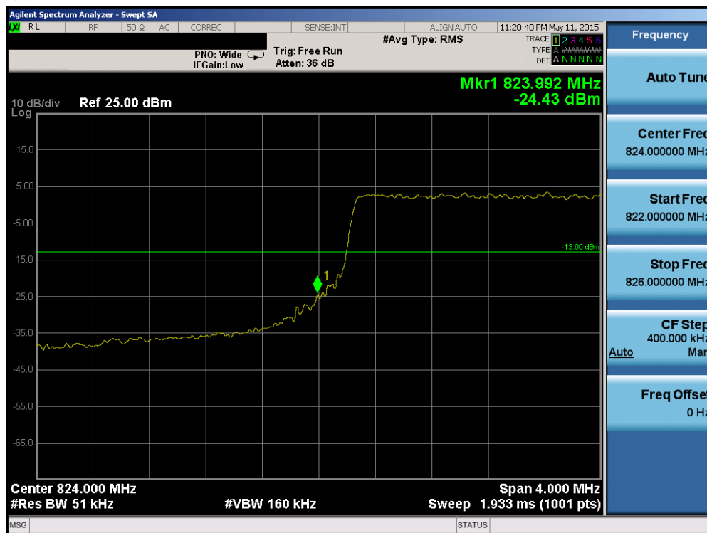
Plot 6-85. Lower Band Edge Plot (Band 5 – 5.0MHz QPSK – RB Size 25)
