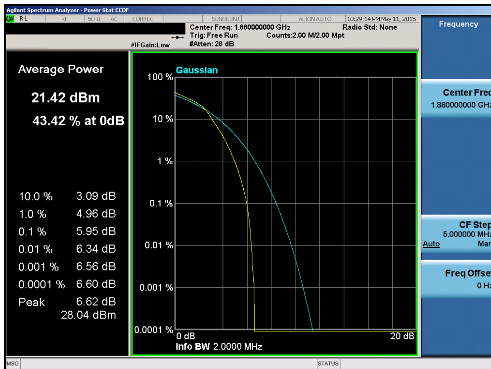
Plot 6-140. PAR Plot (Band 2 – 1.4MHz 16-QAM – RB Size 6)
