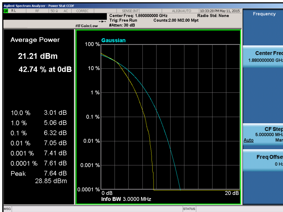
Plot 6-142. PAR Plot (Band 2 – 3.0MHz 16-QAM – RB Size 15)
