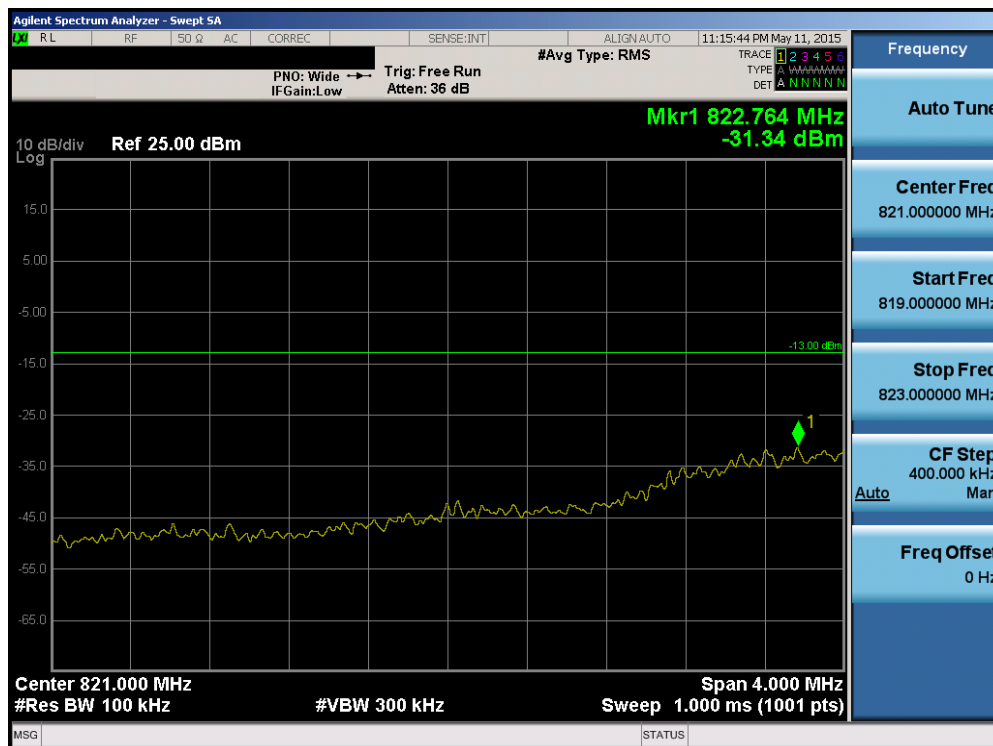
Plot 6-78. Lower Extended Band Edge Plot (Band 5 – 1.4MHz QPSK – RB Size 6)
