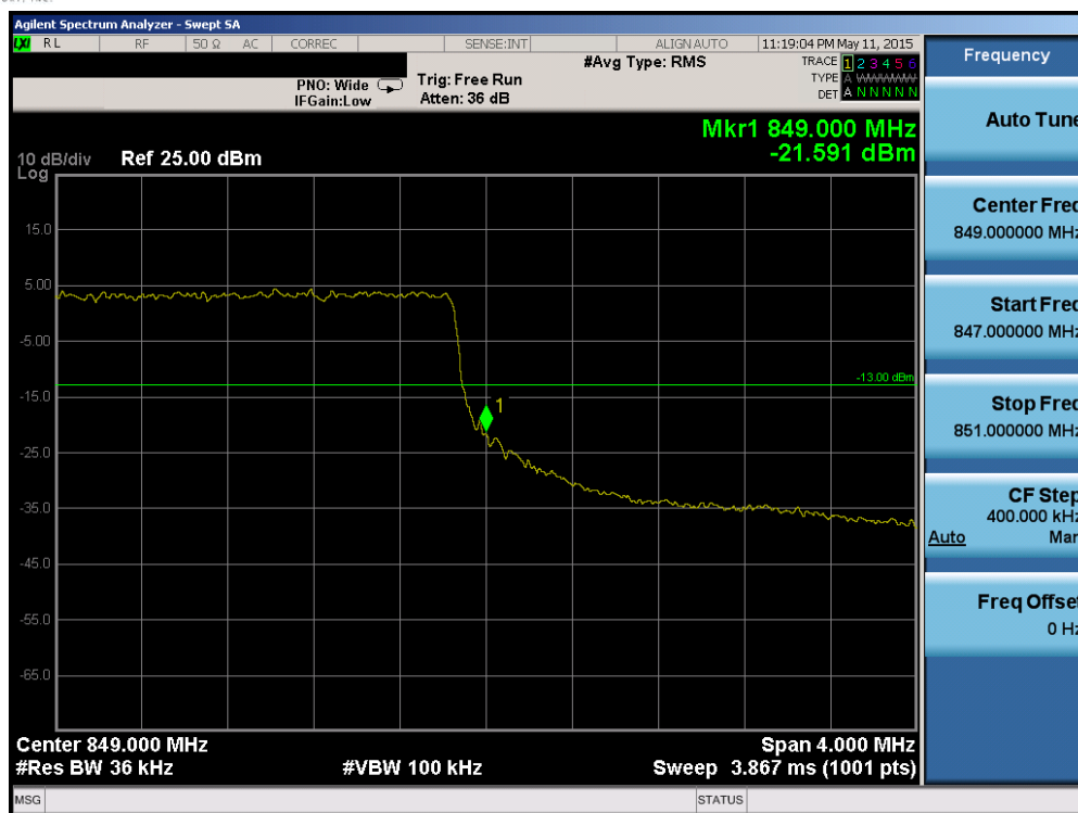
Plot 6-83. Upper Band Edge Plot (Band 5 – 3.0MHz QPSK – RB Size 15)
