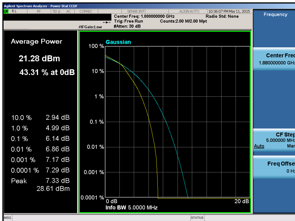
Plot 6-144. PAR Plot (Band 2 – 5.0MHz 16-QAM – RB Size 25)
