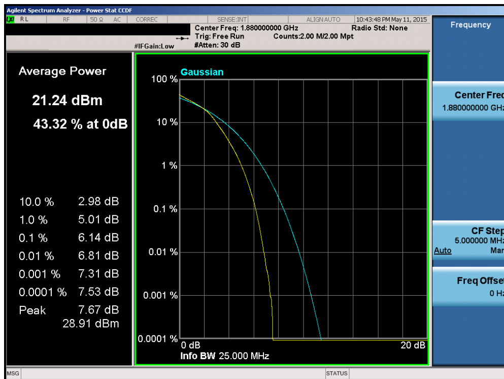
Plot 6-150. PAR Plot (Band 2 – 20.0MHz 16-QAM – RB Size 100)
