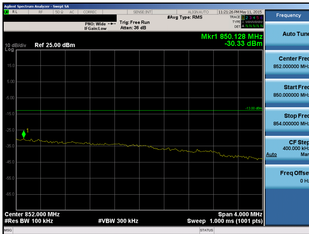
Plot 6-88. Upper Extended Band Edge Plot (Band 5 – 5.0MHz QPSK – RB Size 25)
