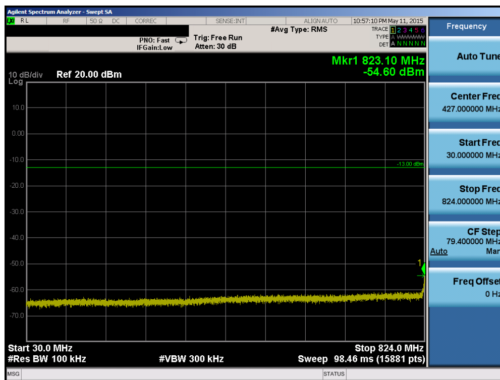
Plot 6-28. Conducted Spurious Plot (Cellular WCDMA Mode – Ch. 4183)
