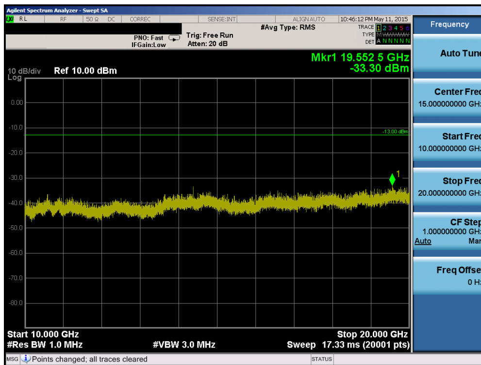
Plot 6-21. Conducted Spurious Plot (PCS GSM Mode – Ch. 661)
