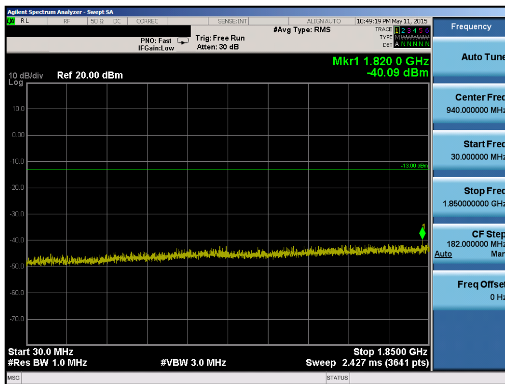
Plot 6-22. Conducted Spurious Plot (PCS GSM Mode – Ch. 810)
