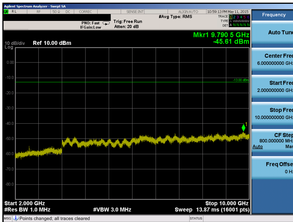
Plot 6-27. Conducted Spurious Plot (Cellular WCDMA Mode – Ch. 4132)
