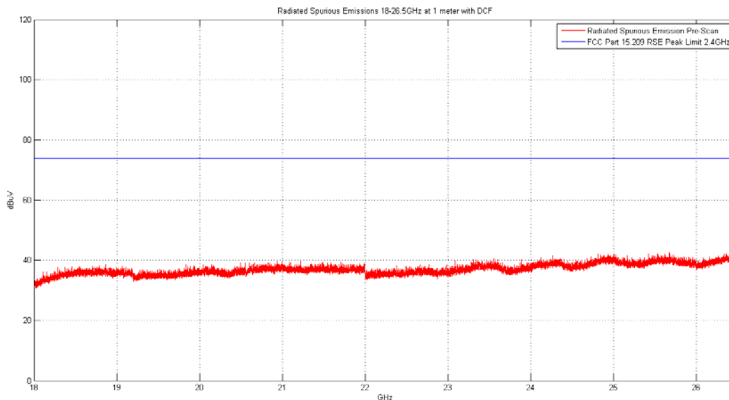
Plot 6-37. Radiated Spurious Plot above 18GHz (Pol. H)
