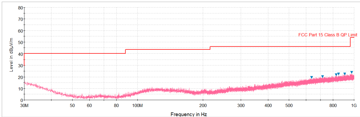
Plot 6-41. Radiated Spurious Plot below 1GHz (Pol. H)
