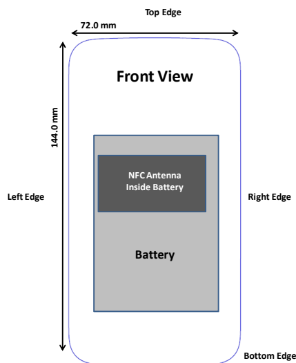
Figure F-2 NFC Antenna Location
