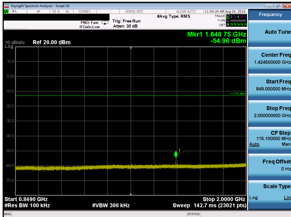
Plot 7-10. Conducted Spurious Plot (Band 5 – 1.4MHz QPSK – RB Size 1, RB Offset 0 – Low Channel)
