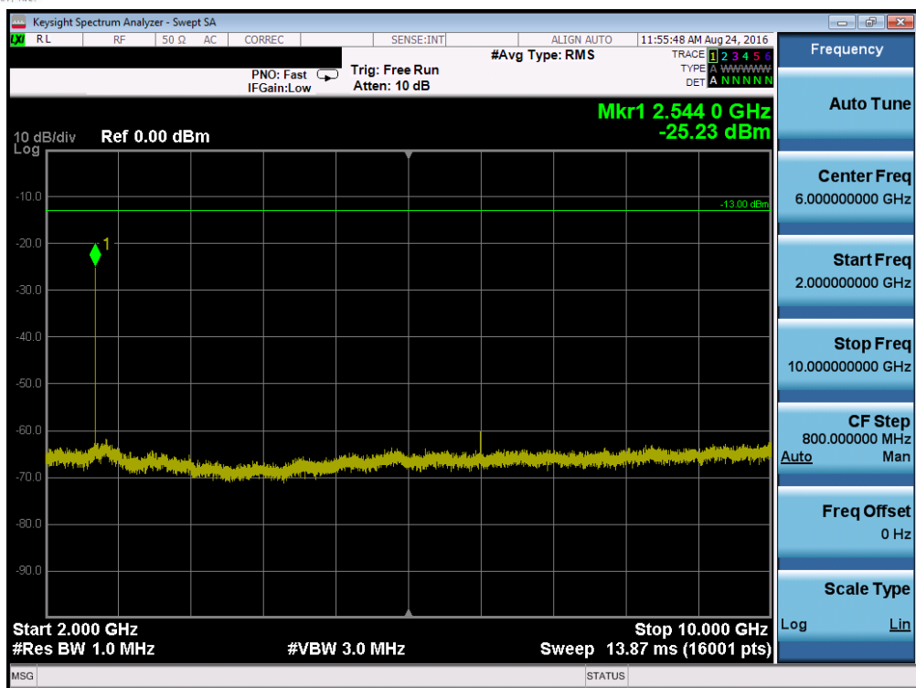
Plot 17-17. Conducted Spurious Plot (Band 5 – 1.4MHz QPSK – RB Size 1, RB Offset 0 – High Channel)
