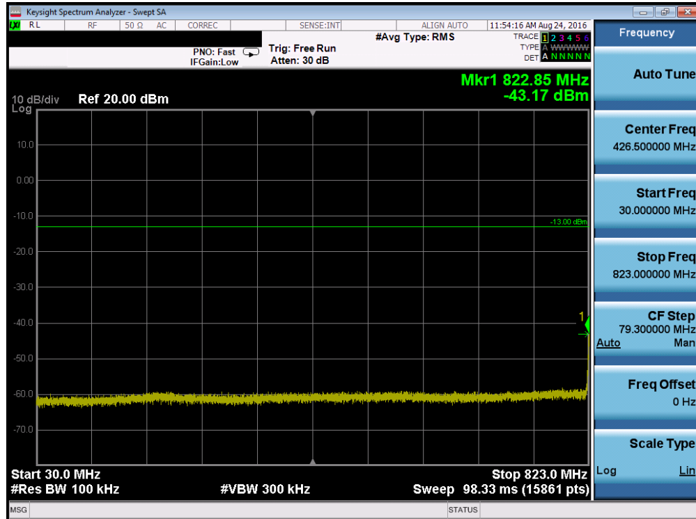
Plot 7-9. Conducted Spurious Plot (Band 5 – 1.4MHz QPSK – RB Size 1, RB Offset 0 – Low Channel)
