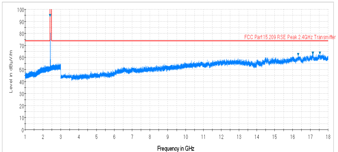
Plot 7-43. Radiated Spurious Plot above 1GHz (BT – Ch. 0, Ant. Pol. V)
