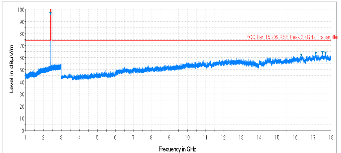
Plot 7-42. Radiated Spurious Plot above 1GHz (BT – Ch. 0, Ant. Pol. H)
