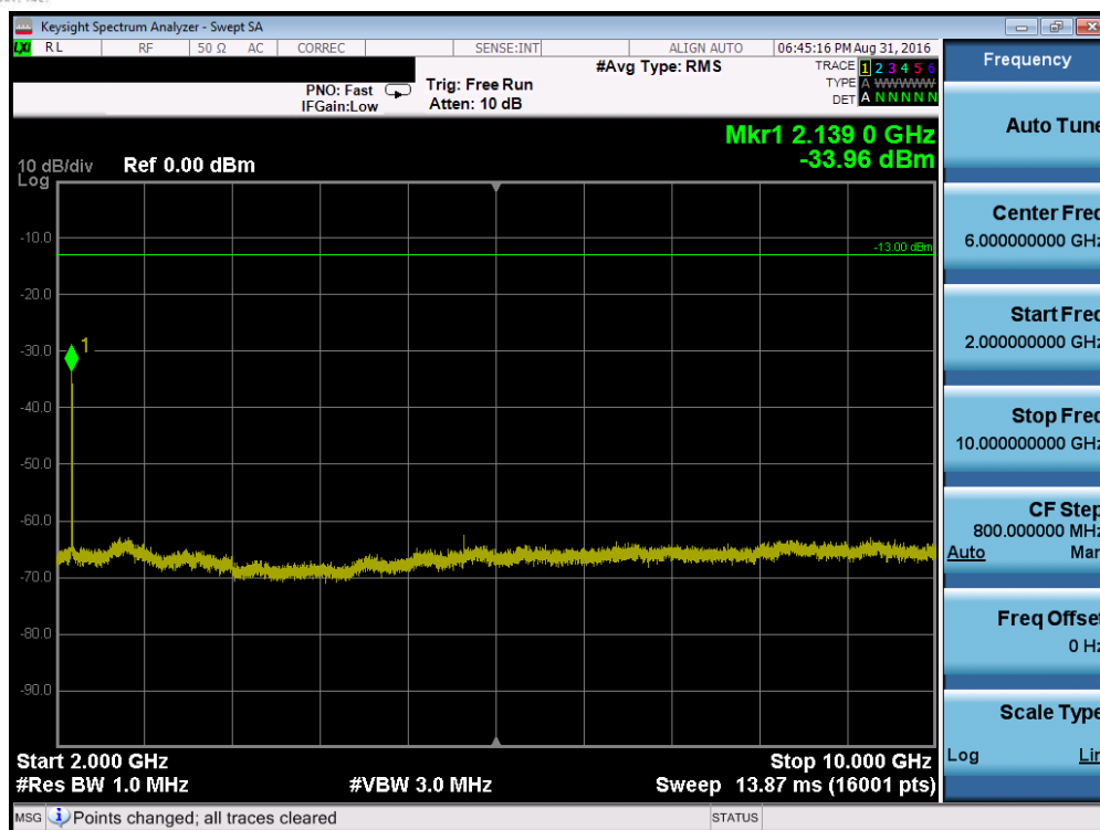
Plot 7-45. Conducted Spurious Plot (Band 17 – 5.0MHz QPSK – RB Size 1, RB Offset 0 – High Channel)
