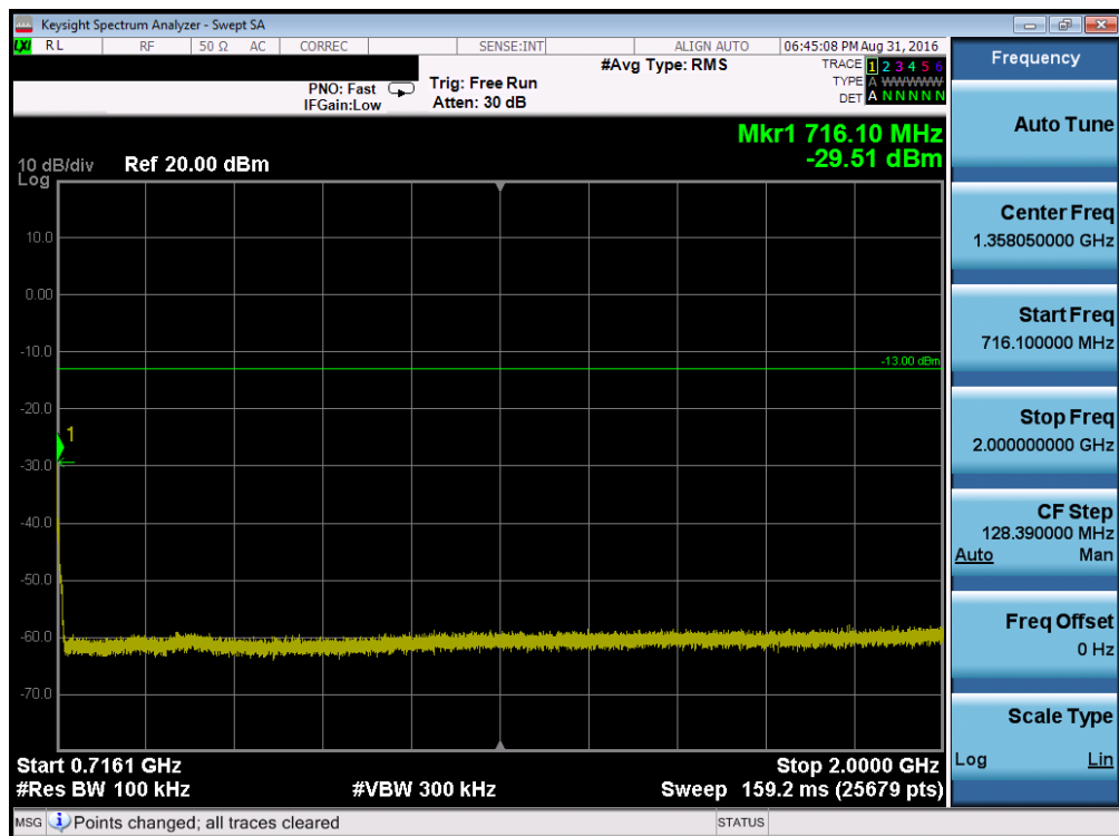
Plot 7-44. Conducted Spurious Plot (Band 17 – 5.0MHz QPSK – RB Size 1, RB Offset 0 – High Channel)
