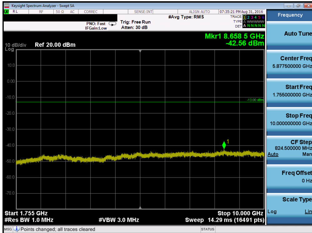
Plot 7-56. Conducted Spurious Plot (Band 4 – 10.0MHz QPSK – RB Size 1, RB Offset 0 – Low Channel)
