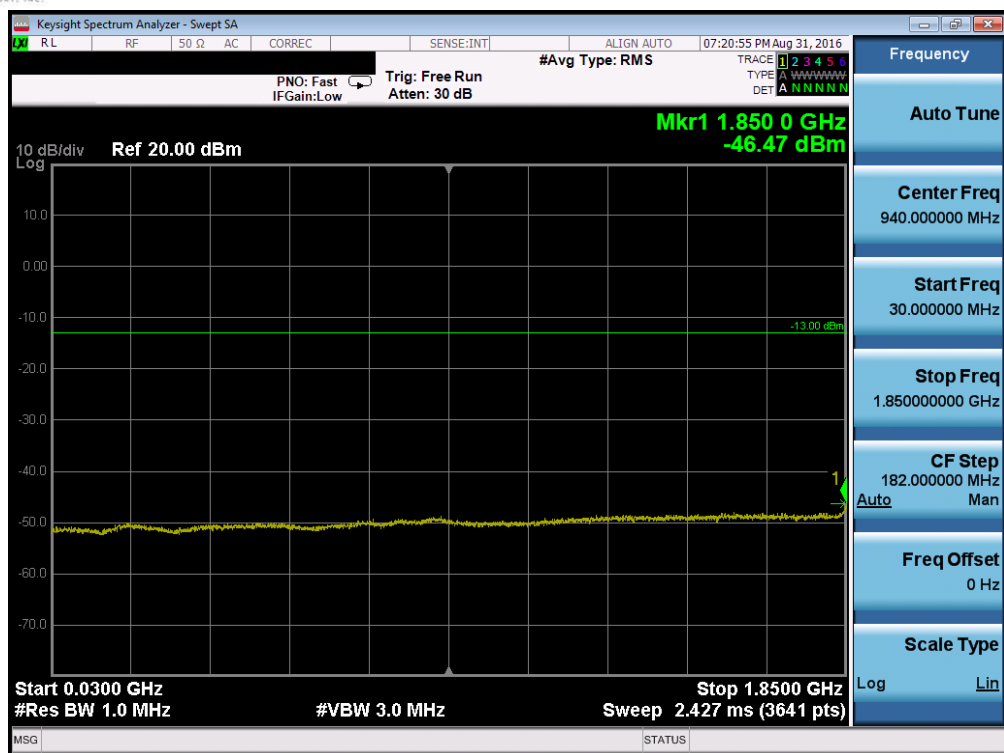
Plot 7-67. Conducted Spurious Plot (Band 2 – 10.0MHz QPSK – RB Size 1, RB Offset 0 – Mid Channel)
