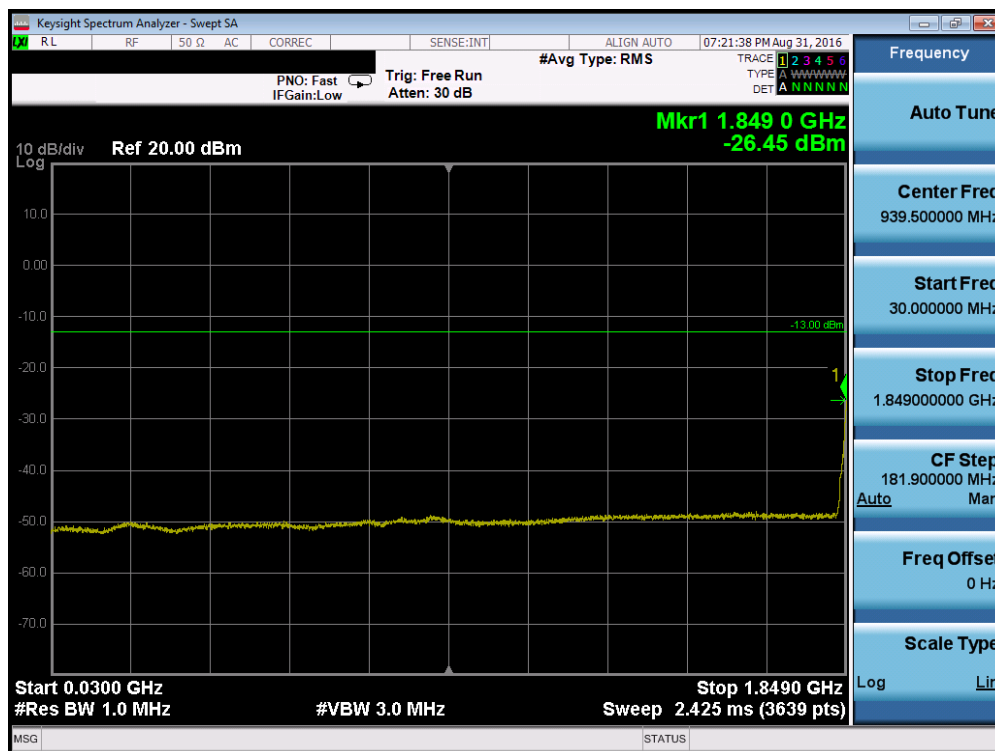
Plot 7-64. Conducted Spurious Plot (Band 2 – 10.0MHz QPSK – RB Size 1, RB Offset 0– Low Channel)
