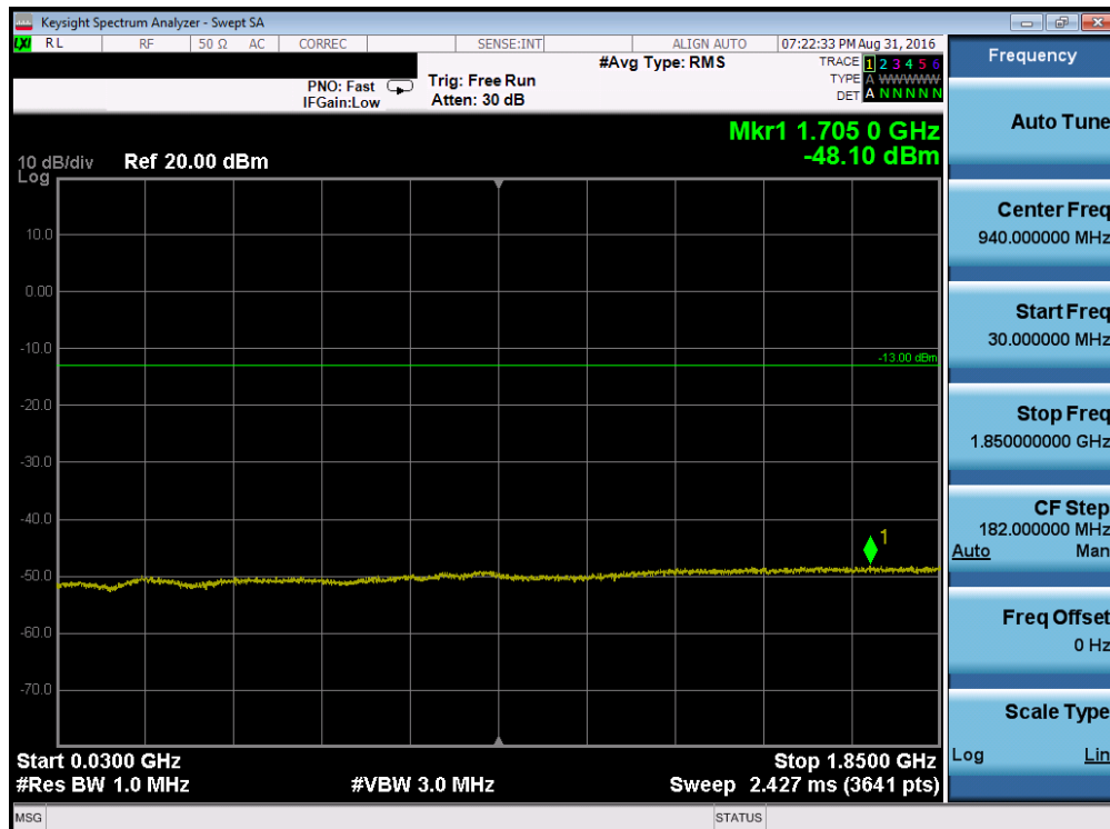
Plot 7-70. Conducted Spurious Plot (Band 2 – 10.0MHz QPSK – RB Size 1, RB Offset 0 – High Channel)
