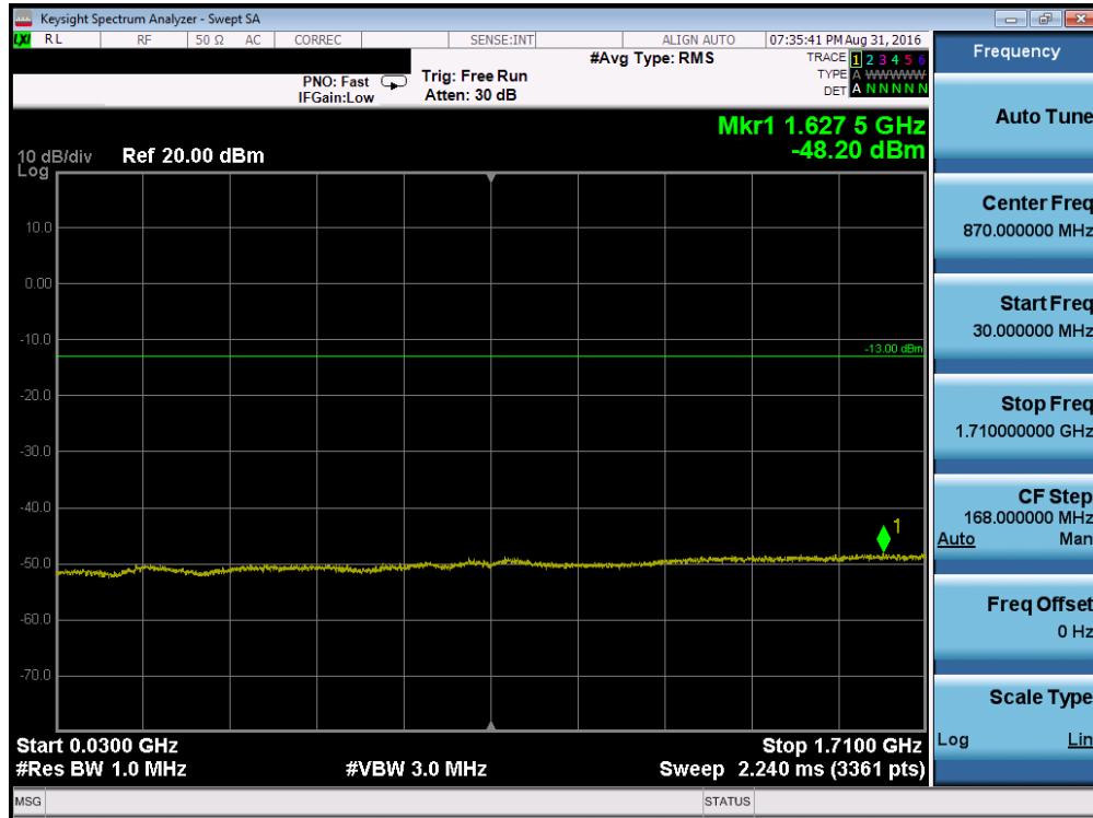
Plot 7-61. Conducted Spurious Plot (Band 4 – 10.0MHz QPSK – RB Size 1, RB Offset 0 – High Channel)
