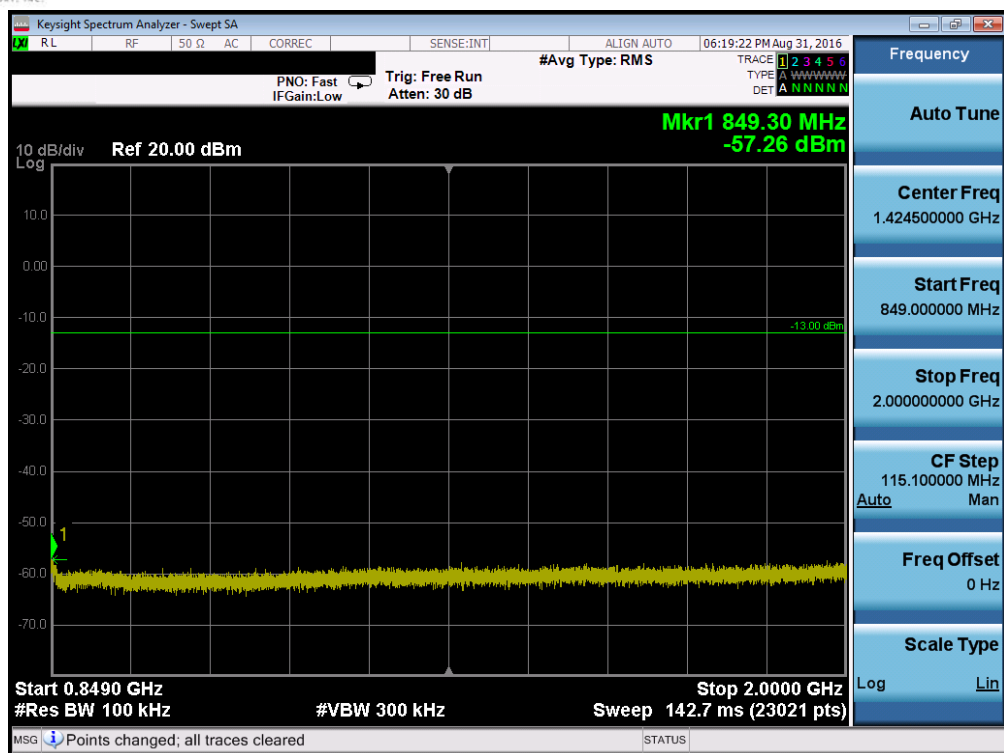
Plot 7-47. Conducted Spurious Plot (Band 5 – 10.0MHz QPSK – RB Size 1, RB Offset 0 – Low Channel)
