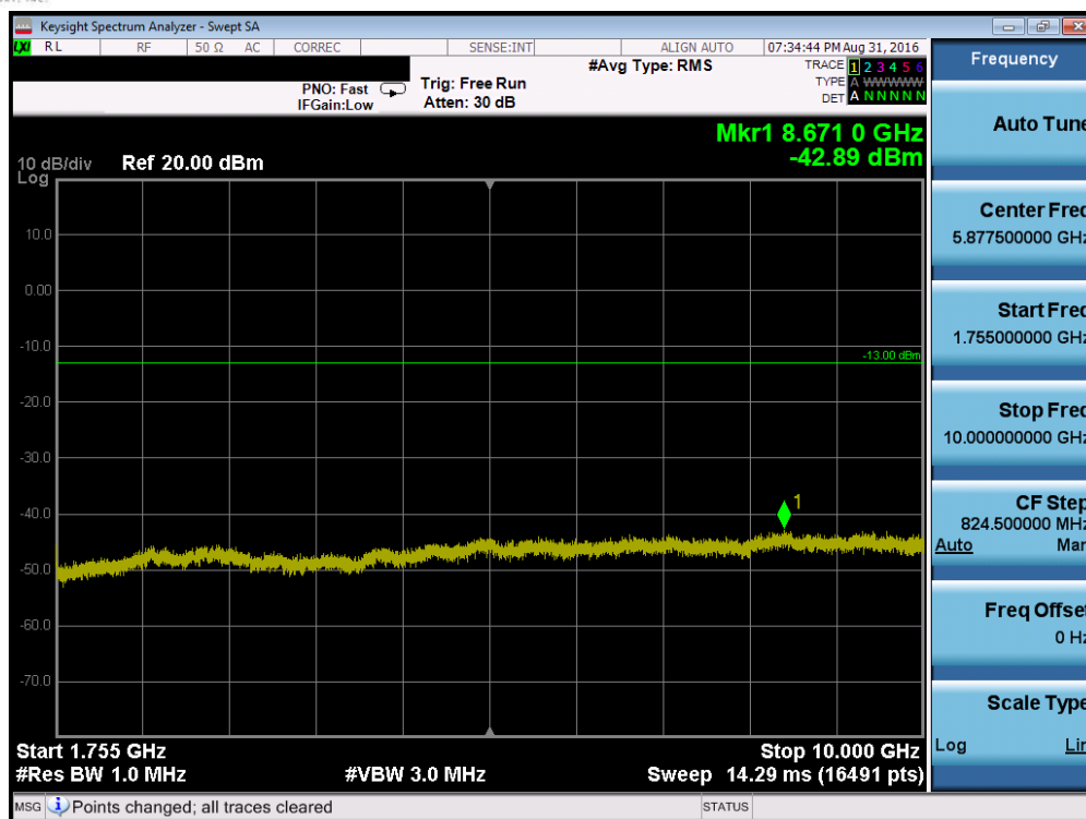
Plot 7-59. Conducted Spurious Plot (Band 4 – 10.0MHz QPSK – RB Size 1, RB Offset 0 – Mid Channel)
