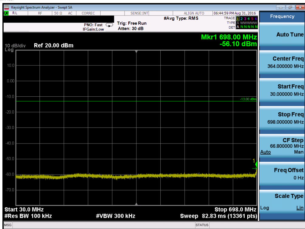
Plot 7-43. Conducted Spurious Plot (Band 17 – 5.0MHz QPSK – RB Size 1, RB Offset 0 – High Channel)
