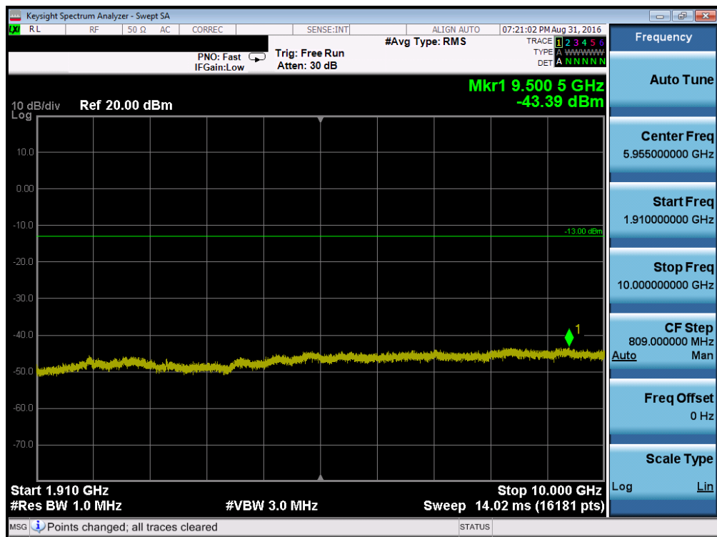
Plot 7-68. Conducted Spurious Plot (Band 2 – 10.0MHz QPSK – RB Size 1, RB Offset 0 – Mid Channel)
