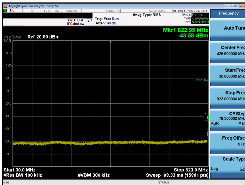
Plot 7-46. Conducted Spurious Plot (Band 5 – 10.0MHz QPSK – RB Size 1, RB Offset 0– Low Channel)
