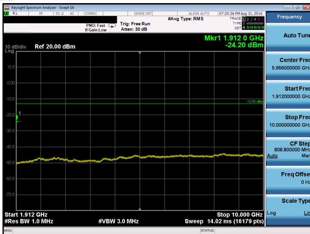
Plot 7-71. Conducted Spurious Plot (Band 2 – 10.0MHz QPSK – RB Size 1, RB Offset 0 – High Channel)
