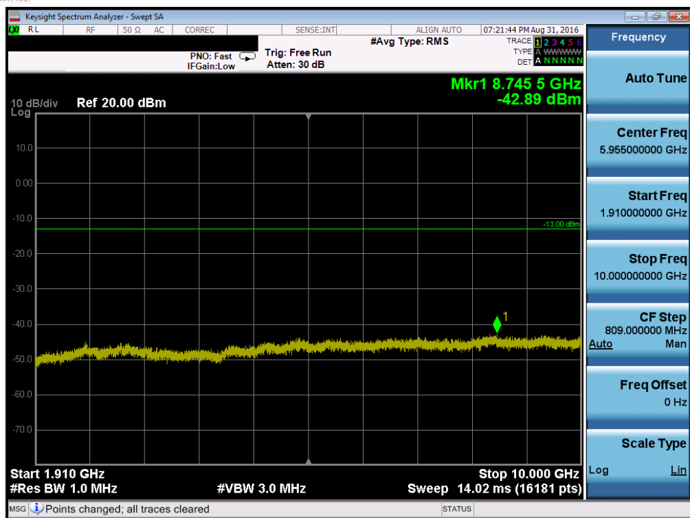
Plot 7-65. Conducted Spurious Plot (Band 2 – 10.0MHz QPSK – RB Size 1, RB Offset 0 – Low Channel)
