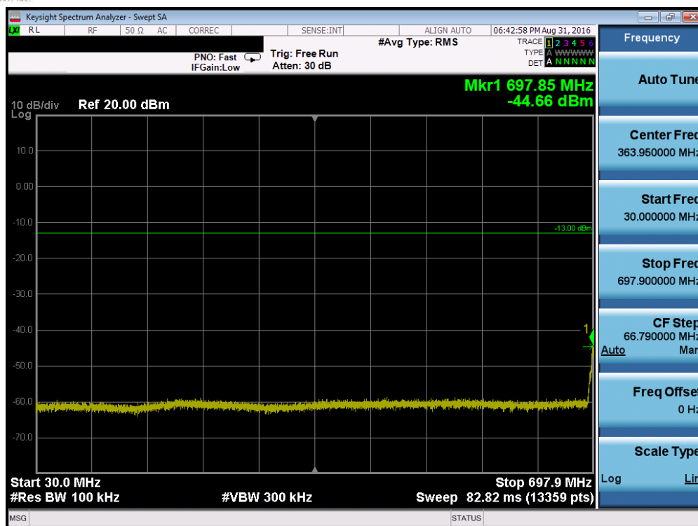
Plot 7-37. Conducted Spurious Plot (Band 17 – 5.0MHz QPSK – RB Size 1, RB Offset 0 – Low Channel)
