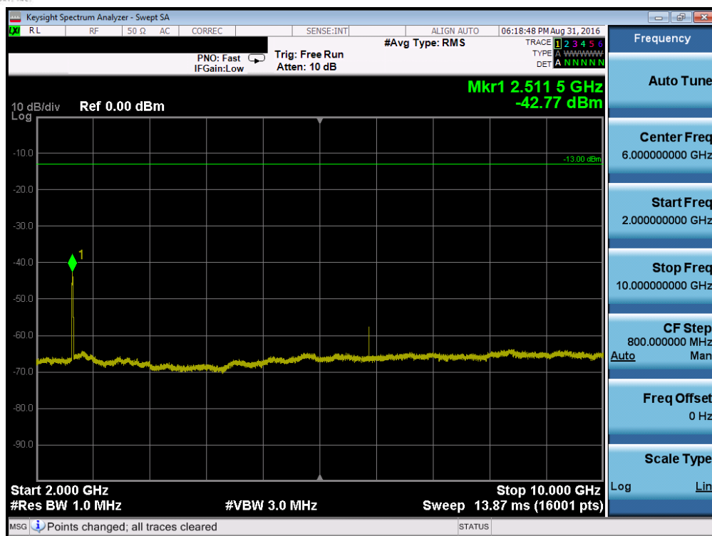
Plot 7-51. Conducted Spurious Plot (Band 5 – 10.0MHz QPSK – RB Size 1, RB Offset 0 – Mid Channel)
