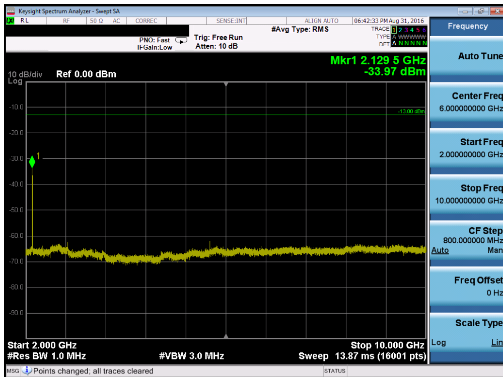
Plot 7-42. Conducted Spurious Plot (Band 17 – 5.0MHz QPSK – RB Size 1, RB Offset 0 – Mid Channel)
