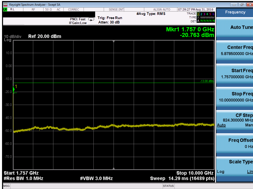
Plot 7-62. Conducted Spurious Plot (Band 4 – 10.0MHz QPSK – RB Size 1, RB Offset 0 – High Channel)
