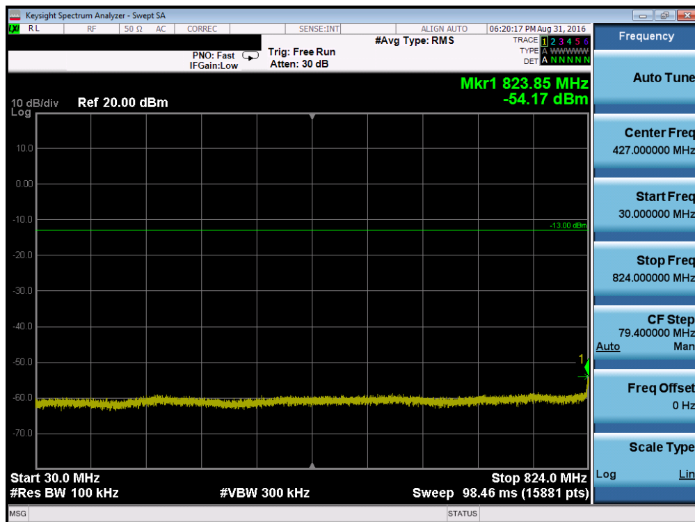
Plot 7-52. Conducted Spurious Plot (Band 5 – 10.0MHz QPSK – RB Size 1, RB Offset 0 – High Channel)
