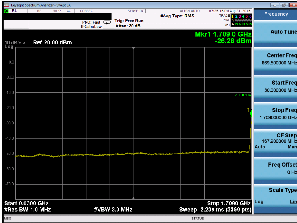
Plot 7-55. Conducted Spurious Plot (Band 4 – 10.0MHz QPSK – RB Size 1, RB Offset 0– Low Channel)
