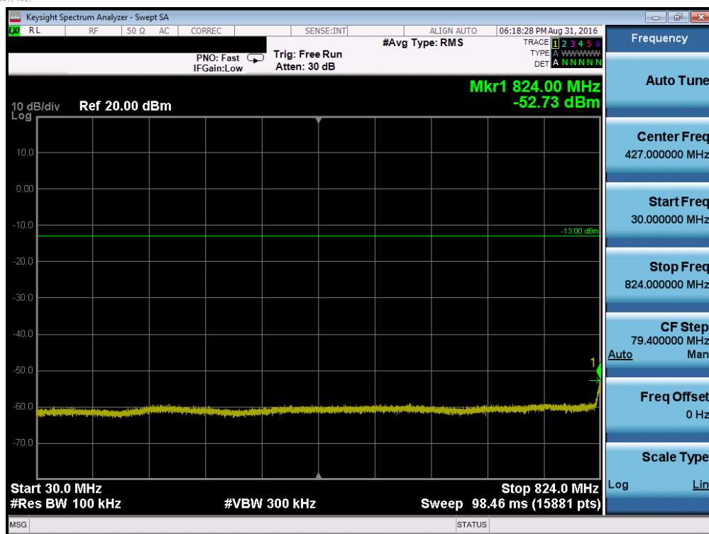
Plot 7-49. Conducted Spurious Plot (Band 5 – 10.0MHz QPSK – RB Size 1, RB Offset 0 – Mid Channel)
