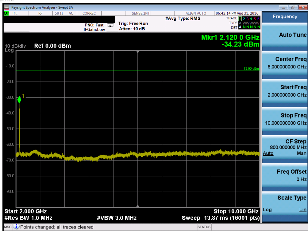
Plot 7-39. Conducted Spurious Plot (Band 17 - 5.0MHz QPSK - RB Size 1, RB Offset 0 - Low Channel)
