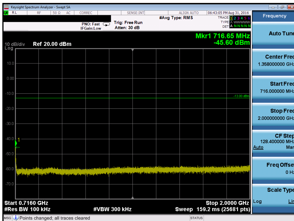
Plot 7-38. Conducted Spurious Plot (Band 17 – 5.0MHz QPSK – RB Size 1, RB Offset 0 – Low Channel)
