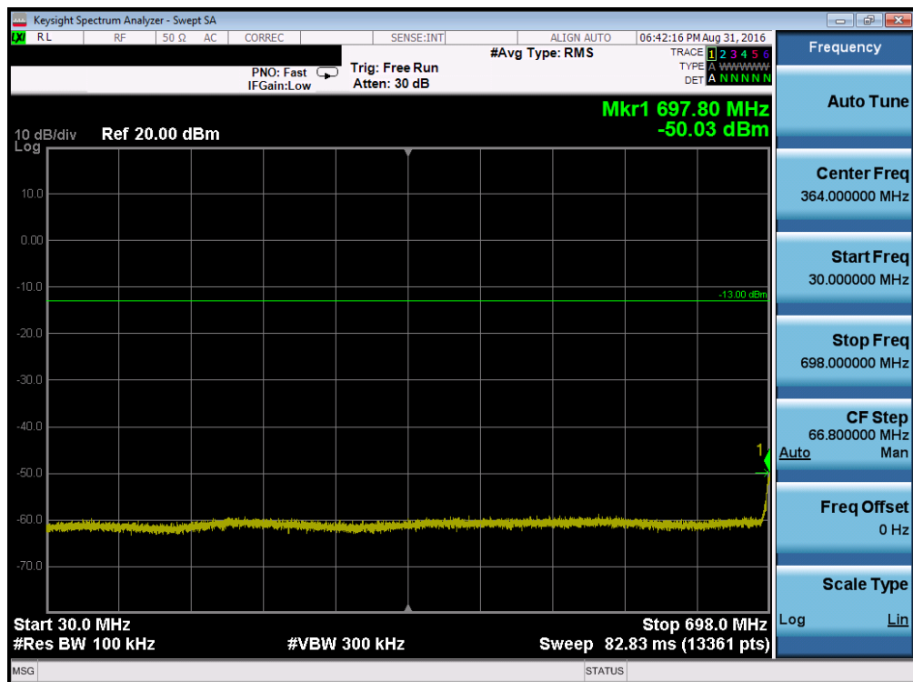
Plot 7-40. Conducted Spurious Plot (Band 17 - 5.0MHz QPSK - RB Size 1, RB Offset 0 - Mid Channel)
