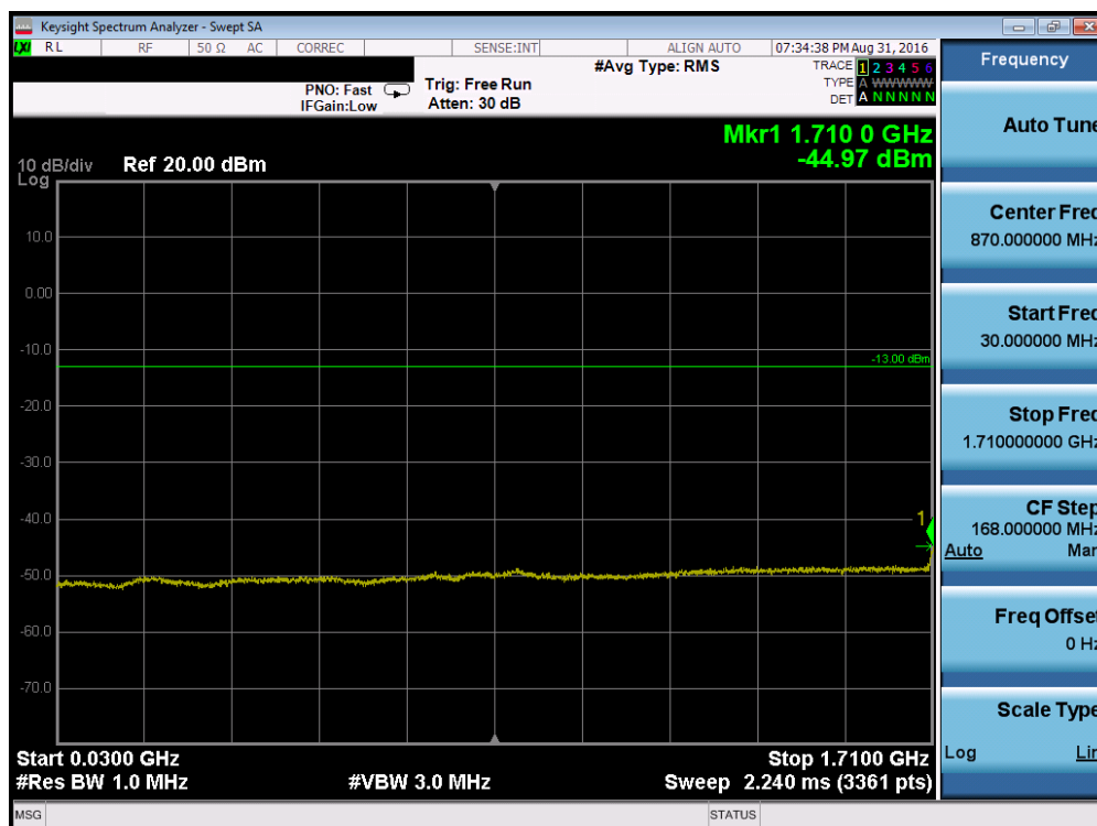
Plot 7-58. Conducted Spurious Plot (Band 4 – 10.0MHz QPSK – RB Size 1, RB Offset 0 – Mid Channel)
