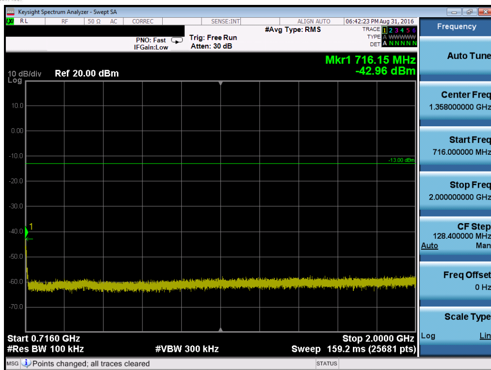
Plot 7-41. Conducted Spurious Plot (Band 17 – 5.0MHz QPSK – RB Size 1, RB Offset 0 – Mid Channel)
