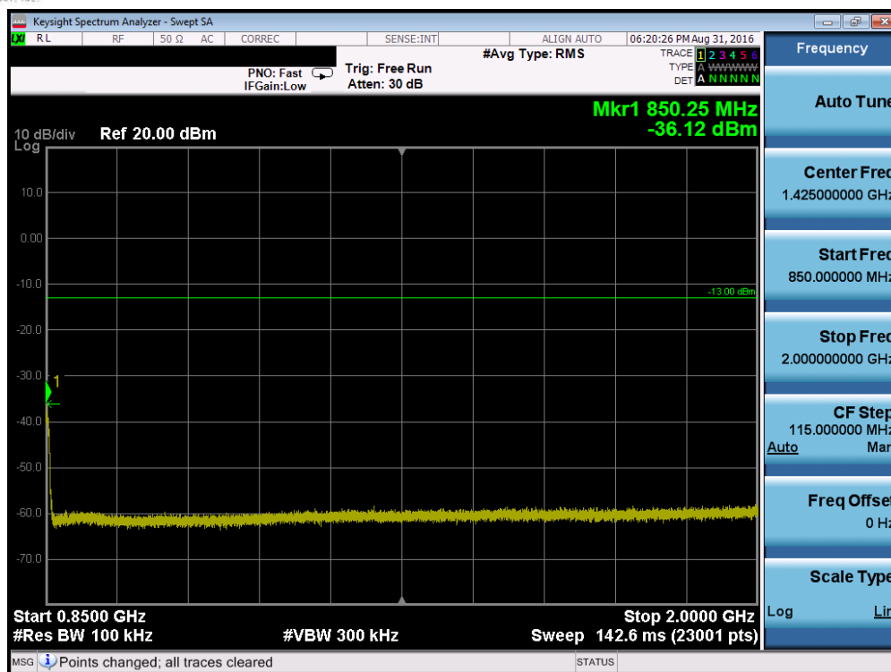
Plot 7-53. Conducted Spurious Plot (Band 5 – 10.0MHz QPSK – RB Size 1, RB Offset 0 – High Channel)
