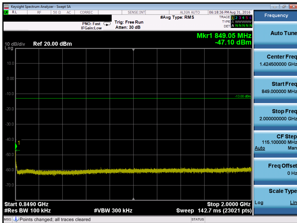
Plot 7-50. Conducted Spurious Plot (Band 5 – 10.0MHz QPSK – RB Size 1, RB Offset 0 – Mid Channel)
