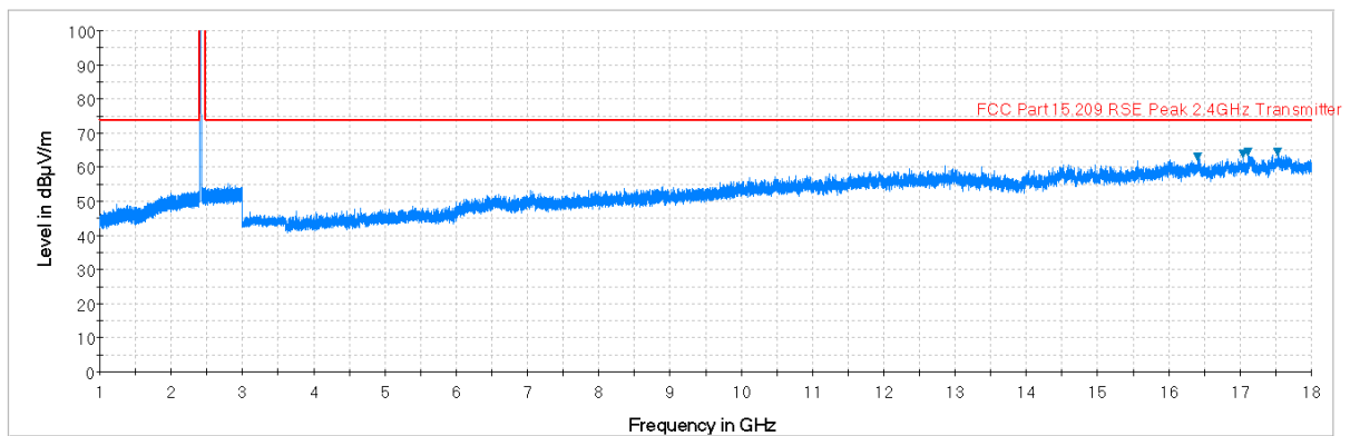
Plot 7-41. Radiated Spurious Plot above 1GHz (802.11b – Ch. 1, Ant. Pol. V)
