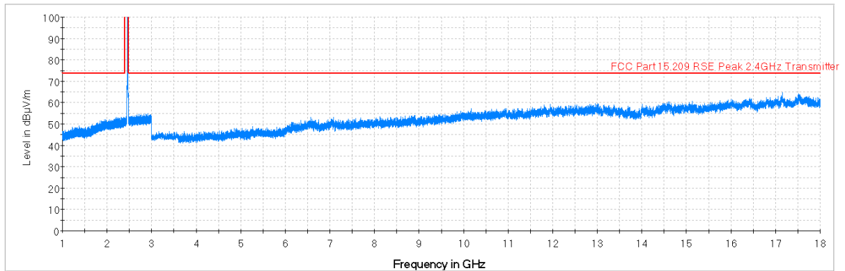
Plot 7-45. Radiated Spurious Plot above 1GHz (802.11b – Ch. 11, Ant. Pol. V)
