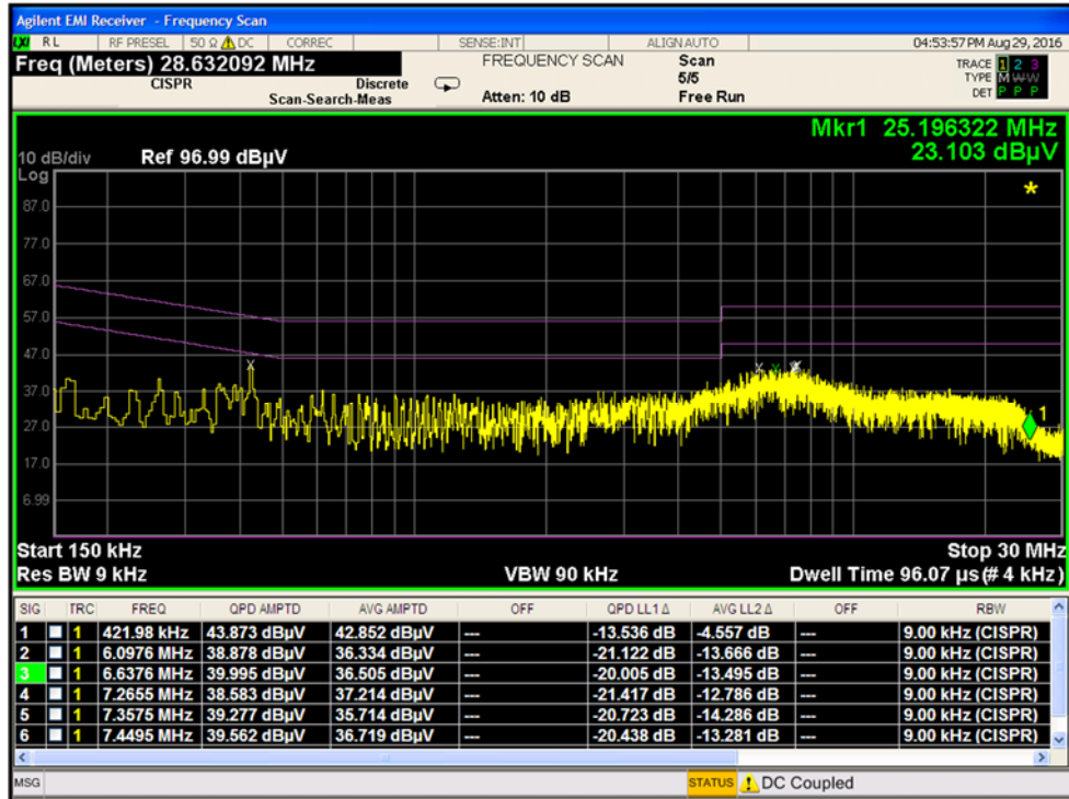
Plot 7-57. Line Conducted Plot with 802.11b (L1)
