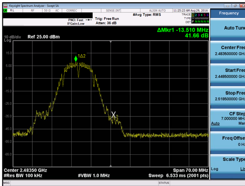
Plot 7-23. Band Edge Plot (802.11b – Ch. 13)
