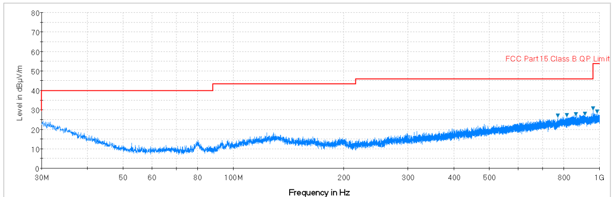
Plot 7-55. Radiated Spurious Plot below 1GHz (Pol. H)
