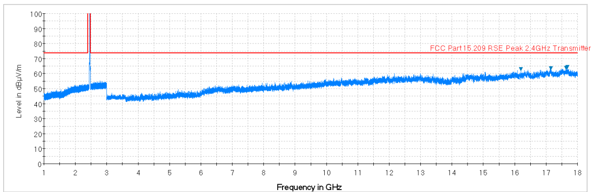
Plot 7-44. Radiated Spurious Plot above 1GHz (802.11b – Ch. 11, Ant. Pol. H)
