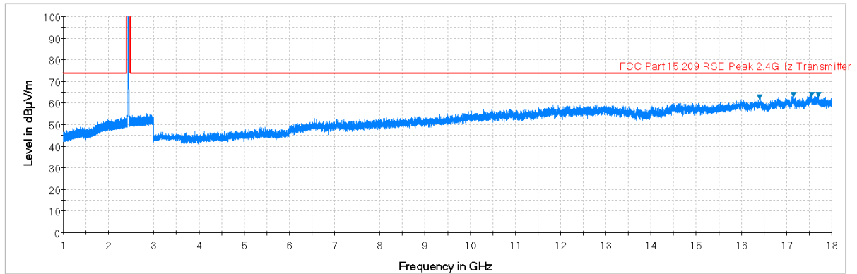
Plot 7-43. Radiated Spurious Plot above 1GHz (802.11b – Ch. 6, Ant. Pol. V)
