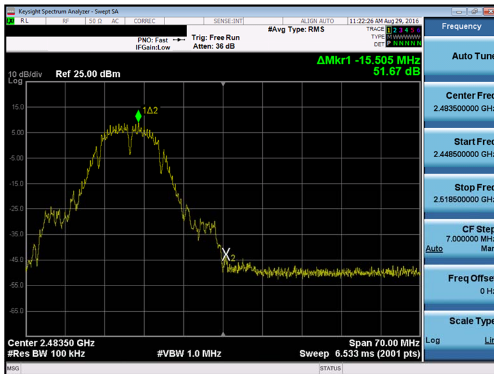
Plot 7-22. Band Edge Plot (802.11b – Ch. 12)
