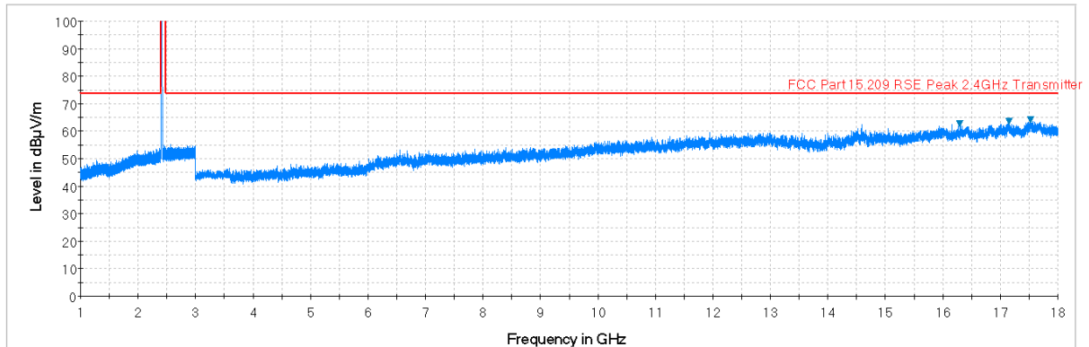
Plot 7-40. Radiated Spurious Plot above 1GHz (802.11b – Ch. 1, Ant. Pol. H)
