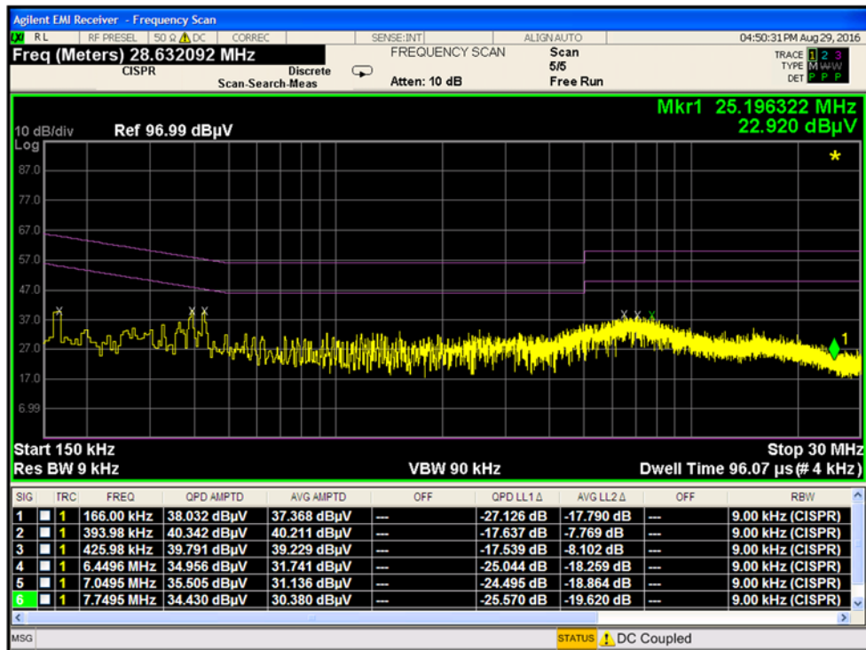
Plot 7-58. Line Conducted Plot with 802.11b (N)
