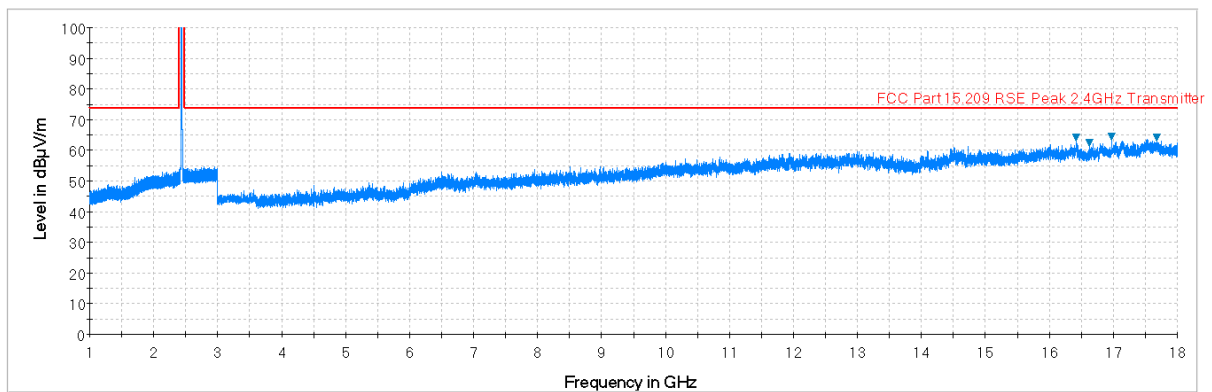
Plot 7-42. Radiated Spurious Plot above 1GHz (802.11b – Ch. 6, Ant. Pol. H)
