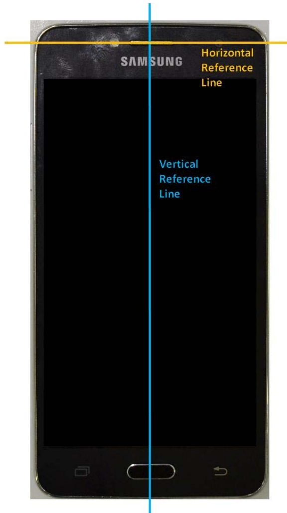
SAR Test Setup Photo 10: Vertical and Horizontal Reference Lines
