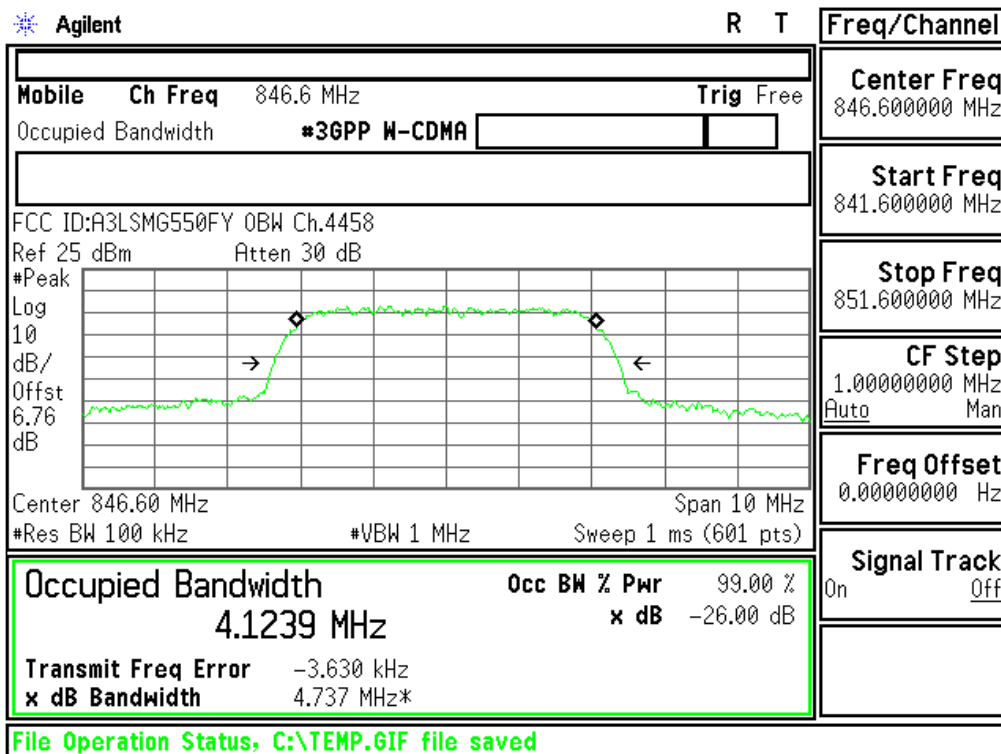
Plot 6-5. Occupied Bandwidth Plot (Cellular WCDMA Mode - Ch.4233(DL4458))
