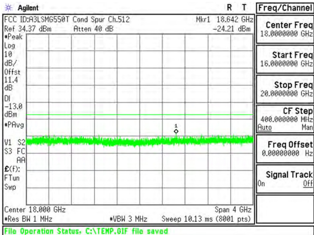
Plot 6-21. Conducted Spurious Plot (PCS GSM Mode - Ch.512)
