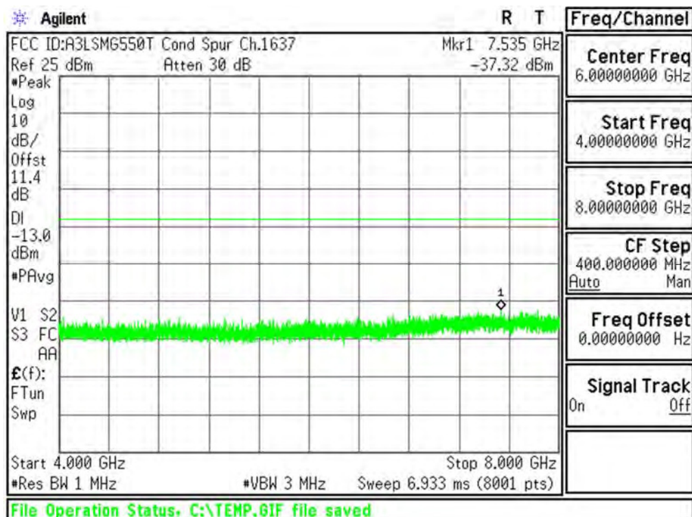
Plot 6-47. Conducted Spurious Plot (AWS WCDMA Mode - Ch.1412(DL1637))
