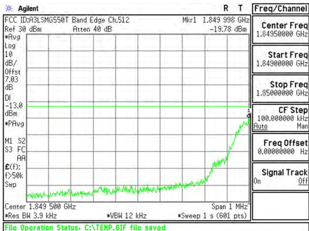
Plot 6-76. Lower Band Edge Plot (PCS GSM Mode – Ch.512)
