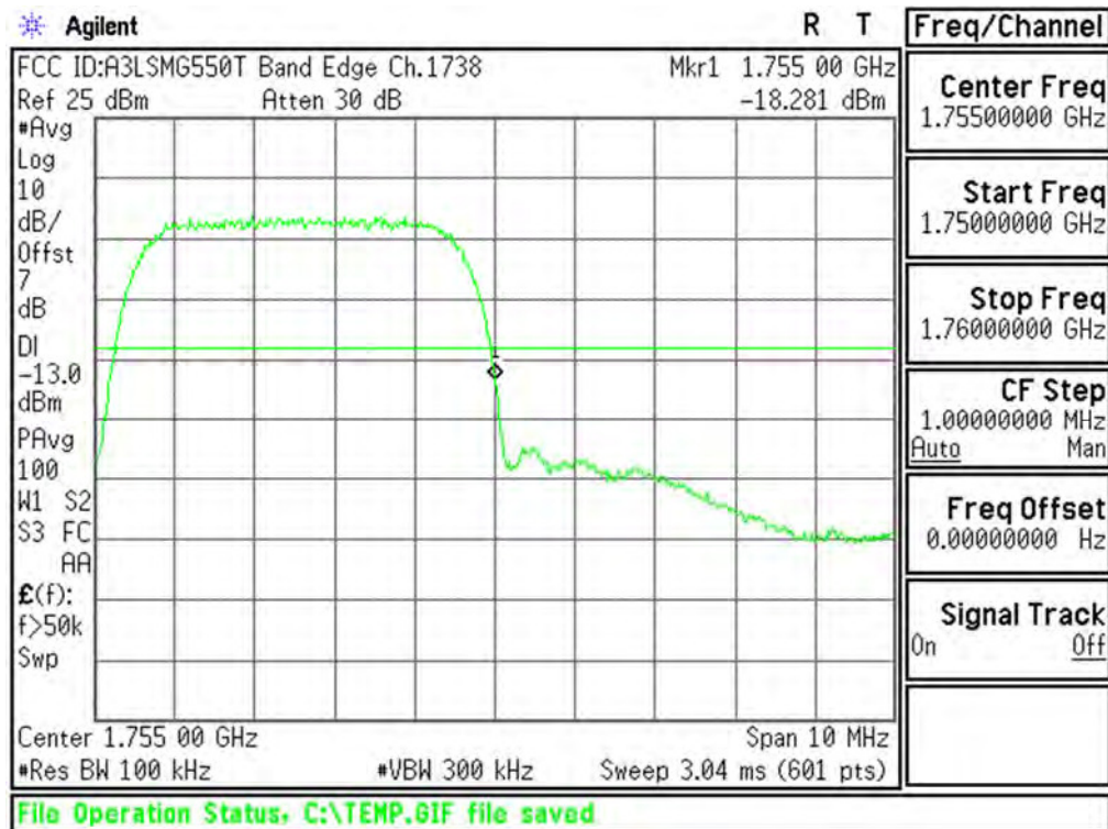
Plot 6-85. Upper Band Edge Plot (AWS WCDMA Mode - Ch.1513(DL1738))
