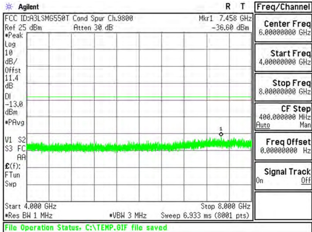
Plot 6-62. Conducted Spurious Plot (PCS WCDMA Mode - Ch.9400(DL9800))
