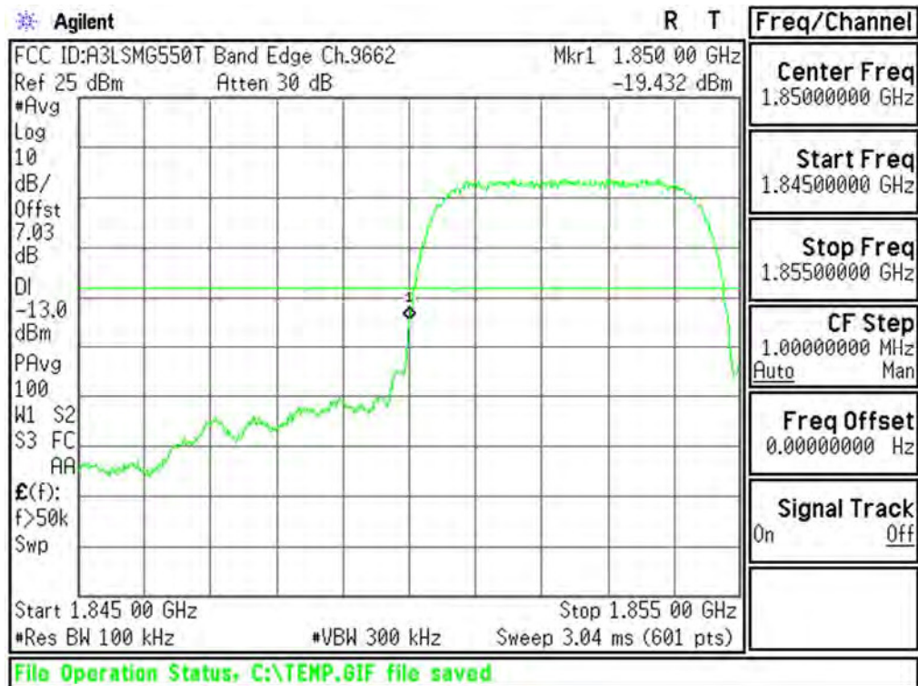
Plot 6-87. Lower Band Edge Plot (PCS WCDMA Mode - Ch.9262(DL9662))
