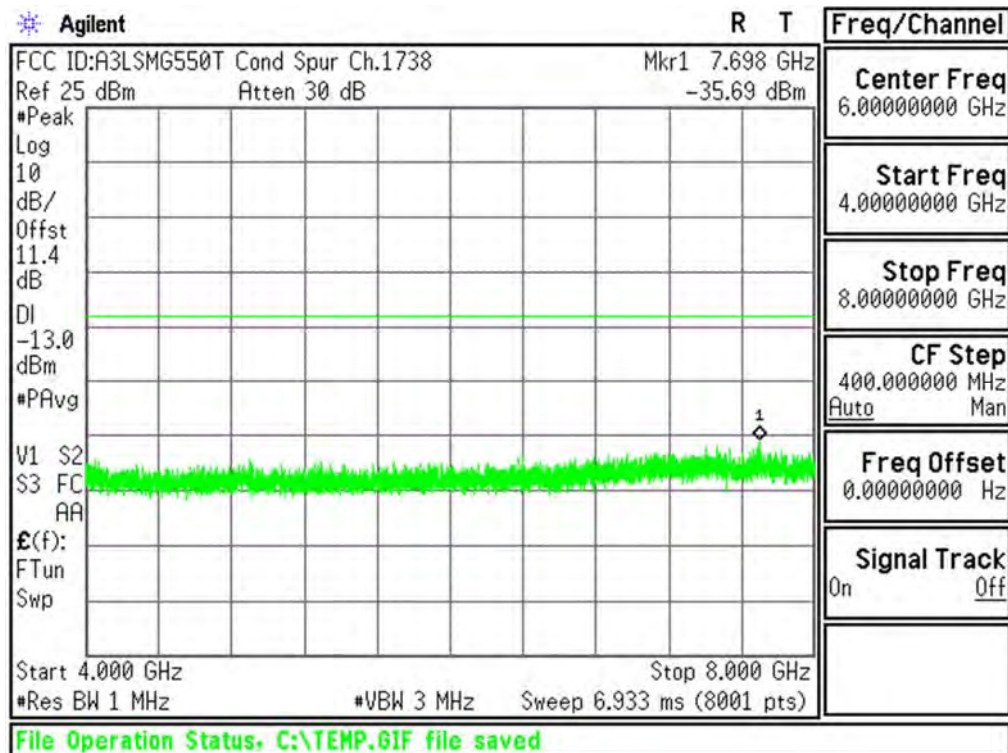
Plot 6-52. Conducted Spurious Plot (AWS WCDMA Mode - Ch.1513(DL1738))
