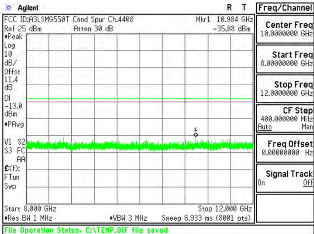
Plot 6-37. Conducted Spurious Plot (Cellular WCDMA Mode - Ch.4183(DL4408))
