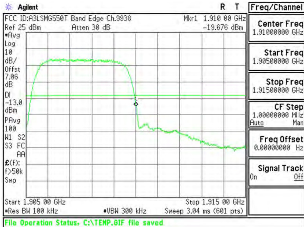
Plot 6-89. Upper Band Edge Plot (PCS WCDMA Mode - Ch.9538(DL9938))
