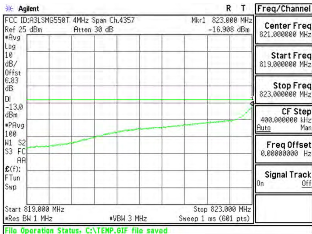
Plot 6-80. Extended Lower Band Edge Plot (Cellular WCDMA Mode - Ch.4132(DL4357))
