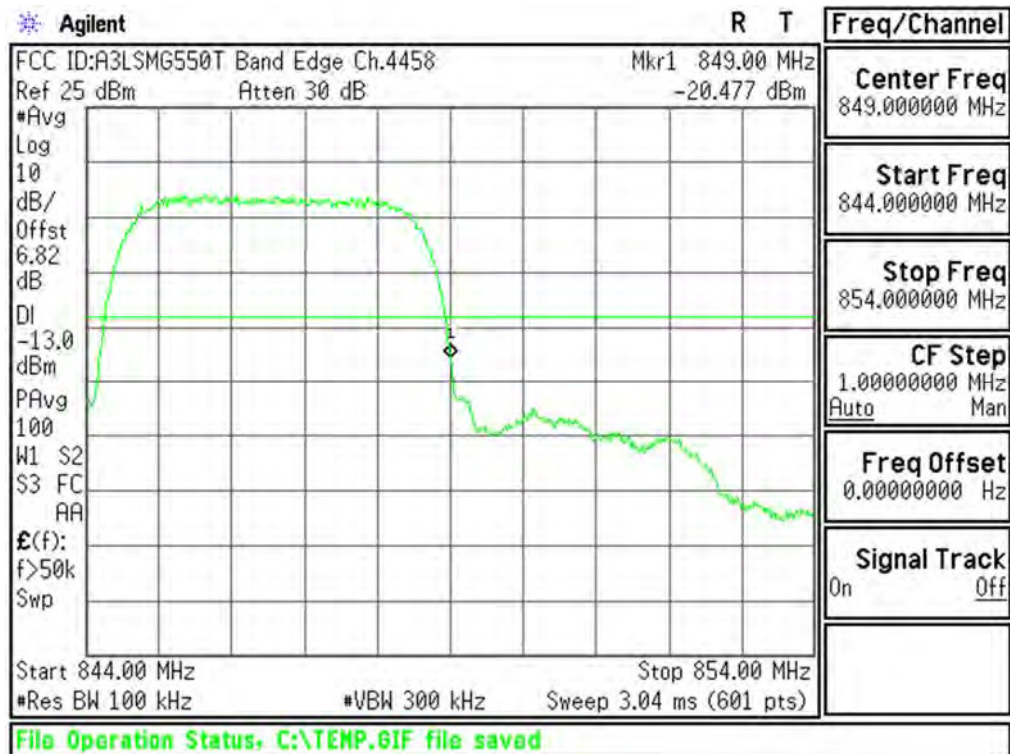
Plot 6-81. Upper Band Edge Plot (Cellular WCDMA Mode - Ch.4233(DL4458))
