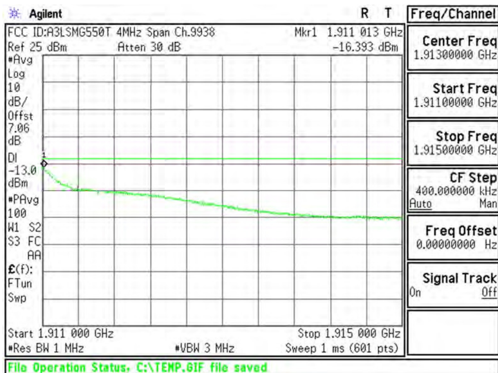
Plot 6-90. Extended Upper Band Edge Plot (PCS WCDMA Mode - Ch.9538(DL9938))
