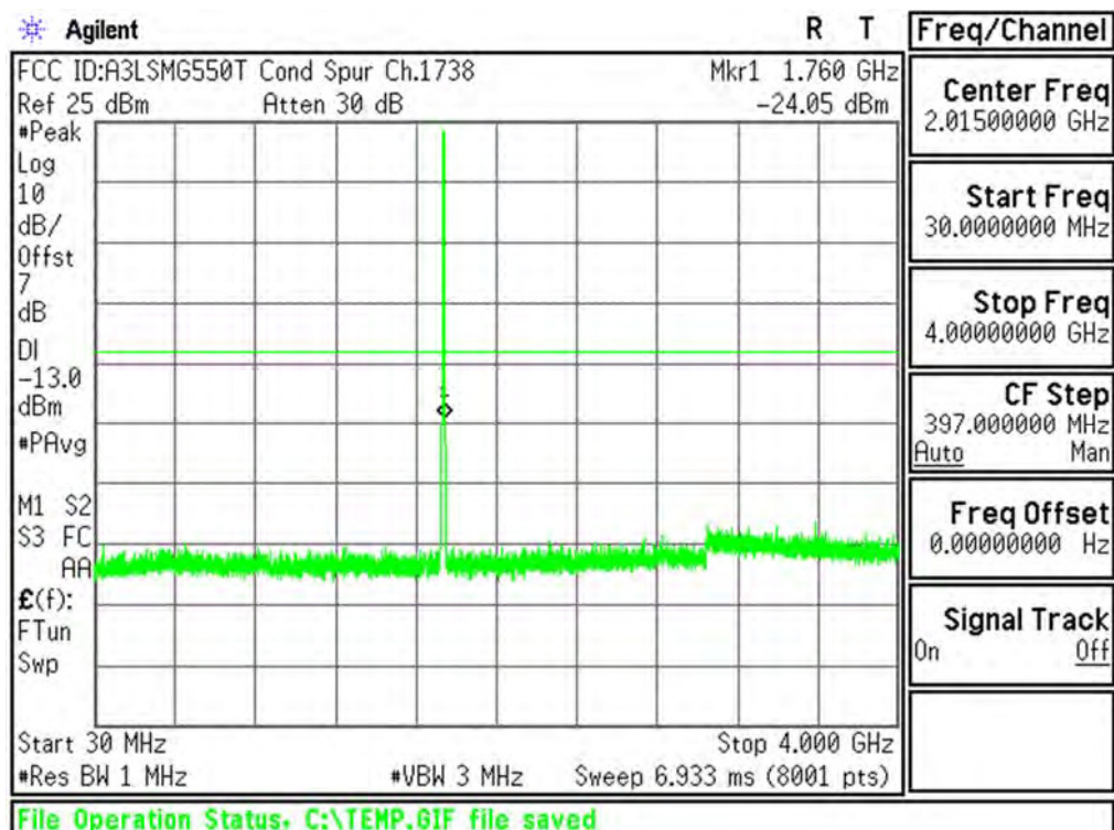
Plot 6-51. Conducted Spurious Plot (AWS WCDMA Mode - Ch.1513(DL1738))
