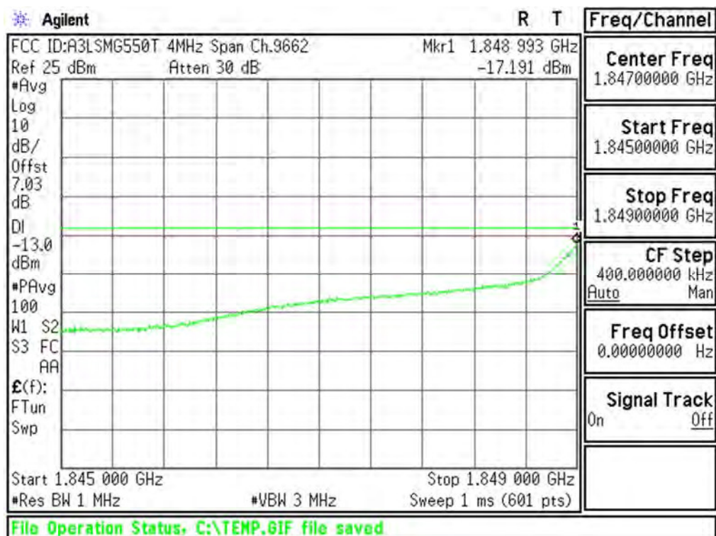
Plot 6-88. Extended Lower Band Edge Plot (PCS WCDMA Mode - Ch.9262(DL9662))
