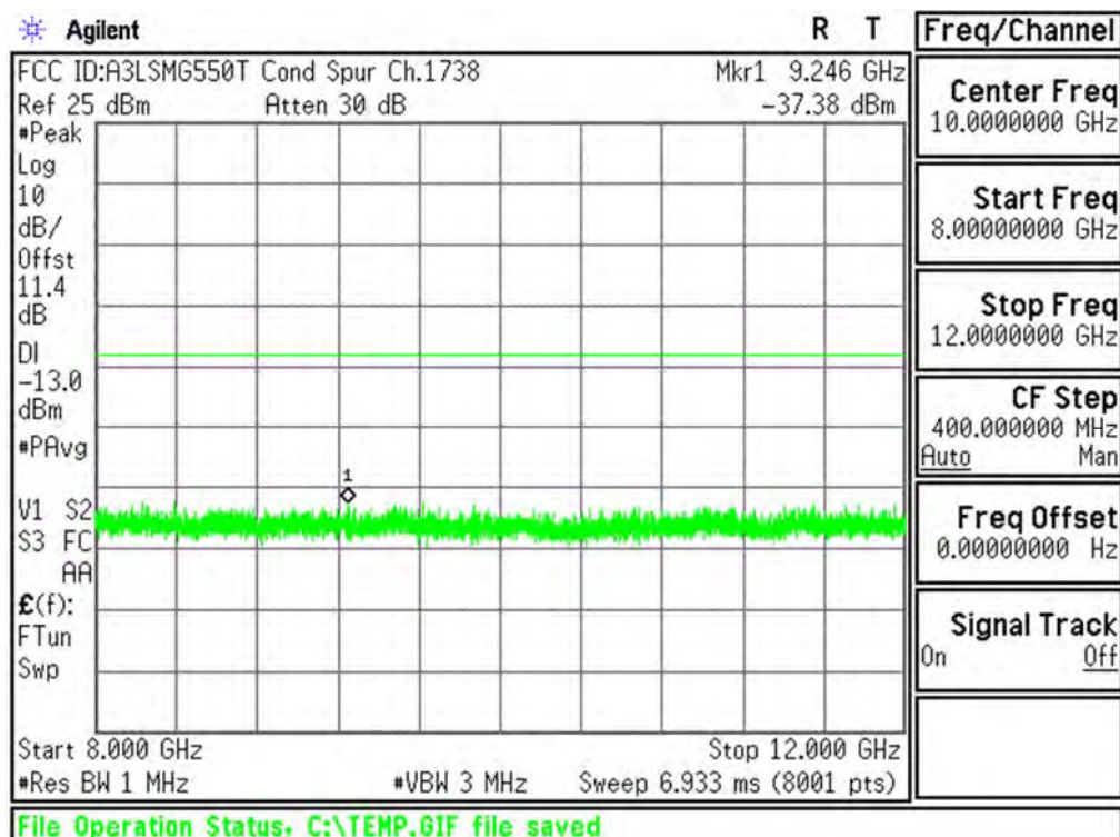
Plot 6-53. Conducted Spurious Plot (AWS WCDMA Mode - Ch.1513(DL1738))
