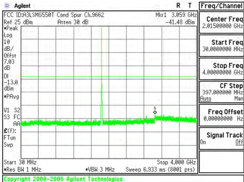
Plot 6-56. Conducted Spurious Plot (PCS WCDMA Mode - Ch.9262(DL9662))
