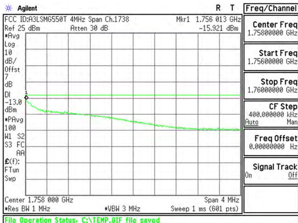
Plot 6-86. Extended Upper Band Edge Plot (AWS WCDMA Mode - Ch.1513(DL1738))
