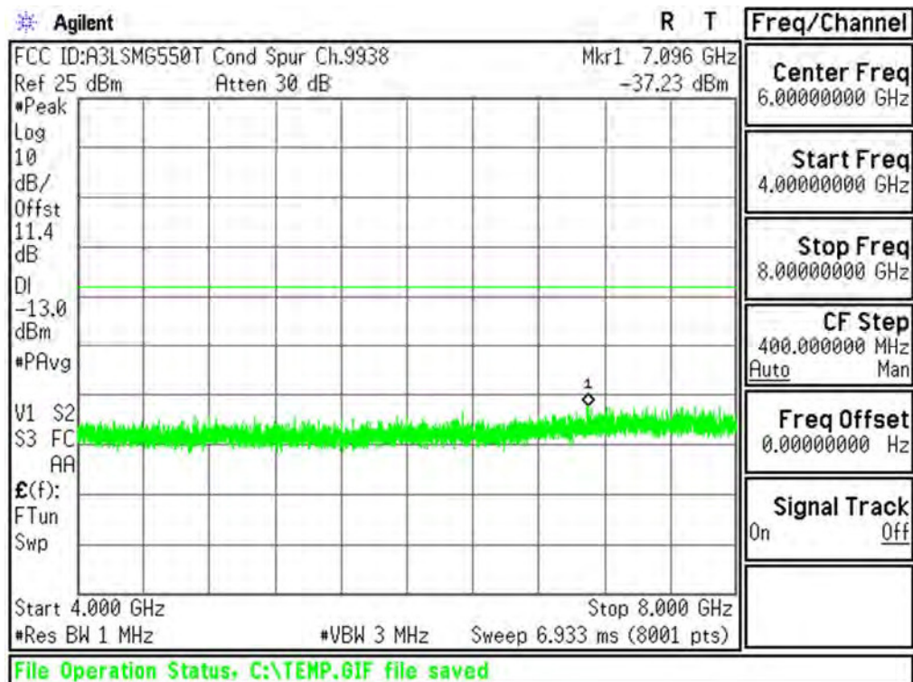
Plot 6-67. Conducted Spurious Plot (PCS WCDMA Mode - Ch.9538(DL9938))
