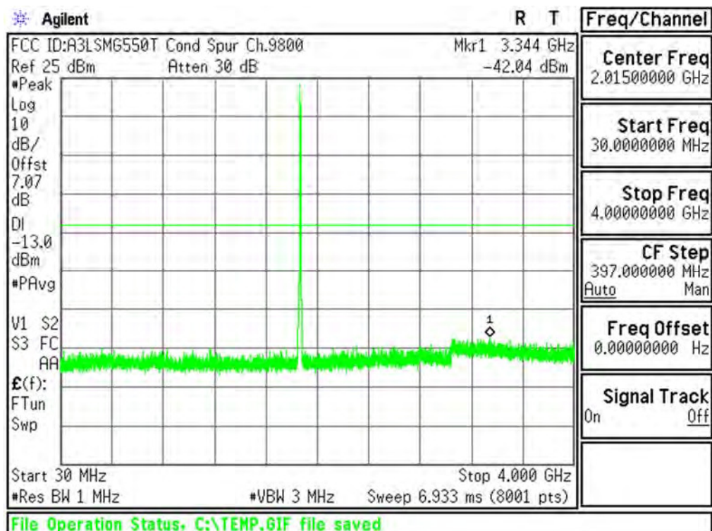
Plot 6-61. Conducted Spurious Plot (PCS WCDMA Mode - Ch.9400(DL9800))
