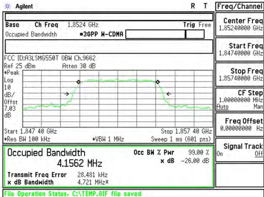
Plot 6-7. Occupied Bandwidth Plot (PCS WCDMA Mode - Ch.9262(DL9662))
