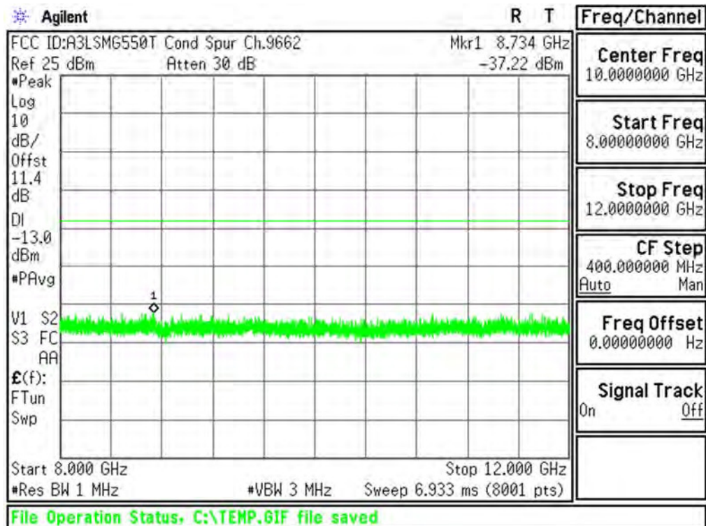
Plot 6-58. Conducted Spurious Plot (PCS WCDMA Mode - Ch.9262(DL9662))
