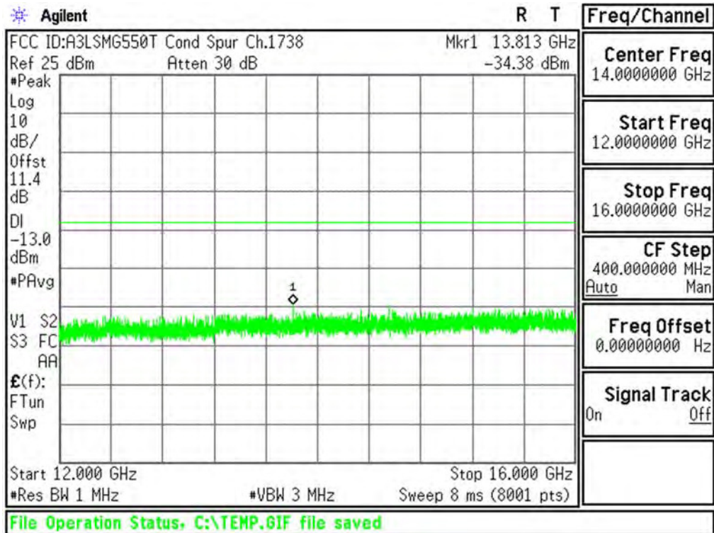
Plot 6-54. Conducted Spurious Plot (AWS WCDMA Mode - Ch.1513(DL1738))
