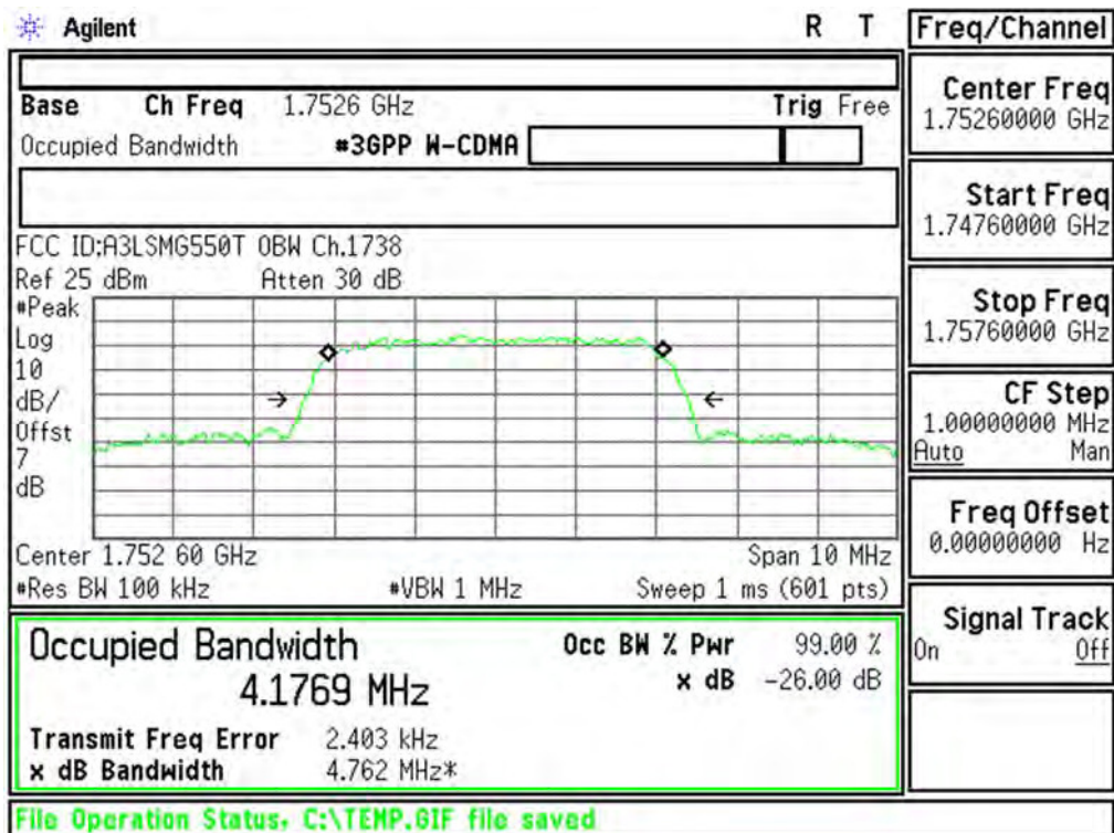
Plot 6-6. Occupied Bandwidth Plot (AWS WCDMA Mode - Ch.1513(DL1738))
