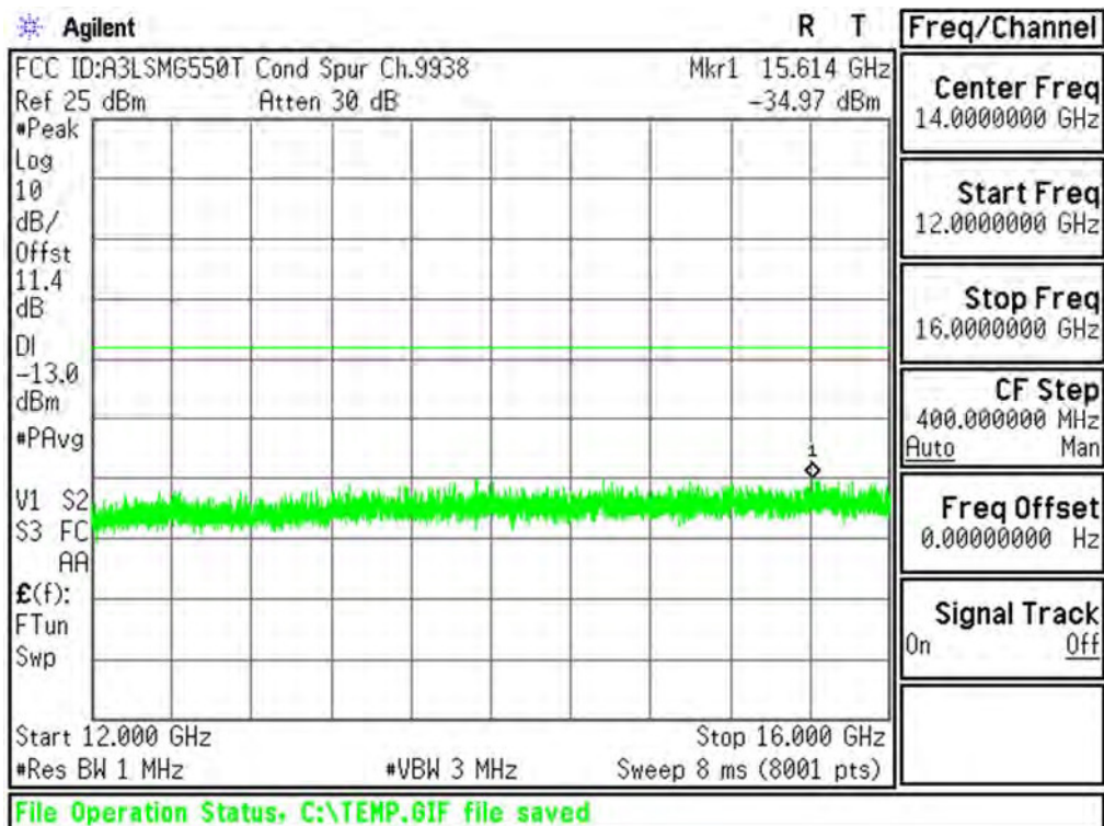
Plot 6-69. Conducted Spurious Plot (PCS WCDMA Mode - Ch.9538(DL9938))
