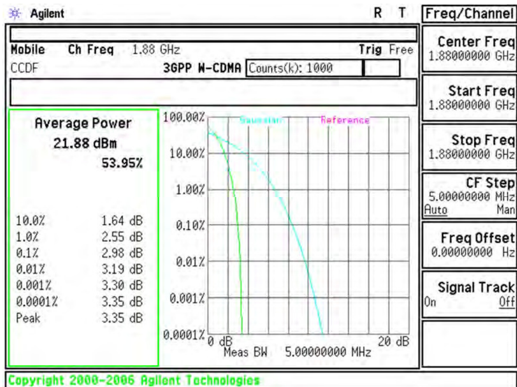
Plot 6-93. Peak-Average Ratio Plot (PCS WCDMA Mode - Ch.9400(DL9800))
