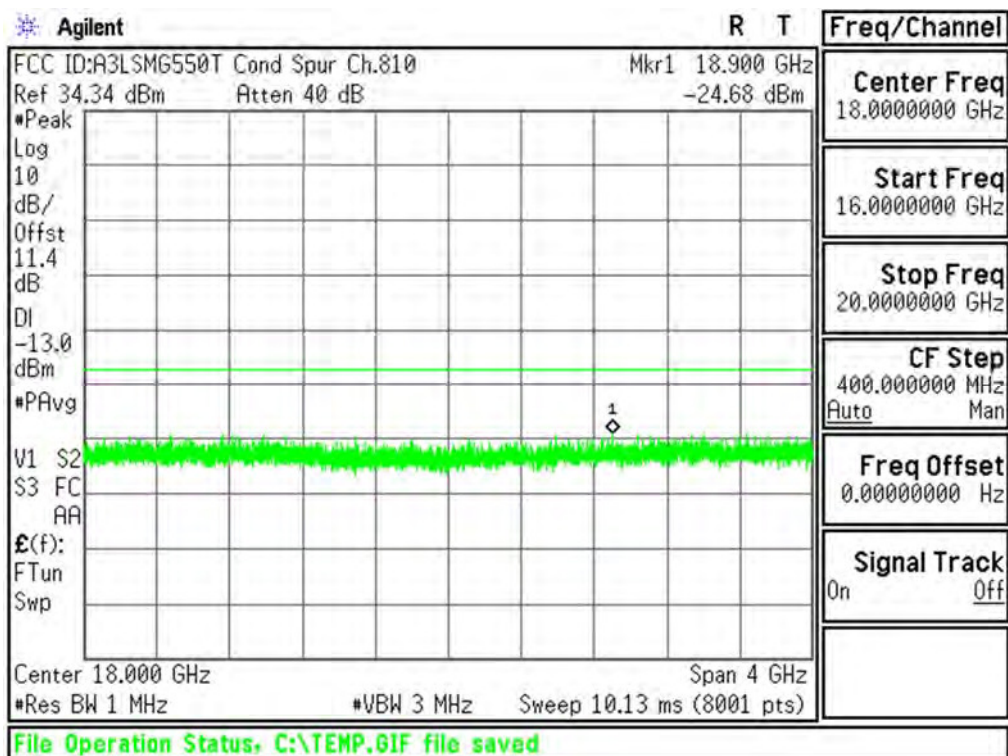
Plot 6-31. Conducted Spurious Plot (PCS GSM Mode - Ch.810)
