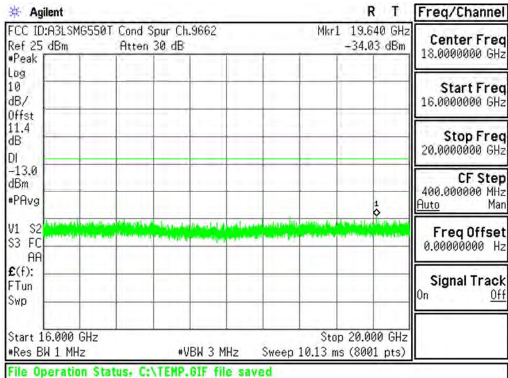
Plot 6-60. Conducted Spurious Plot (PCS WCDMA Mode - Ch.9262(DL9662))
