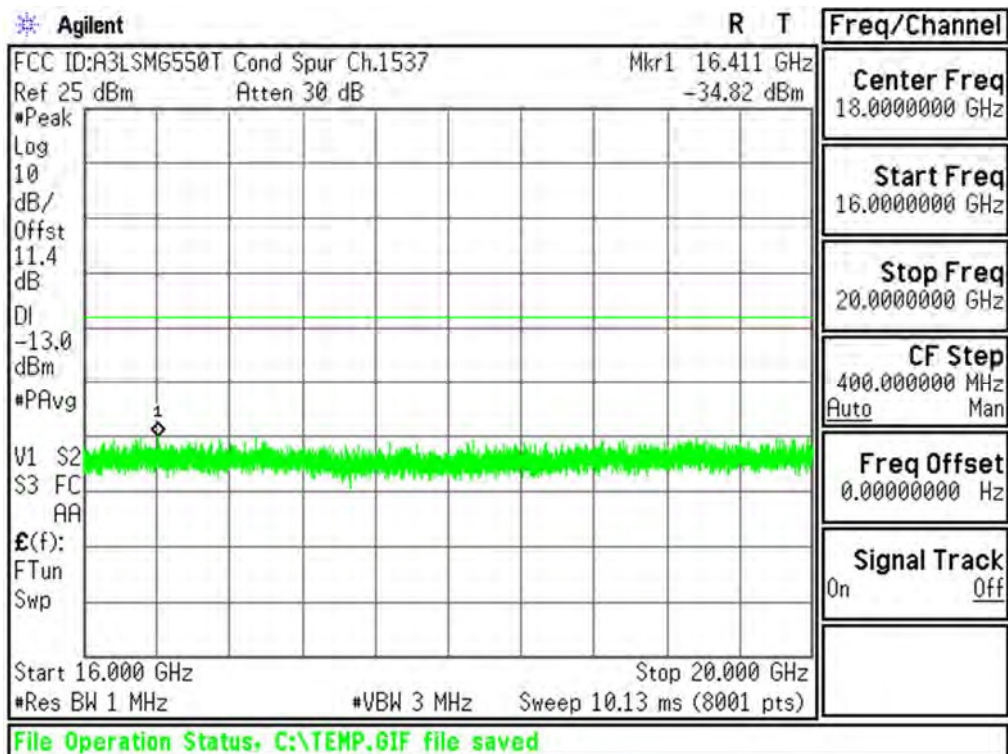
Plot 6-45. Conducted Spurious Plot (AWS WCDMA Mode - Ch.1312(DL1537))
