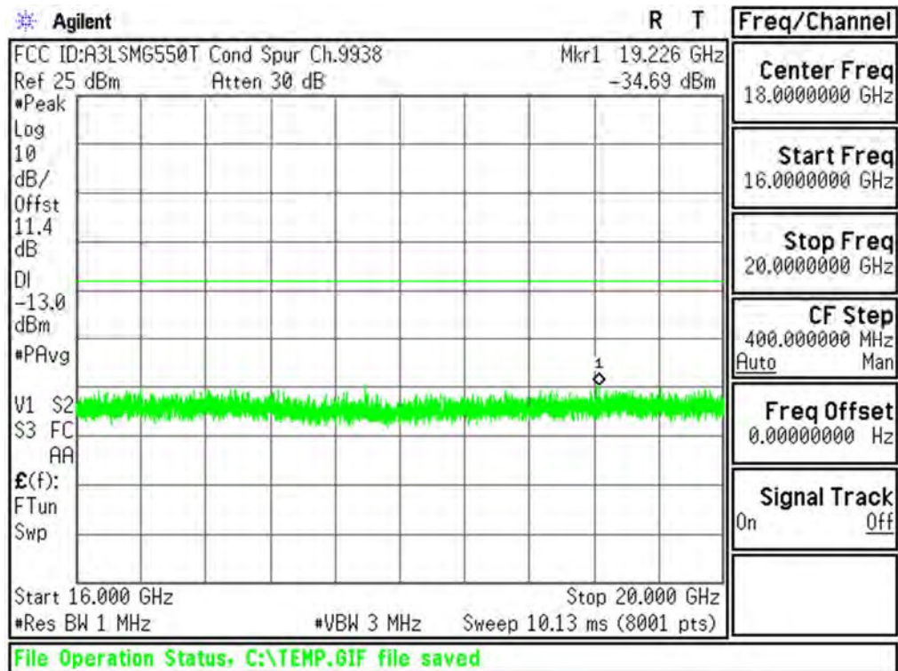
Plot 6-70. Conducted Spurious Plot (PCS WCDMA Mode - Ch.9538(DL9938))
