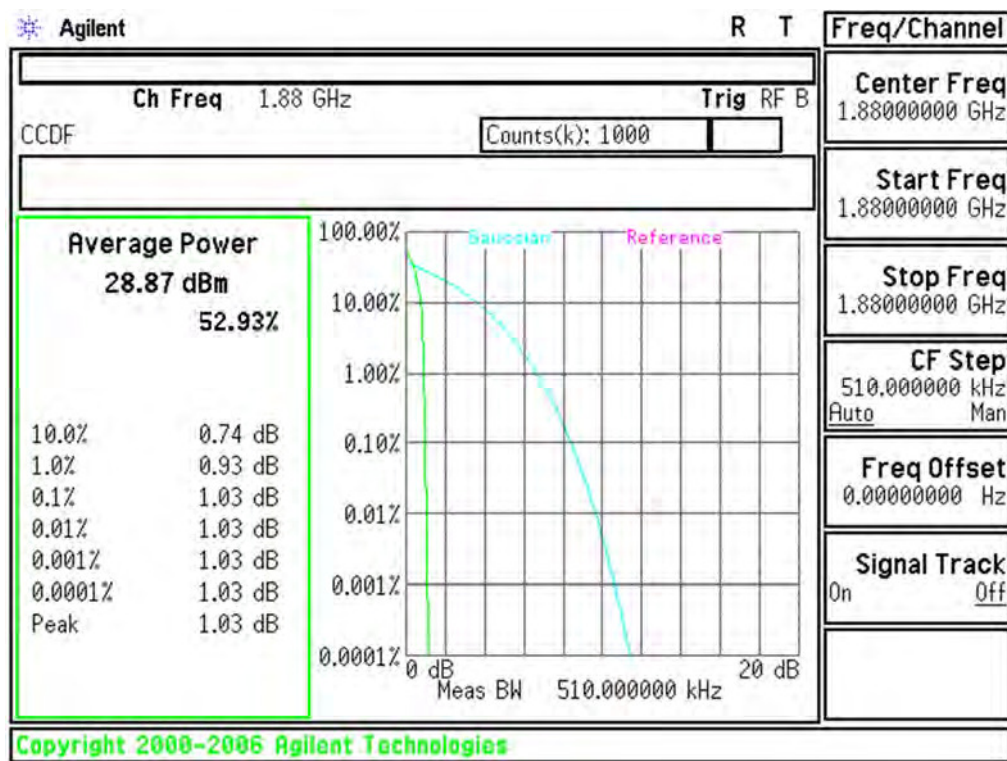
Plot 6-92. Peak-Average Ratio Plot (EDGE1900 Mode - Ch.661)
