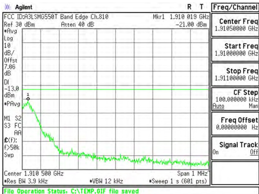
Plot 6-78. Upper Band Edge Plot (PCS GSM Mode – Ch.810)
