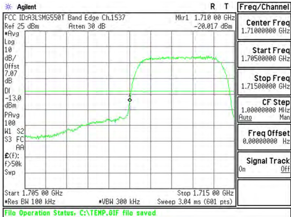
Plot 6-83. Lower Band Edge Plot (AWS WCDMA Mode - Ch.1312(DL1537))
