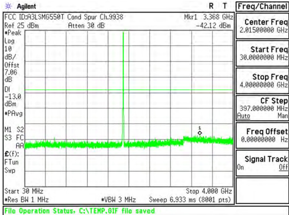
Plot 6-66. Conducted Spurious Plot (PCS WCDMA Mode - Ch.9538(DL9938))
