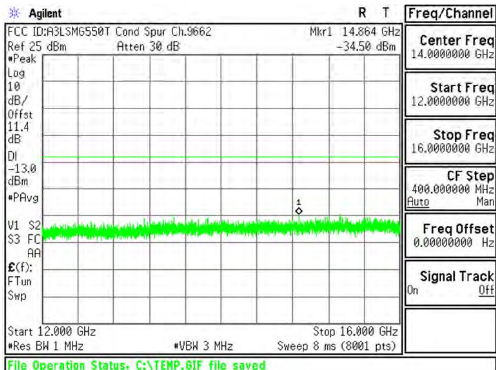
Plot 6-59. Conducted Spurious Plot (PCS WCDMA Mode - Ch.9262(DL9662))
