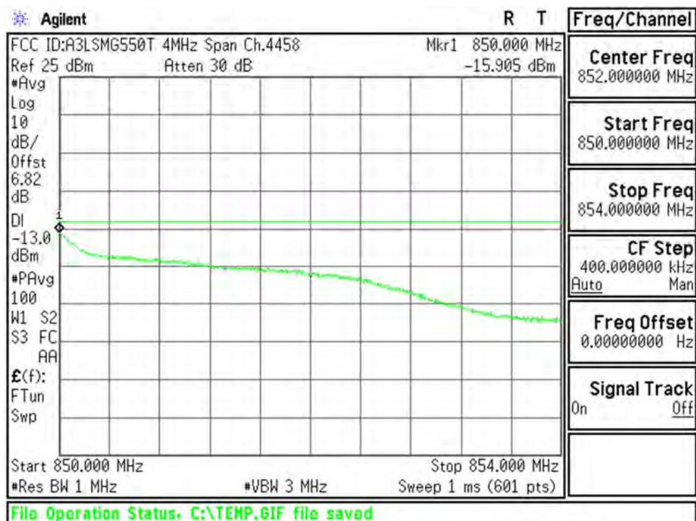
Plot 6-82. Extended Upper Band Edge Plot (Cellular WCDMA Mode - Ch.4233(DL4458))
