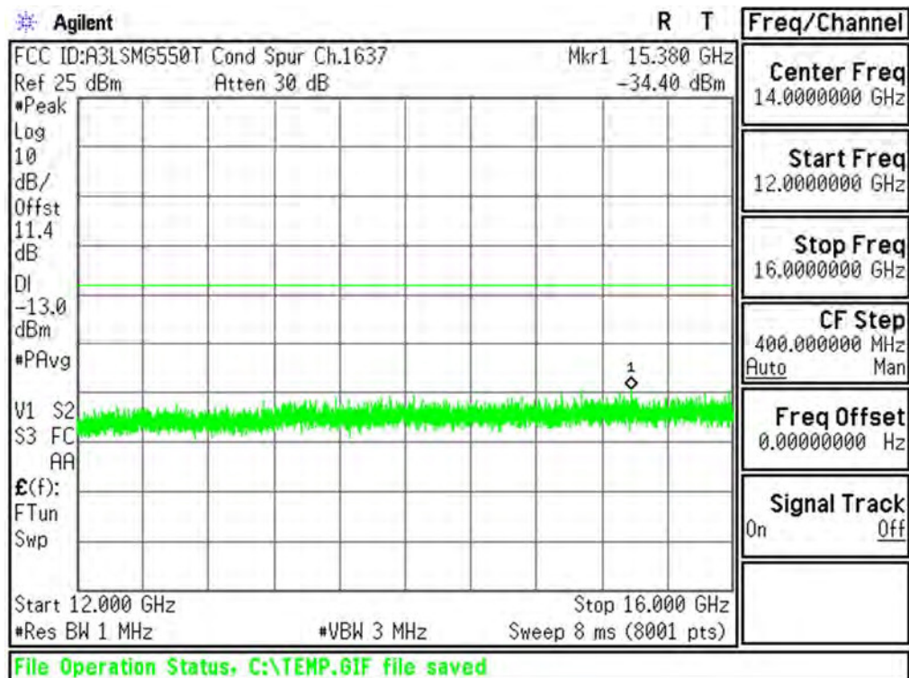
Plot 6-49. Conducted Spurious Plot (AWS WCDMA Mode - Ch.1412(DL1637))
