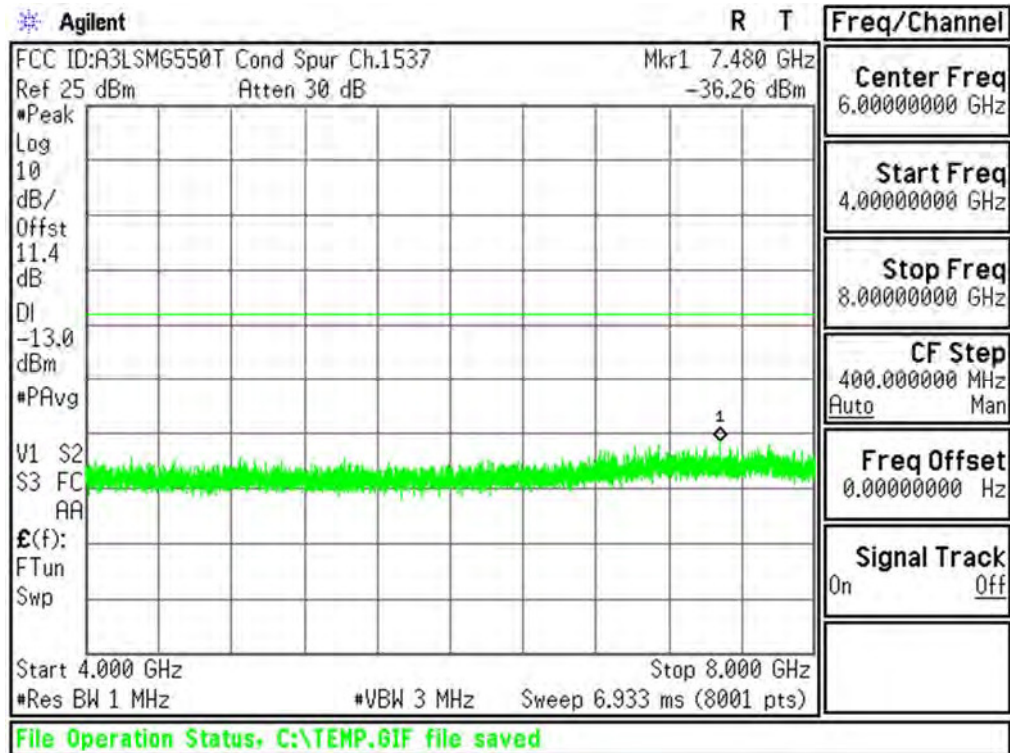
Plot 6-42. Conducted Spurious Plot (AWS WCDMA Mode - Ch.1312(DL1537))
