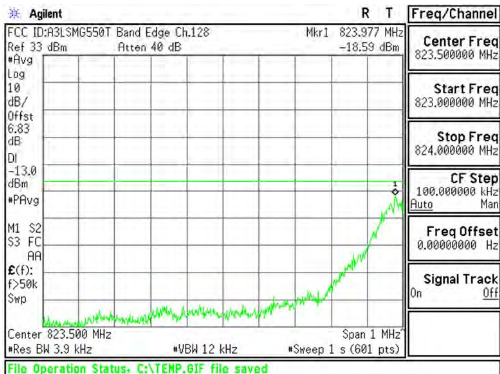
Plot 6-72. Lower Band Edge Plot (Cellular GSM Mode – Ch.128)
