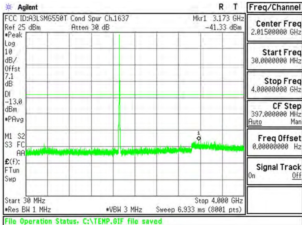
Plot 6-46. Conducted Spurious Plot (AWS WCDMA Mode - Ch.1412(DL1637))
