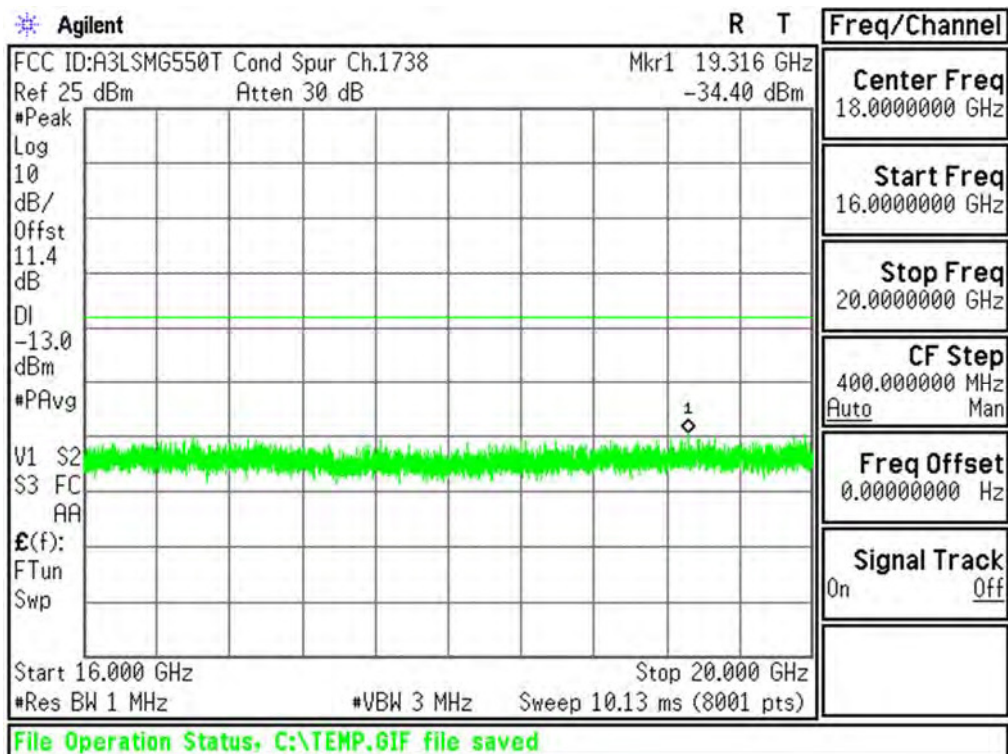
Plot 6-55. Conducted Spurious Plot (AWS WCDMA Mode - Ch.1513(DL1738))
