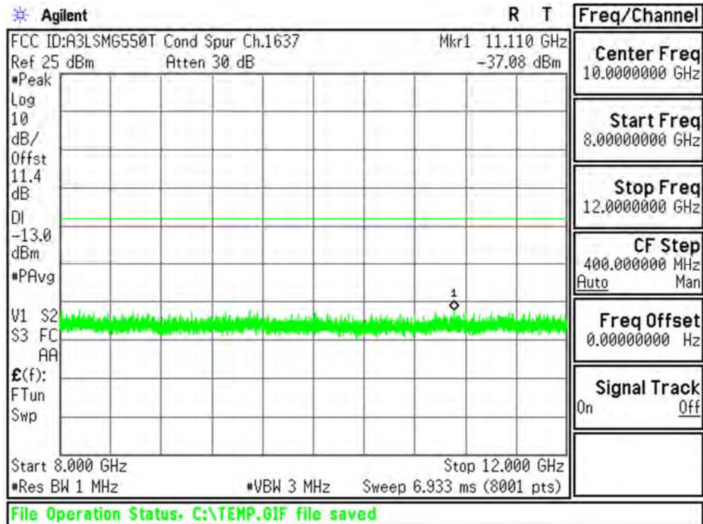
Plot 6-48. Conducted Spurious Plot (AWS WCDMA Mode - Ch.1412(DL1637))
