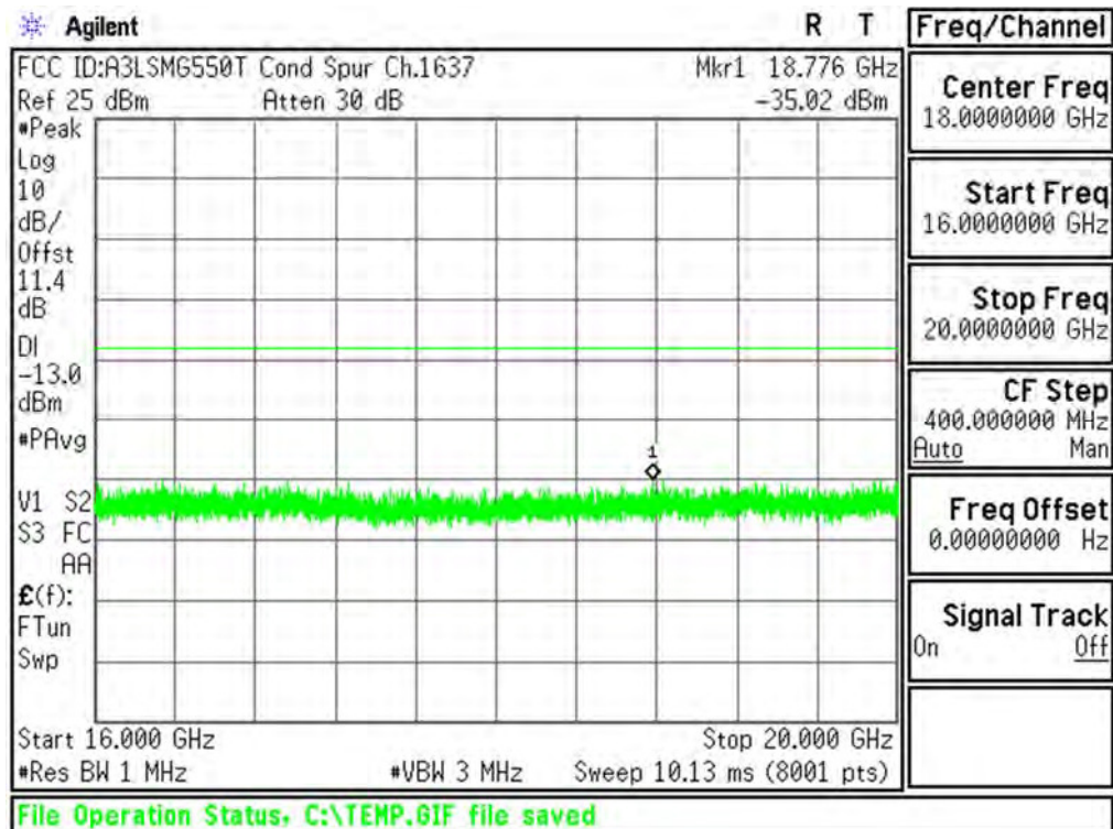
Plot 6-50. Conducted Spurious Plot (AWS WCDMA Mode - Ch.1412(DL1637))
