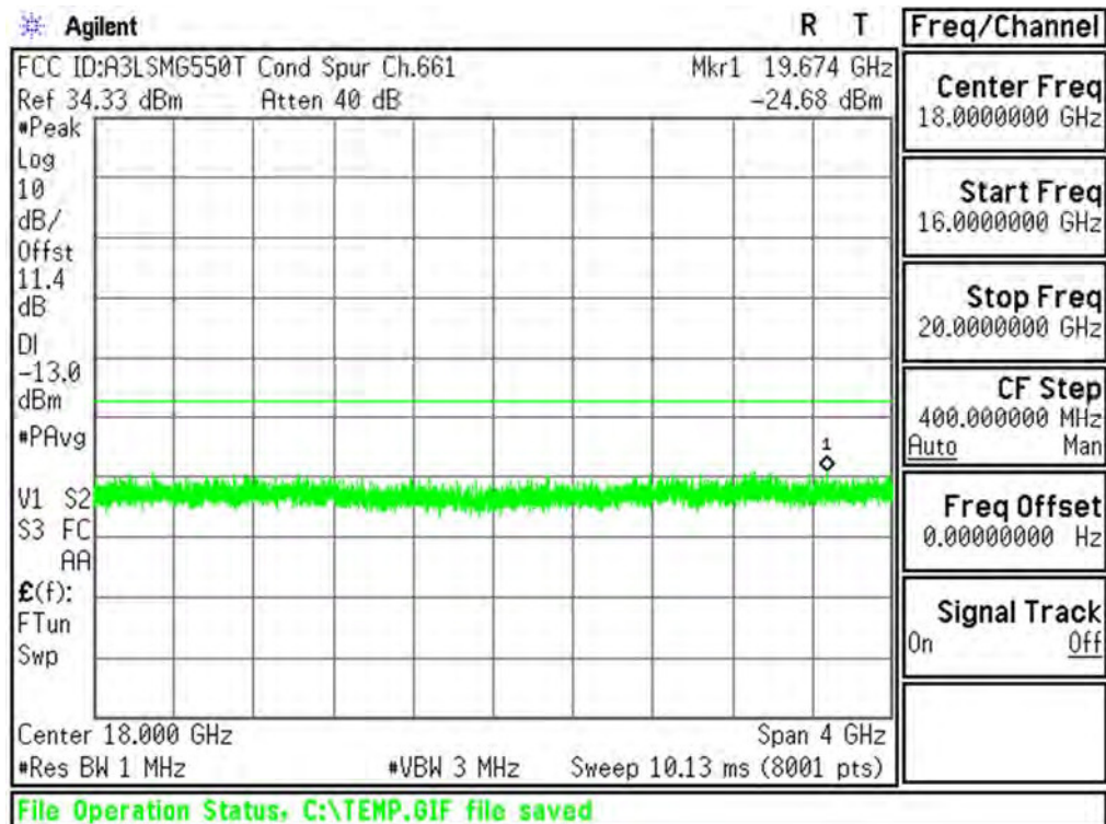
Plot 6-26. Conducted Spurious Plot (PCS GSM Mode - Ch.661)
