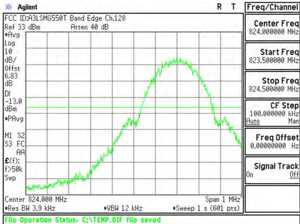
Plot 6-71. Lower Band Edge Plot (Cellular GSM Mode – Ch.128)
