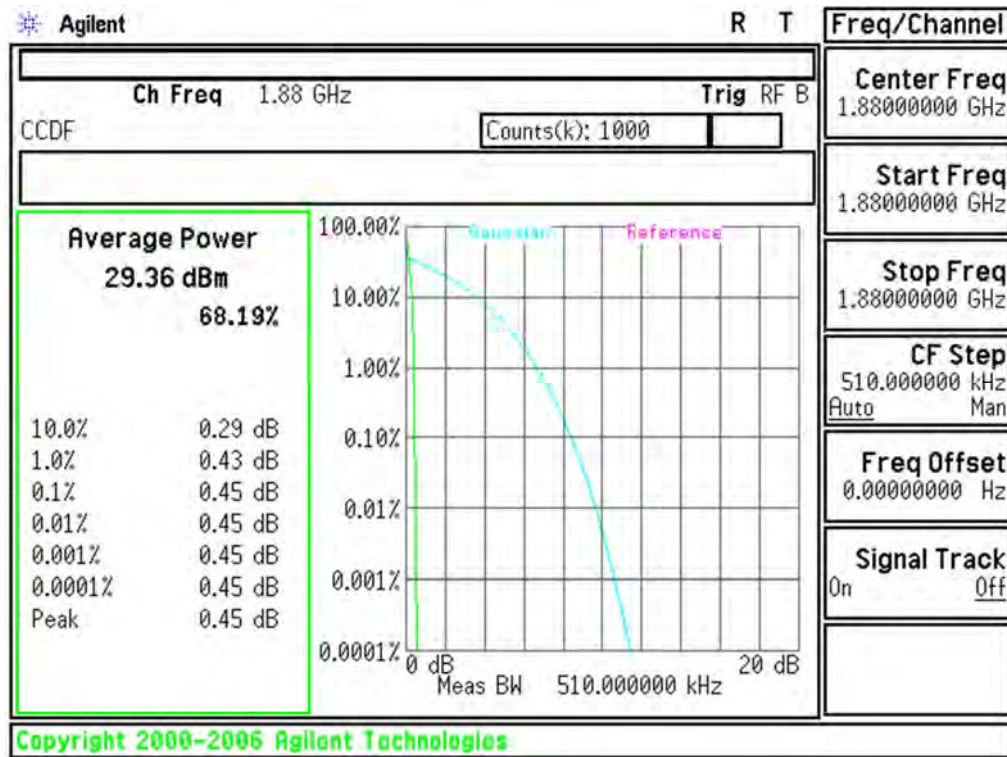
Plot 6-91. Peak-Average Ratio Plot (PCS GSM Mode - Ch.661)
