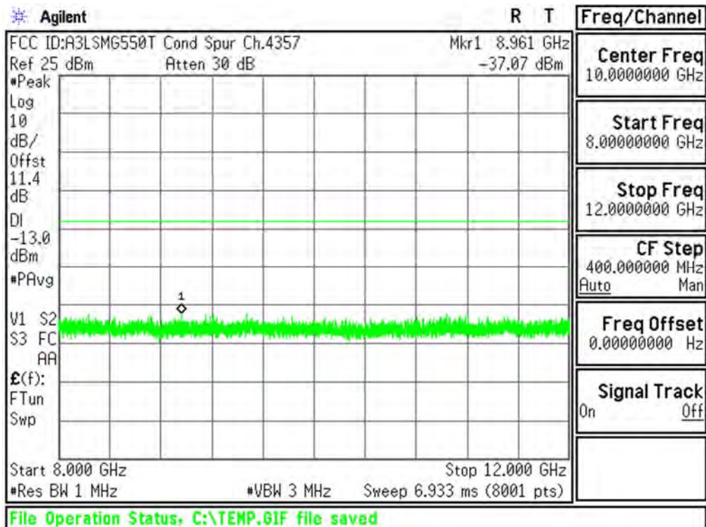
Plot 6-34. Conducted Spurious Plot (Cellular WCDMA Mode - Ch.4132(DL4357))
