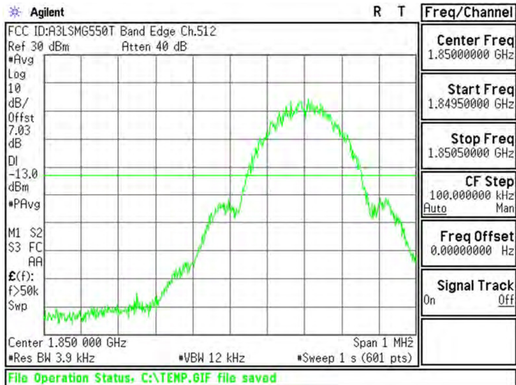
Plot 6-75. Lower Band Edge Plot (PCS GSM Mode – Ch.512)
