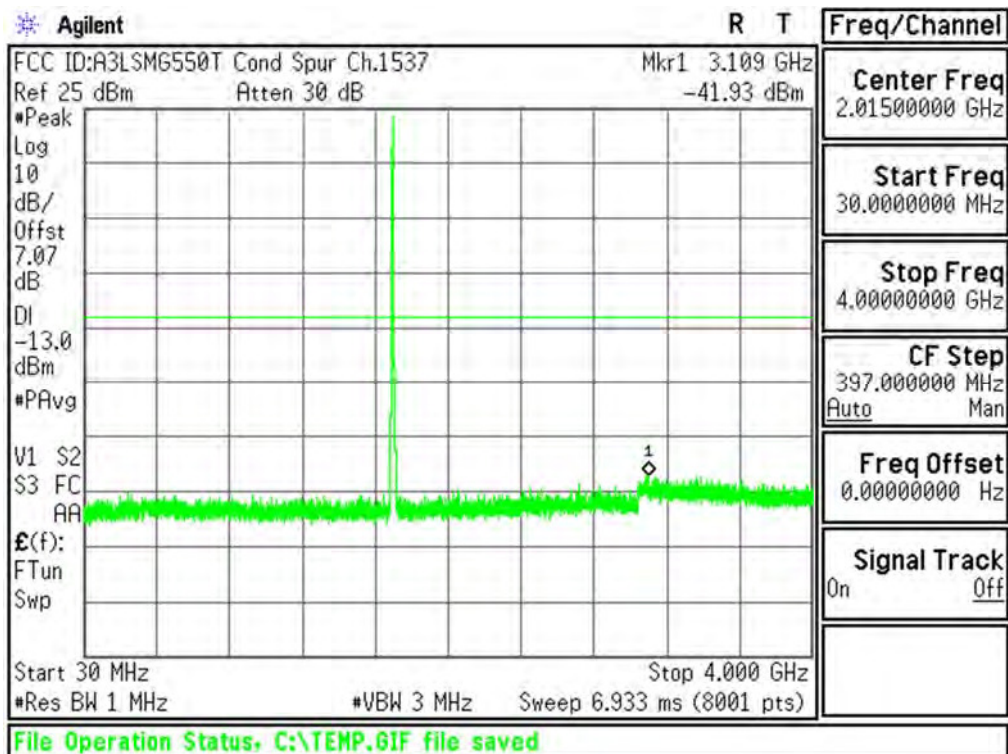
Plot 6-41. Conducted Spurious Plot (AWS WCDMA Mode - Ch.1312(DL1537))
