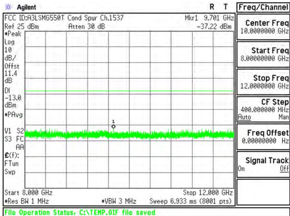
Plot 6-43. Conducted Spurious Plot (AWS WCDMA Mode - Ch.1312(DL1537))
