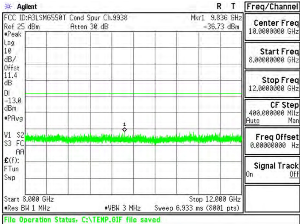
Plot 6-68. Conducted Spurious Plot (PCS WCDMA Mode - Ch.9538(DL9938))
