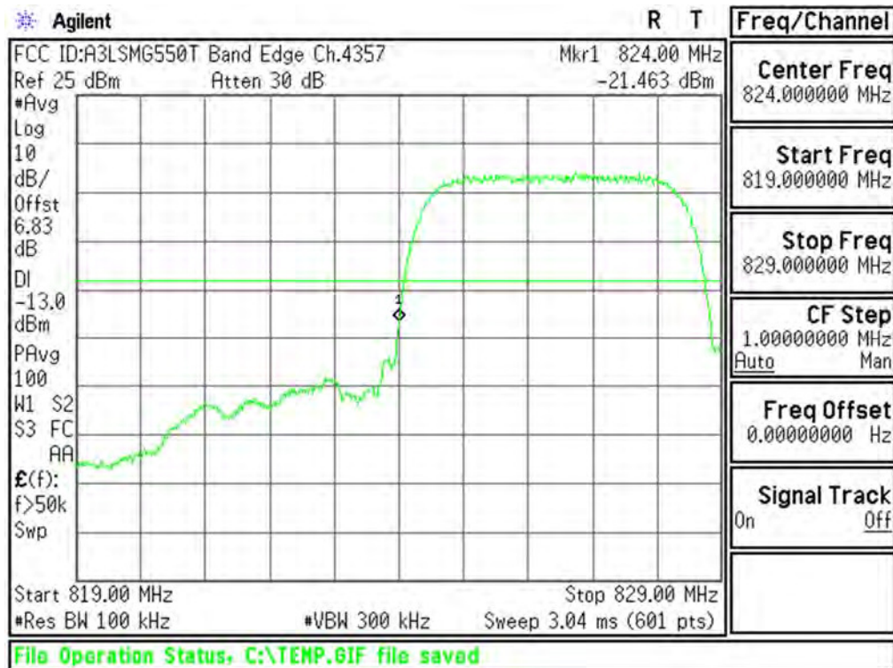
Plot 6-79. Lower Band Edge Plot (Cellular WCDMA Mode - Ch.4132(DL4357))
