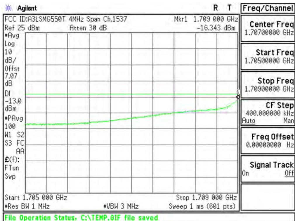
Plot 6-84. Extended Lower Band Edge Plot (AWS WCDMA Mode - Ch.1312(DL1537))
