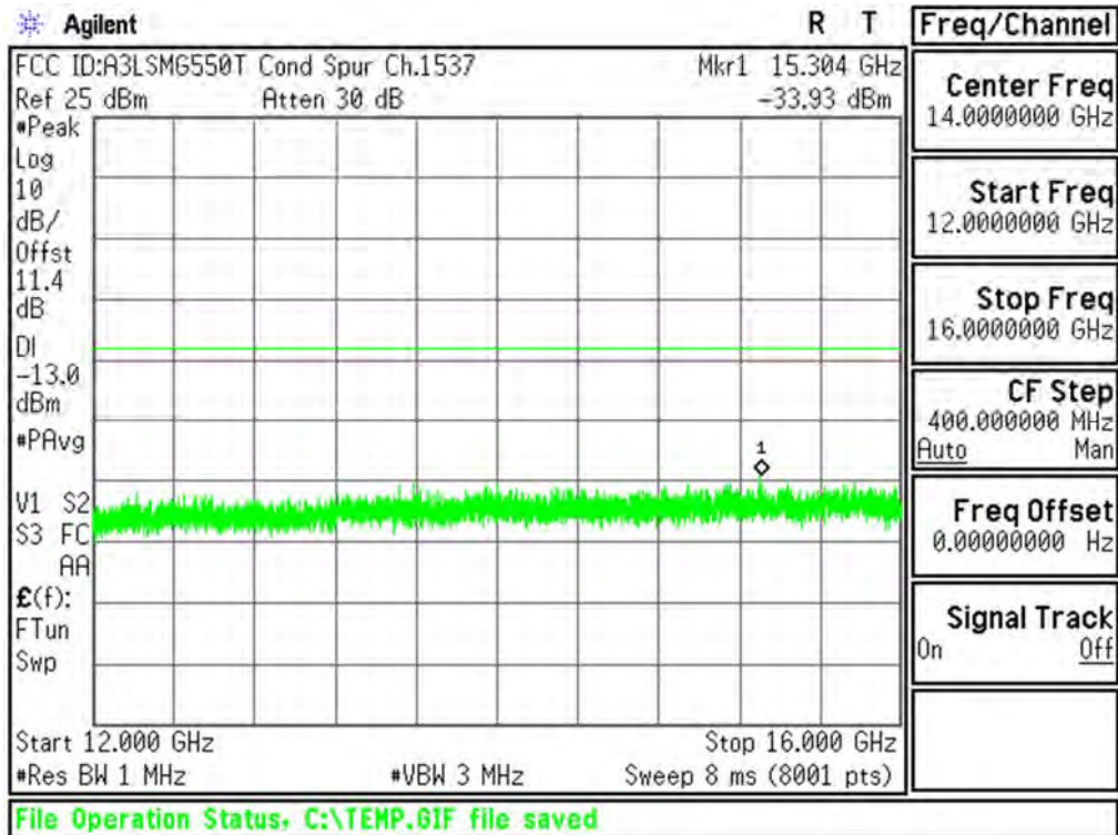
Plot 6-44. Conducted Spurious Plot (AWS WCDMA Mode - Ch.1312(DL1537))
