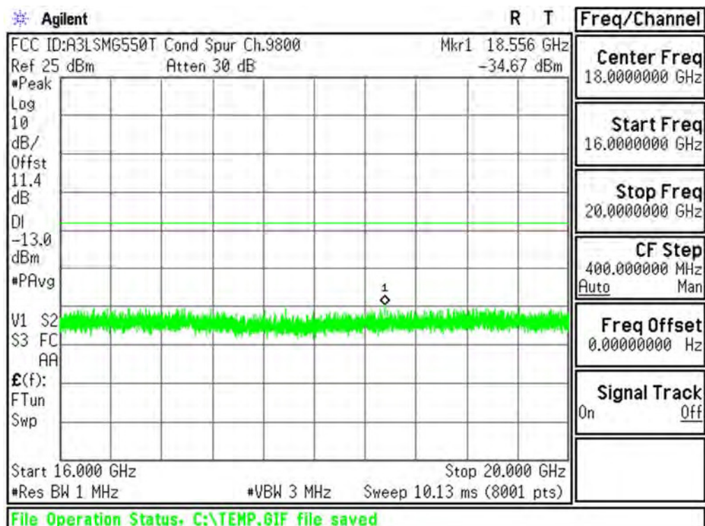
Plot 6-65. Conducted Spurious Plot (PCS WCDMA Mode - Ch.9400(DL9800))
