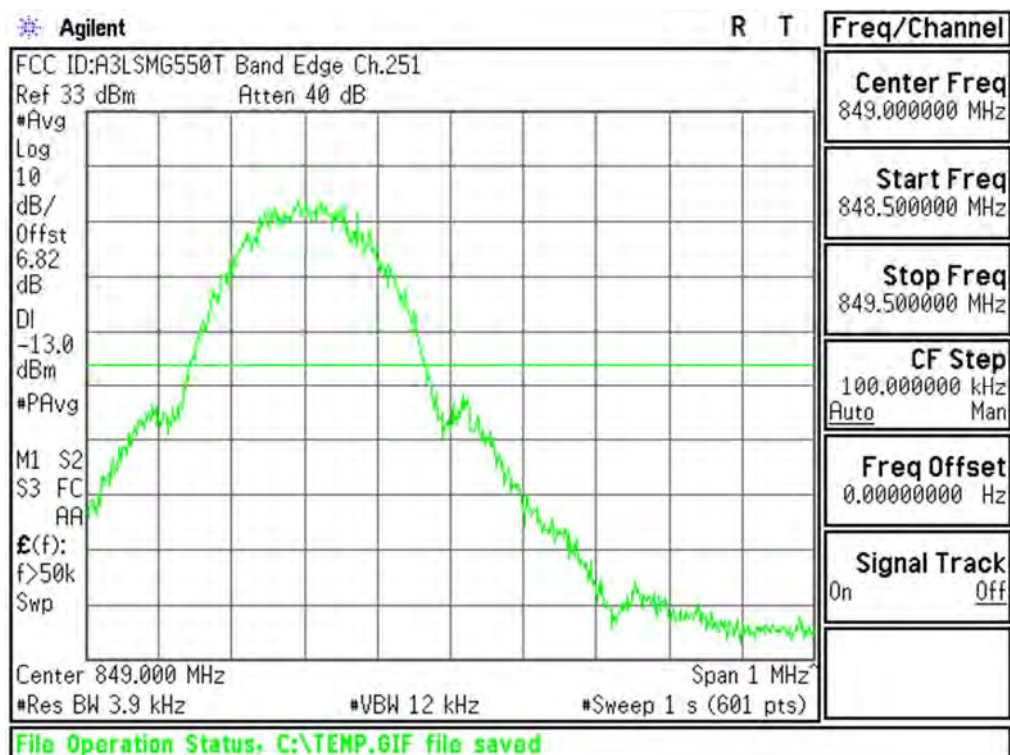
Plot 6-73. Upper Band Edge Plot (Cellular GSM Mode – Ch.251)
