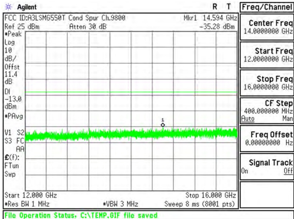
Plot 6-64. Conducted Spurious Plot (PCS WCDMA Mode - Ch.9400(DL9800))
