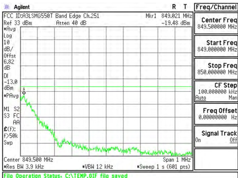
Plot 6-74. Upper Band Edge Plot (Cellular GSM Mode – Ch.251)
