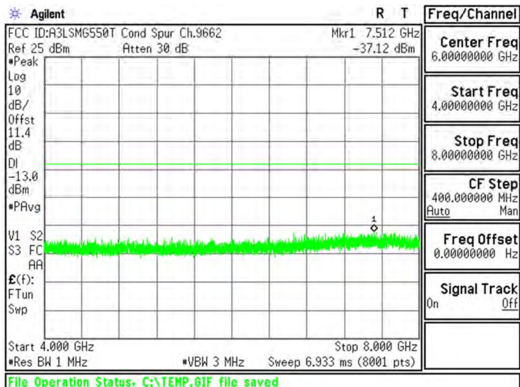
Plot 6-57. Conducted Spurious Plot (PCS WCDMA Mode - Ch.9262(DL9662))
