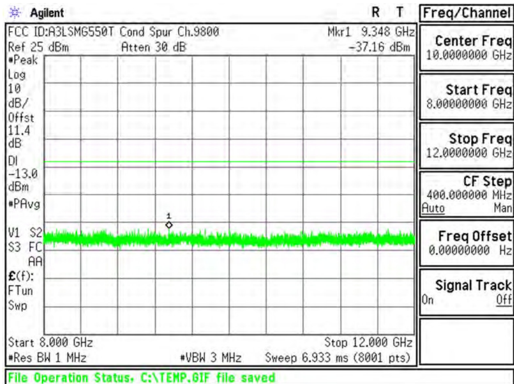
Plot 6-63. Conducted Spurious Plot (PCS WCDMA Mode - Ch.9400(DL9800))
