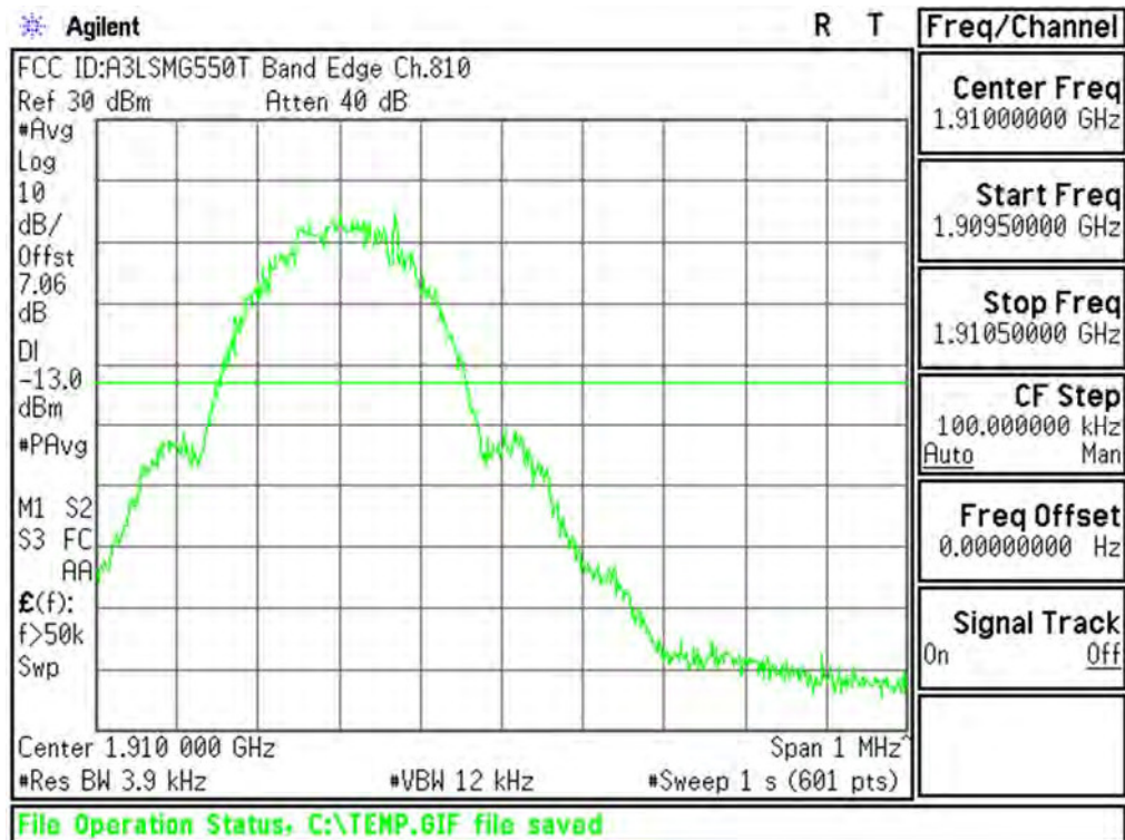
Plot 6-77. Upper Band Edge Plot (PCS GSM Mode – Ch.810)
