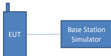
Figure 8-1 Power Measurement Setup for licensed modes
