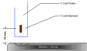
Figure 5-11 Measurement Distance
