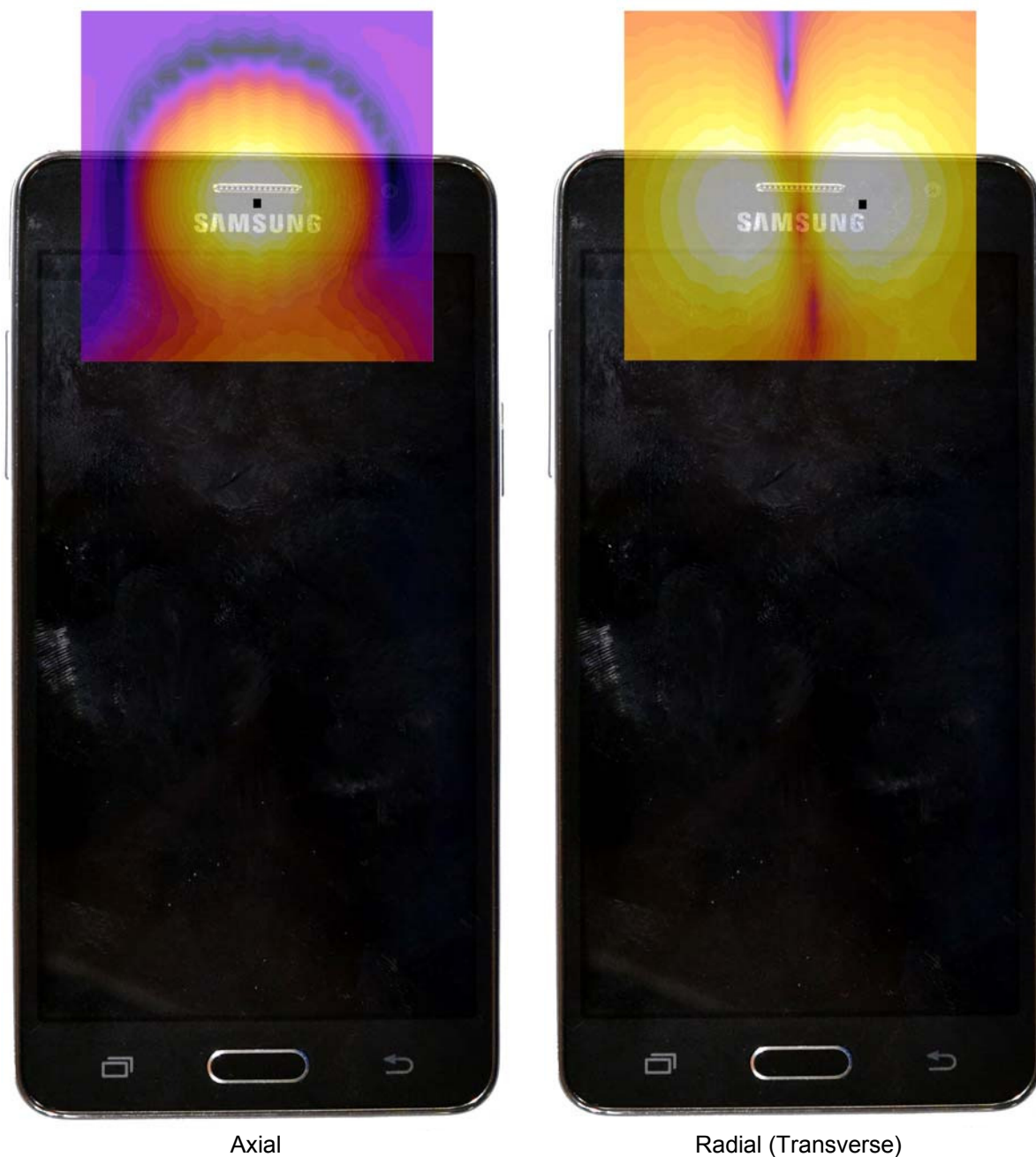
Axial Radial (Transverse) Figure 15-3 T-Coil Scan Overlay Magnetic Field Distributions
