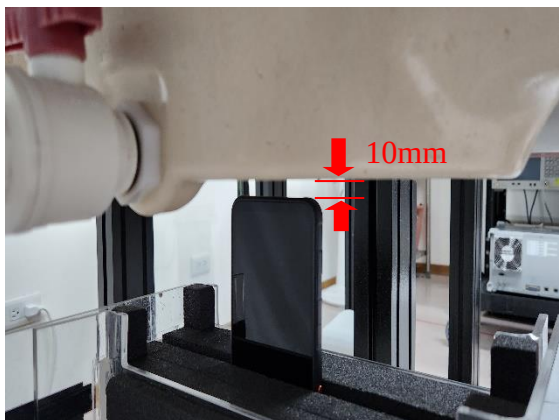
Photograph 9. Body, Bottom Edge, 10mm
