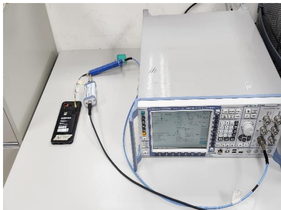
Photograph 5. Test Case 18, Band handover
