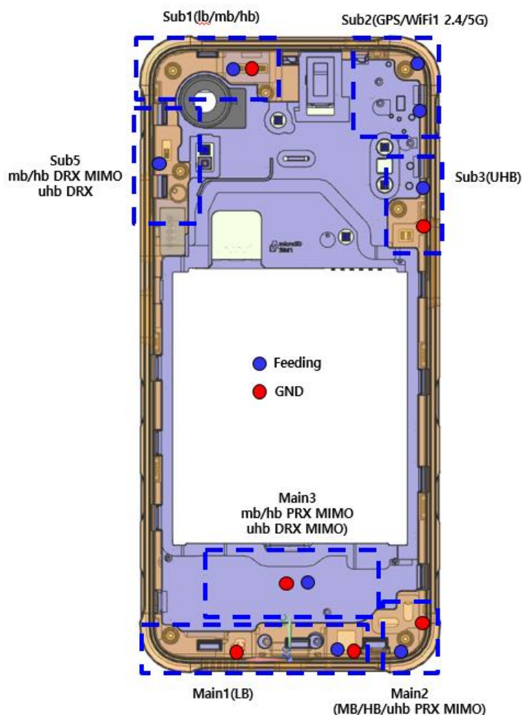
Photograph 17. Antenna position of EUT
