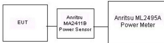
Figure 9-3 Power Measurement Setup
