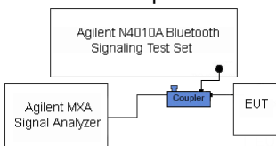
Figure 7-2. Test Instrument & Measurement Setup
