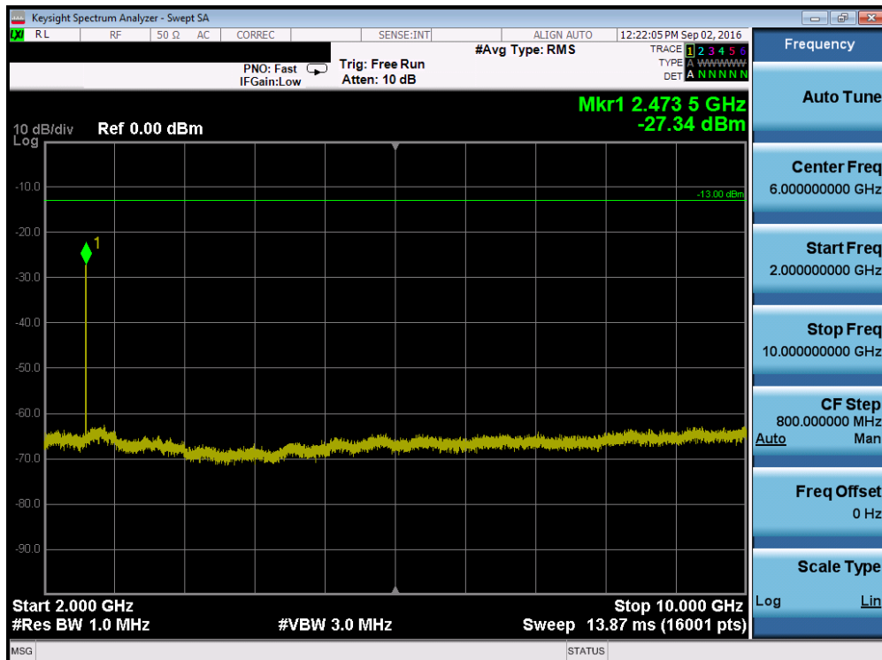
Plot 7-48. Conducted Spurious Plot (Band 5 – 1.4MHz QPSK – RB Size 1, RB Offset 0 – Low Channel)
