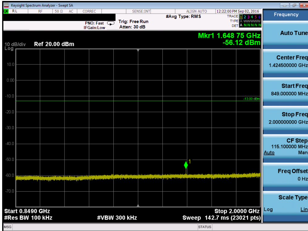
Plot 7-47. Conducted Spurious Plot (Band 5 – 1.4MHz QPSK – RB Size 1, RB Offset 0 – Low Channel)
