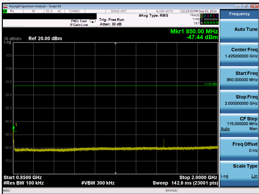
Plot 7-53. Conducted Spurious Plot (Band 5 – 1.4MHz QPSK – RB Size 1, RB Offset 0 – High Channel)
