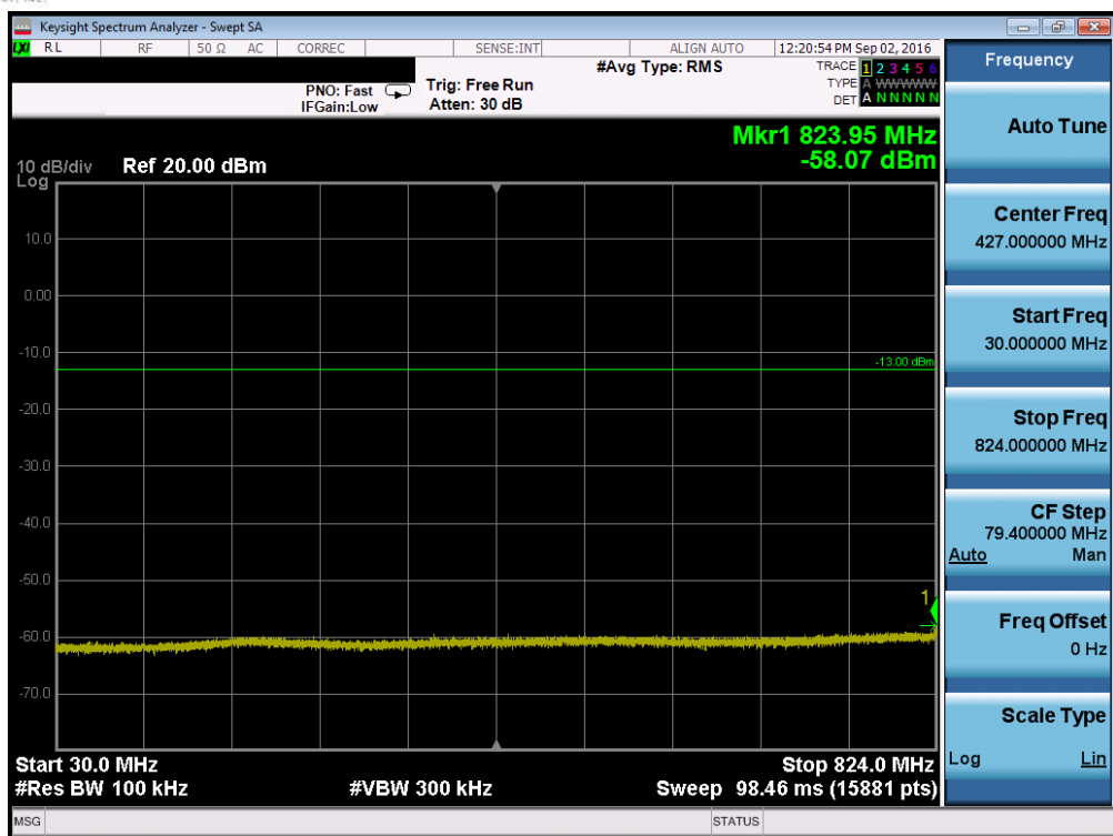
Plot 7-49. Conducted Spurious Plot (Band 5 – 1.4MHz QPSK – RB Size 1, RB Offset 0 – Mid Channel)
