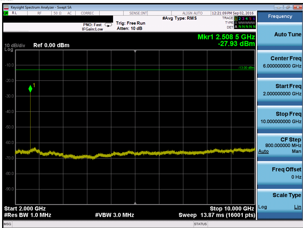
Plot 7-51. Conducted Spurious Plot (Band 5 - 1.4MHz QPSK - RB Size 1, RB Offset 0 - Mid Channel)
