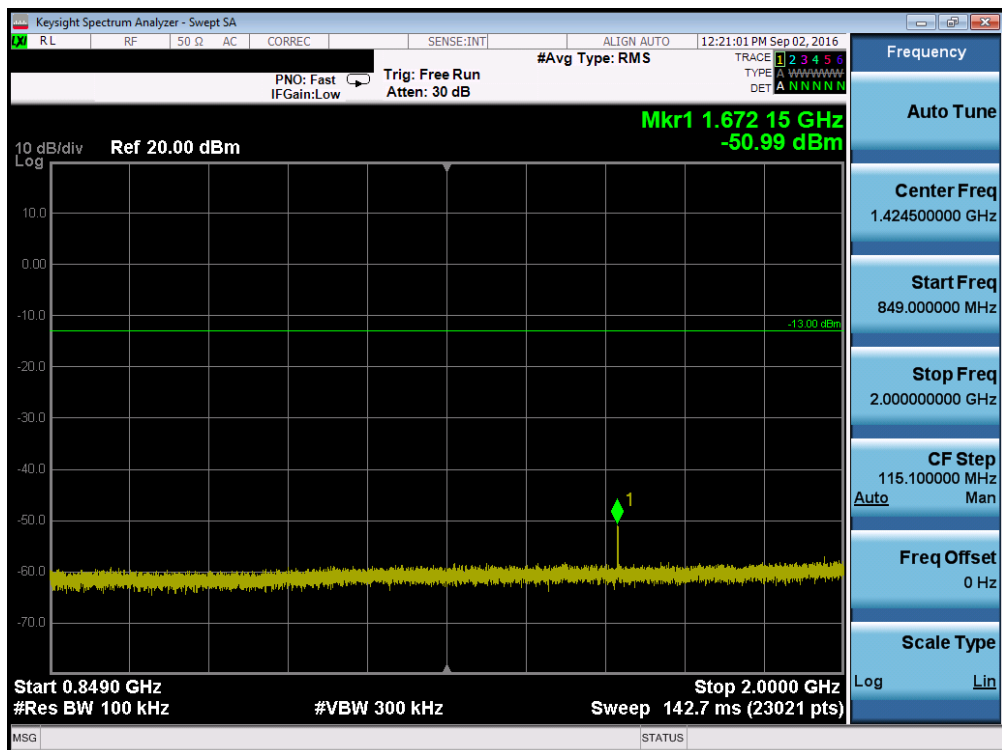
Plot 7-50. Conducted Spurious Plot (Band 5 – 1.4MHz QPSK – RB Size 1, RB Offset 0 – Mid Channel)
