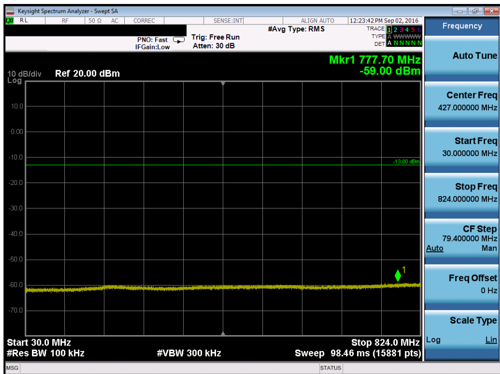
Plot 7-52. Conducted Spurious Plot (Band 5 - 1.4MHz QPSK - RB Size 1, RB Offset 0 - High Channel)
