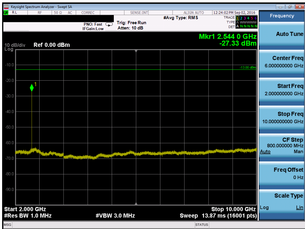
Plot 7-54. Conducted Spurious Plot (Band 5 – 1.4MHz QPSK – RB Size 1, RB Offset 0 – High Channel)
