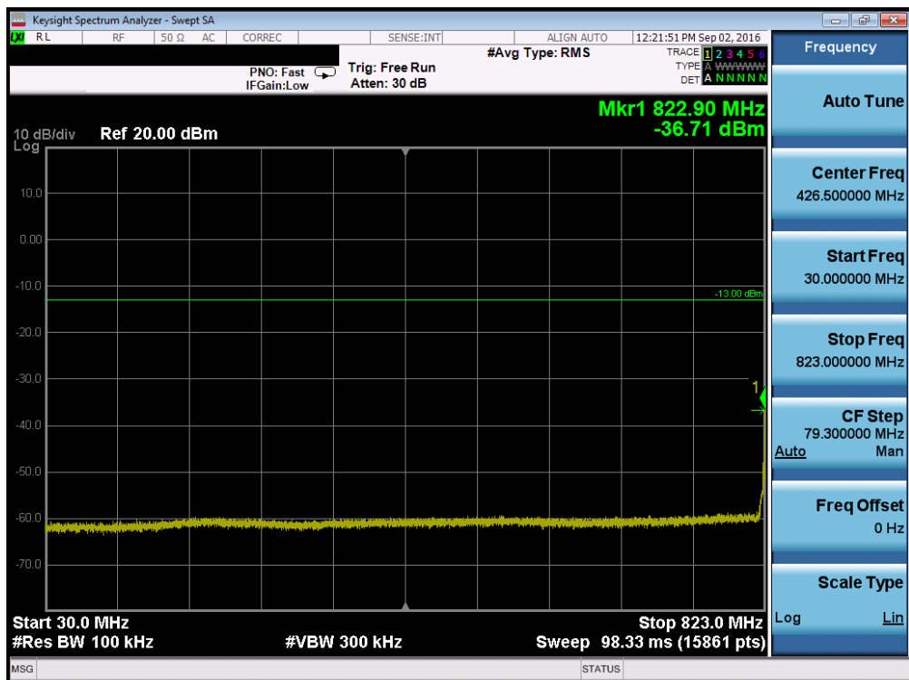
Plot 7-46. Conducted Spurious Plot (Band 5 – 1.4MHz QPSK – RB Size 1, RB Offset 0 – Low Channel)
