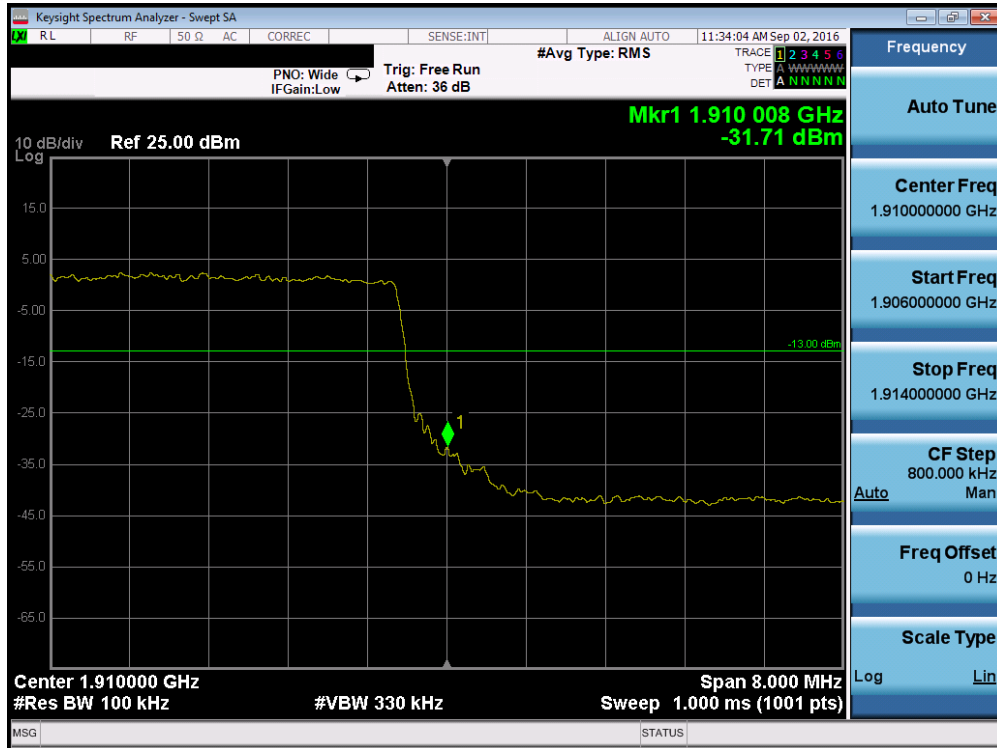
Plot 7-125. Upper Band Edge Plot (Band 2 – 10.0MHz QPSK – RB Size 50)
