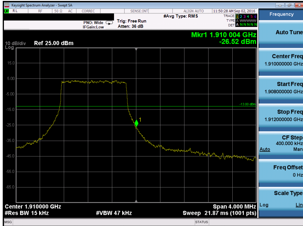
Plot 7-113. Upper Band Edge Plot (Band 2 – 1.4MHz QPSK – RB Size 6)
