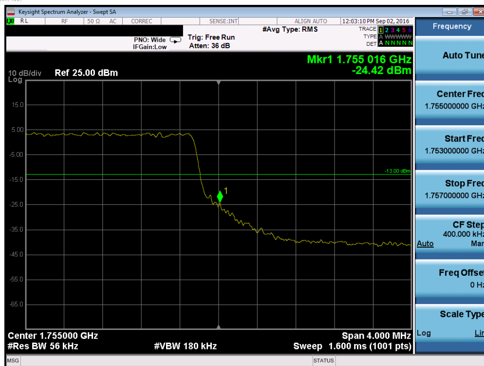
Plot 7-97. Upper Band Edge Plot (Band 4 – 5.0MHz QPSK – RB Size 25)
