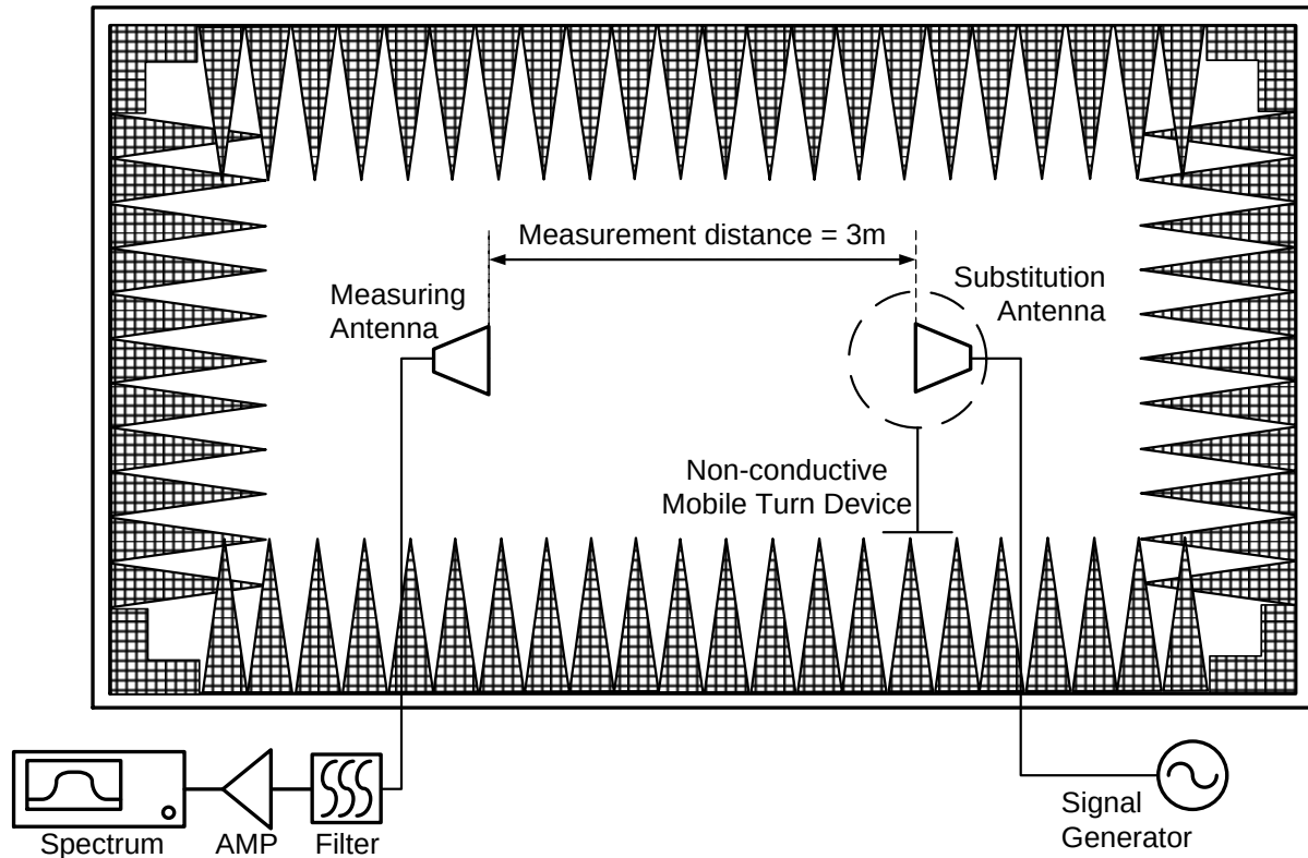
Figure 6-7. Test Instruments & Measurement Setup
