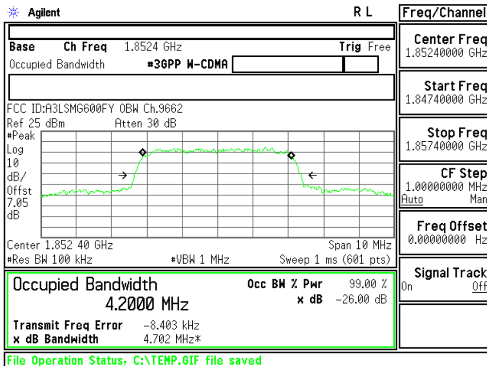
Plot 6-6. Occupied Bandwidth Plot (PCS WCDMA Mode - Ch.9262(DL9662))
