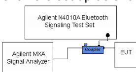
Figure 7-2. Test Instrument & Measurement Setup
