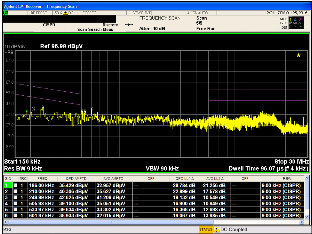
Plot 7-5. Line Conducted Plot (L1)
