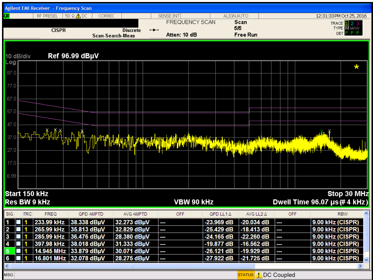
Plot 7-6. Line Conducted Plot (N)
