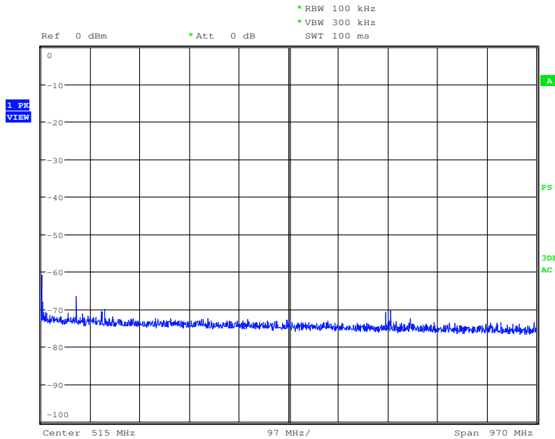
Plot 7-1. Radiated Spurious Plot below 1GHz (Ant. Pol. H)
