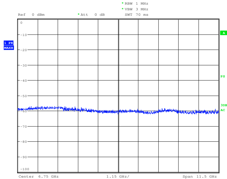
Plot 7-3. Radiated Spurious Plot above 1GHz (Ant. Pol. H)
