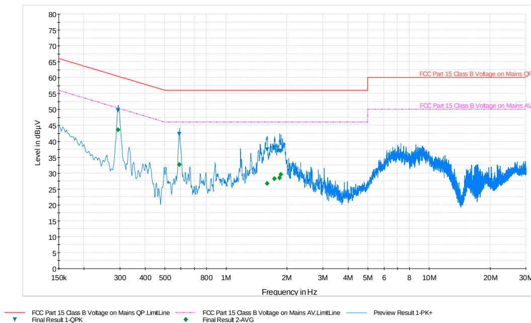
Plot 6-66. Line Conducted Plot with 802.11a (N)
