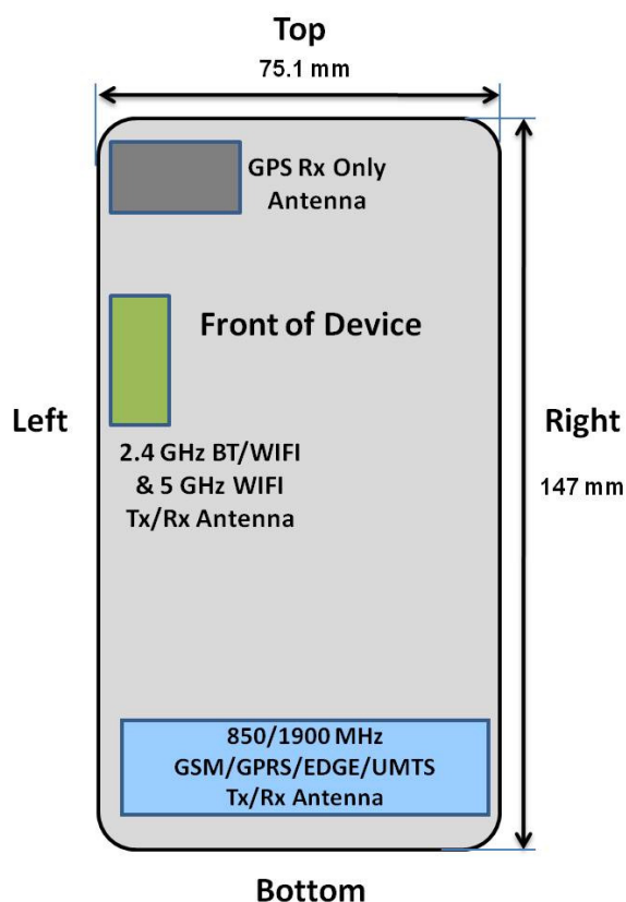
Figure 1-1 DUT Antenna Locations
