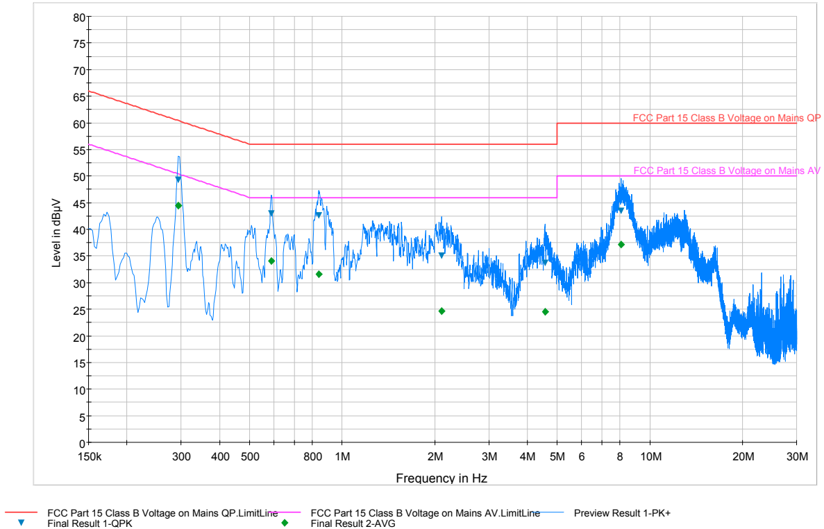
Plot 6-6. Line-Conducted Test Plot (L1)
