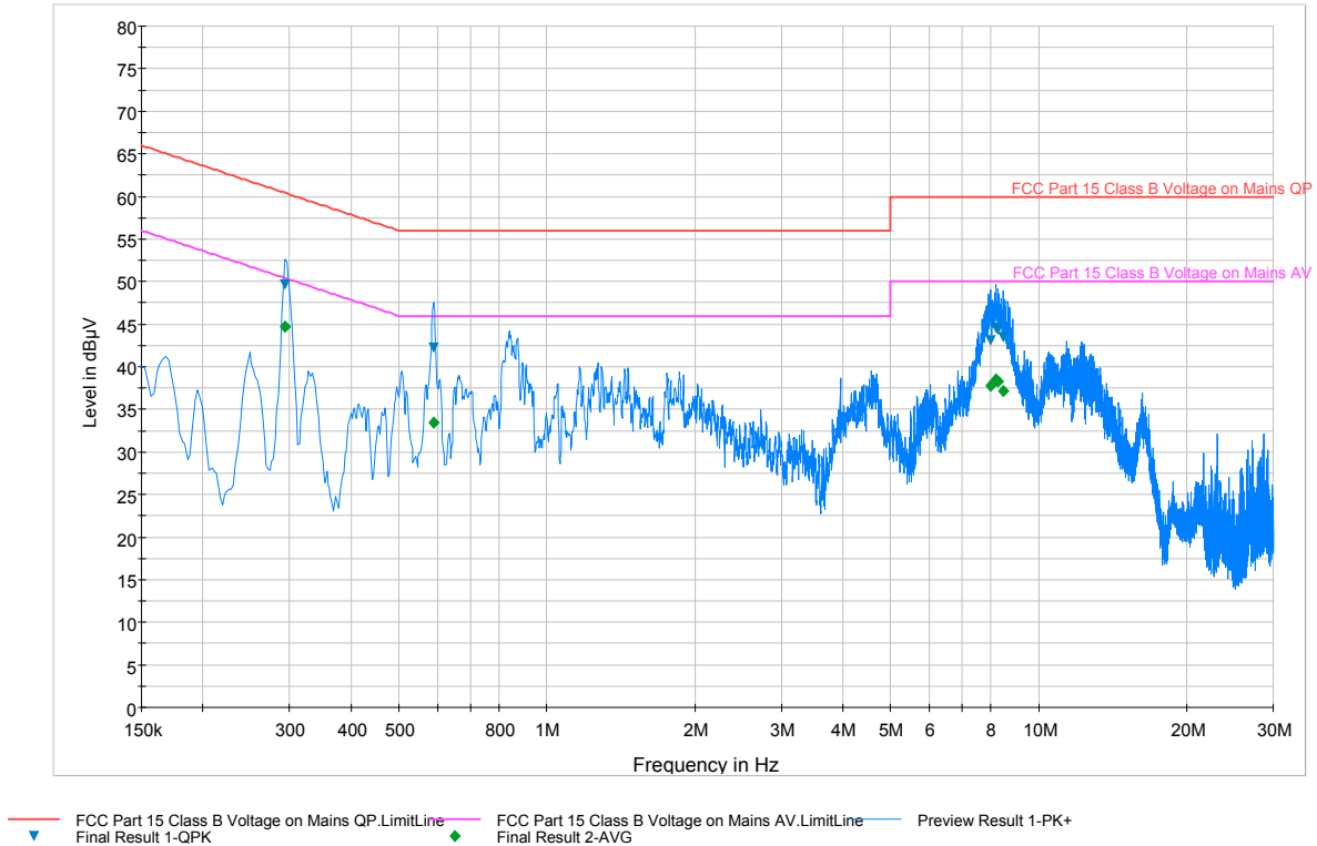
Plot 6-7. Line-Conducted Test Plot (N)
