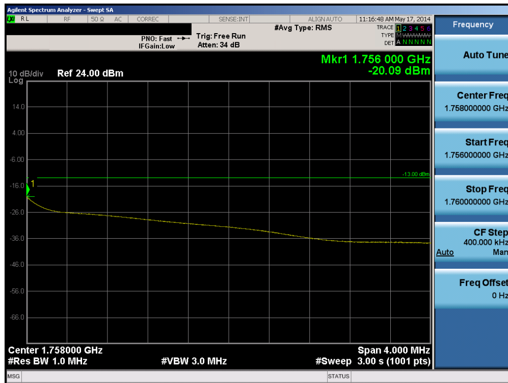
Plot 6-11. 4MHz Span Plot (AWS WCDMA Mode – Ch. 1862)
