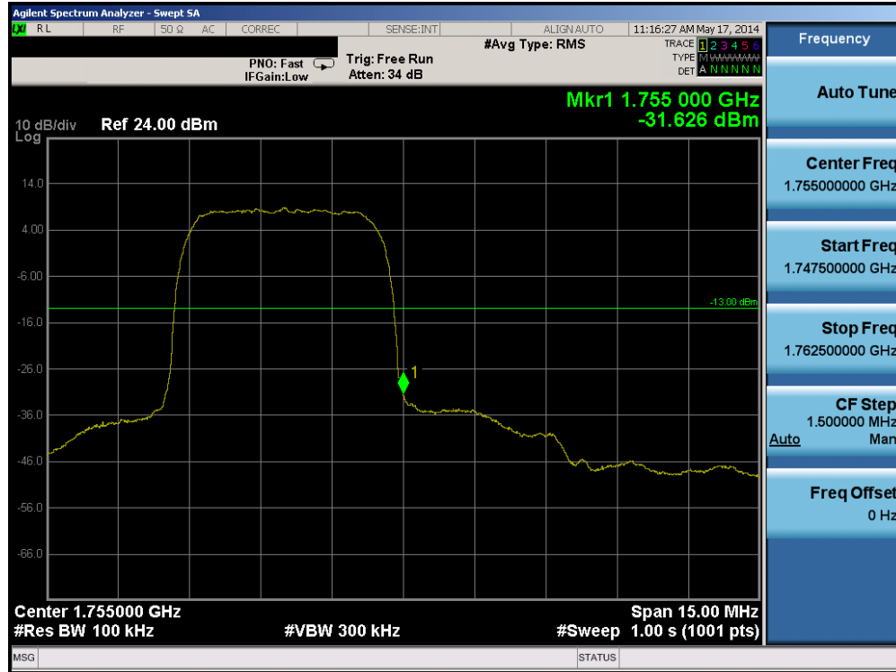
Plot 6-10. Band Edge Plot (AWS WCDMA Mode – Ch. 1862)
