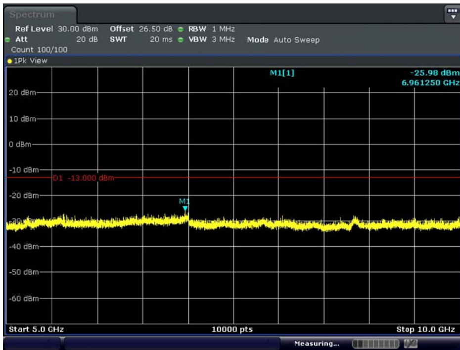
BAND 17. Conducted Spurious Plot_2 (23800ch_10MHz_QPSK_RB 1_0)
