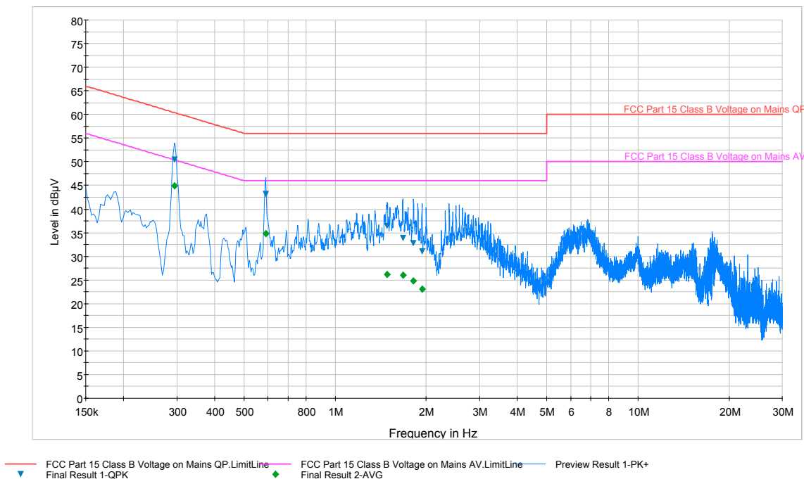
Plot 6-19. Line Conducted Plot with Bluetooth LE (N)
