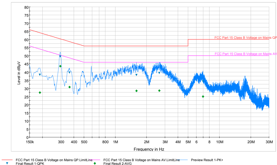
Plot 6-18. Line Conducted Plot with Bluetooth LE (L1)
