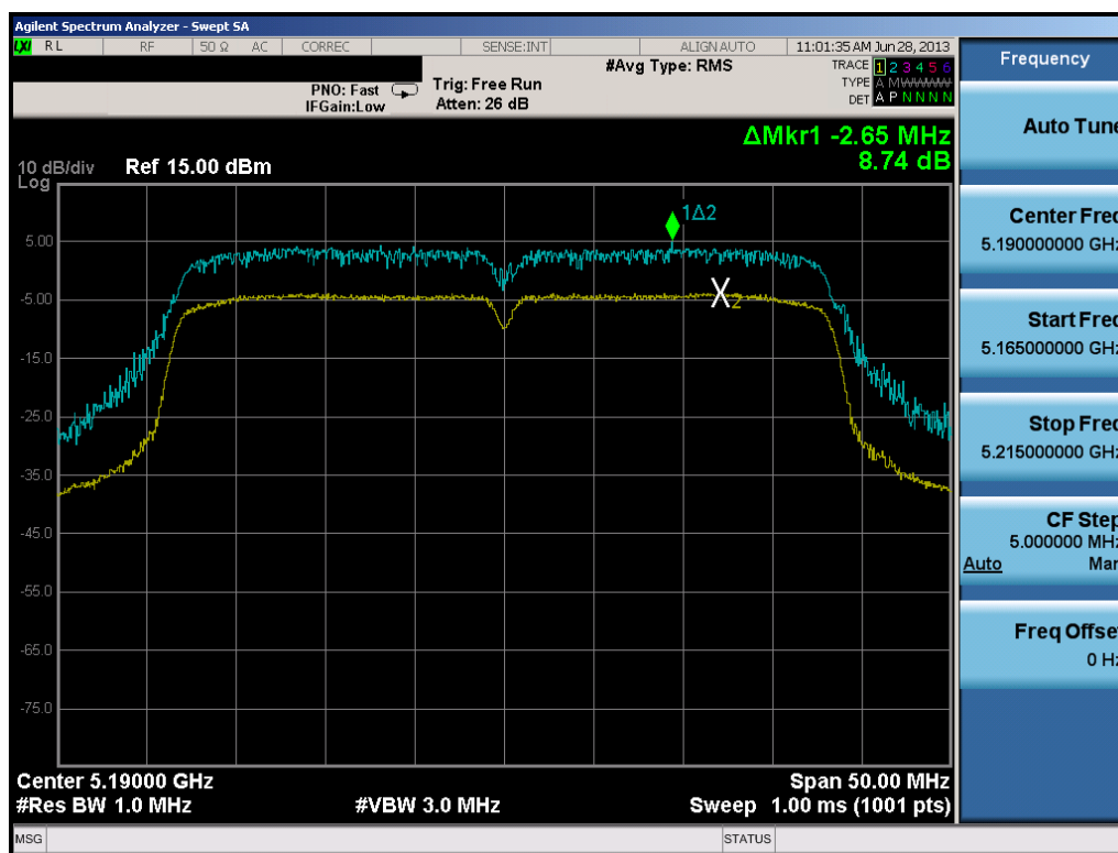
Plot 6-53. Peak Excursion Ratio Plot (40MHz BW 802.11n)
