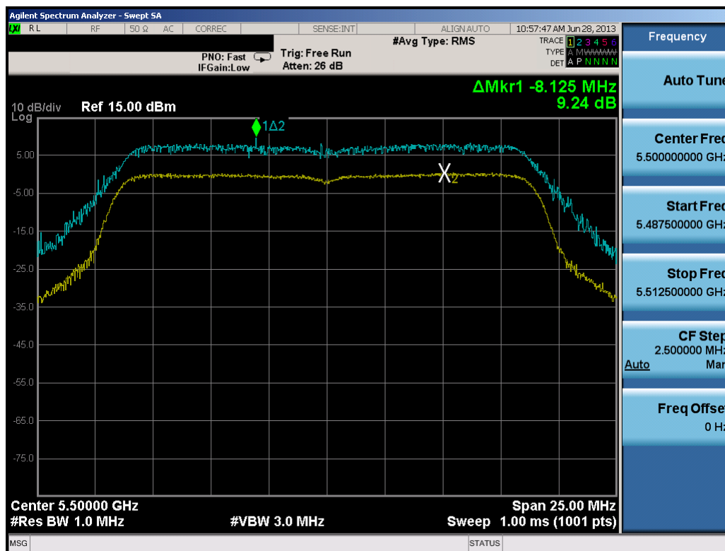
Plot 6-52. Peak Excursion Ratio Plot (20MHz BW 802.11n)
