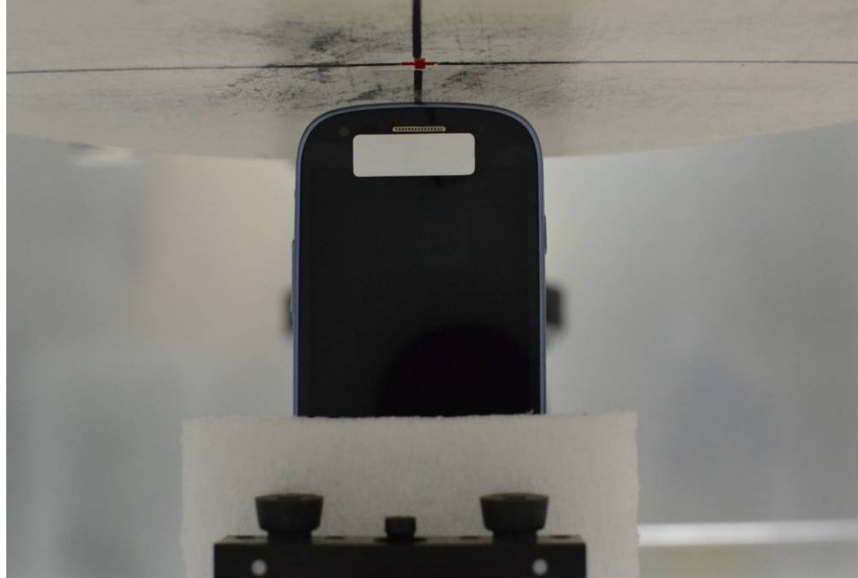
SAR Test Setup Photo 7 – Top Side at 1.0 cm
