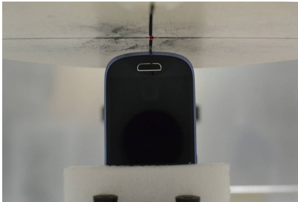
SAR Test Setup Photo 8 – Bottom Side at 1.0 cm
