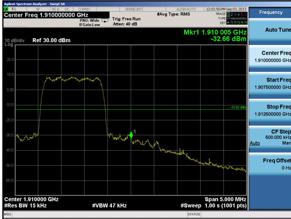
Plot 6-19. Band Edge Plot (PCS CDMA Mode – Ch. 1175)
