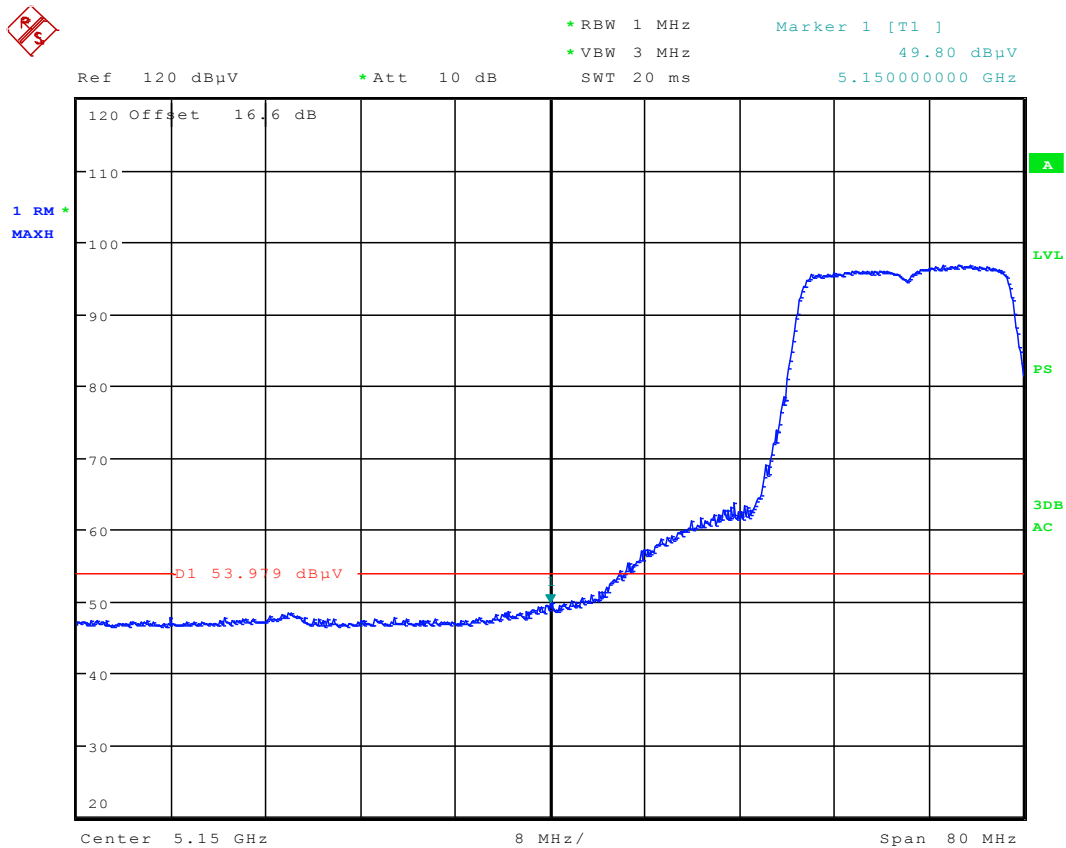
Plot 6-56. Radiated Restricted Lower Band Edge Plot (Average – UNII Band 1)
