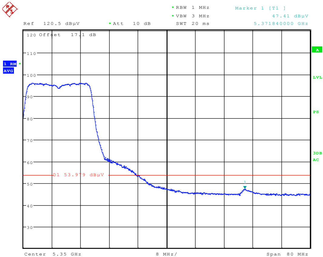
Plot 6-58. Radiated Restricted Upper Band Edge Plot (Average – UNII Band 2)
