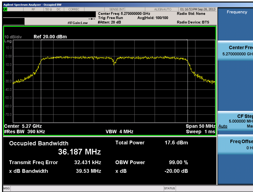
Plot 6-26. 20dB Bandwidth Plot (40MHz BW 802.11n (UNII Band 2) – Ch. 54)
