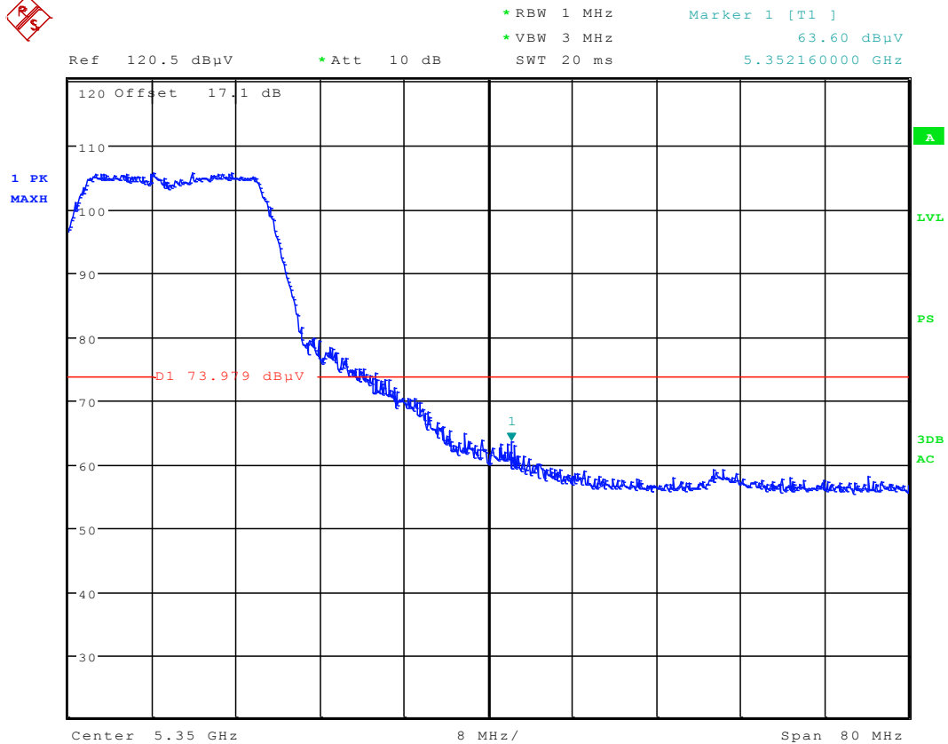
Plot 6-59. Radiated Restricted Upper Band Edge Plot (Peak – UNII Band 2)
