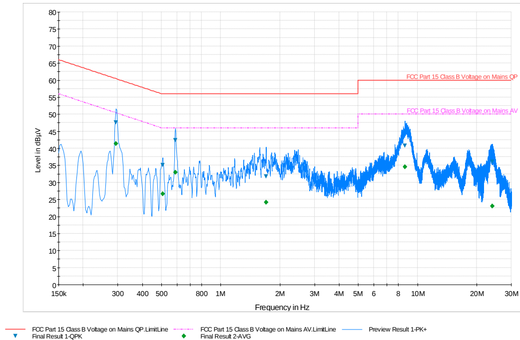
Plot 6-72. Line Conducted Plot with 802.11a UNII Band 2 (L1)
