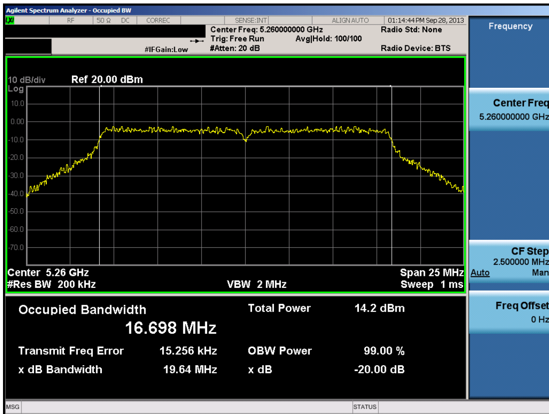
Plot 6-27. 20dB Bandwidth Plot (20MHz BW 802.11a (UNII Band 2) – Ch. 52)
