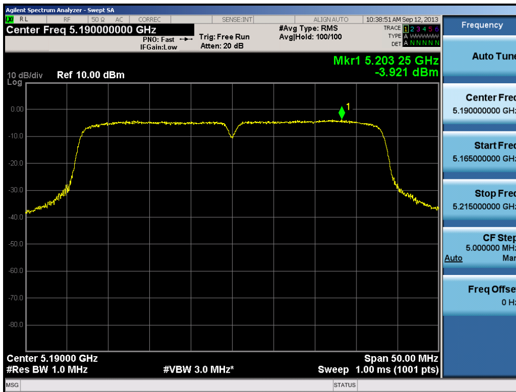
Plot 6-34. Peak Power Spectral Density Plot (40MHz BW 802.11n (UNII Band 1) – Ch. 38)
