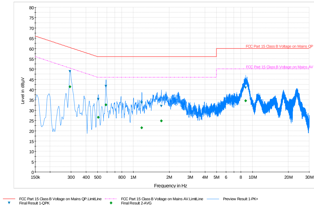
Plot 6-74. Line Conducted Plot with 802.11a UNII Band 3 (L1)
