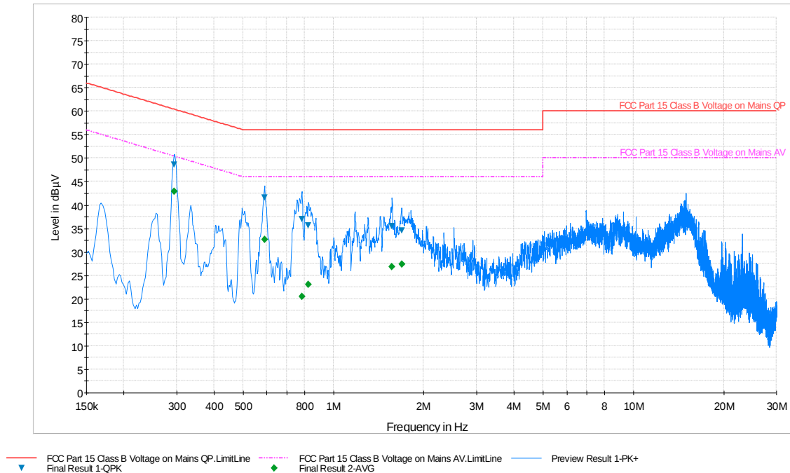
Plot 6-71. Line Conducted Plot with 802.11a UNII Band 1 (N)
