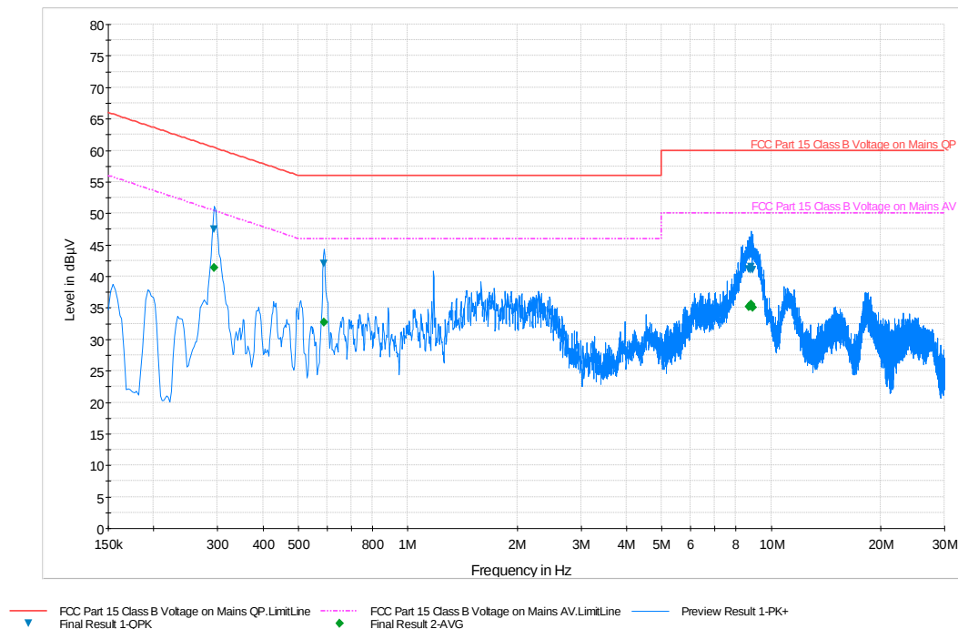
Plot 6-73. Line Conducted Plot with 802.11a UNII Band 2 (N)
