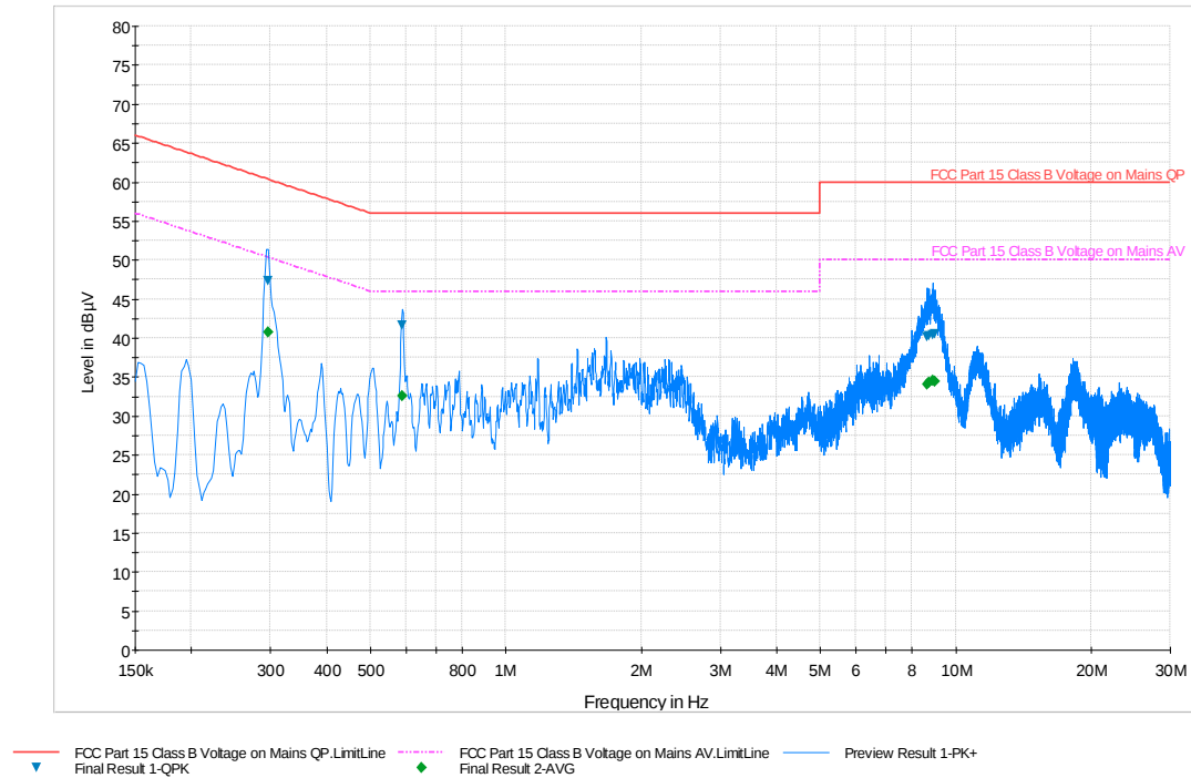
Plot 6-75. Line Conducted Plot with 802.11a UNII Band 3 (N)
