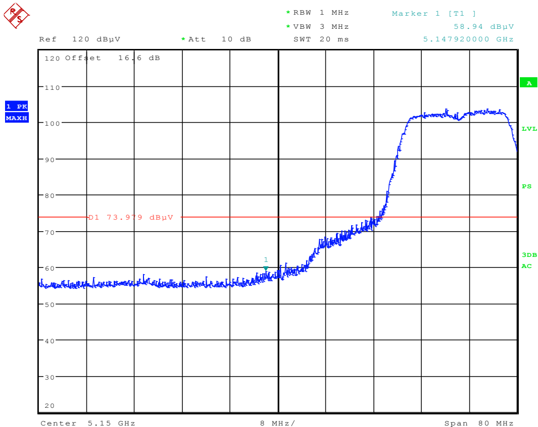
Plot 6-57. Radiated Restricted Lower Band Edge Plot (Peak – UNII Band 1)
