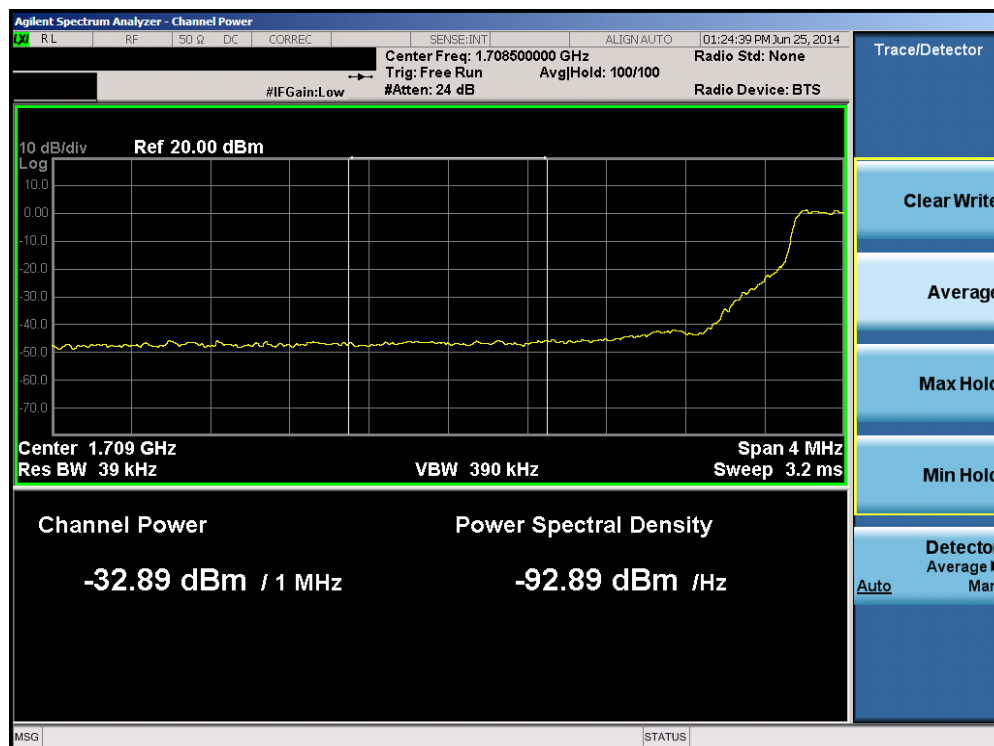
Plot 6-90. Lower Extended Band Edge Plot (Band 4 – 5.0MHz QPSK – RB Size 25)
