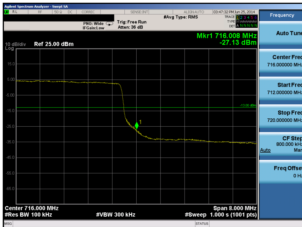
Plot 6-66. Upper Band Edge Plot (Band 17 – 10.0MHz QPSK – RB Size 50)
