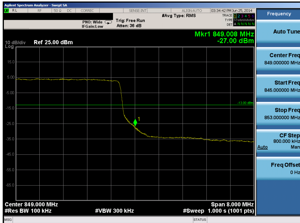
Plot 6-80. Upper Band Edge Plot (Band 5 – 10.0MHz QPSK – RB Size 50)
