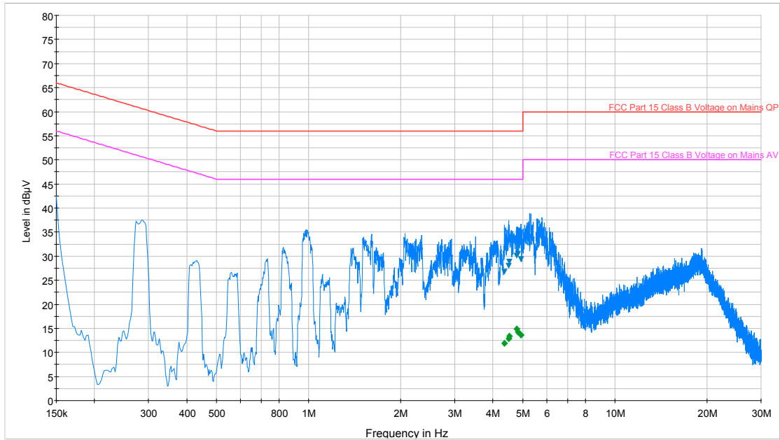
Plot 6-45. Line-Conducted Test Plot (N)
