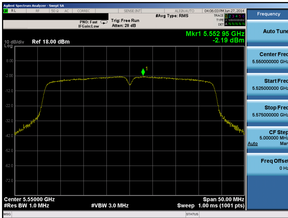
Plot 6-52. Peak Power Spectral Density Plot (40MHz BW 802.11a/n (UNII Band 2C) – Ch. 110)
