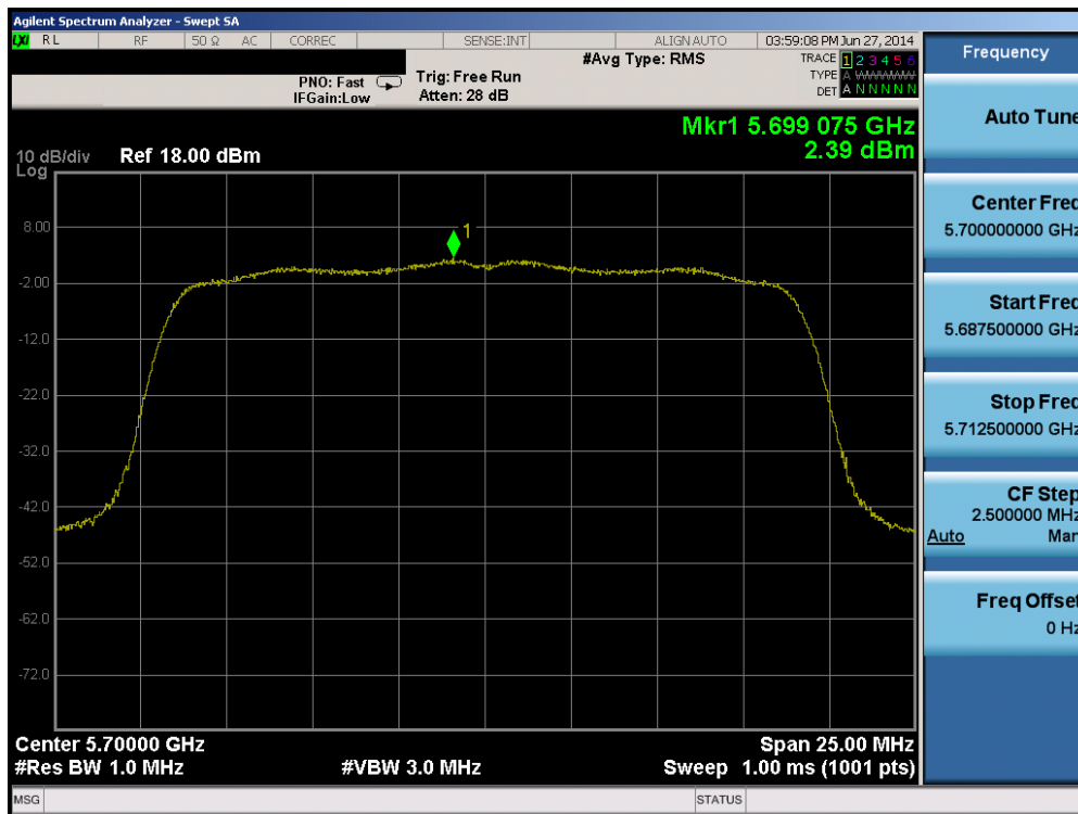
Plot 6-50. Peak Power Spectral Density Plot (20MHz BW 802.11n (UNII Band 2C) – Ch. 140)
