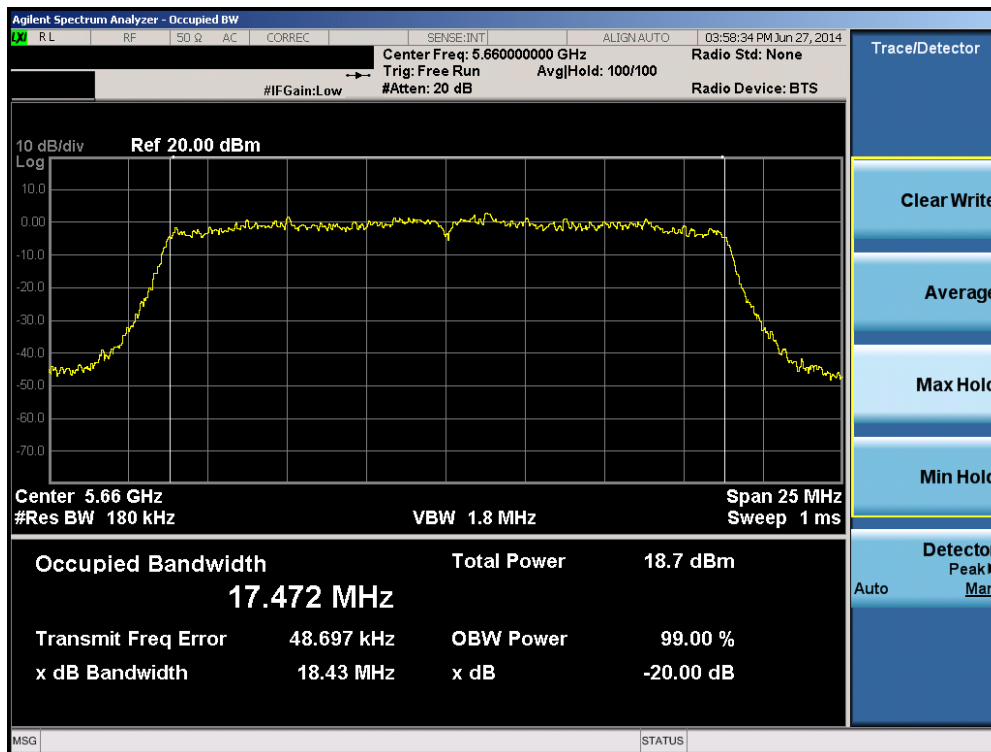
Plot 6-26. 20dB Bandwidth Plot (20MHz BW 802.11n (UNII Band 2C) – Ch. 132)
