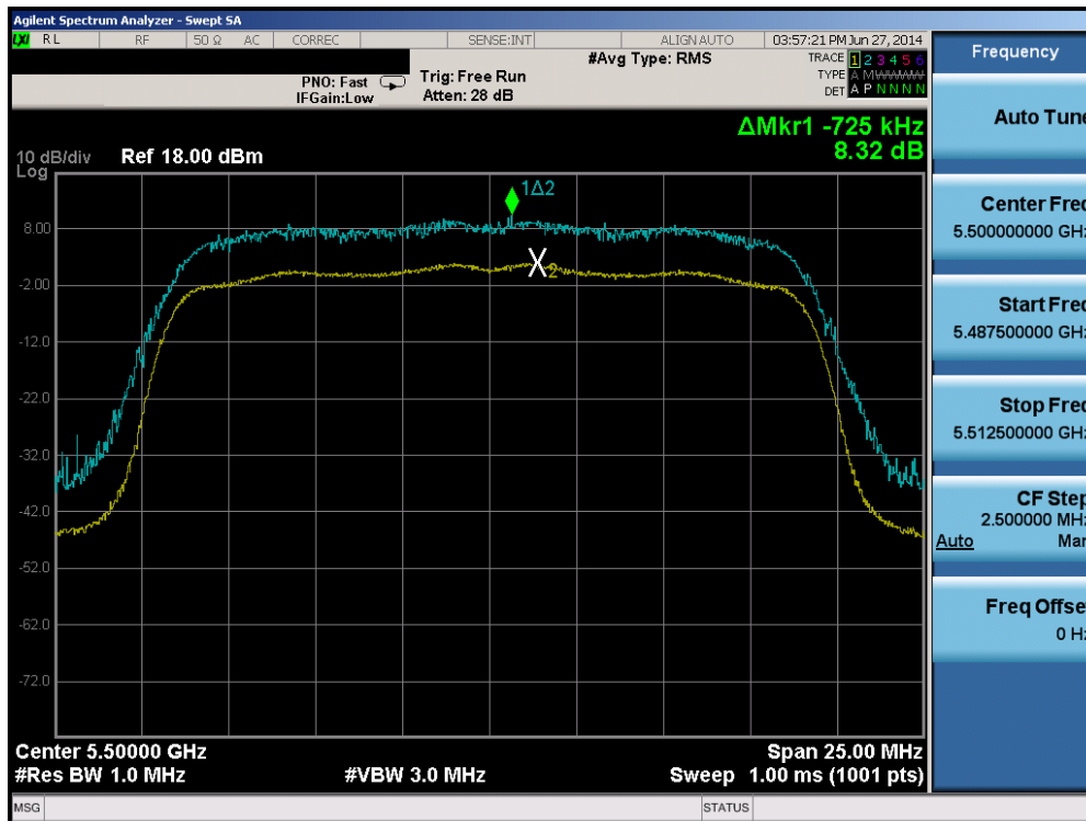
Plot 6-55. Peak Excursion Ratio Plot (20MHz BW 802.11n (UNII Band 2C) – Ch. 100)
