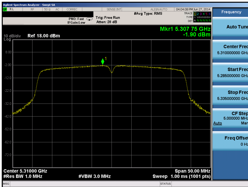
Plot 6-44. Peak Power Spectral Density Plot (40MHz BW 802.11a/n (UNII Band 2A) – Ch. 62)
