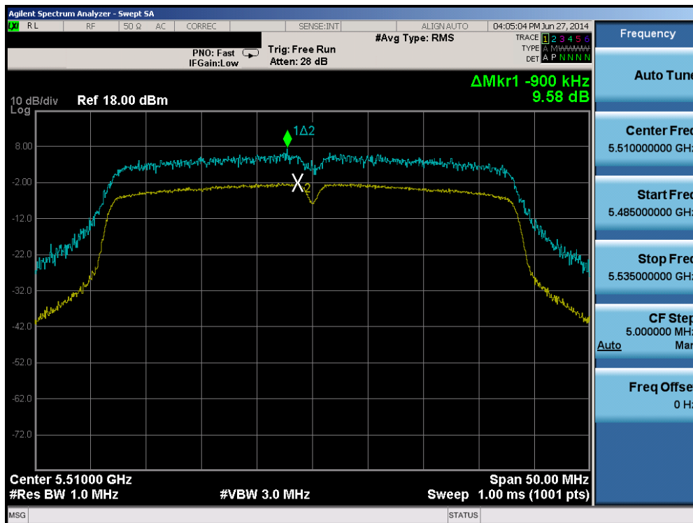
Plot 6-56. Peak Excursion Ratio Plot (40MHz BW 802.11n (UNII Band 2C) – Ch. 102)
