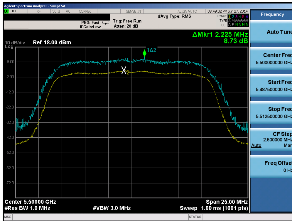
Plot 6-54. Peak Excursion Ratio Plot (802.11a (UNII Band 2C) – Ch. 100)
