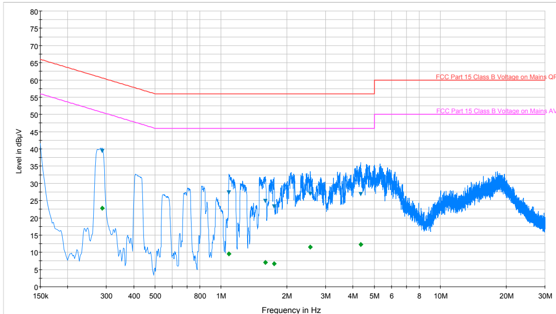
Plot 6-65. Line Conducted Plot with 802.11a (L1)
