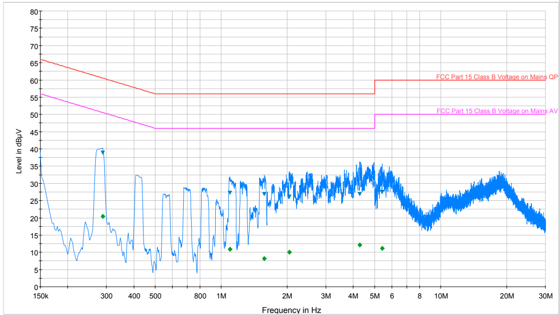
Plot 6-63. Line Conducted Plot with 802.11b (L1)
