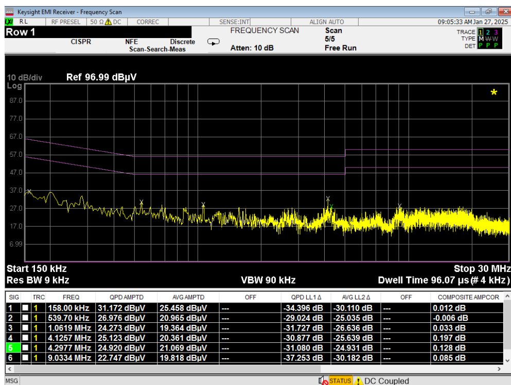
Plot 7-113. Line Conducted Plot with Bluetooth LE (L1)
