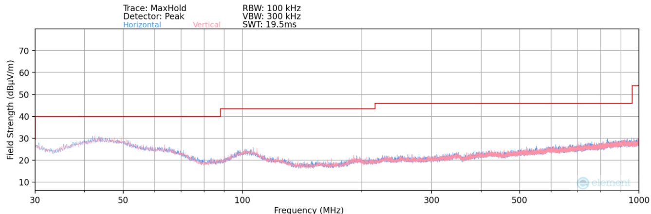
Plot 7-111. Radiated Spurious Plot below 1GHz – Ant 1
