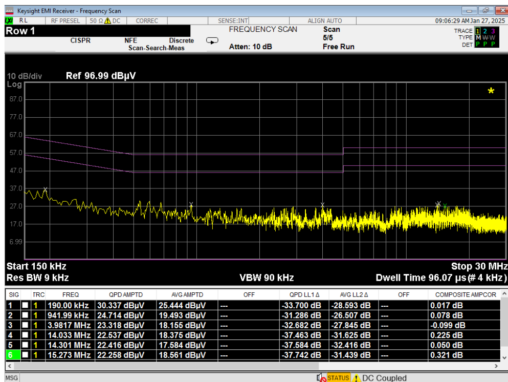
Plot 7-114. Line Conducted Plot with Bluetooth LE (N)
