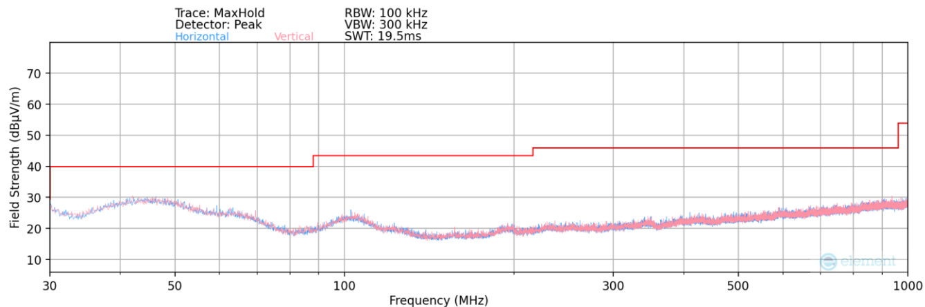
Plot 7-112. Radiated Spurious Plot below 1GHz – Ant 2
