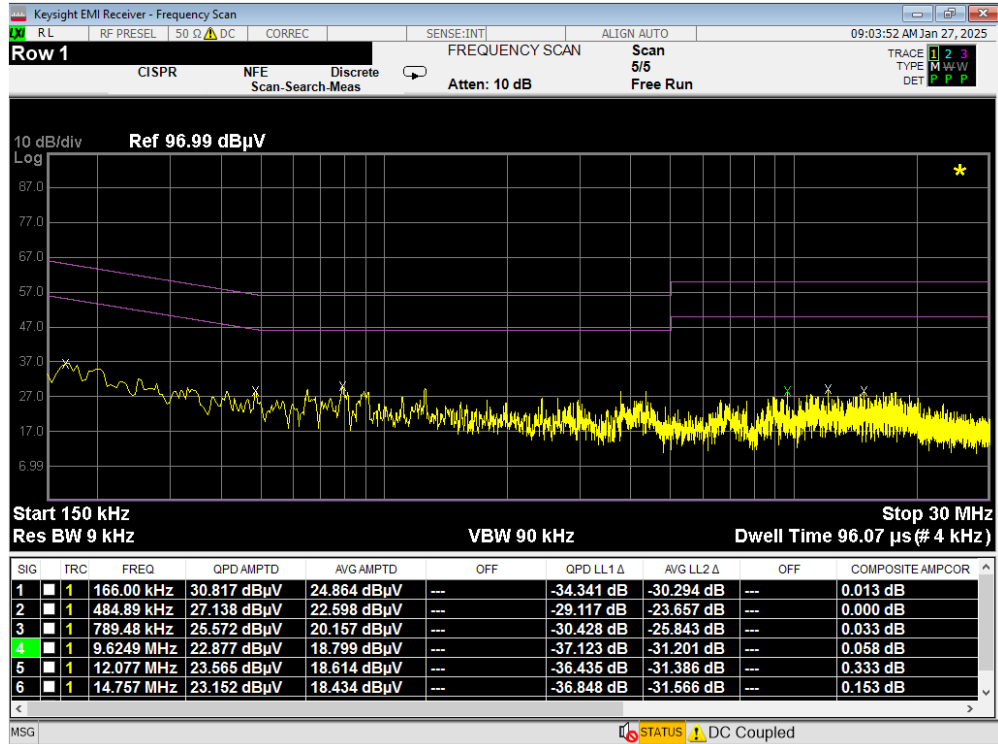
Plot 7-97. Line-Conducted Test Plot (L1)
