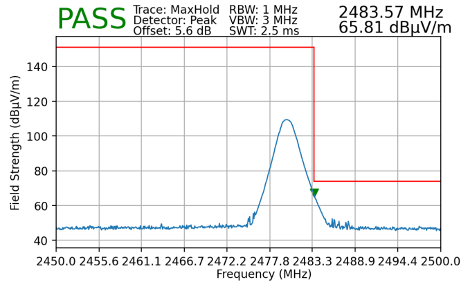
Plot 7-94. Radiated Restricted Upper Band Edge Measurement (Peak)
