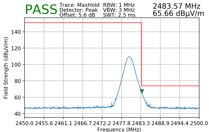
Plot 7-92. Radiated Restricted Upper Band Edge Measurement (Peak)
