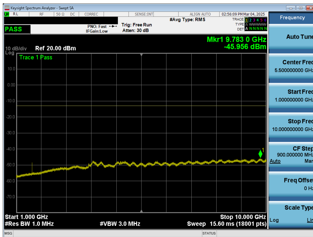
Plot 7-132. Conducted Spurious Plot (LTE Band 13 - 10MHz QPSK - 1 RB)
