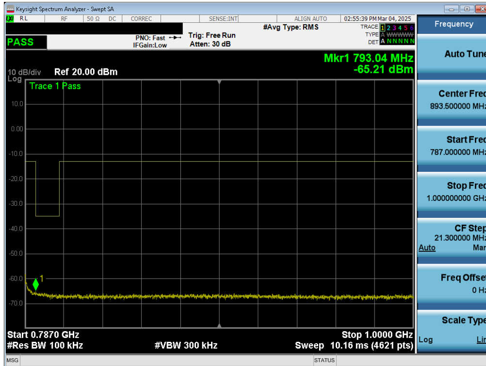
Plot 7-131. Conducted Spurious Plot (LTE Band 13 - 10MHz QPSK - 1 RB)
