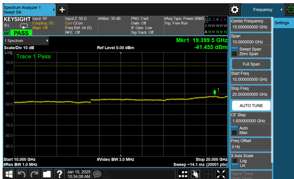
Plot 7-144. Conducted Spurious Plot (NR Band n70 - 15.0MHz - 1 RB - Mid Channel – Ant2)
