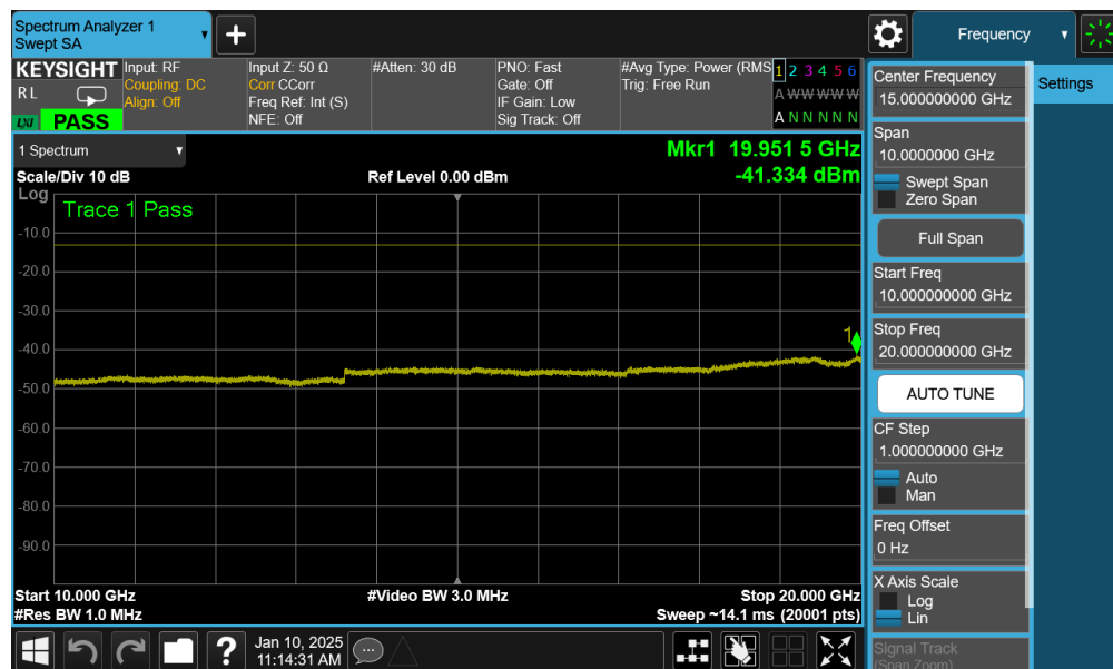
Plot 7-147. Conducted Spurious Plot (NR Band n66 - 40.0MHz - 1 RB - High Channel – Ant2)
