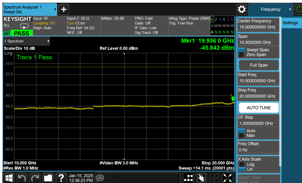
Plot 7-153. Conducted Spurious Plot (NR Band n70 - 15.0MHz - 1 RB - Mid Channel – Ant4)
