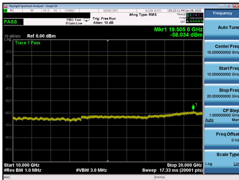
Plot 7-138. Conducted Spurious Plot (WCDMA Ch. 1312- Low Channel – Ant2)
