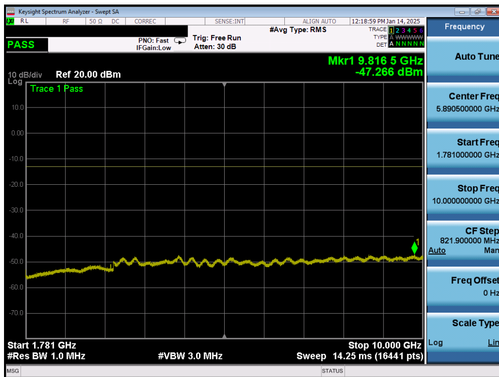
Plot 7-149. Conducted Spurious Plot (LTE Band 66/4 - 20MHz QPSK - 1 RB - High Channel – Ant4)
