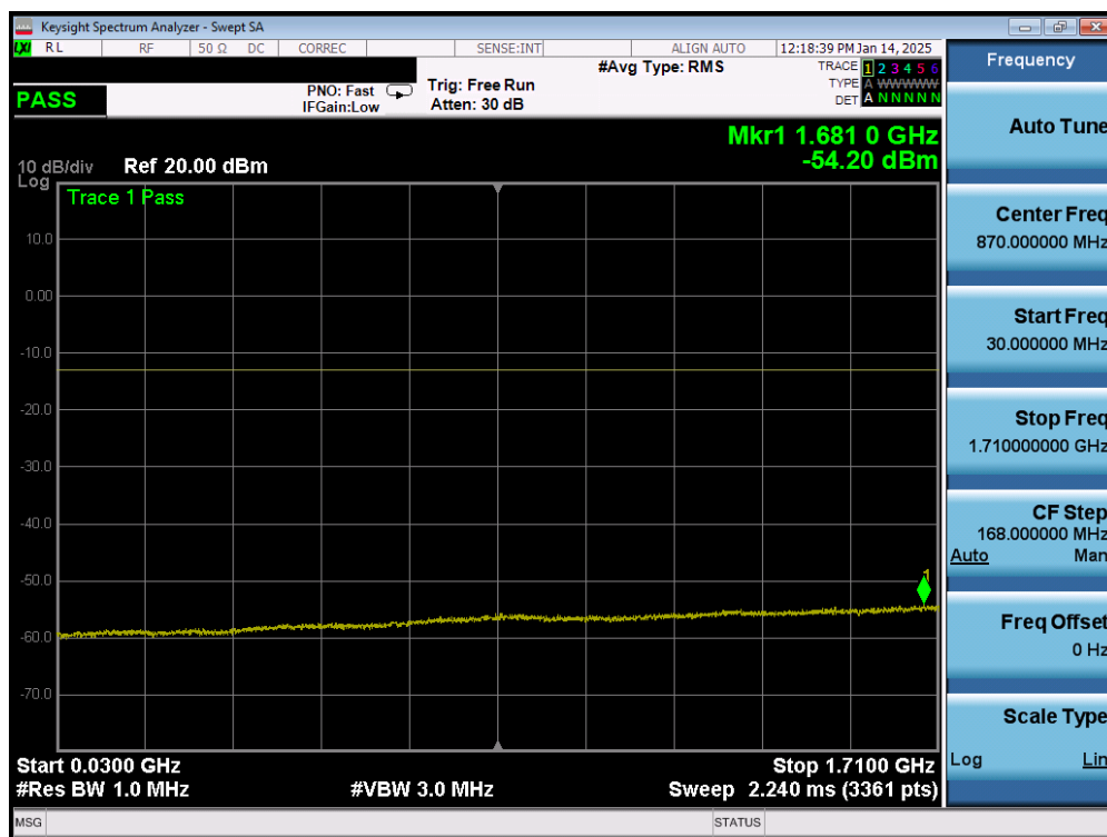
Plot 7-148. Conducted Spurious Plot (LTE Band 66/4 - 20MHz QPSK - 1 RB - High Channel – Ant4)
