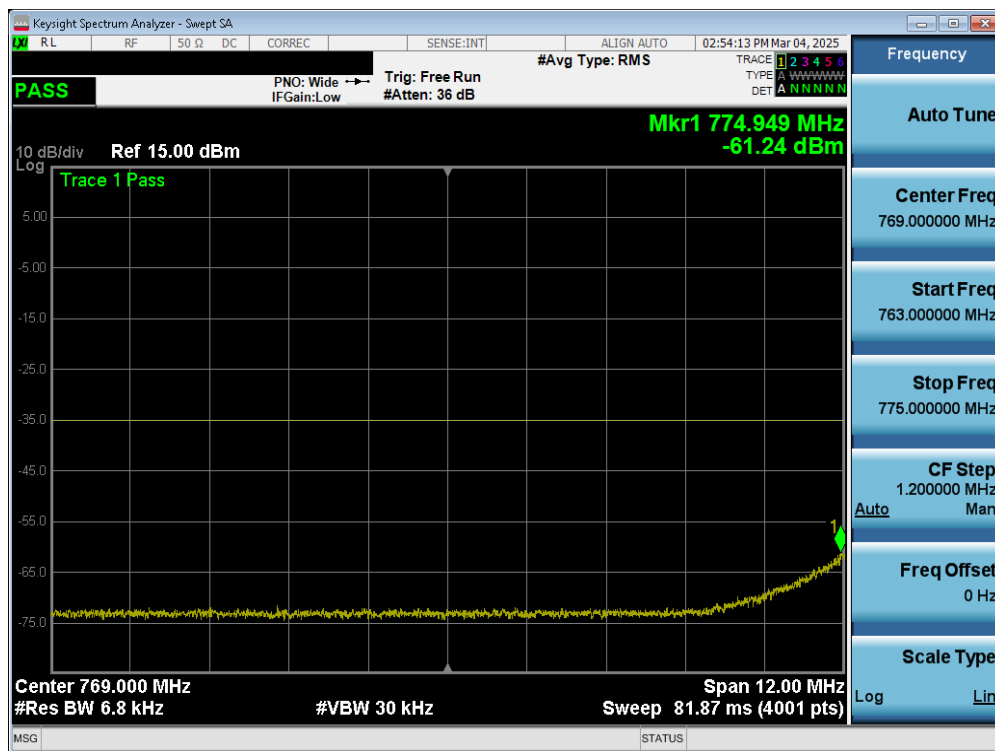
Plot 7-162. Lower Emission Mask Plot (LTE Band 13 - 5MHz QPSK – Full RB - Ant1)
