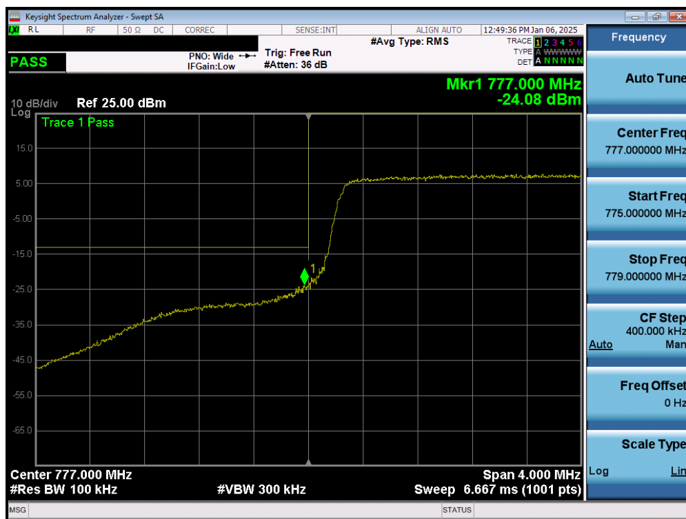
Plot 7-161. Lower Band Edge Plot (LTE Band 13 - 5MHz QPSK – Full RB - Ant1)
