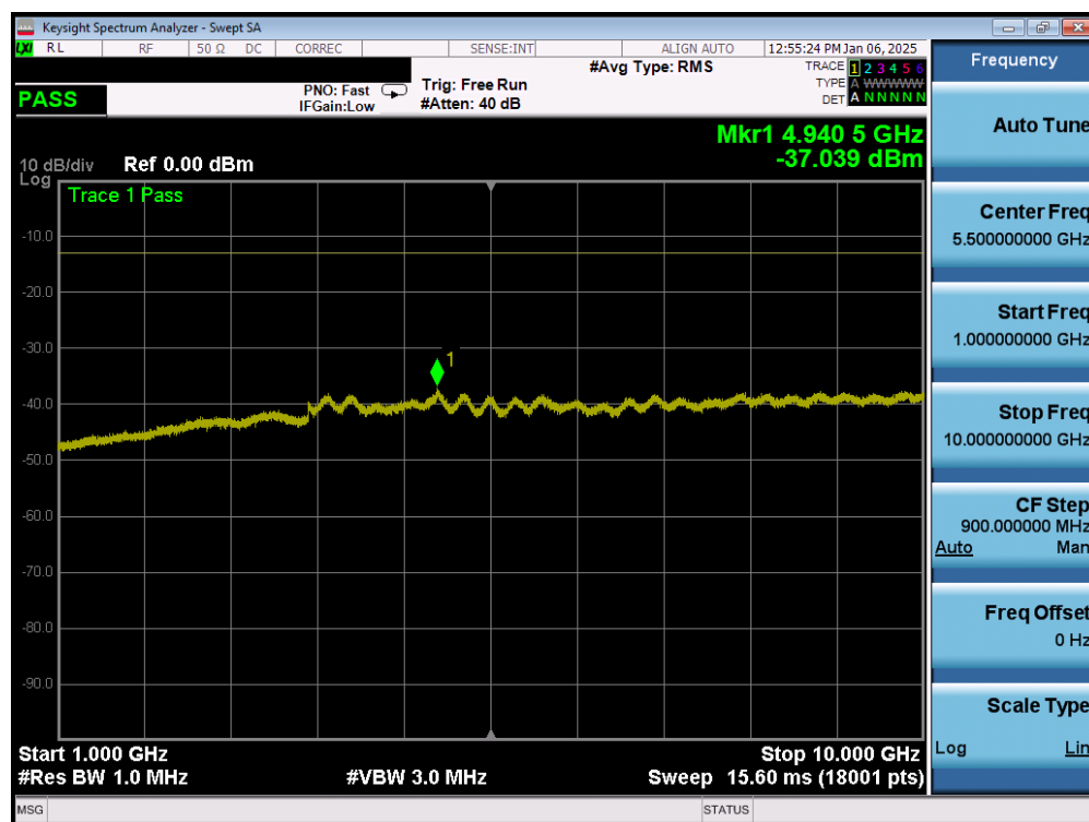
Plot 7-129. Conducted Spurious Plot (LTE Band 12 - 10MHz QPSK - 1 RB - High Channel - Ant1)
