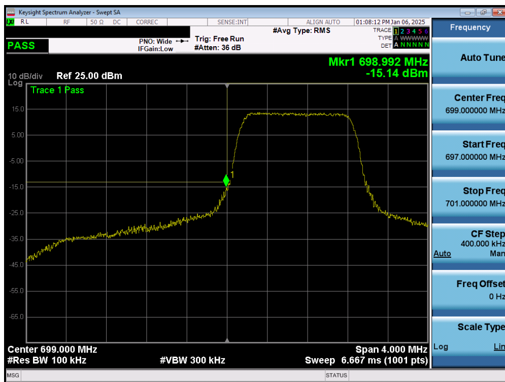
Plot 7-159. Lower Band Edge Plot (LTE Band 12 – 1.4MHz QPSK – Full RB - Ant1)
