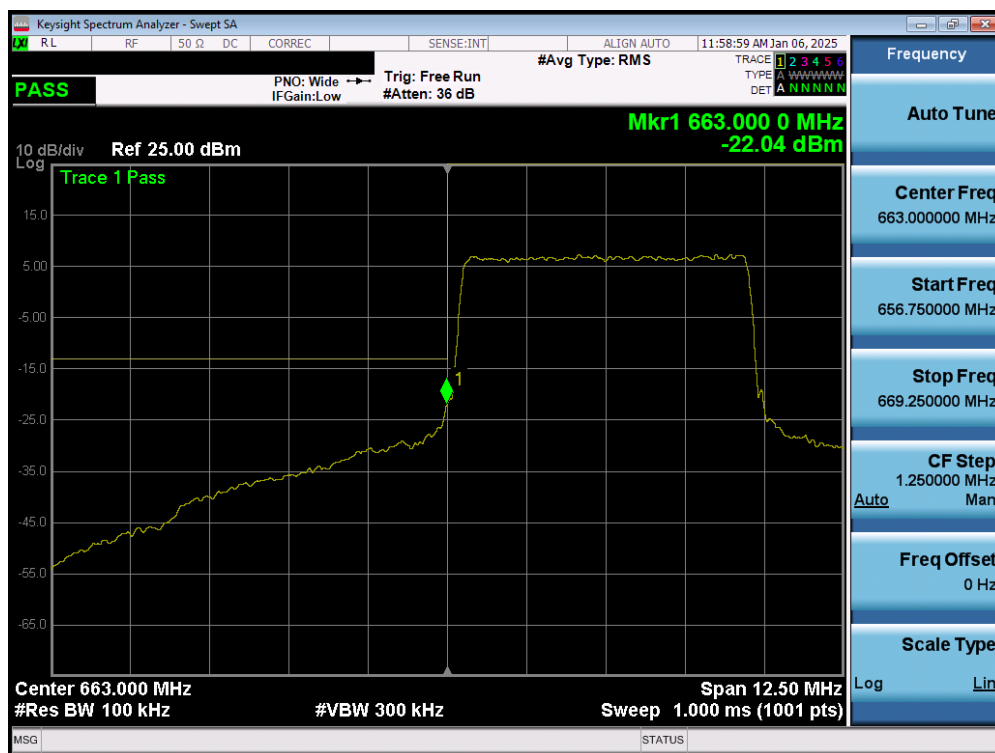
Plot 7-157. Lower Band Edge Plot (LTE Band 71 - 5MHz QPSK – Full RB - Ant1)
