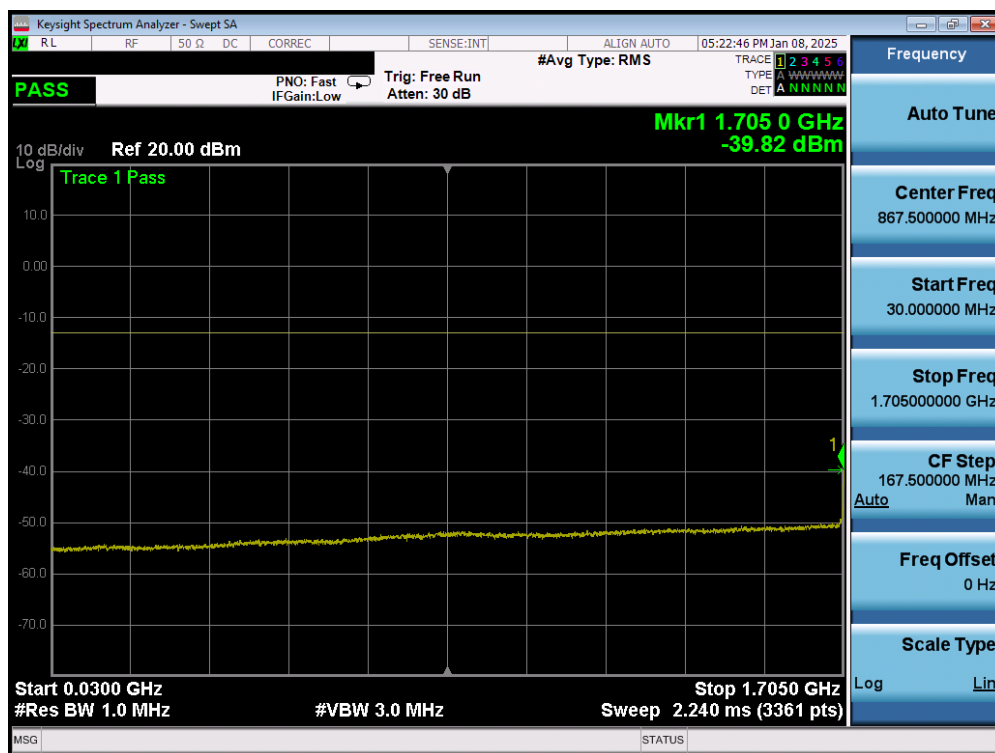
Plot 7-136. Conducted Spurious Plot (WCDMA Ch. 1312- Low Channel – Ant2)
