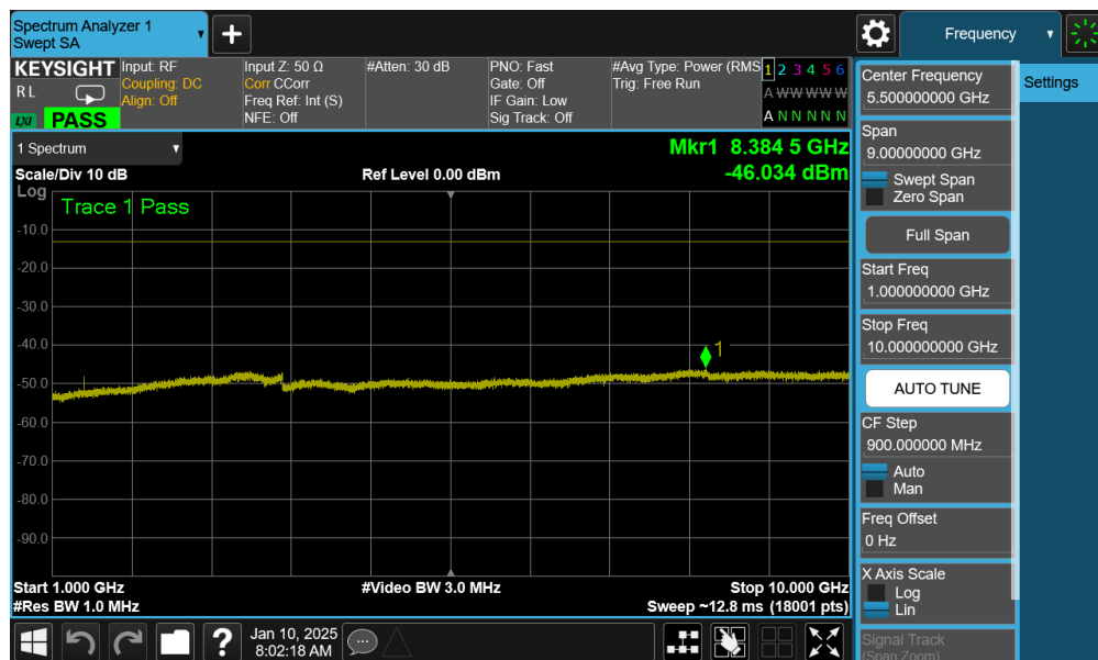
Plot 7-135. Conducted Spurious Plot (NR Band n71 - 20.0MHz - 1 RB - Mid Channel - Ant1)
