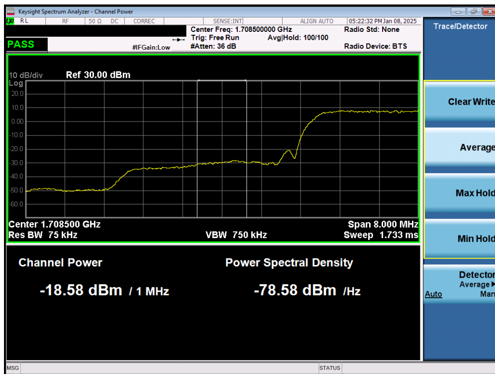
Plot 7-168. Lower Extended Band Edge Plot (WCDMA AWS – Ch. 1312 – Ant2)
