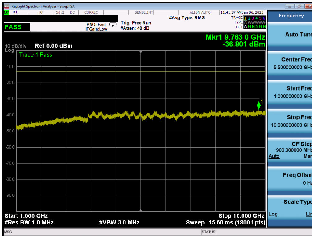
Plot 7-126. Conducted Spurious Plot (LTE Band 71 - 20MHz QPSK - 1 RB - Low Channel - Ant1)
