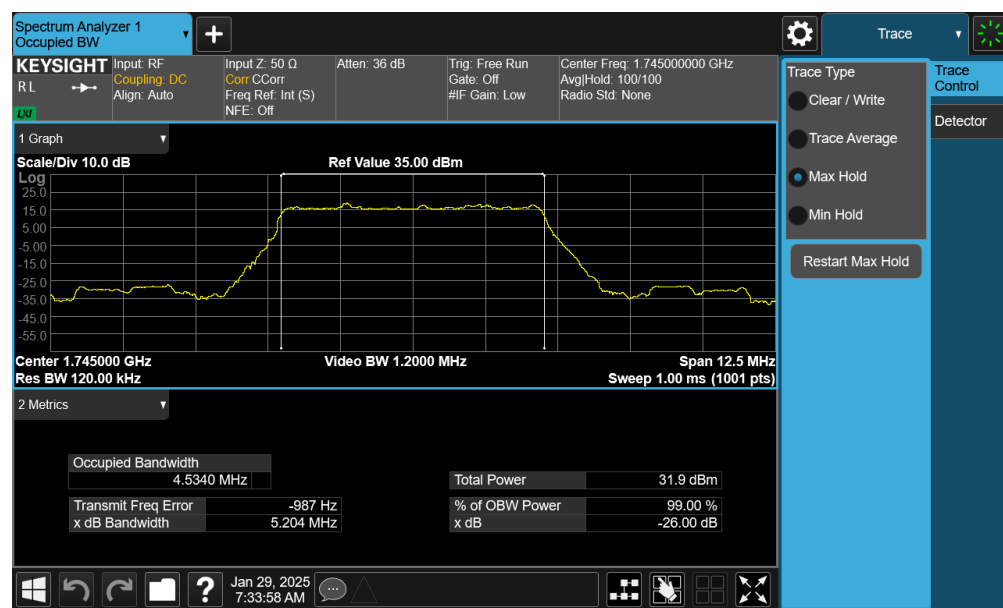
Plot 7-121. Occupied Bandwidth Plot (NR Band n66 - 5.0MHz DFT-s-OFDM BPSK - Full RB – Ant4)
