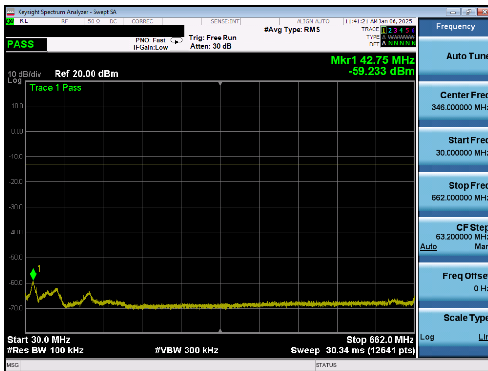
Plot 7-124. Conducted Spurious Plot (LTE Band 71 - 20MHz QPSK - 1 RB - Low Channel - Ant1)
