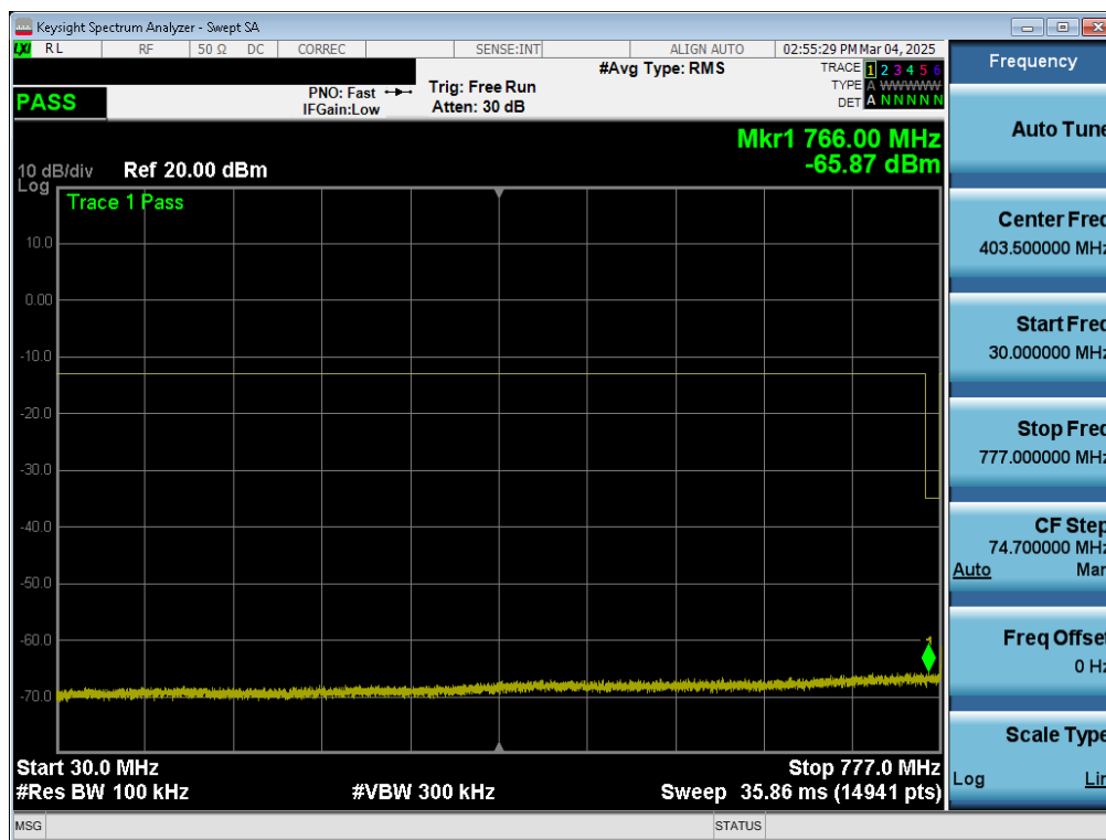
Plot 7-130. Conducted Spurious Plot (LTE Band 13 - 10MHz QPSK - 1 RB)
