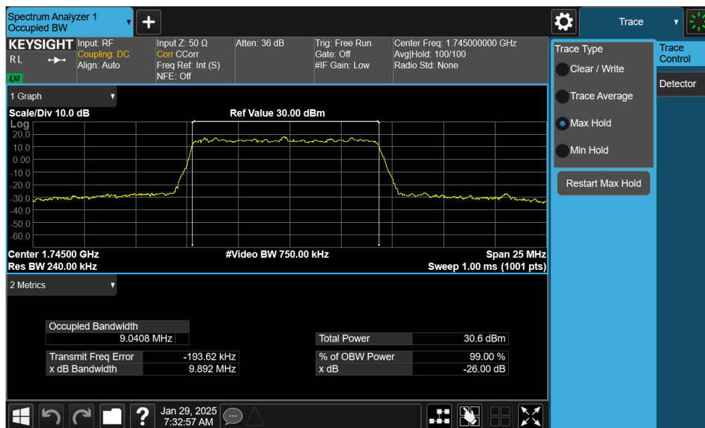
Plot 7-120. Occupied Bandwidth Plot (NR Band n66 - 10.0MHz CP-OFDM 16QAM - Full RB – Ant4)
