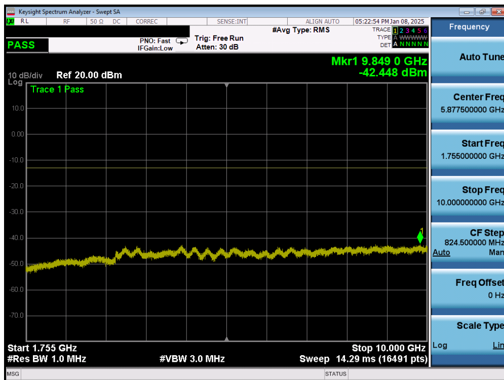
Plot 7-137. Conducted Spurious Plot (WCDMA Ch. 1312- Low Channel – Ant2)
