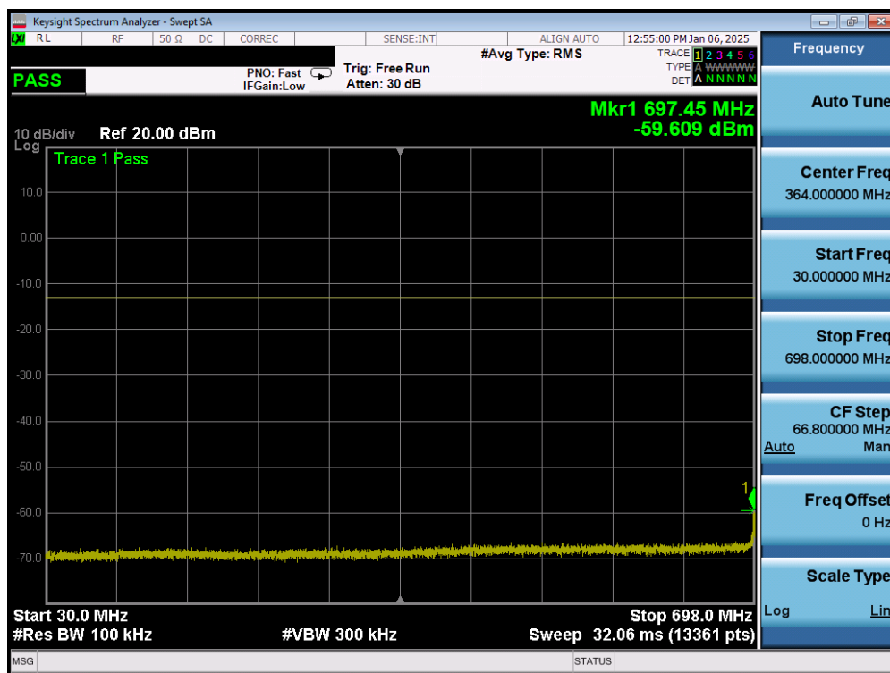
Plot 7-127. Conducted Spurious Plot (LTE Band 12 - 10MHz QPSK - 1 RB - High Channel - Ant1)
