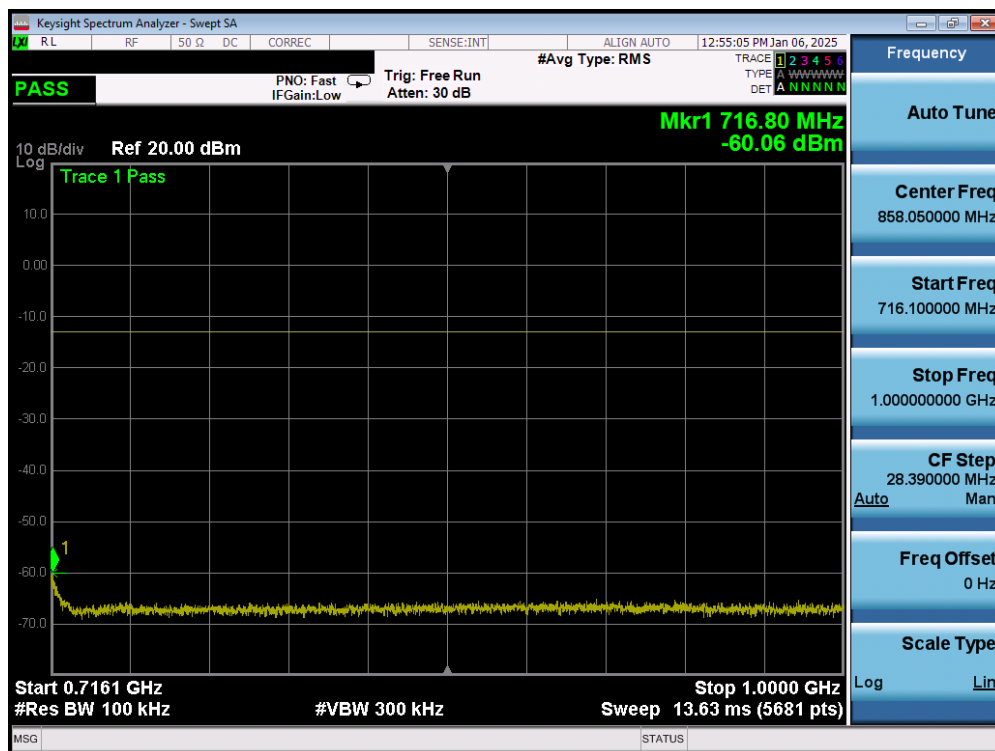
Plot 7-128. Conducted Spurious Plot (LTE Band 12 - 10MHz QPSK - 1 RB - High Channel - Ant1)
