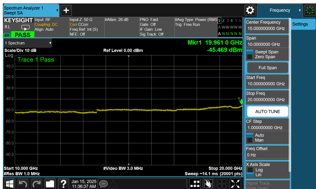
Plot 7-156. Conducted Spurious Plot (NR Band n66 - 40.0MHz - 1 RB - Mid Channel – Ant4)
