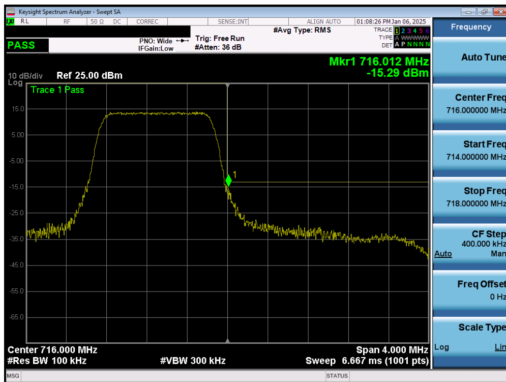
Plot 7-160. Upper Band Edge Plot (LTE Band 12 – 1.4MHz QPSK – Full RB - Ant1)
