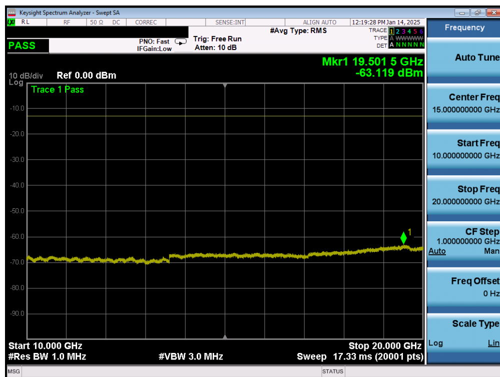
Plot 7-150. Conducted Spurious Plot (LTE Band 66/4 - 20MHz QPSK - 1 RB - High Channel – Ant4)
