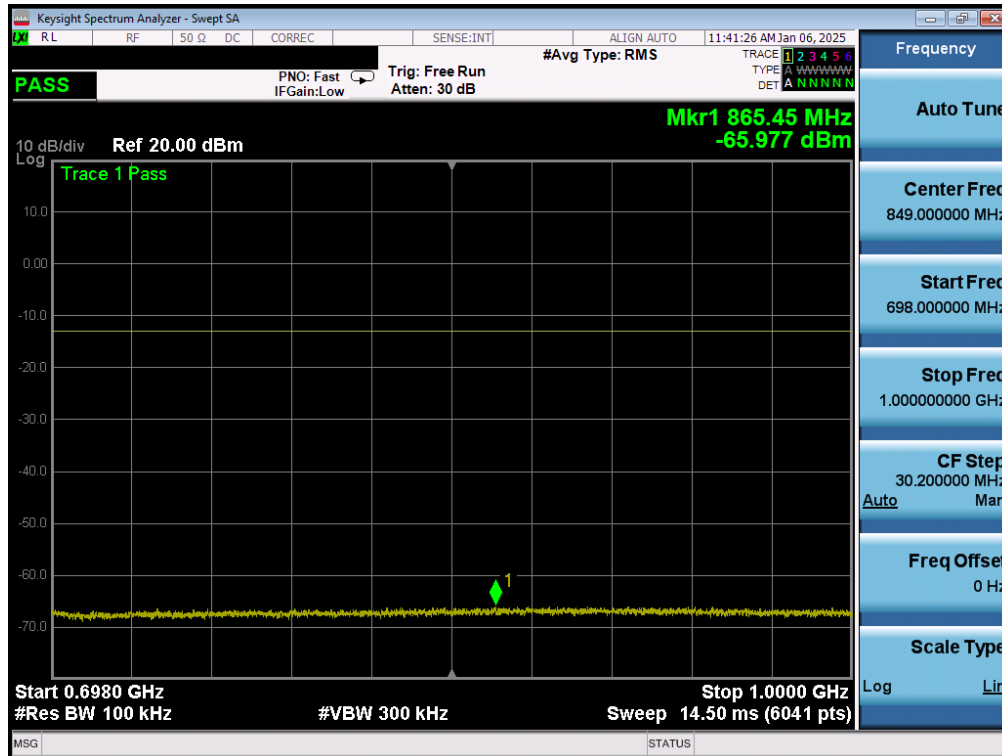
Plot 7-125. Conducted Spurious Plot (LTE Band 71 - 20MHz QPSK - 1 RB - Low Channel - Ant1)
