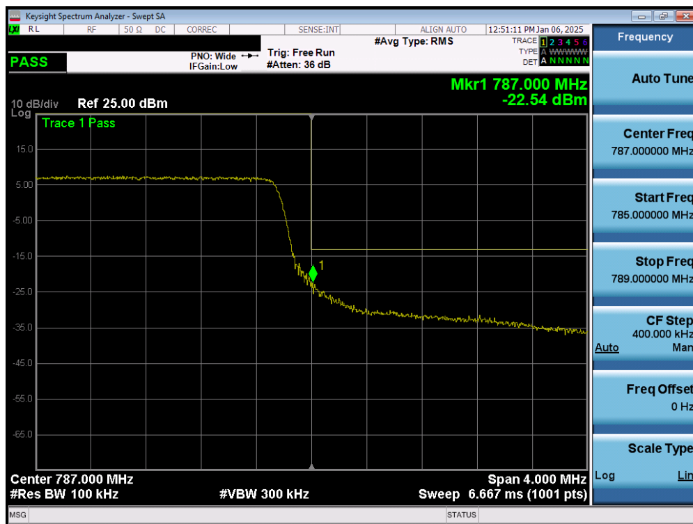
Plot 7-163. Upper Band Edge Plot (LTE Band 13 - 5MHz QPSK – Full RB - Ant1)
