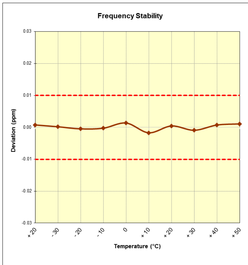
Figure 7-3. Frequency Stability Plot
