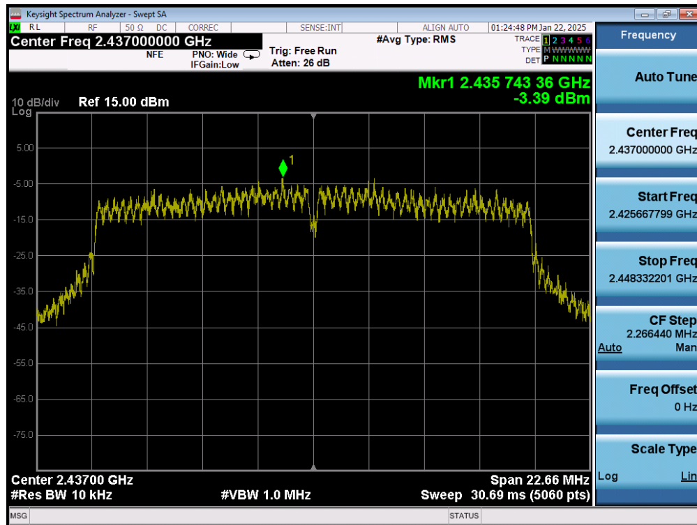
Plot 7-53. Power Spectral Density Plot (802.11n (2.4GHz) – Ch. 6) MIMO ANT2
