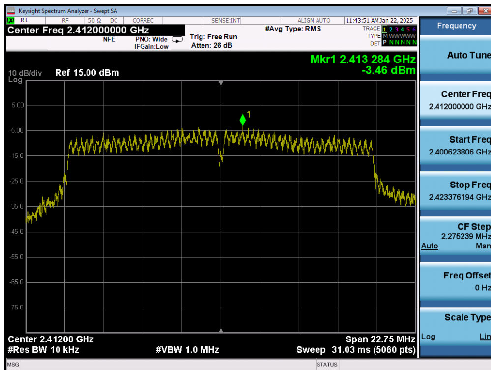
Plot 7-40. Power Spectral Density Plot (802.11ac (2.4GHz) – Ch. 1) MIMO ANT1
