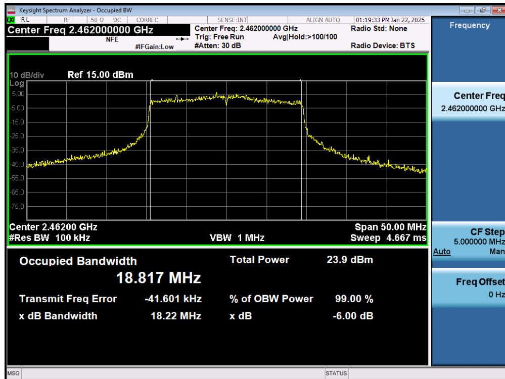
Plot 7-30. 6dB Bandwidth Plot (802.11ax (2.4GHz) – Ch. 11) MIMO ANT2
