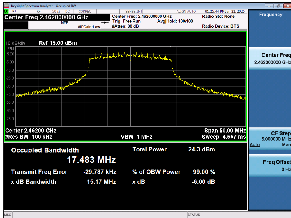
Plot 7-24. 6dB Bandwidth Plot (802.11n (2.4GHz) – Ch. 11) MIMO ANT2
