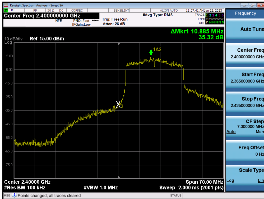
Plot 7-69. Band Edge Plot (802.11ax (2.4GHz) – Ch. 1) MIMO ANT1
