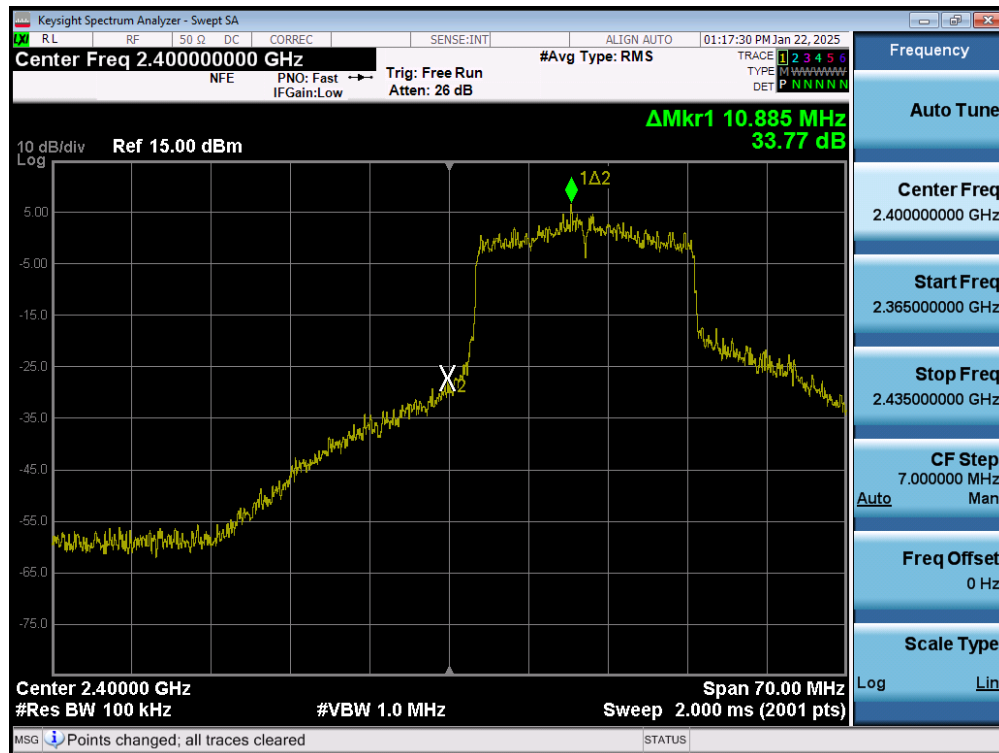
Plot 7-79. Band Edge Plot (802.11ax (2.4GHz) – Ch. 1) MIMO ANT2
