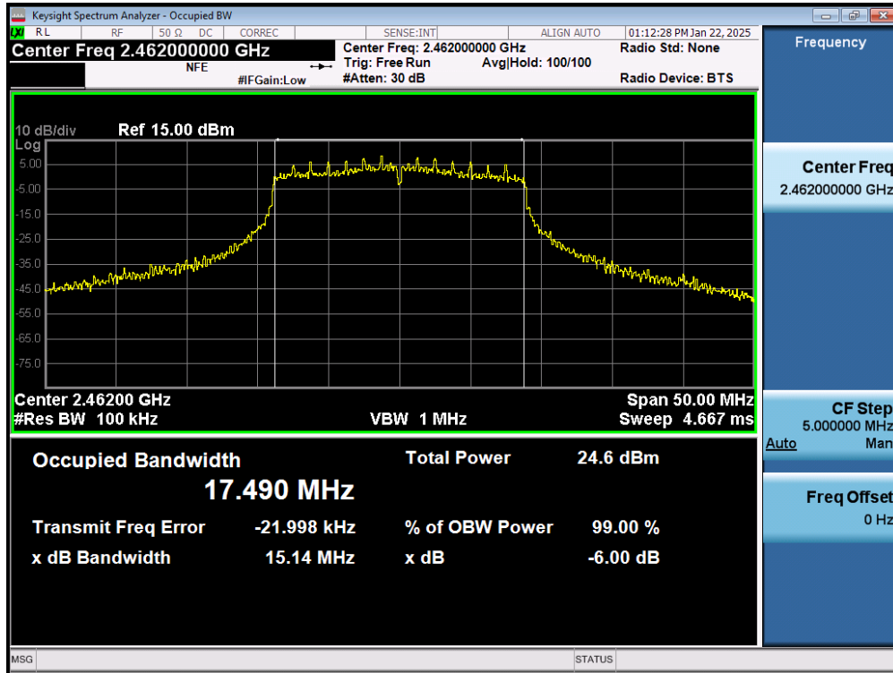
Plot 7-27. 6dB Bandwidth Plot (802.11ac (2.4GHz) – Ch. 11) MIMO ANT2
