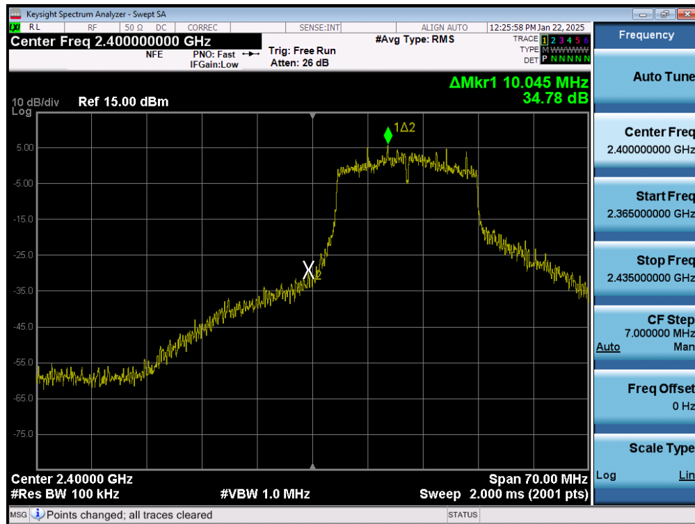
Plot 7-65. Band Edge Plot (802.11n (2.4GHz) – Ch. 1) MIMO ANT1
