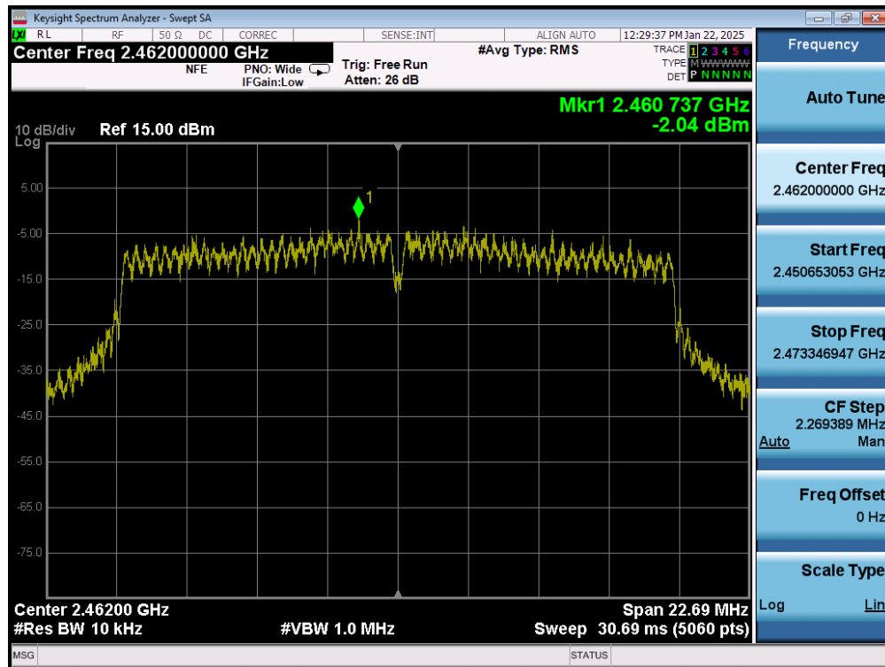
Plot 7-39. Power Spectral Density Plot (802.11n (2.4GHz) – Ch. 11) MIMO ANT1
