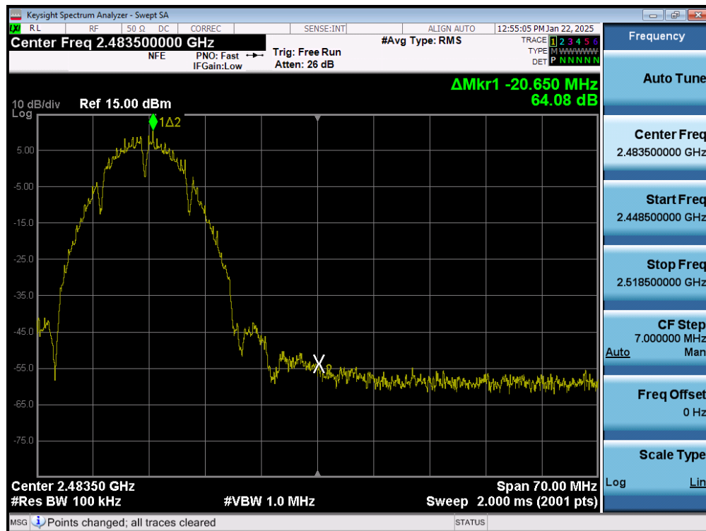
Plot 7-72. Band Edge Plot (802.11b – Ch. 11) MIMO ANT2
