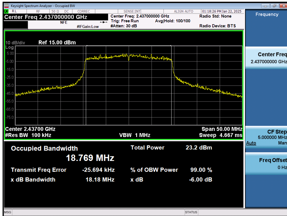
Plot 7-29. 6dB Bandwidth Plot (802.11ax (2.4GHz) – Ch. 6) MIMO ANT2
