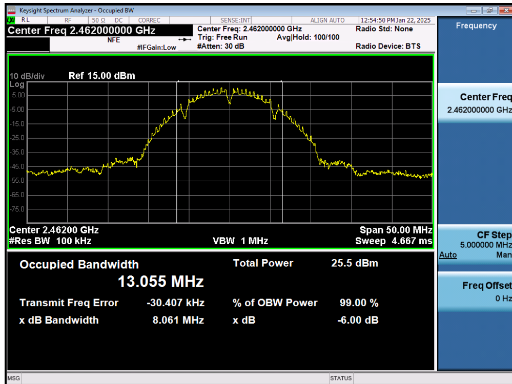
Plot 7-18. 6dB Bandwidth Plot (802.11b – Ch. 11) MIMO ANT2
