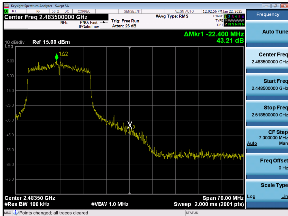
Plot 7-70. Band Edge Plot (802.11ax (2.4GHz) – Ch. 11) MIMO ANT1
