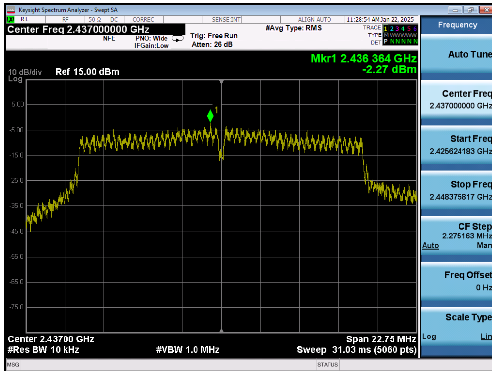
Plot 7-35. Power Spectral Density Plot (802.11g – Ch. 6) MIMO ANT1
