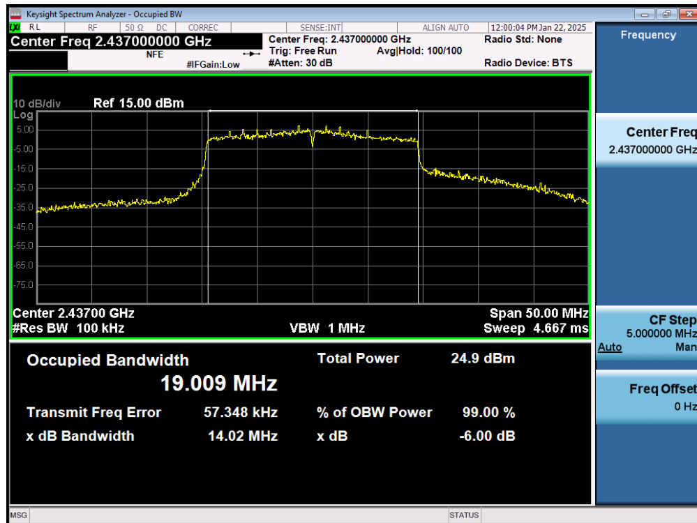
Plot 7-14. 6dB Bandwidth Plot (802.11ax (2.4GHz) – Ch. 6) MIMO ANT1
