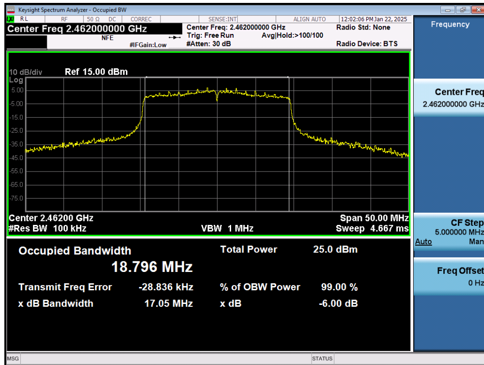
Plot 7-15. 6dB Bandwidth Plot (802.11ax (2.4GHz) – Ch. 11) MIMO ANT1
