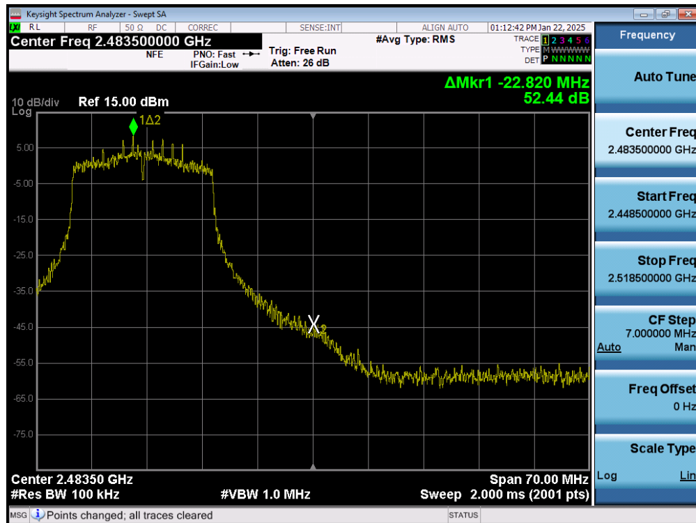
Plot 7-78. Band Edge Plot (802.11ac (2.4GHz) – Ch. 11) MIMO ANT2
