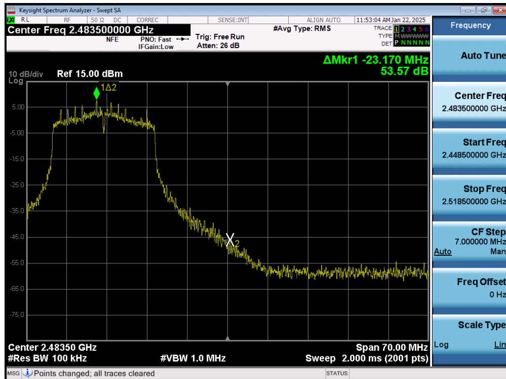
Plot 7-68. Band Edge Plot (802.11ac (2.4GHz) – Ch. 11) MIMO ANT1
