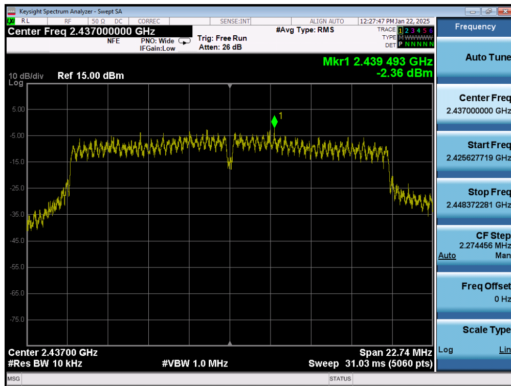
Plot 7-38. Power Spectral Density Plot (802.11n (2.4GHz) – Ch. 6) MIMO ANT1
