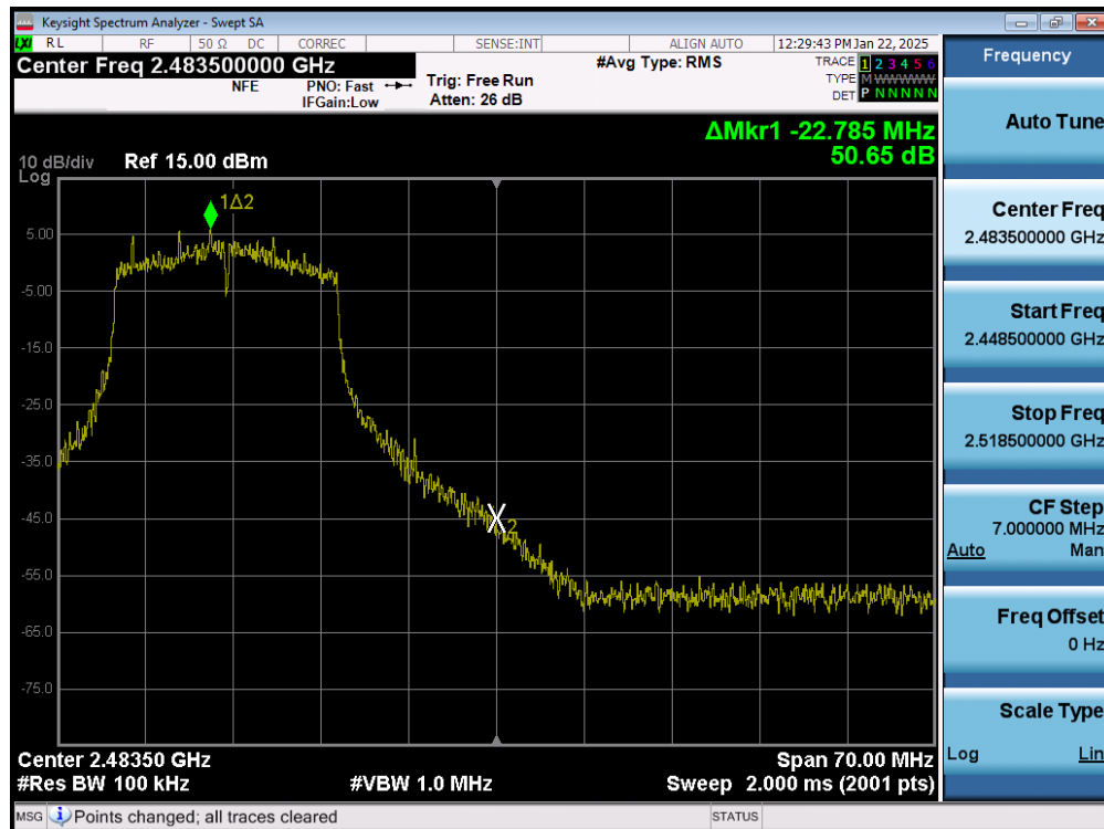
Plot 7-66. Band Edge Plot (802.11n (2.4GHz) – Ch. 11) MIMO ANT1
