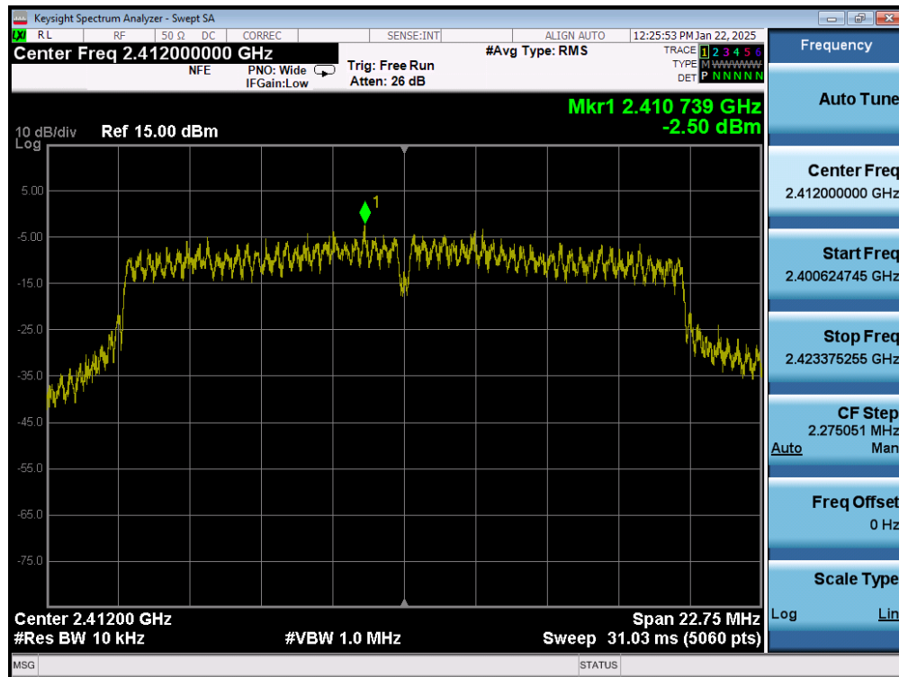
Plot 7-37. Power Spectral Density Plot (802.11n (2.4GHz) – Ch. 1) MIMO ANT1
