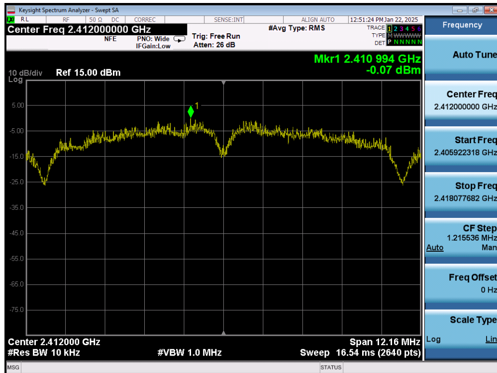
Plot 7-46. Power Spectral Density Plot (802.11b – Ch. 1) MIMO ANT2
