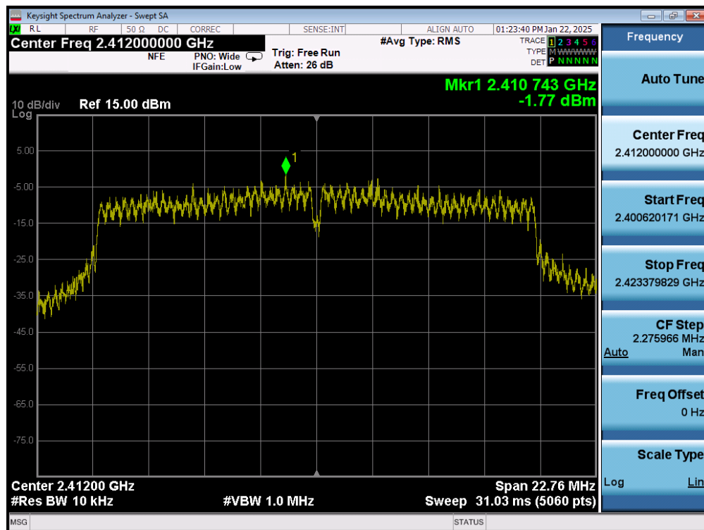
Plot 7-52. Power Spectral Density Plot (802.11n (2.4GHz) – Ch. 1) MIMO ANT2
