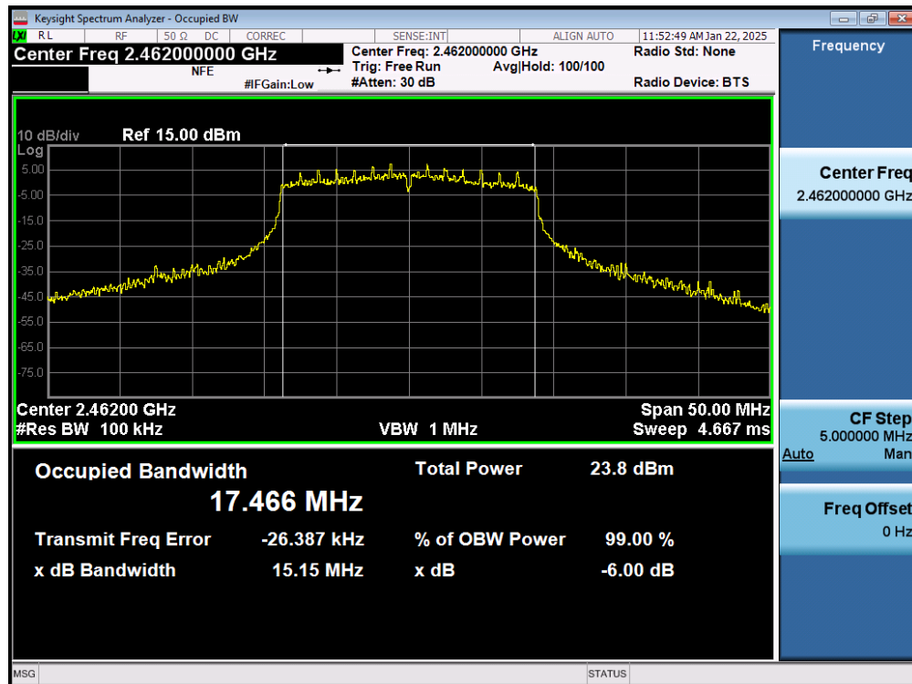
Plot 7-12. 6dB Bandwidth Plot (802.11ac (2.4GHz) – Ch. 11) MIMO ANT1
