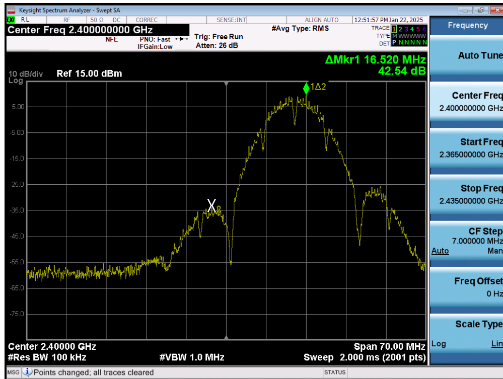
Plot 7-71. Band Edge Plot (802.11b – Ch. 1) MIMO ANT2
