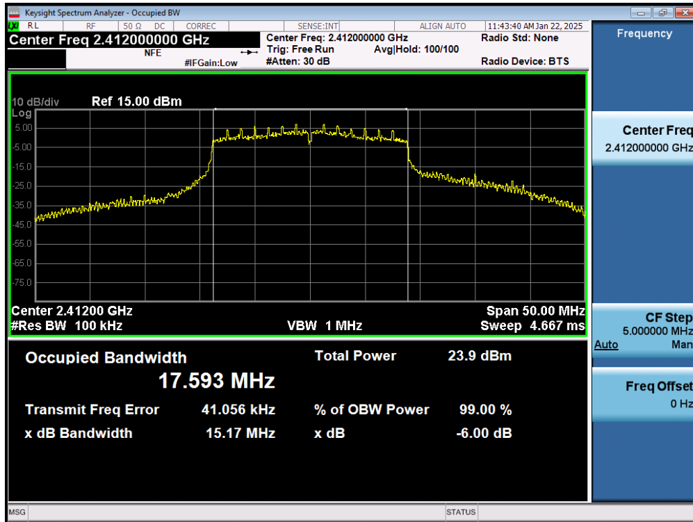
Plot 7-10. 6dB Bandwidth Plot (802.11ac (2.4GHz) – Ch. 1) MIMO ANT1
