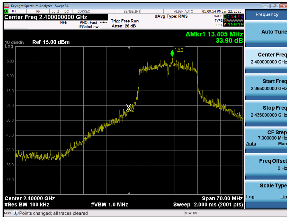
Plot 7-77. Band Edge Plot (802.11ac (2.4GHz) – Ch. 1) MIMO ANT2
