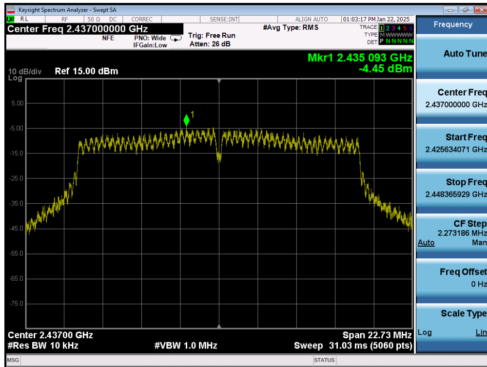
Plot 7-50. Power Spectral Density Plot (802.11g – Ch. 6) MIMO ANT2
