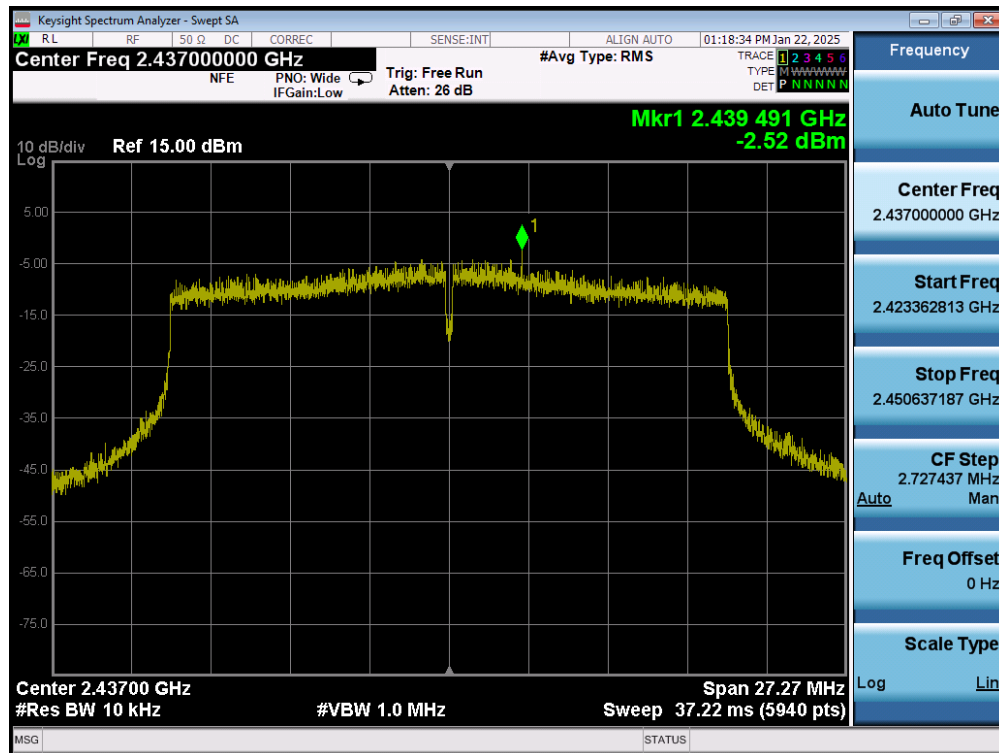
Plot 7-59. Power Spectral Density Plot (802.11ax (2.4GHz) – Ch. 6) MIMO ANT2
