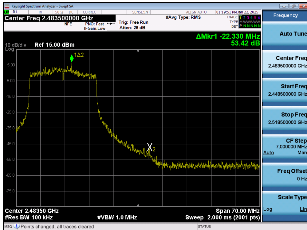
Plot 7-80. Band Edge Plot (802.11ax (2.4GHz) – Ch. 11) MIMO ANT2
