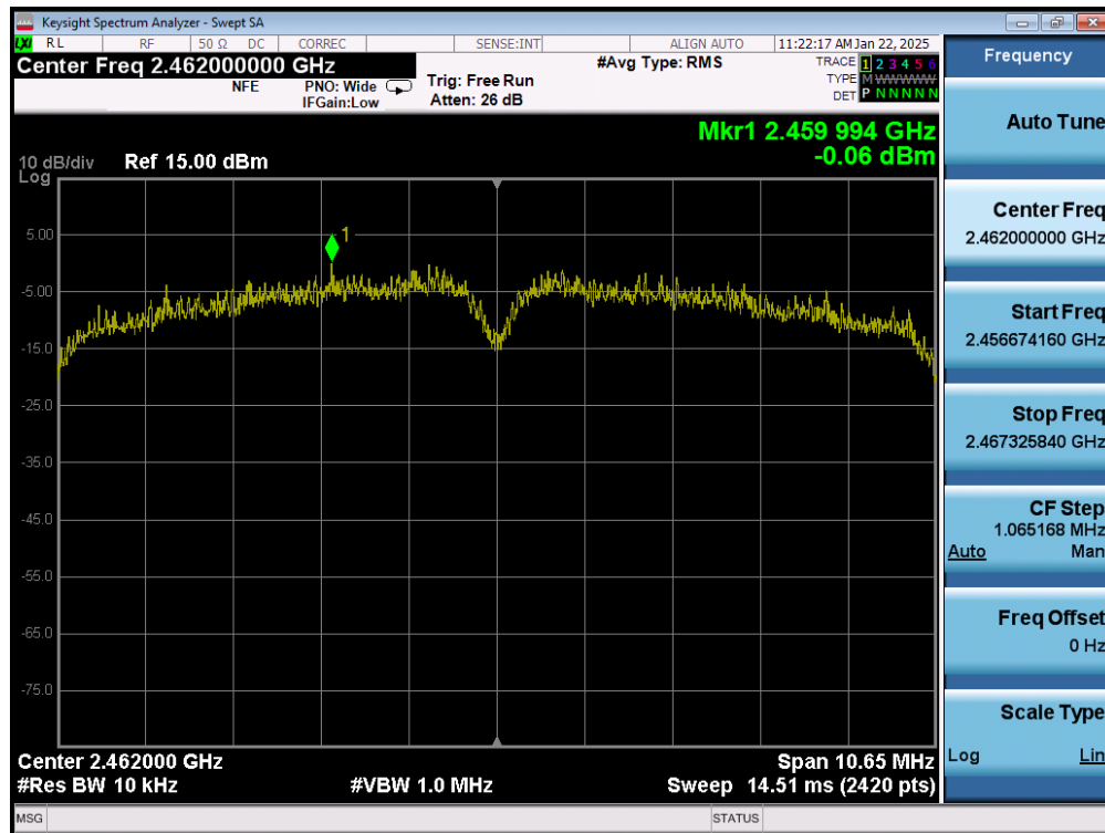
Plot 7-33. Power Spectral Density Plot (802.11b – Ch. 11) MIMO ANT1
