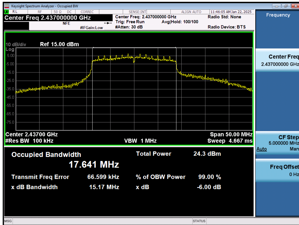
Plot 7-11. 6dB Bandwidth Plot (802.11ac (2.4GHz) – Ch. 6) MIMO ANT1
