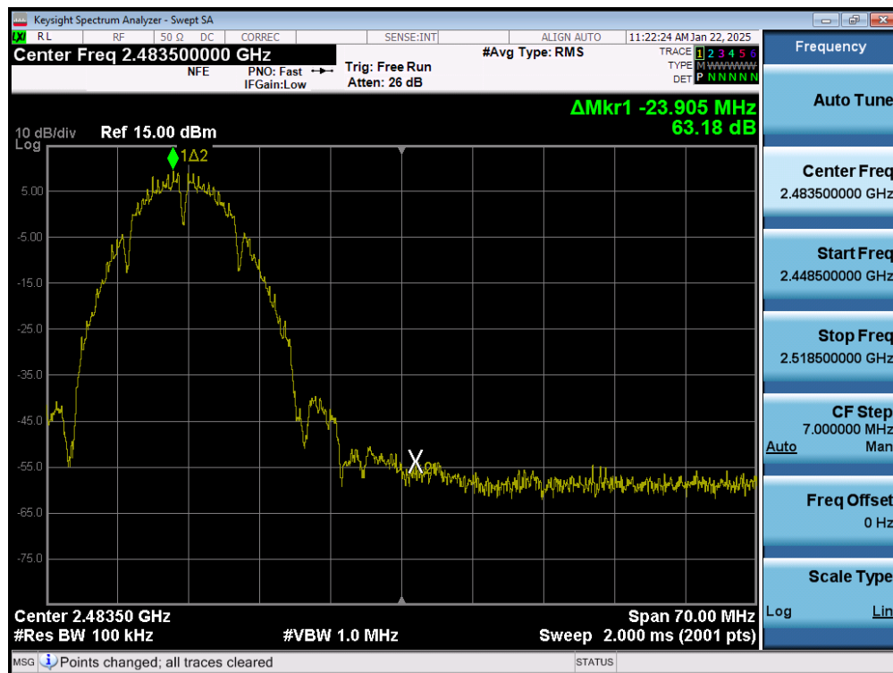
Plot 7-62. Band Edge Plot (802.11b – Ch. 11) MIMO ANT1
