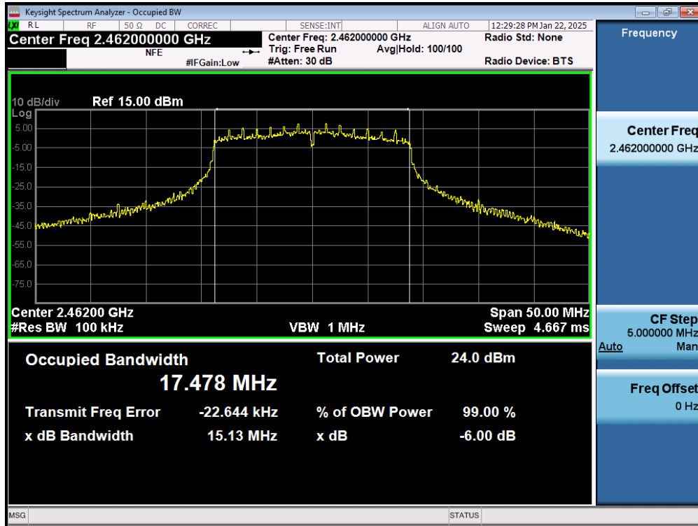
Plot 7-9. 6dB Bandwidth Plot (802.11n (2.4GHz) – Ch. 11) MIMO ANT1
