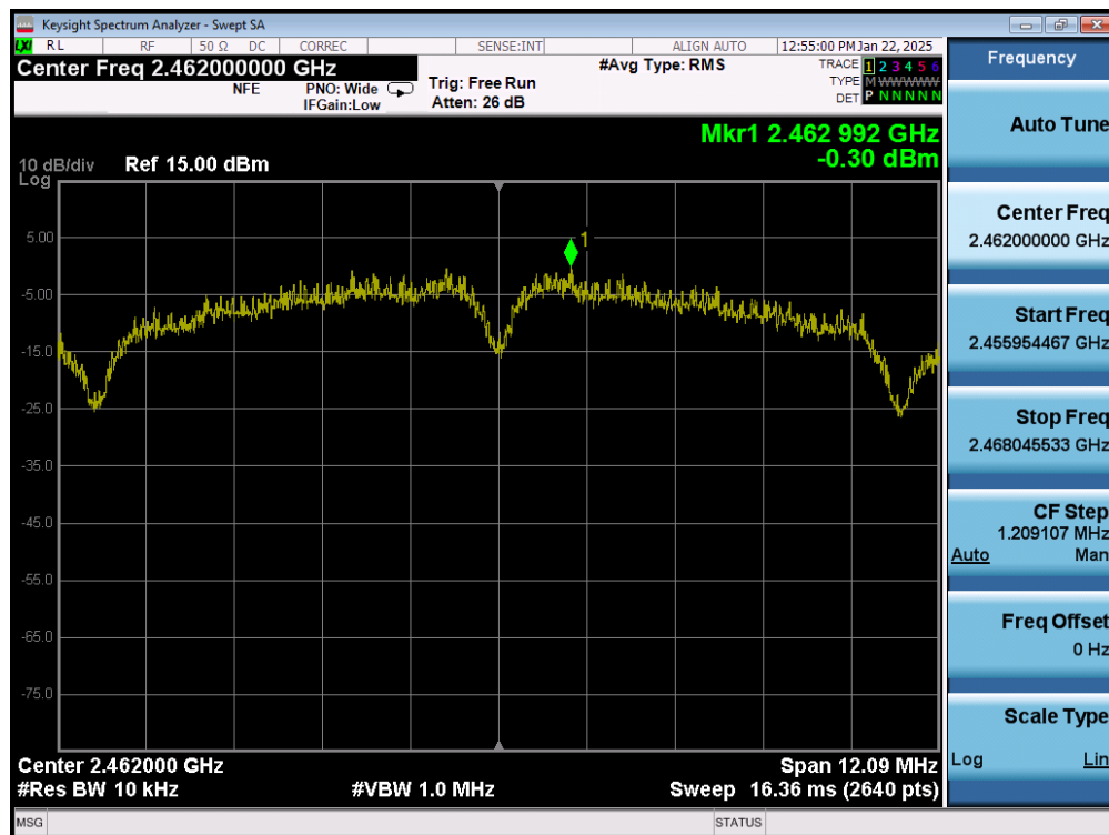
Plot 7-48. Power Spectral Density Plot (802.11b – Ch. 11) MIMO ANT2
