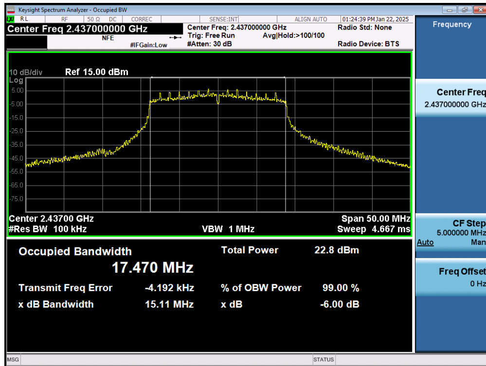
Plot 7-23. 6dB Bandwidth Plot (802.11n (2.4GHz) – Ch. 6) MIMO ANT2
