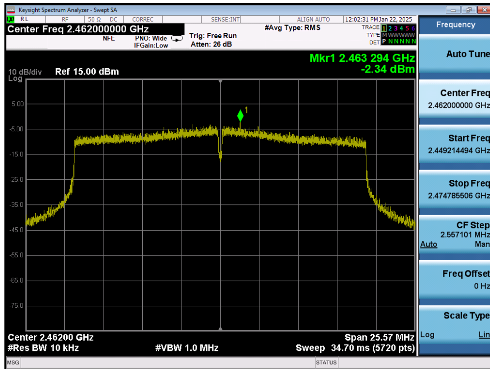
Plot 7-45. Power Spectral Density Plot (802.11ax (2.4GHz) – Ch. 11) MIMO ANT1
