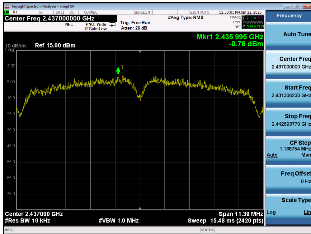
Plot 7-47. Power Spectral Density Plot (802.11b – Ch. 6) MIMO ANT2
