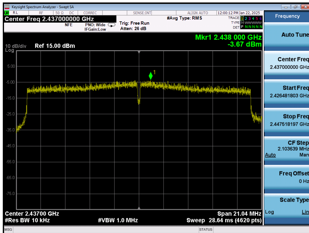
Plot 7-44. Power Spectral Density Plot (802.11ax (2.4GHz) – Ch. 6) MIMO ANT1
