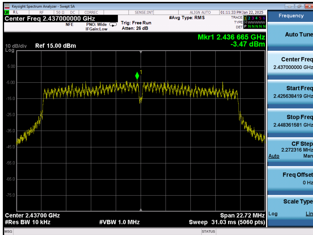
Plot 7-56. Power Spectral Density Plot (802.11ac (2.4GHz) – Ch. 6) MIMO ANT2
