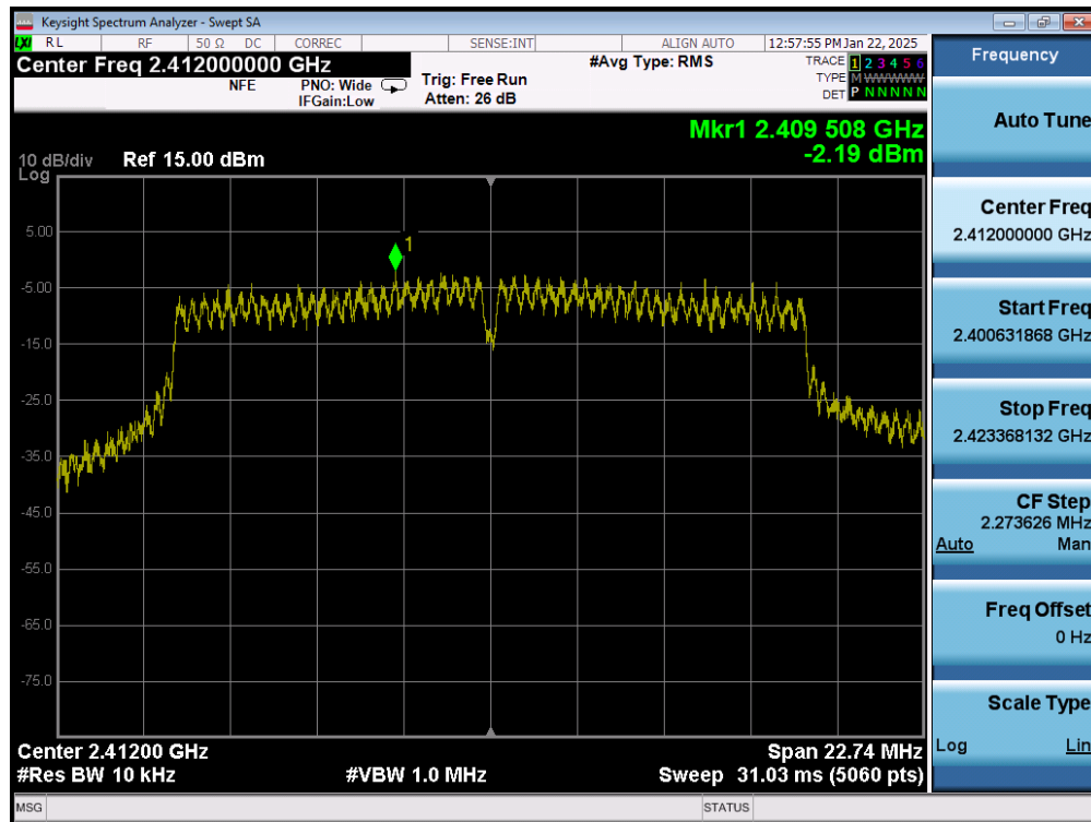
Plot 7-49. Power Spectral Density Plot (802.11g – Ch. 1) MIMO ANT2
