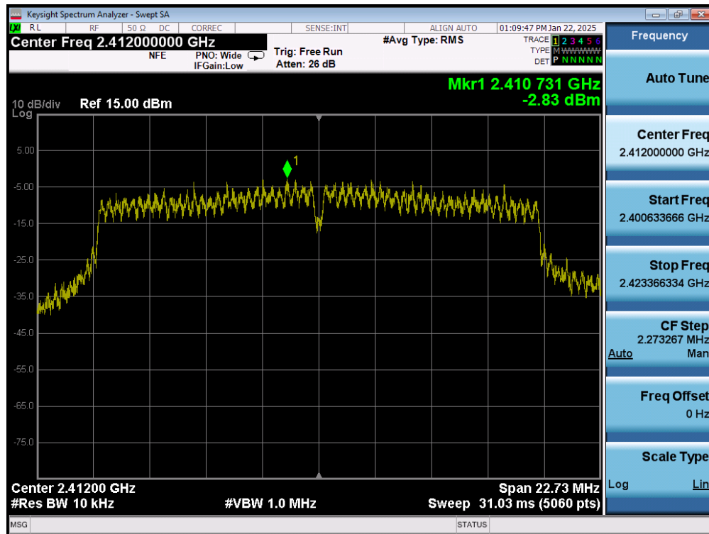
Plot 7-55. Power Spectral Density Plot (802.11ac (2.4GHz) – Ch. 1) MIMO ANT2
