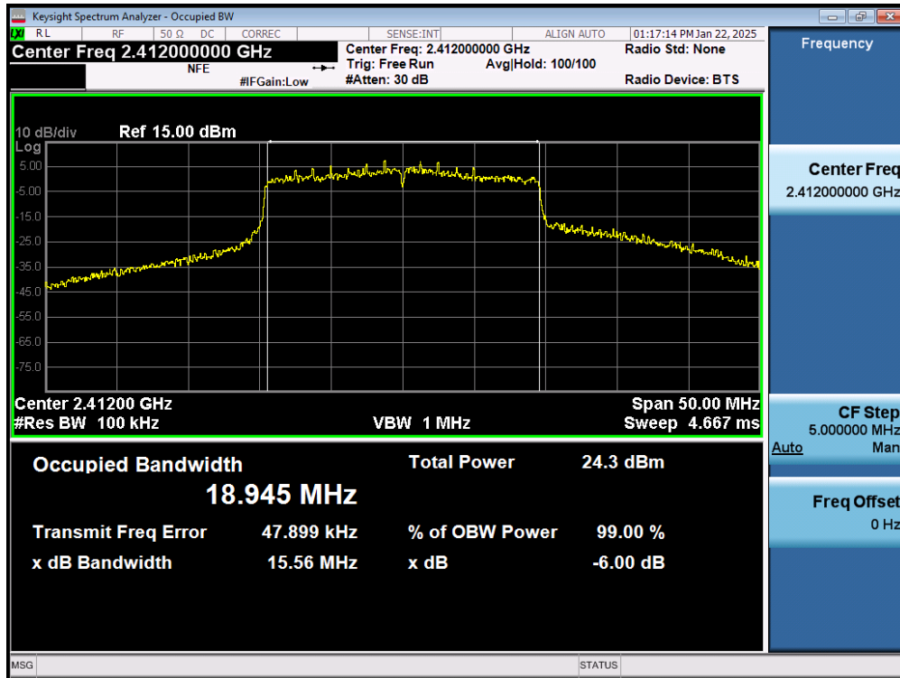
Plot 7-28. 6dB Bandwidth Plot (802.11ax (2.4GHz) – Ch. 1) MIMO ANT2
