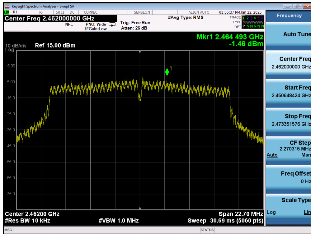
Plot 7-51. Power Spectral Density Plot (802.11g – Ch. 11) MIMO ANT2
