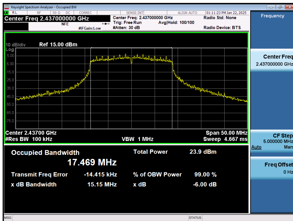
Plot 7-26. 6dB Bandwidth Plot (802.11ac (2.4GHz) – Ch. 6) MIMO ANT2
