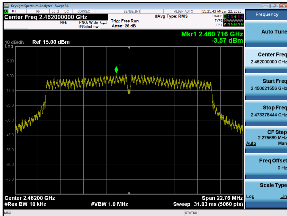
Plot 7-36. Power Spectral Density Plot (802.11g – Ch. 11) MIMO ANT1
