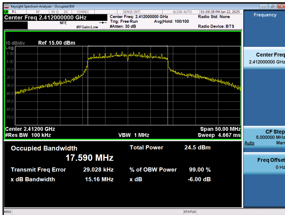
Plot 7-25. 6dB Bandwidth Plot (802.11ac (2.4GHz) – Ch. 1) MIMO ANT2
