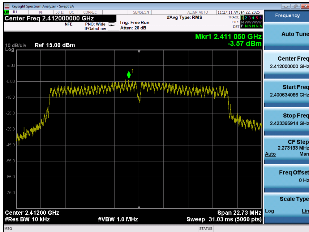
Plot 7-34. Power Spectral Density Plot (802.11g – Ch. 1) MIMO ANT1
