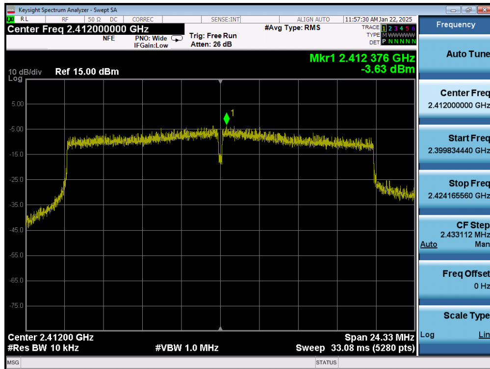
Plot 7-43. Power Spectral Density Plot (802.11ax (2.4GHz) – Ch. 1) MIMO ANT1
