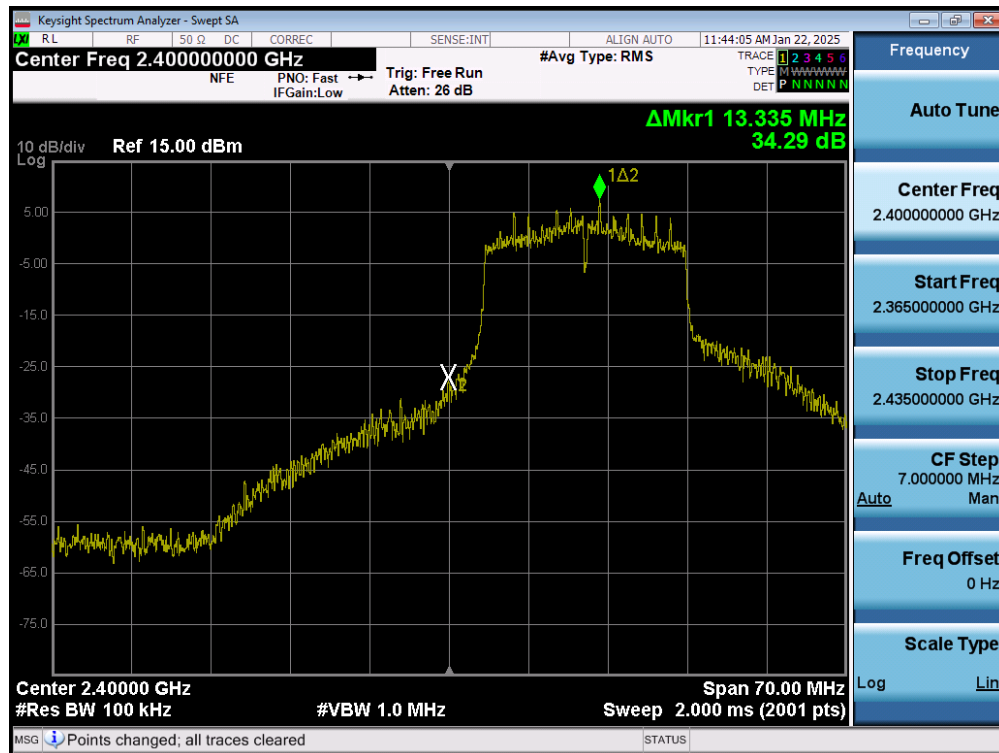
Plot 7-67. Band Edge Plot (802.11ac (2.4GHz) – Ch. 1) MIMO ANT1
