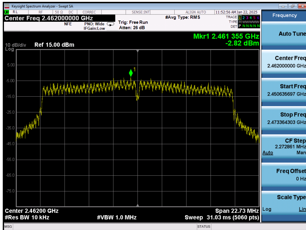
Plot 7-42. Power Spectral Density Plot (802.11ac (2.4GHz) – Ch. 11) MIMO ANT1
