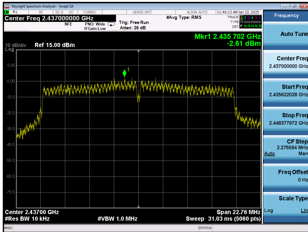
Plot 7-41. Power Spectral Density Plot (802.11ac (2.4GHz) – Ch. 6) MIMO ANT1
