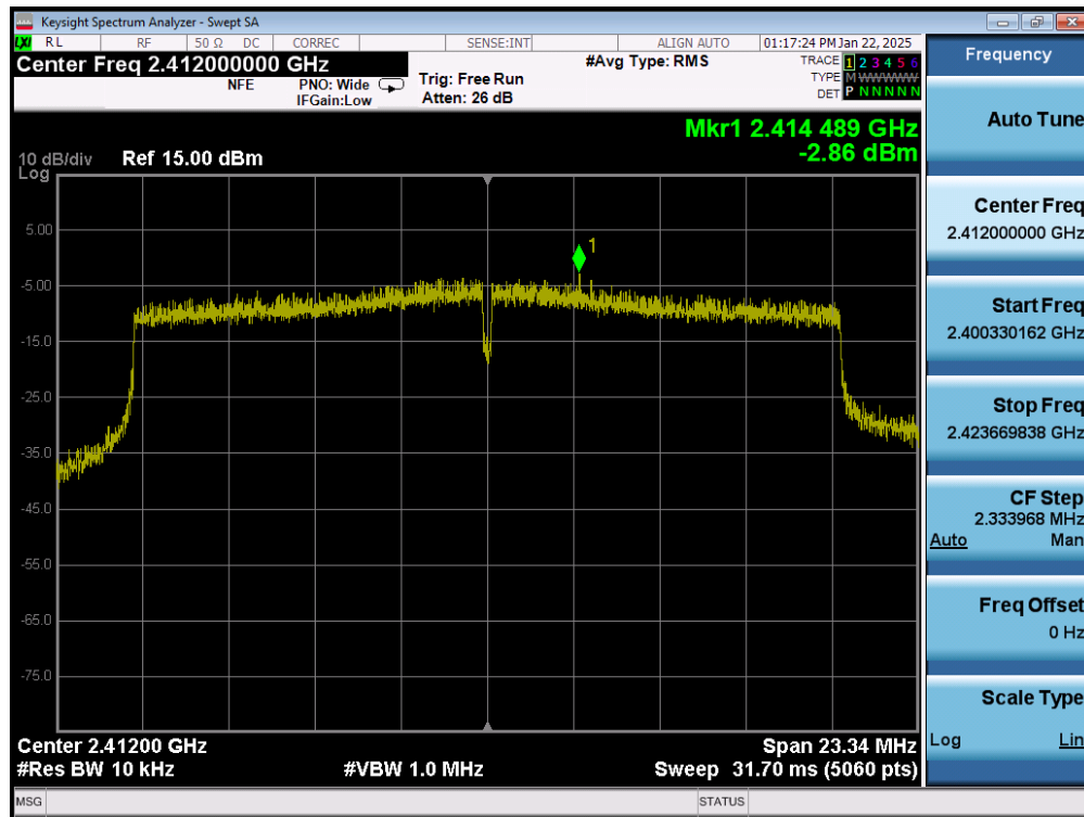
Plot 7-58. Power Spectral Density Plot (802.11ax (2.4GHz) – Ch. 1) MIMO ANT2
