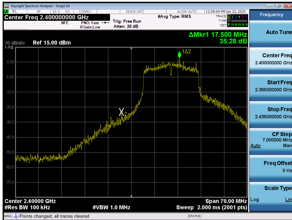
Plot 7-73. Band Edge Plot (802.11g– Ch. 1) MIMO ANT2
