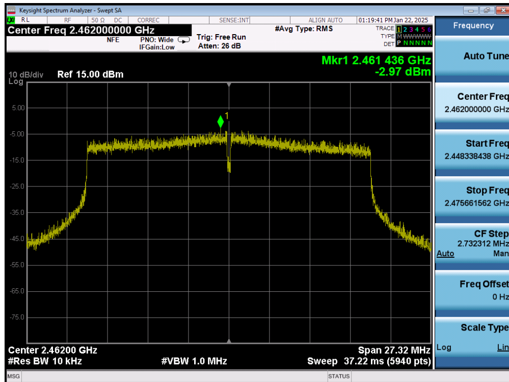
Plot 7-60. Power Spectral Density Plot (802.11ax (2.4GHz) – Ch. 11) MIMO ANT2
