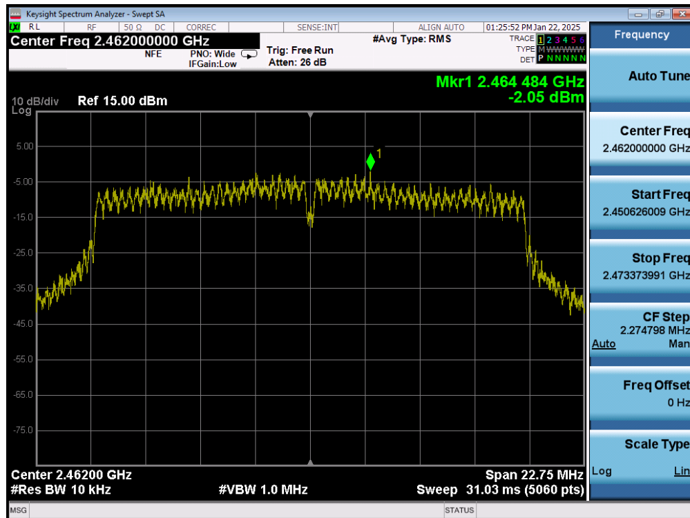
Plot 7-54. Power Spectral Density Plot (802.11n (2.4GHz) – Ch. 11) MIMO ANT2
