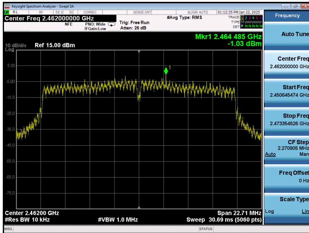
Plot 7-57. Power Spectral Density Plot (802.11ac (2.4GHz) – Ch. 11) MIMO ANT2
