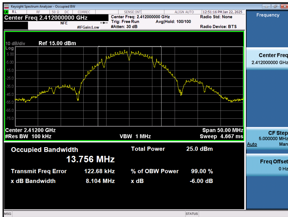
Plot 7-16. 6dB Bandwidth Plot (802.11b – Ch. 1) MIMO ANT2
