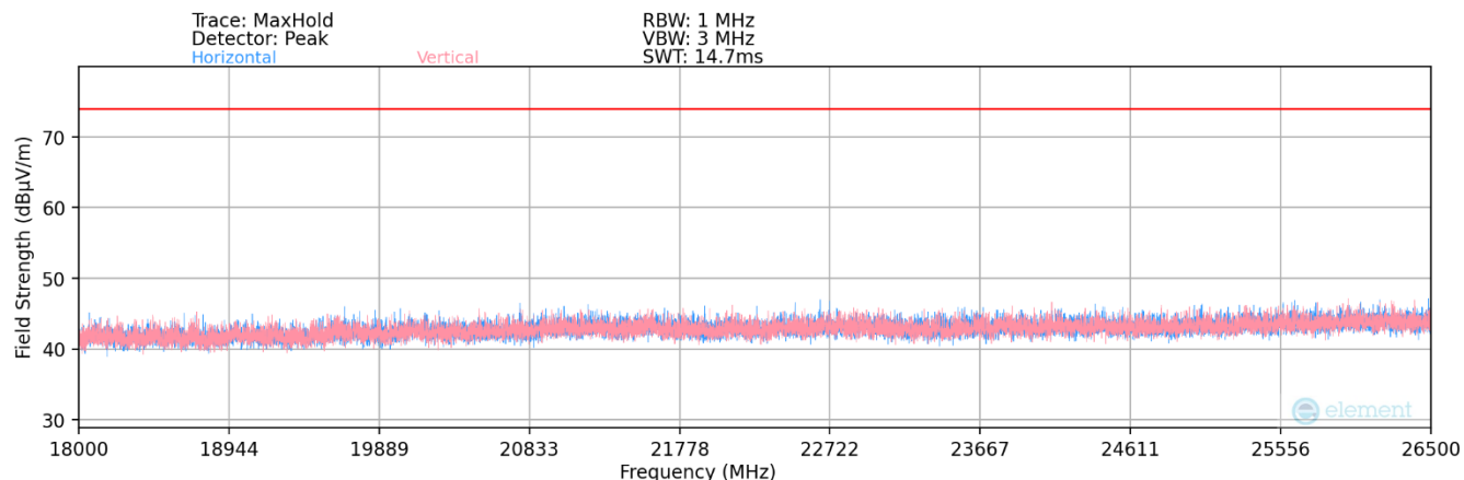
Plot 7-70. Radiated Spurious Plot above 18GHz MIMO (802.11ax OFDMA – 26 Tones)
