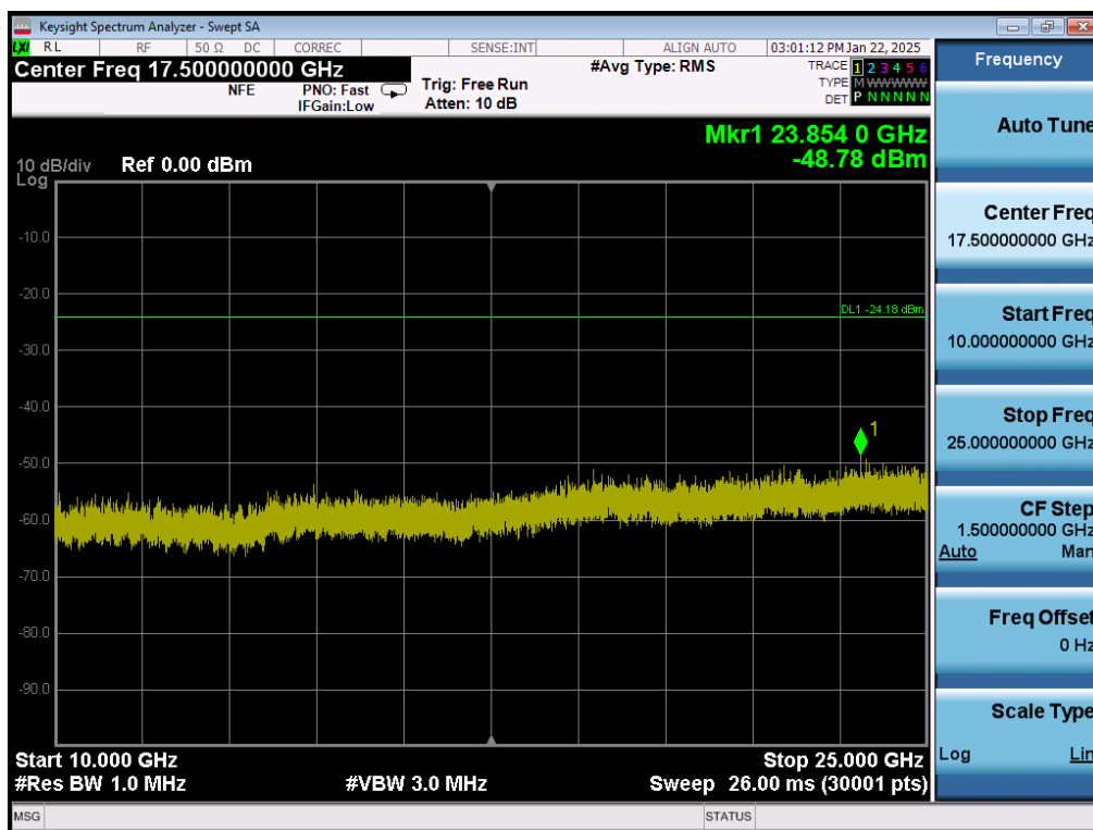
Plot 7-66. Conducted Spurious Plot MIMO ANT2 (802.11ax OFDMA – 242 Tones – Ch. 11)
