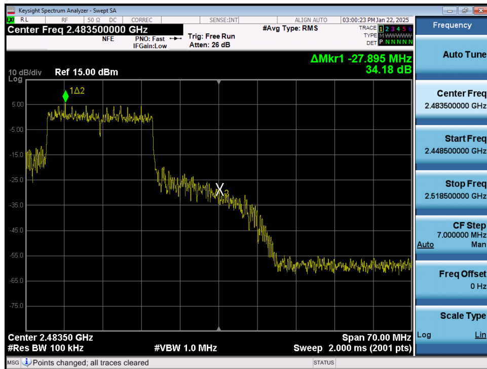
Plot 7-42. Band Edge Plot MIMO ANT2 (802.11ax OFDMA – 242 Tones – Ch. 11)
