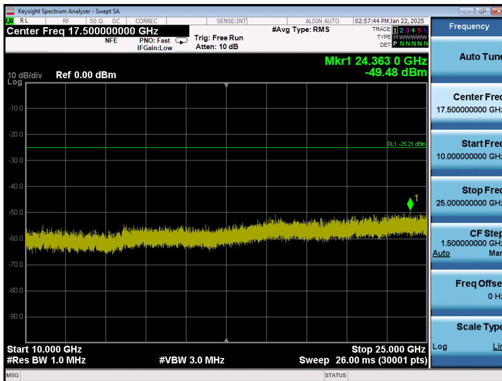
Plot 7-64. Conducted Spurious Plot MIMO ANT2 (802.11ax OFDMA – 242 Tones – Ch. 6)
