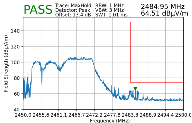
Plot 7-82. Radiated Restricted Upper Band Edge Measurement MIMO (Peak – 106 Tones)
