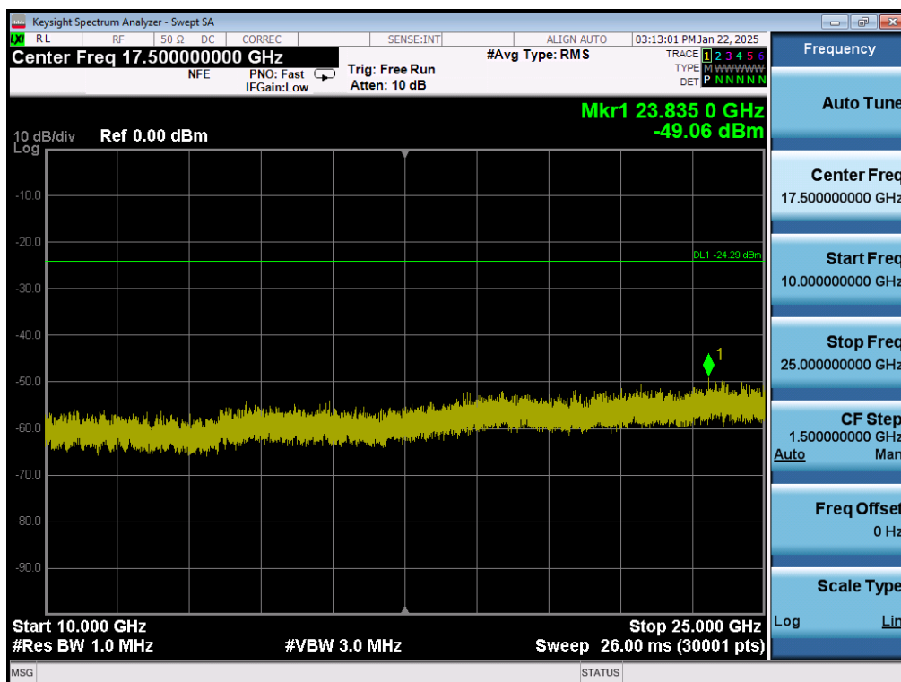
Plot 7-54. Conducted Spurious Plot MIMO ANT1 (802.11ax OFDMA – 242 Tones – Ch. 11)
