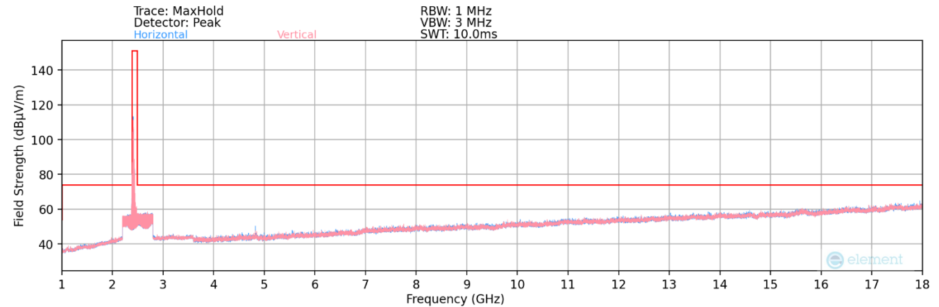
Plot 7-67. Radiated Spurious Plot above 1GHz MIMO (802.11ax OFDMA – 26 Tones – Ch. 1)
