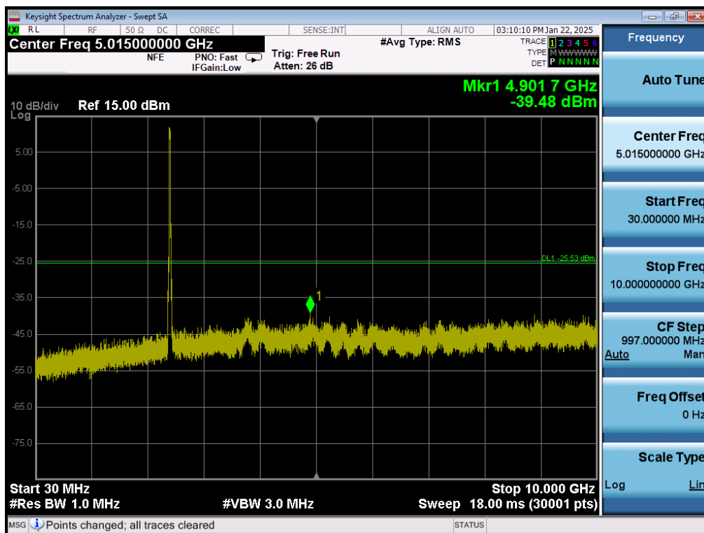
Plot 7-49. Conducted Spurious Plot MIMO ANT1 (802.11ax OFDMA – 242 Tones – Ch. 1)
