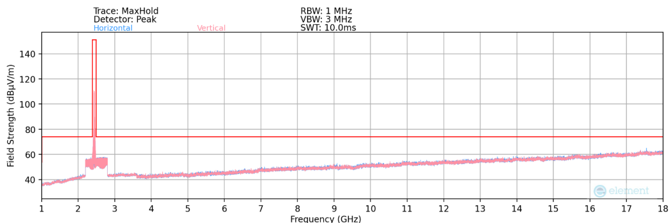
Plot 7-72. Radiated Spurious Plot above 1GHz MIMO (802.11ax OFDMA – 242 Tones – Ch. 6)
