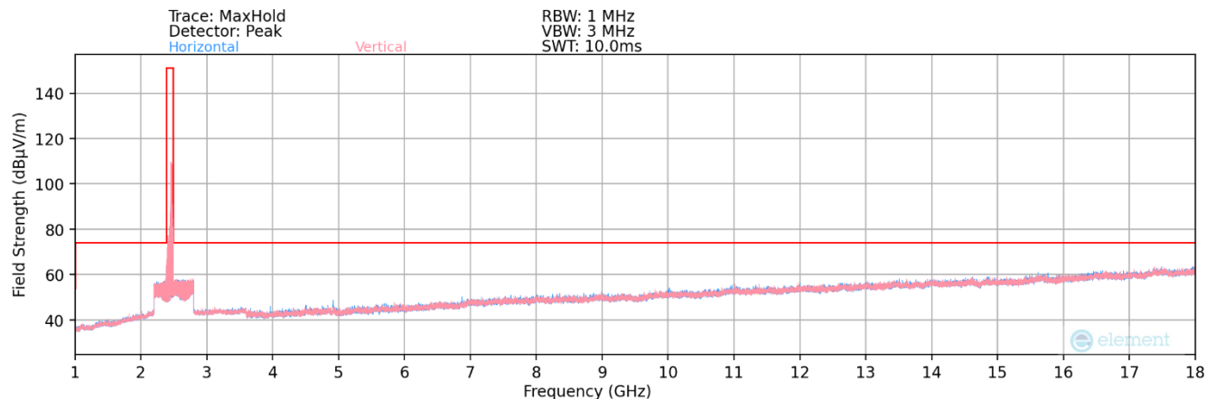
Plot 7-73. Radiated Spurious Plot above 1GHz MIMO (802.11ax OFDMA – 242 Tones – Ch. 11)
