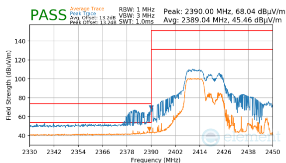
Plot 7-76. Radiated Restricted Lower Band Edge Measurement MIMO (Average and Peak – 106 Tones)
