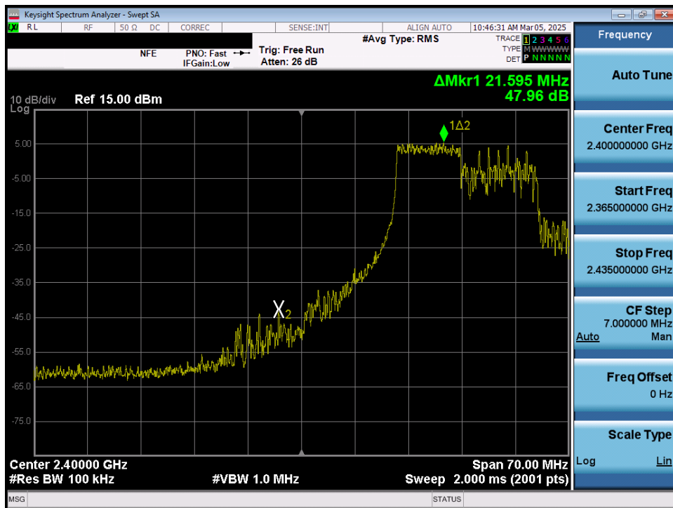
Plot 7-36. Band Edge Plot MIMO ANT2 (802.11ax OFDMA – 106 Tones – Ch. 3)
