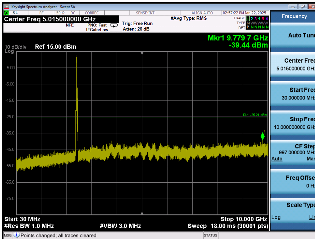
Plot 7-63. Conducted Spurious Plot MIMO ANT2 (802.11ax OFDMA – 242 Tones – Ch. 6)
