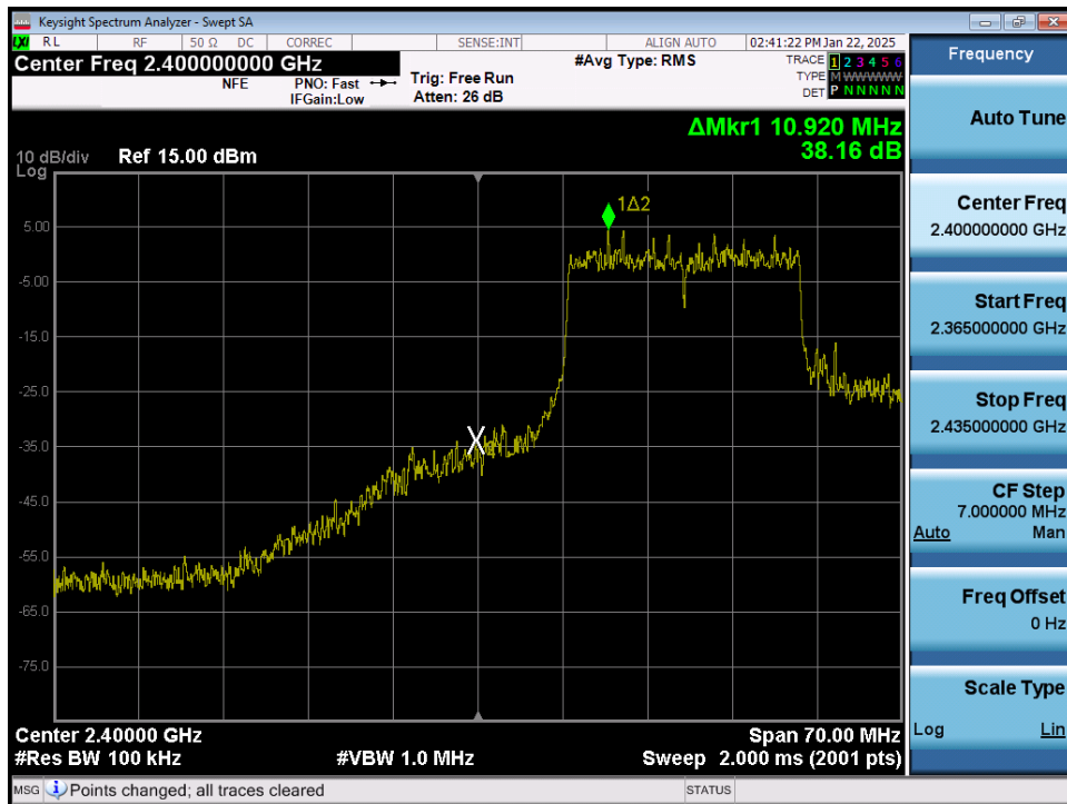
Plot 7-40. Band Edge Plot MIMO ANT2 (802.11ax OFDMA – 242 Tones – Ch. 2)
