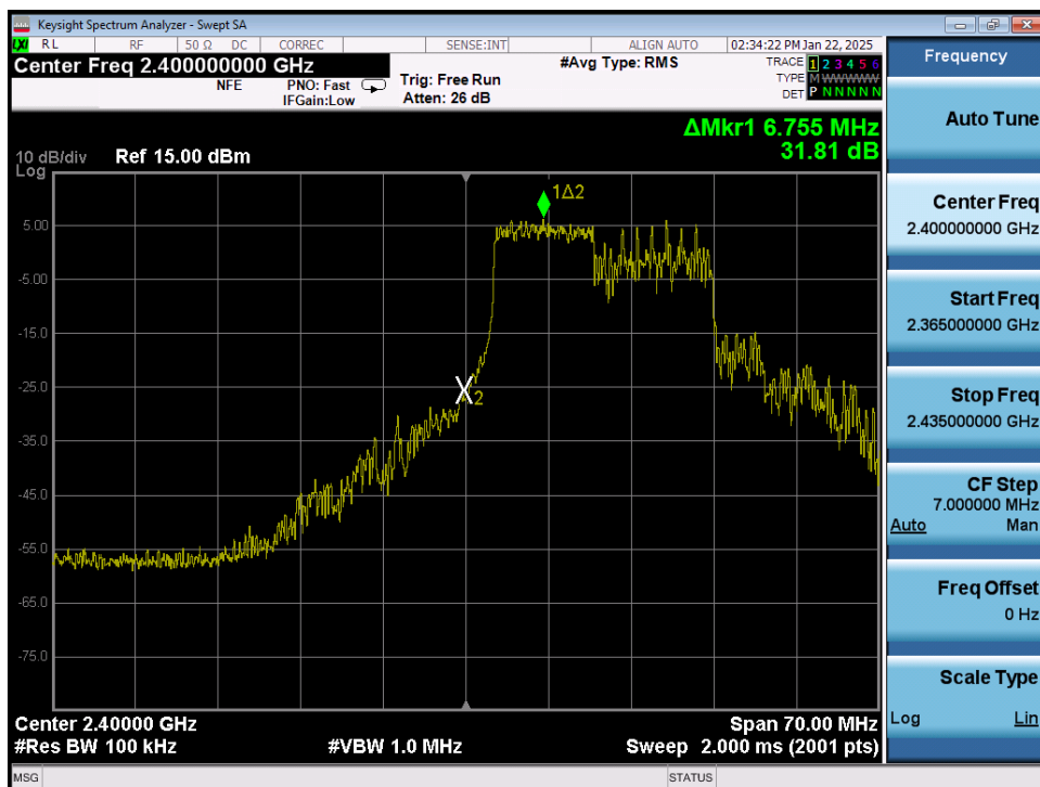
Plot 7-34. Band Edge Plot MIMO ANT2 (802.11ax OFDMA – 106 Tones – Ch. 1)
