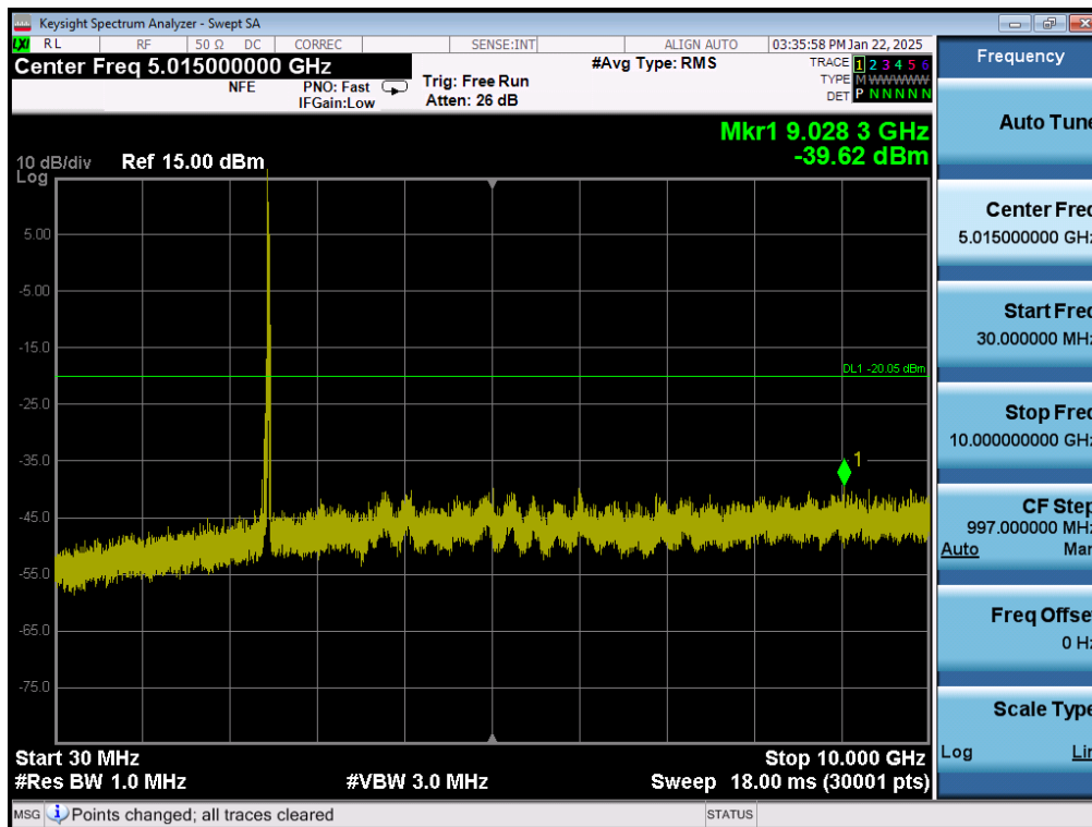
Plot 7-47. Conducted Spurious Plot MIMO ANT1 (802.11ax OFDMA – 26 Tones – Ch. 11)
