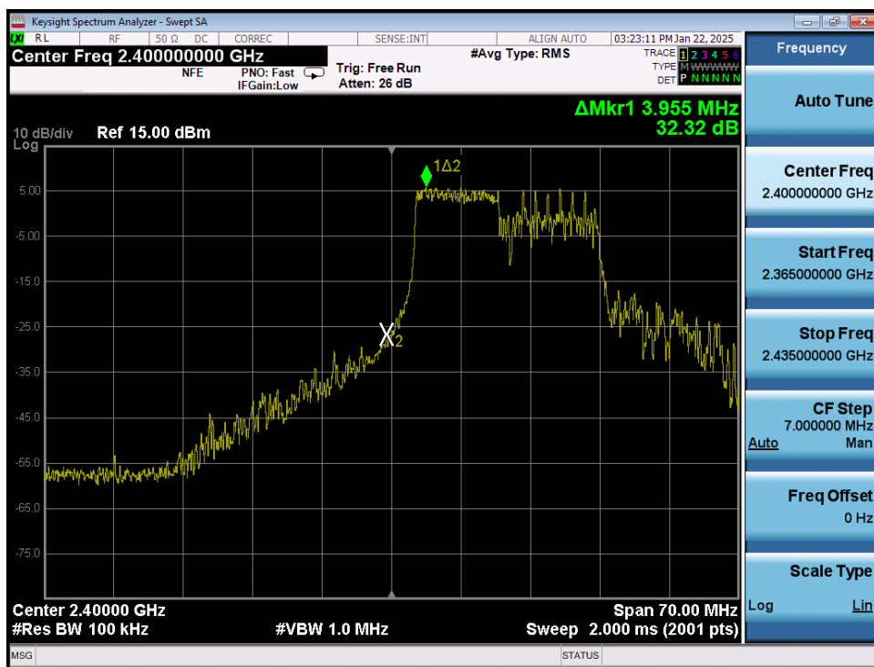
Plot 7-25. Band Edge Plot MIMO ANT1 (802.11ax OFDMA – 106 Tones – Ch. 1)
