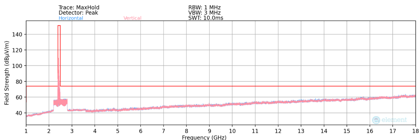
Plot 7-71. Radiated Spurious Plot above 1GHz MIMO (802.11ax OFDMA – 242 Tones – Ch. 1)
