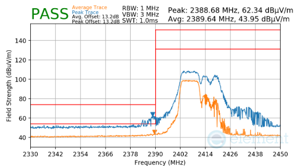
Plot 7-75. Radiated Restricted Lower Band Edge Measurement MIMO (Average and Peak – 106 Tones)
