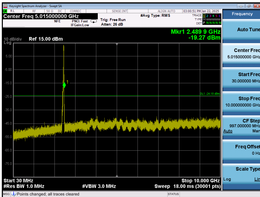
Plot 7-65. Conducted Spurious Plot MIMO ANT2 (802.11ax OFDMA – 242 Tones – Ch. 11)
