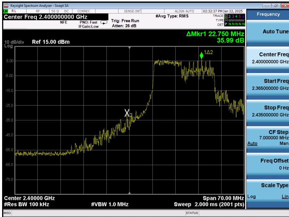
Plot 7-35. Band Edge Plot MIMO ANT2 (802.11ax OFDMA – 106 Tones – Ch. 2)
