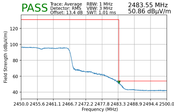
Plot 7-86. Radiated Restricted Upper Band Edge Measurement MIMO (Average – 242 Tones)
