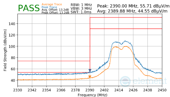
Plot 7-85. Radiated Restricted Lower Band Edge Measurement MIMO (Average and Peak – 242 Tones)
