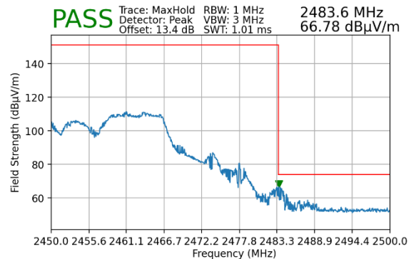
Plot 7-80. Radiated Restricted Upper Band Edge Measurement MIMO (Peak – 106 Tones)
