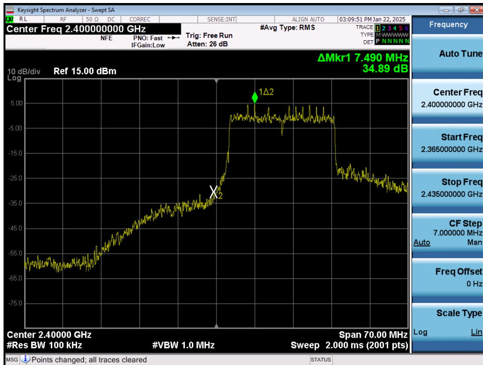
Plot 7-30. Band Edge Plot MIMO ANT1 (802.11ax OFDMA – 242 Tones – Ch. 1)
