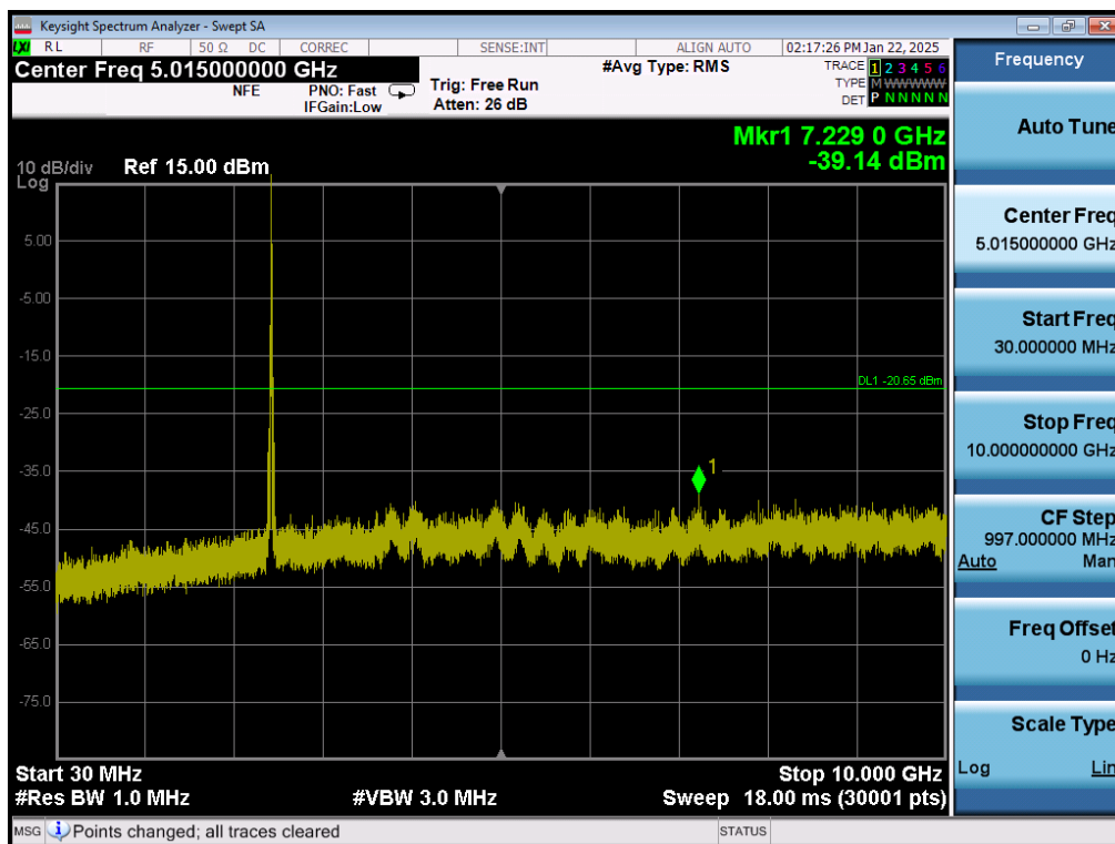
Plot 7-57. Conducted Spurious Plot MIMO ANT2 (802.11ax OFDMA – 26 Tones – Ch. 6)
