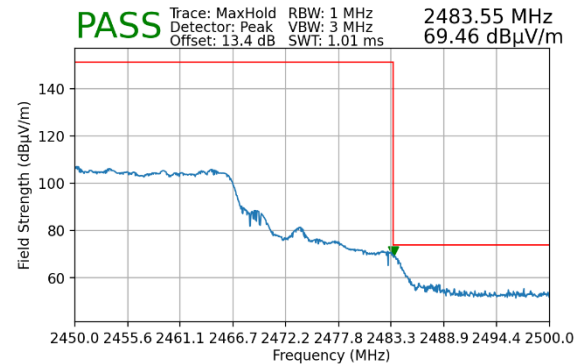
Plot 7-87. Radiated Restricted Upper Band Edge Measurement MIMO (Peak – 242 Tones)
