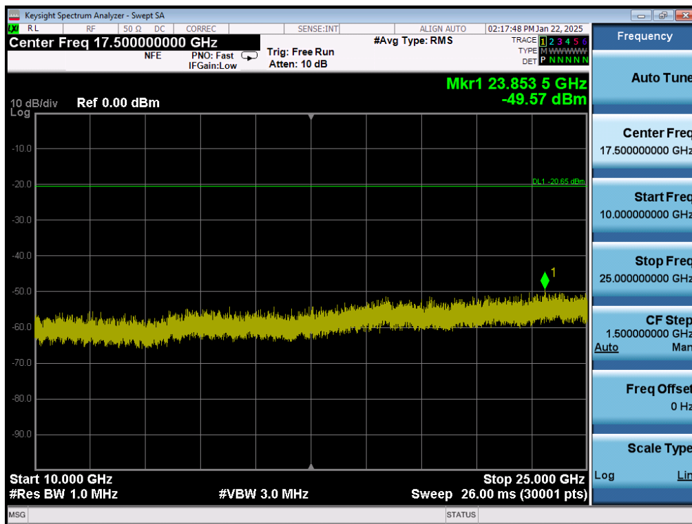
Plot 7-58. Conducted Spurious Plot MIMO ANT2 (802.11ax OFDMA – 26 Tones – Ch. 6)
