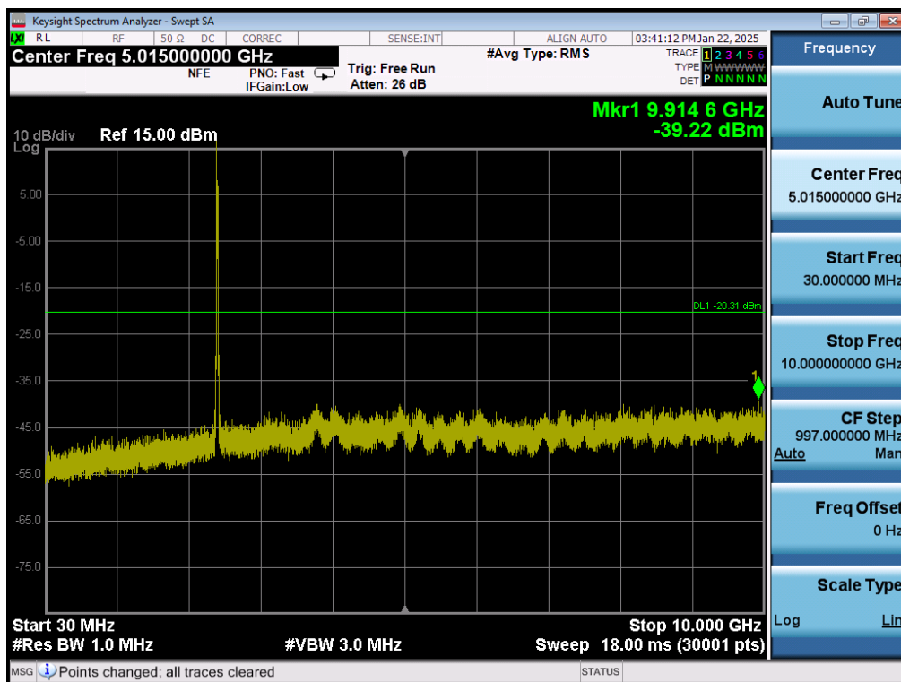
Plot 7-43. Conducted Spurious Plot MIMO ANT1 (802.11ax OFDMA – 26 Tones – Ch. 1)
