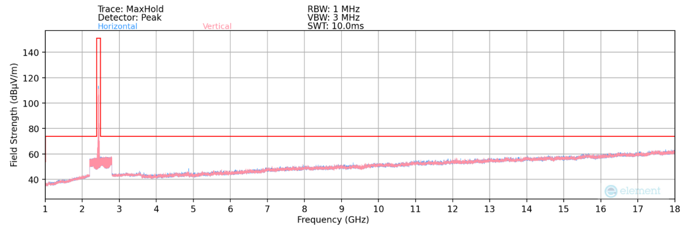
Plot 7-68. Radiated Spurious Plot above 1GHz MIMO (802.11ax OFDMA – 26 Tones – Ch. 6)
