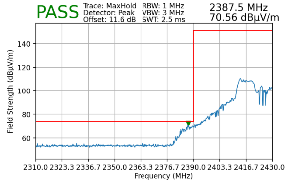
Plot 7-78. Radiated Restricted Lower Band Edge Measurement MIMO (Peak – 106 Tones)
