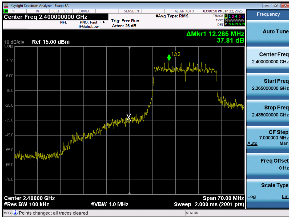
Plot 7-31. Band Edge Plot MIMO ANT1 (802.11ax OFDMA – 242 Tones – Ch. 2)
