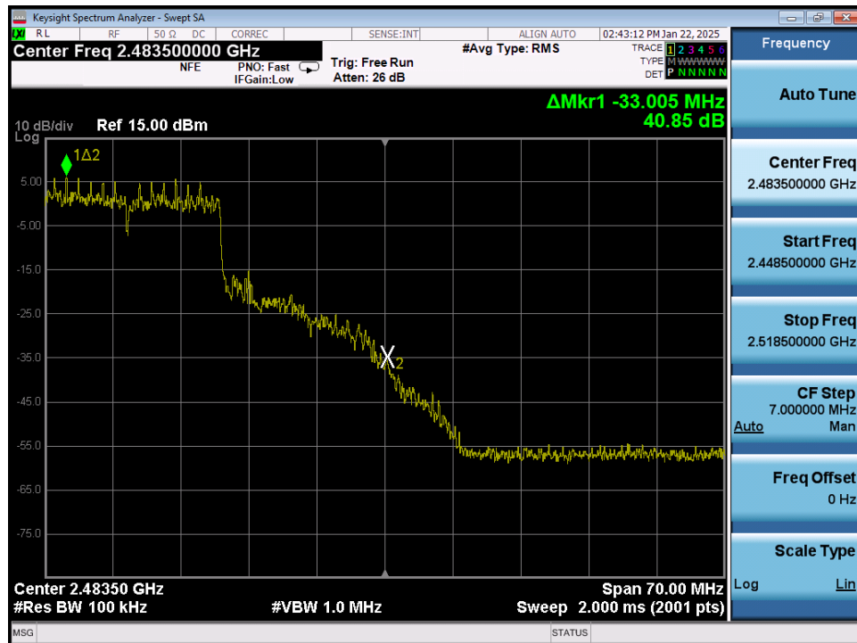
Plot 7-41. Band Edge Plot MIMO ANT2 (802.11ax OFDMA – 242 Tones – Ch. 10)
