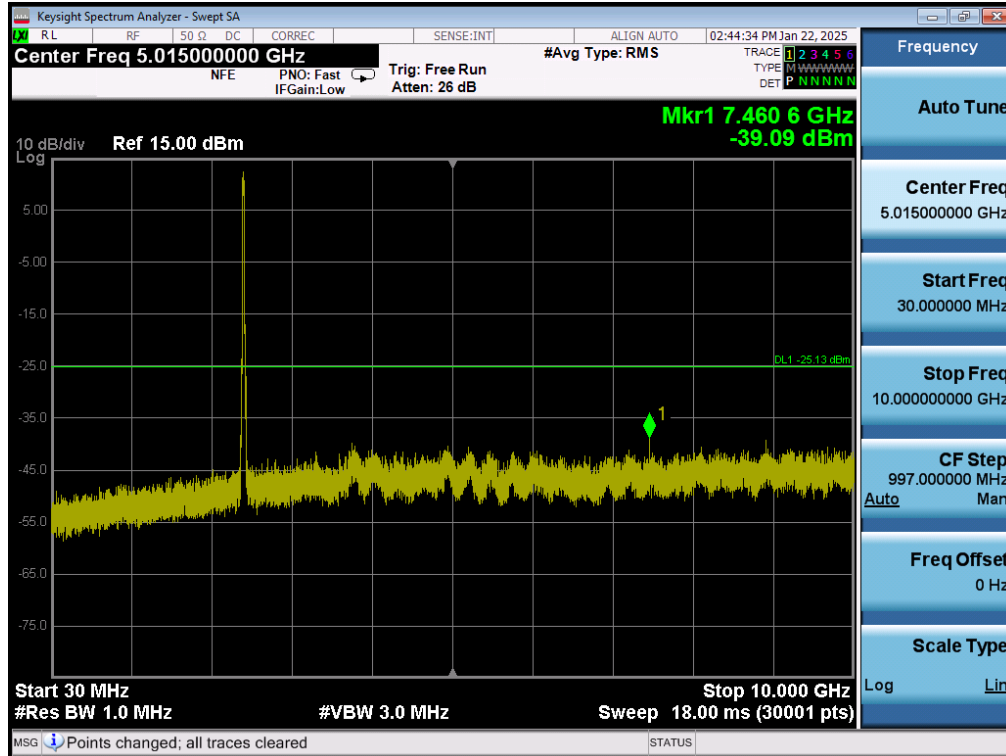
Plot 7-61. Conducted Spurious Plot MIMO ANT2 (802.11ax OFDMA – 242 Tones – Ch. 1)
