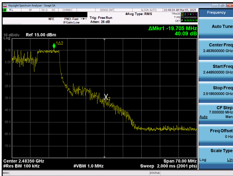
Plot 7-28. Band Edge Plot MIMO ANT1 (802.11ax OFDMA – 106 Tones – Ch. 10)
