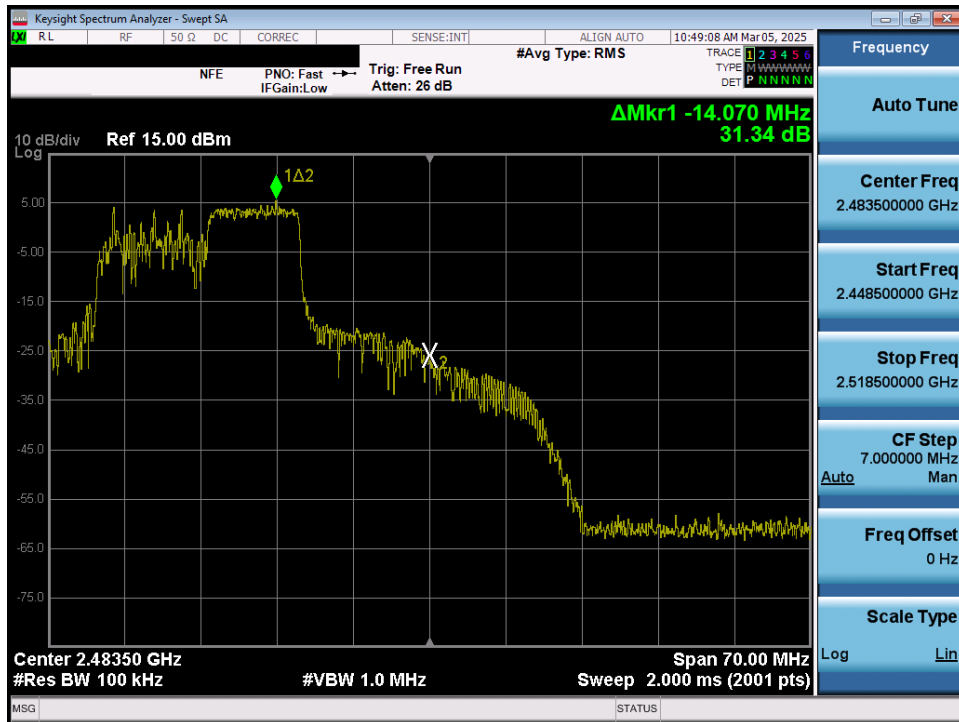
Plot 7-29. Band Edge Plot MIMO ANT1 (802.11ax OFDMA – 106 Tones – Ch. 11)
