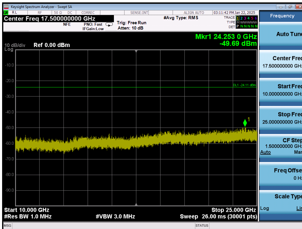
Plot 7-52. Conducted Spurious Plot MIMO ANT1 (802.11ax OFDMA – 242 Tones – Ch. 6)
