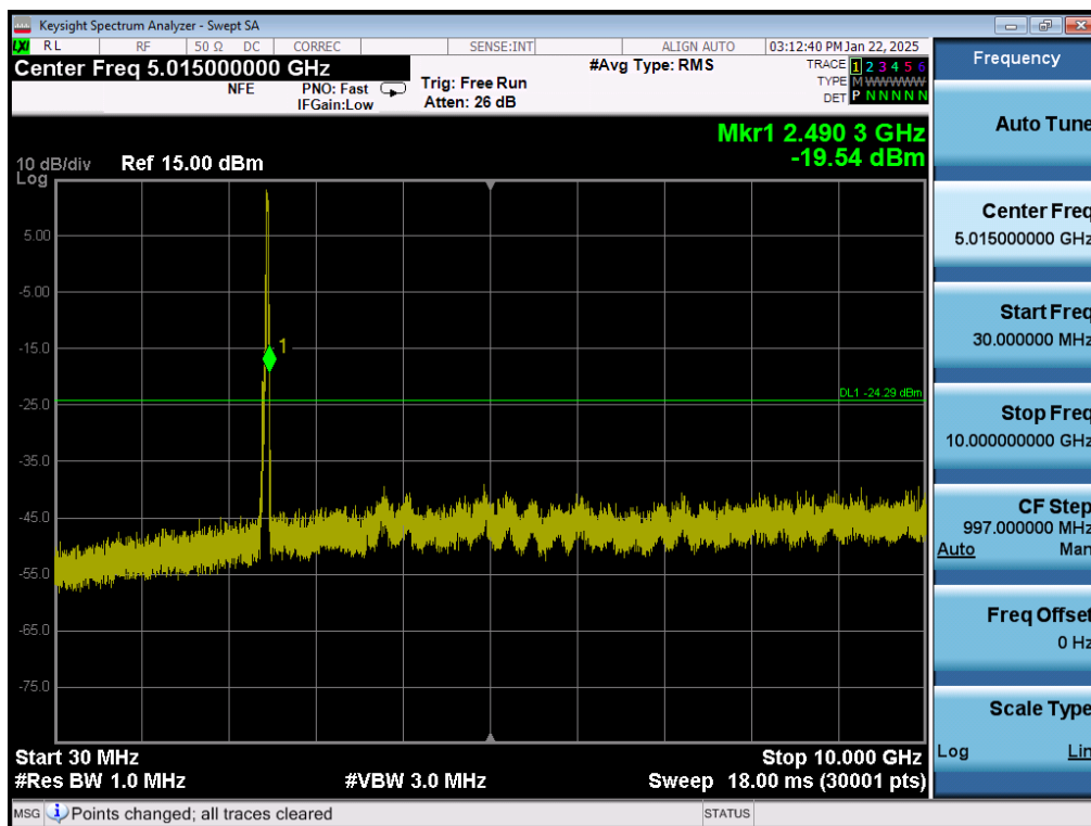
Plot 7-53. Conducted Spurious Plot MIMO ANT1 (802.11ax OFDMA – 242 Tones – Ch. 11)
