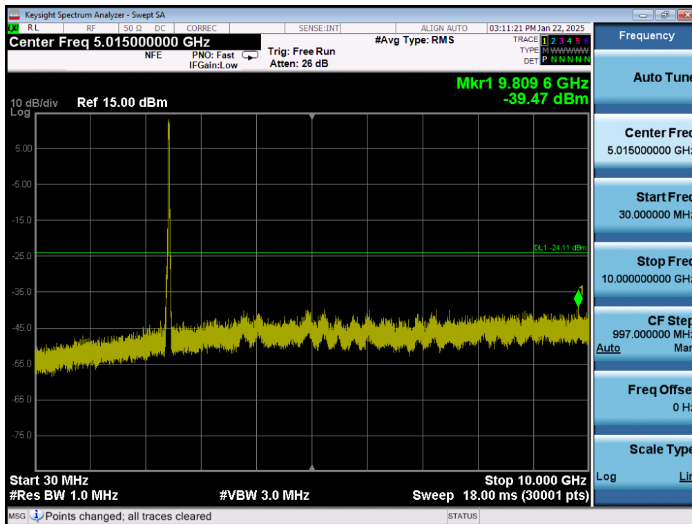
Plot 7-51. Conducted Spurious Plot MIMO ANT1 (802.11ax OFDMA – 242 Tones – Ch. 6)
