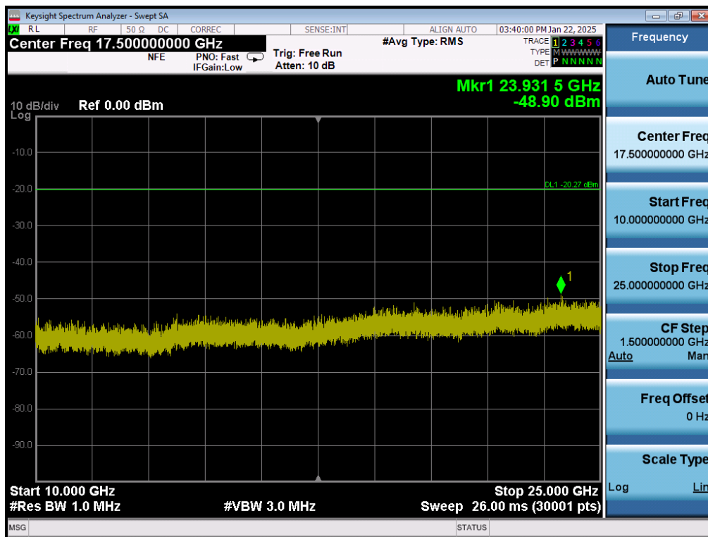
Plot 7-46. Conducted Spurious Plot MIMO ANT1 (802.11ax OFDMA – 26 Tones – Ch. 6)
