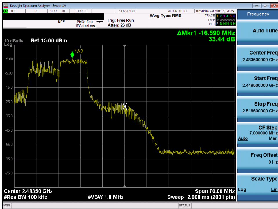
Plot 7-38. Band Edge Plot MIMO ANT2 (802.11ax OFDMA – 106 Tones – Ch. 11)
