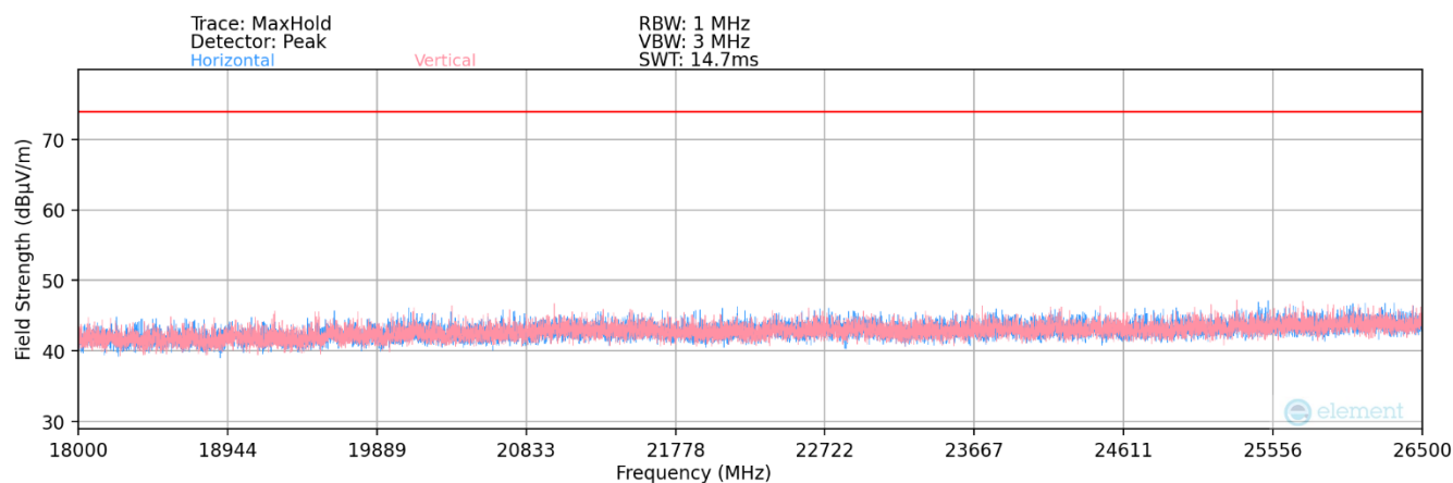
Plot 7-74. Radiated Spurious Plot above 18GHz MIMO (802.11ax OFDMA – 242 Tones)
