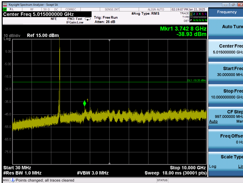
Plot 7-59. Conducted Spurious Plot MIMO ANT2 (802.11ax OFDMA – 26 Tones – Ch. 11)
