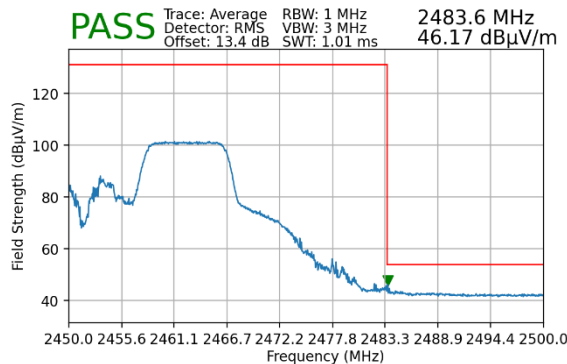
Plot 7-79. Radiated Restricted Upper Band Edge Measurement MIMO (Average – 106 Tones)
