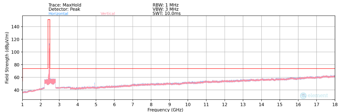
Plot 7-69. Radiated Spurious Plot above 1GHz MIMO (802.11ax OFDMA – 26 Tones – Ch. 11)
