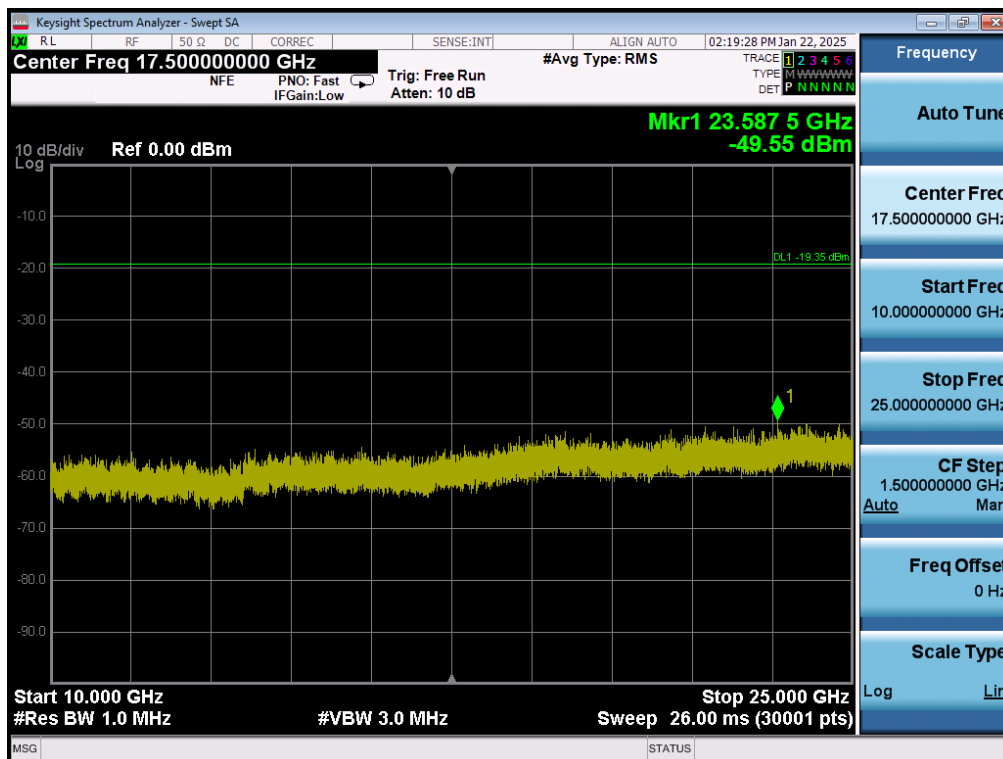
Plot 7-60. Conducted Spurious Plot MIMO ANT2 (802.11ax OFDMA – 26 Tones – Ch. 11)
