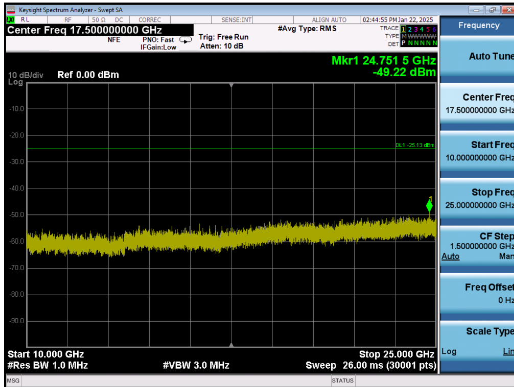
Plot 7-62. Conducted Spurious Plot MIMO ANT2 (802.11ax OFDMA – 242 Tones – Ch. 1)
