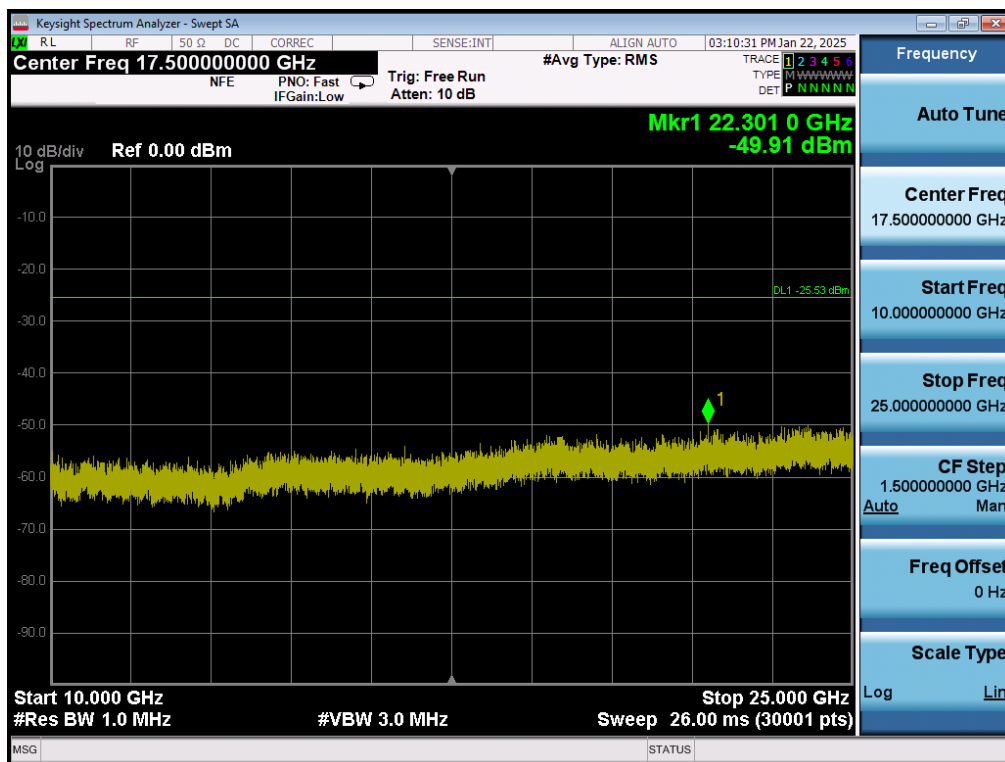
Plot 7-50. Conducted Spurious Plot MIMO ANT1 (802.11ax OFDMA – 242 Tones – Ch. 1)
