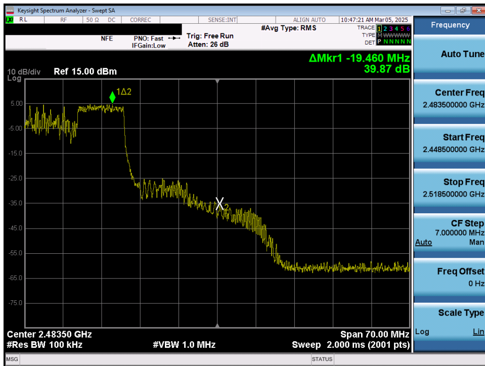
Plot 7-37. Band Edge Plot MIMO ANT2 (802.11ax OFDMA – 106 Tones – Ch. 10)
