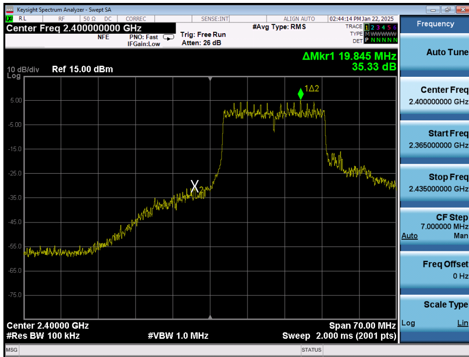
Plot 7-39. Band Edge Plot MIMO ANT2 (802.11ax OFDMA – 242 Tones – Ch. 1)
