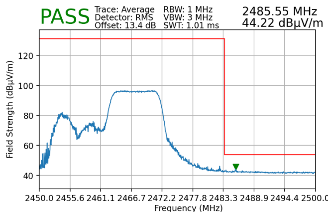
Plot 7-81. Radiated Restricted Upper Band Edge Measurement MIMO (Average – 106 Tones)
