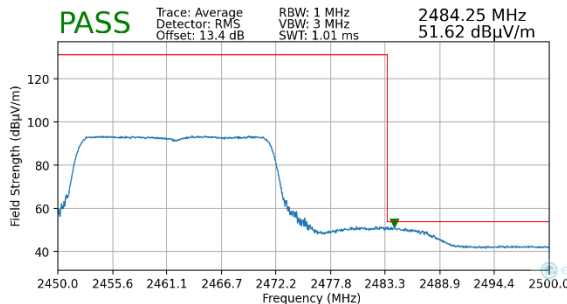
Plot 7-88. Radiated Restricted Upper Band Edge Measurement MIMO (Average – 242 Tones)
