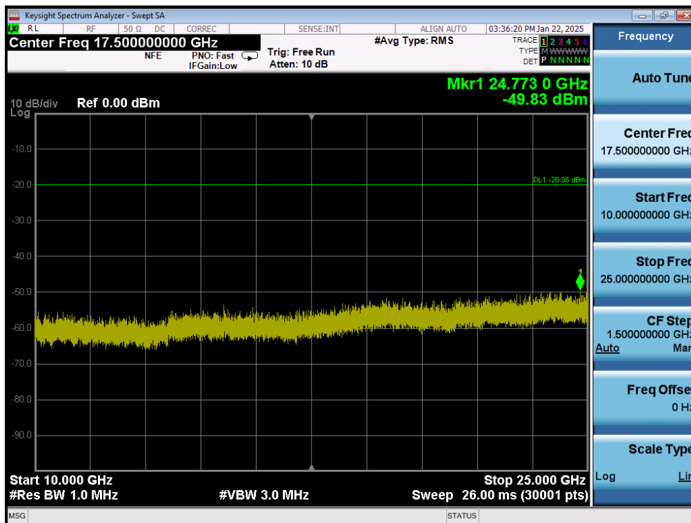
Plot 7-48. Conducted Spurious Plot MIMO ANT1 (802.11ax OFDMA – 26 Tones – Ch. 11)
