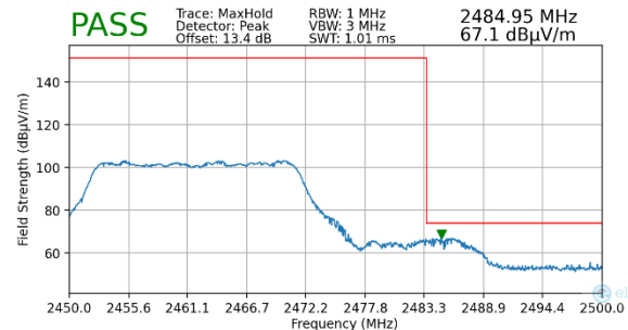
Plot 7-89. Radiated Restricted Upper Band Edge Measurement MIMO (Peak – 242 Tones)
