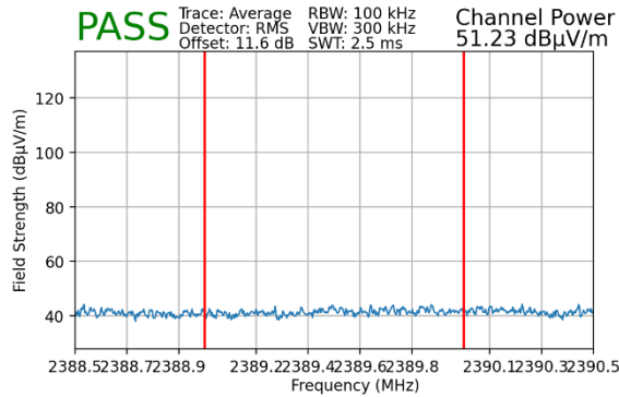
Plot 7-77. Radiated Restricted Lower Band Edge Measurement MIMO (Average – 106 Tones)
