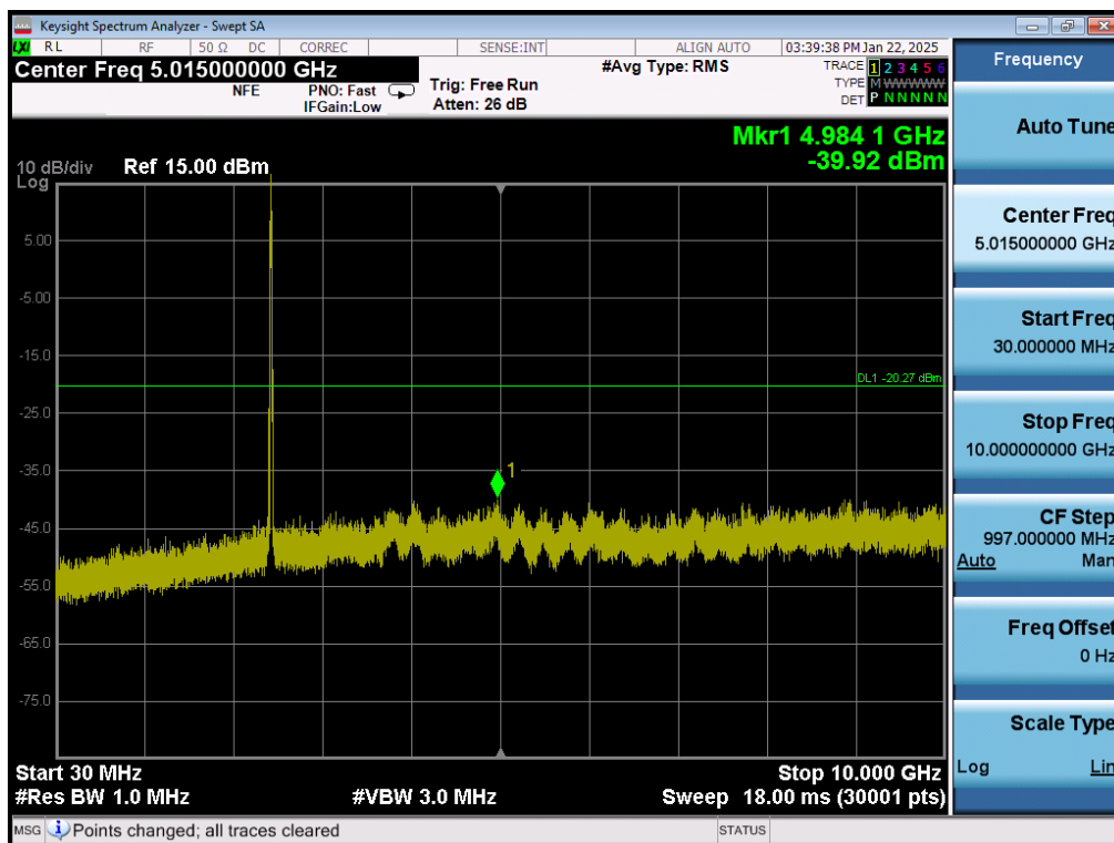
Plot 7-45. Conducted Spurious Plot MIMO ANT1 (802.11ax OFDMA – 26 Tones – Ch. 6)
