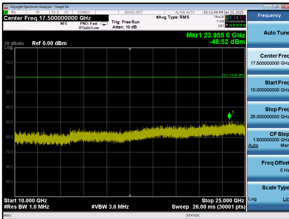
Plot 7-56. Conducted Spurious Plot MIMO ANT2 (802.11ax OFDMA – 26 Tones – Ch. 1)
