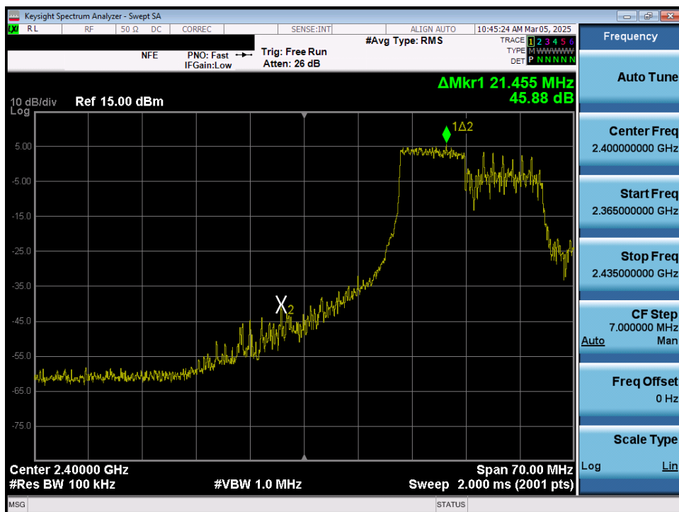
Plot 7-27. Band Edge Plot MIMO ANT1 (802.11ax OFDMA – 106 Tones – Ch. 3)
