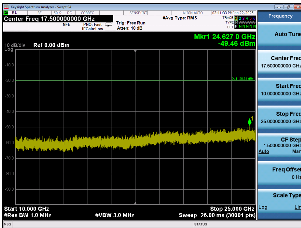
Plot 7-44. Conducted Spurious Plot MIMO ANT1 (802.11ax OFDMA – 26 Tones – Ch. 1)
