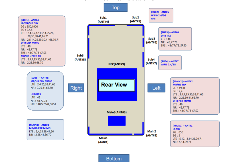
Figure J-1 DUT Antenna Locations
