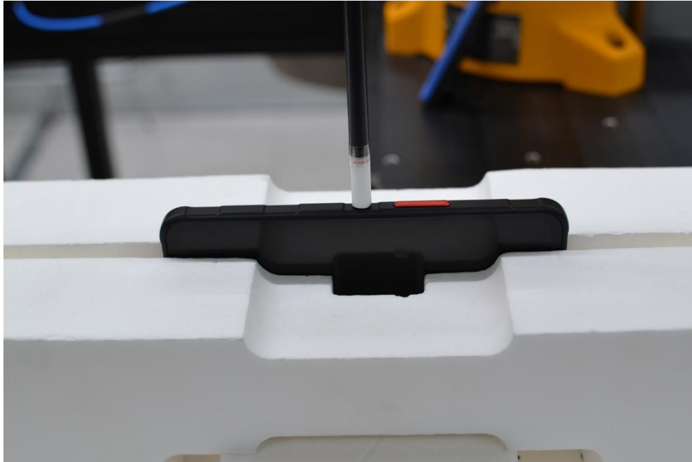
SAR Test Setup Photo 23 – PD, Left Edge at 2mm
