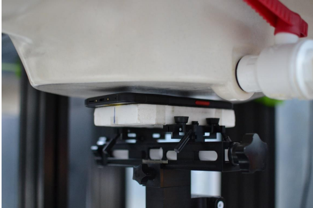
SAR Test Setup Photo 5 – Body-worn and Hotspot, Back Side at 5mm
