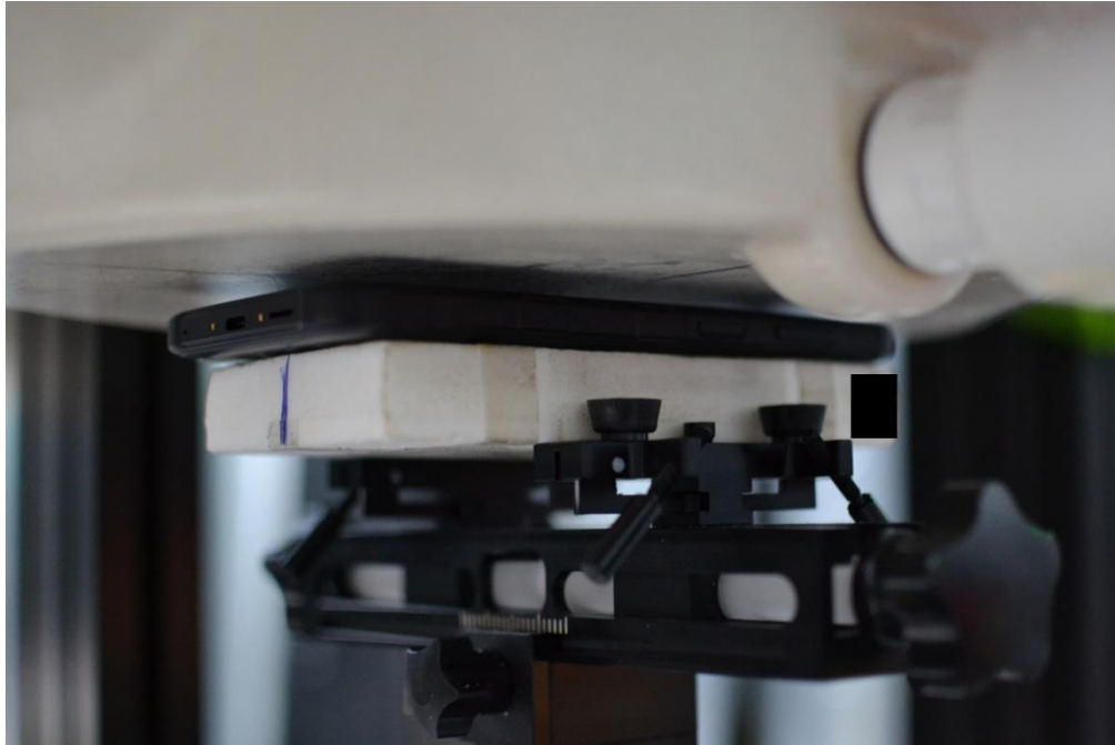
SAR Test Setup Photo 7 – Hotspot, Front Side at 5mm
