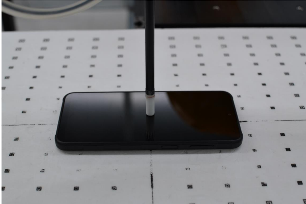
SAR Test Setup Photo 21 – PD, Front Side at 2mm
