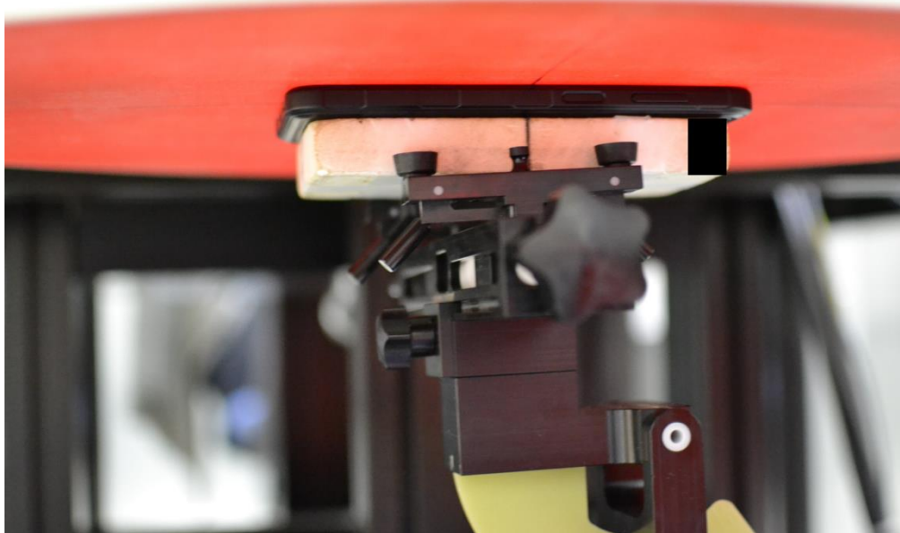
SAR Test Setup Photo 16 – NFC, Phablet, Front Side at 0mm
