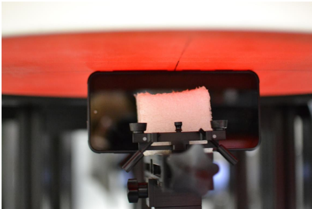
SAR Test Setup Photo 18 – NFC, Phablet, Right Edge at 0mm
