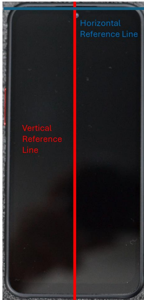
SAR Test Setup Photo 24 – Reference Lines
