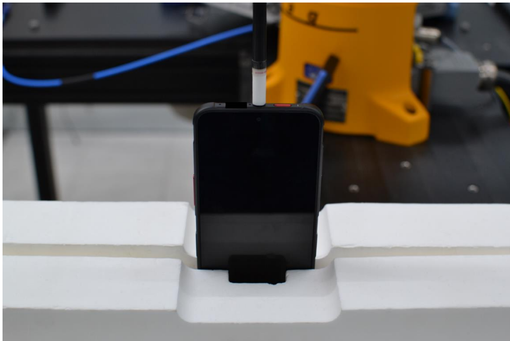
SAR Test Setup Photo 22 – PD, Top Edge at 2mm
