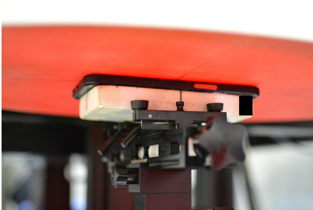
SAR Test Setup Photo 15 – NFC, Phablet, Back Side at 0mm
