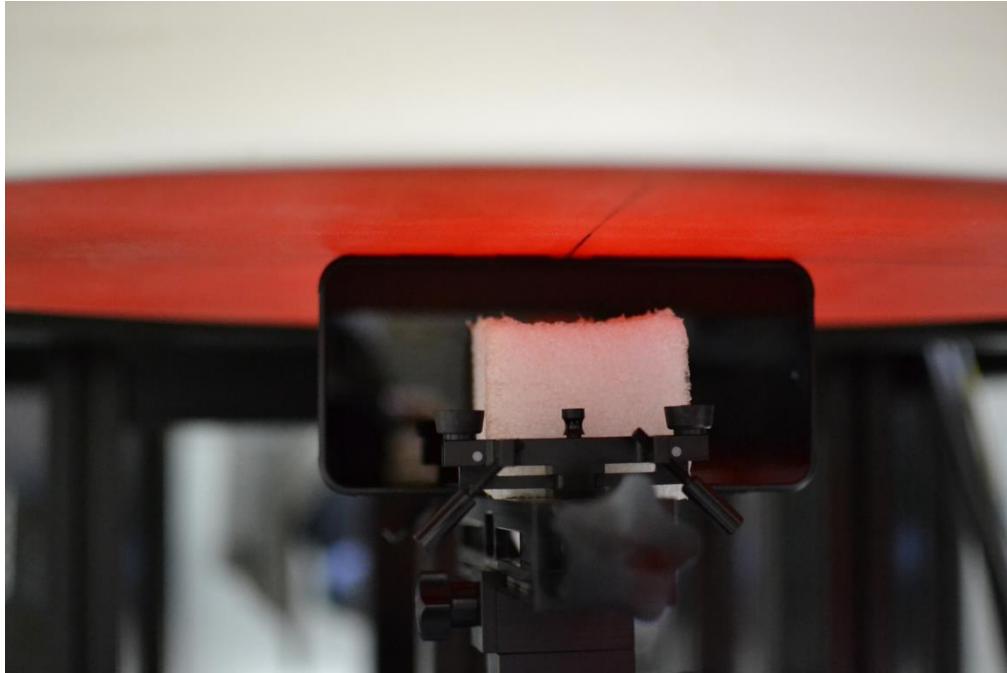
SAR Test Setup Photo 17 – NFC, Phablet, Left Edge at 0mm
