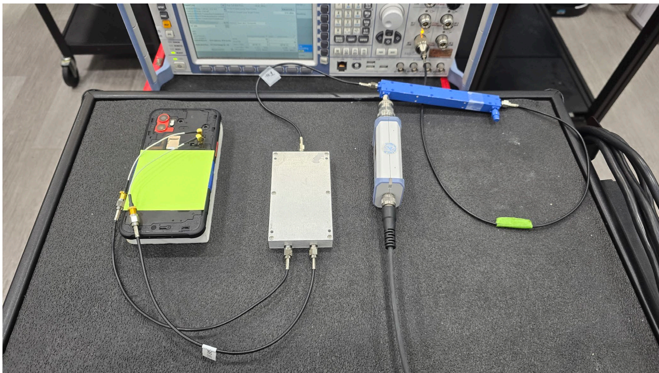
Test Setup Photo 6 – Conducted Test Setup (Figure 5-1b)
