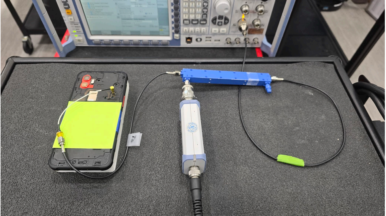
Test Setup Photo 1 – Conducted Test Setup (Figure 5-1a)
