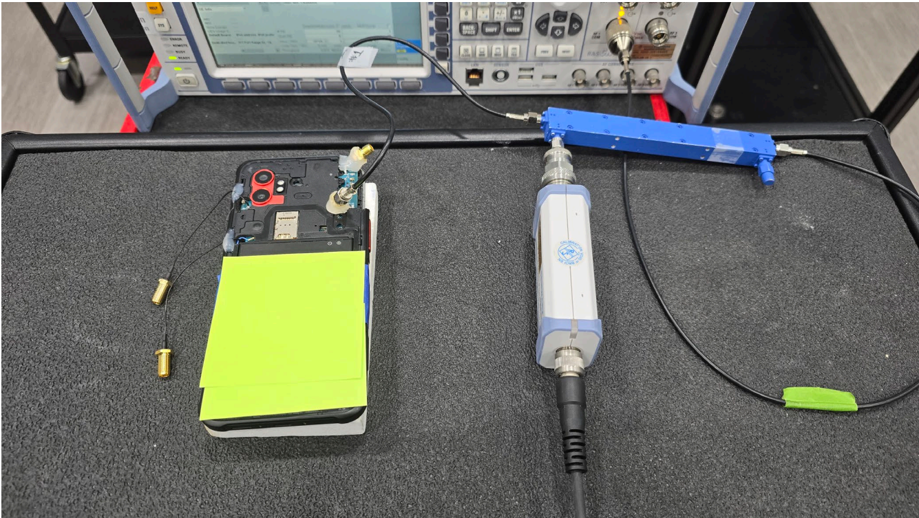
Test Setup Photo 10 – Conducted Test Setup (Figure 5-1a)
