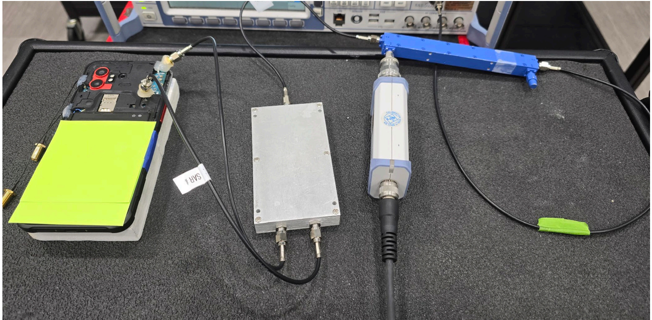
Test Setup Photo 11 – Conducted Test Setup (Figure 5-1b)
