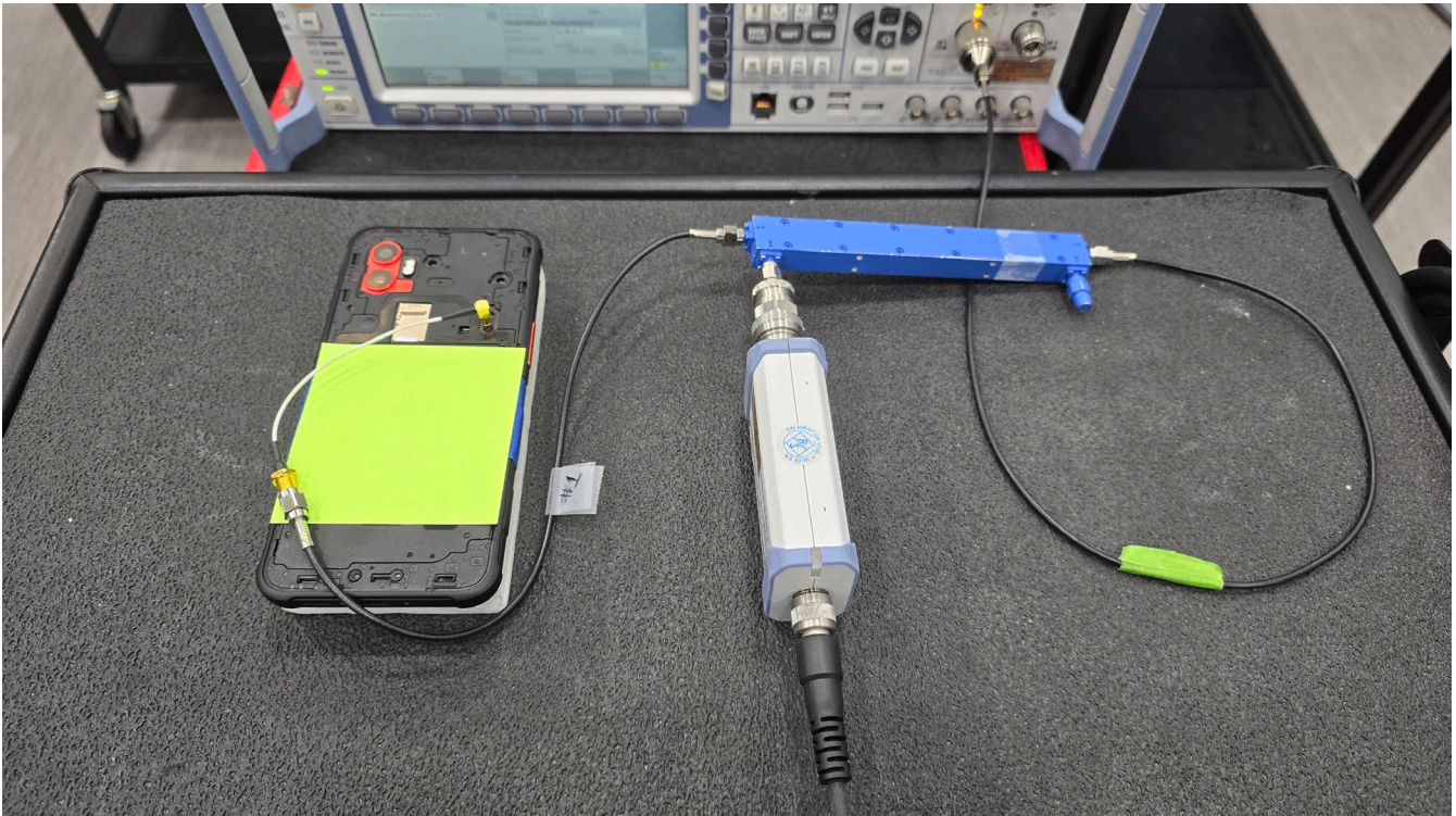
Test Setup Photo 2 – Conducted Test Setup (Figure 5-1a)
