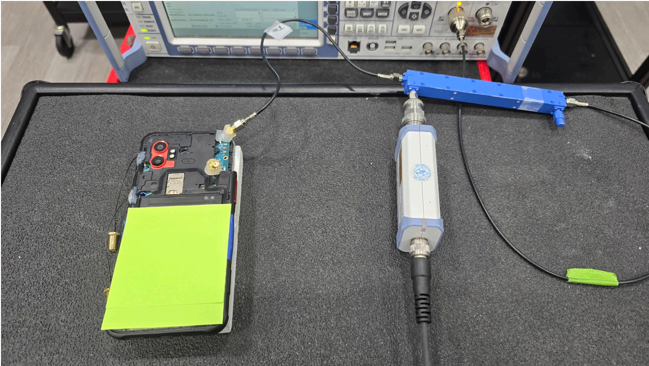
Test Setup Photo 9 – Conducted Test Setup (Figure 5-1a)
