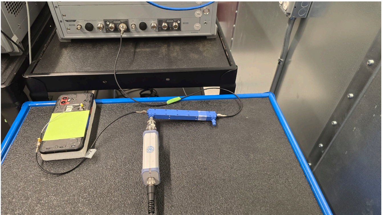
Test Setup Photo 4 – Conducted Test Setup (Figure 5-1a)
