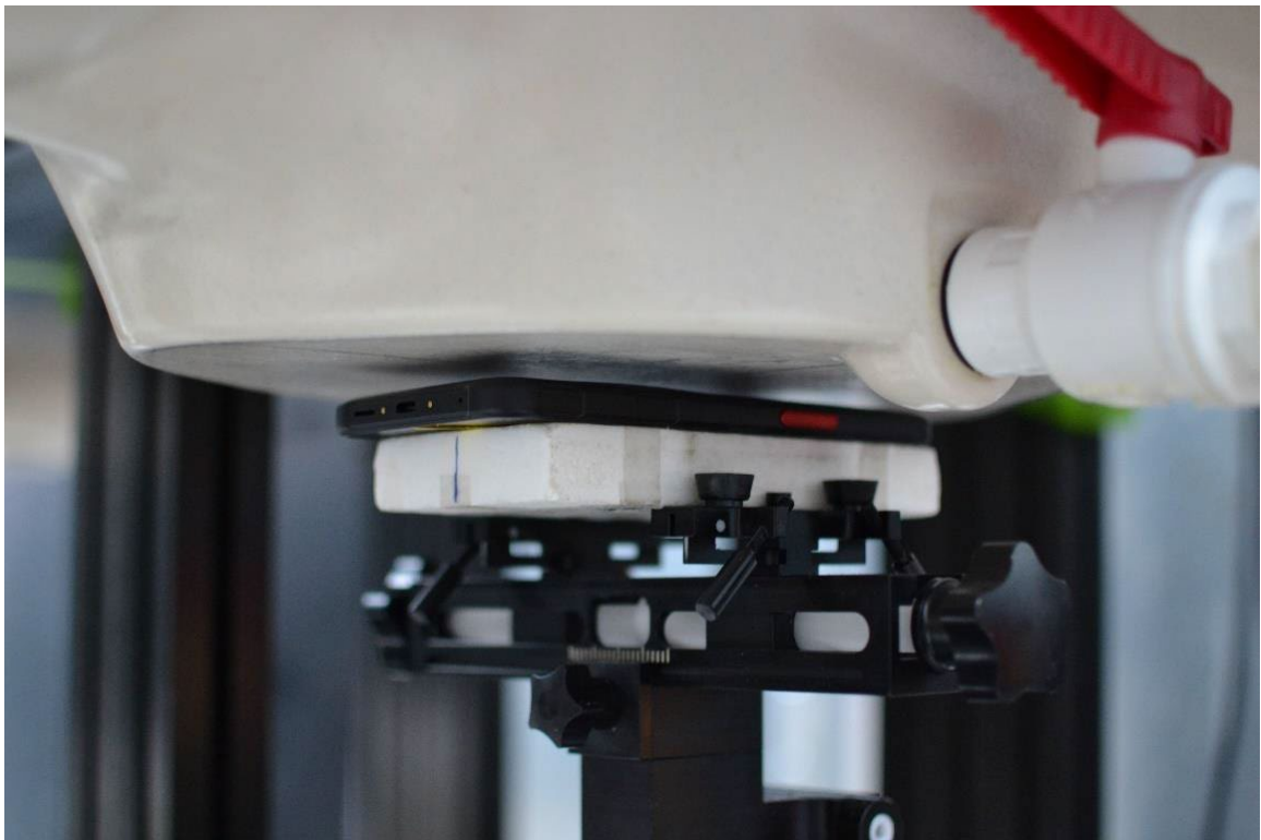
Test Setup Photo 14 – Radiated SAR, Back Side at 5mm
